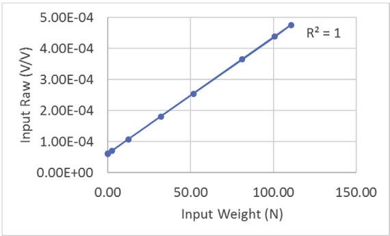
Fig. 9. Load cell number 1 calibration curve.
