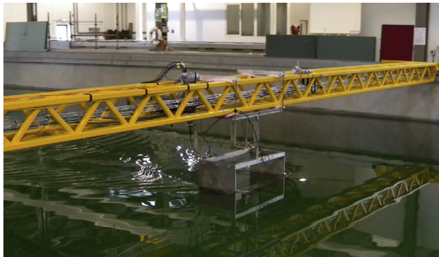
Fig. 3. View of the towing bridge and profile holding structure.
