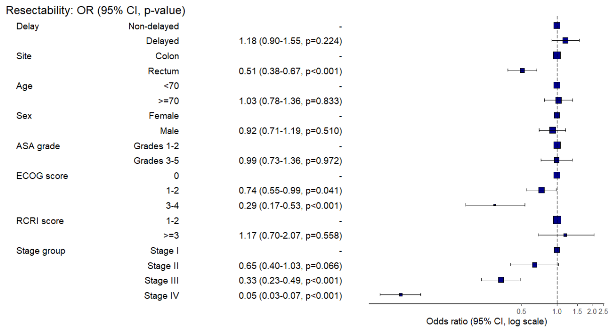
Figure 2: Multivariate logistic regression model exploring the association between delay to surgery and resectability, adjusting for patient and disease factors.
