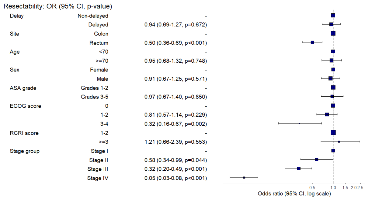
Supplementary Figure 2: Multivariate logistic regression model exploring the association between delay to surgery and resectability for patients receiving elective surgery, adjusting for patient and disease factors.
