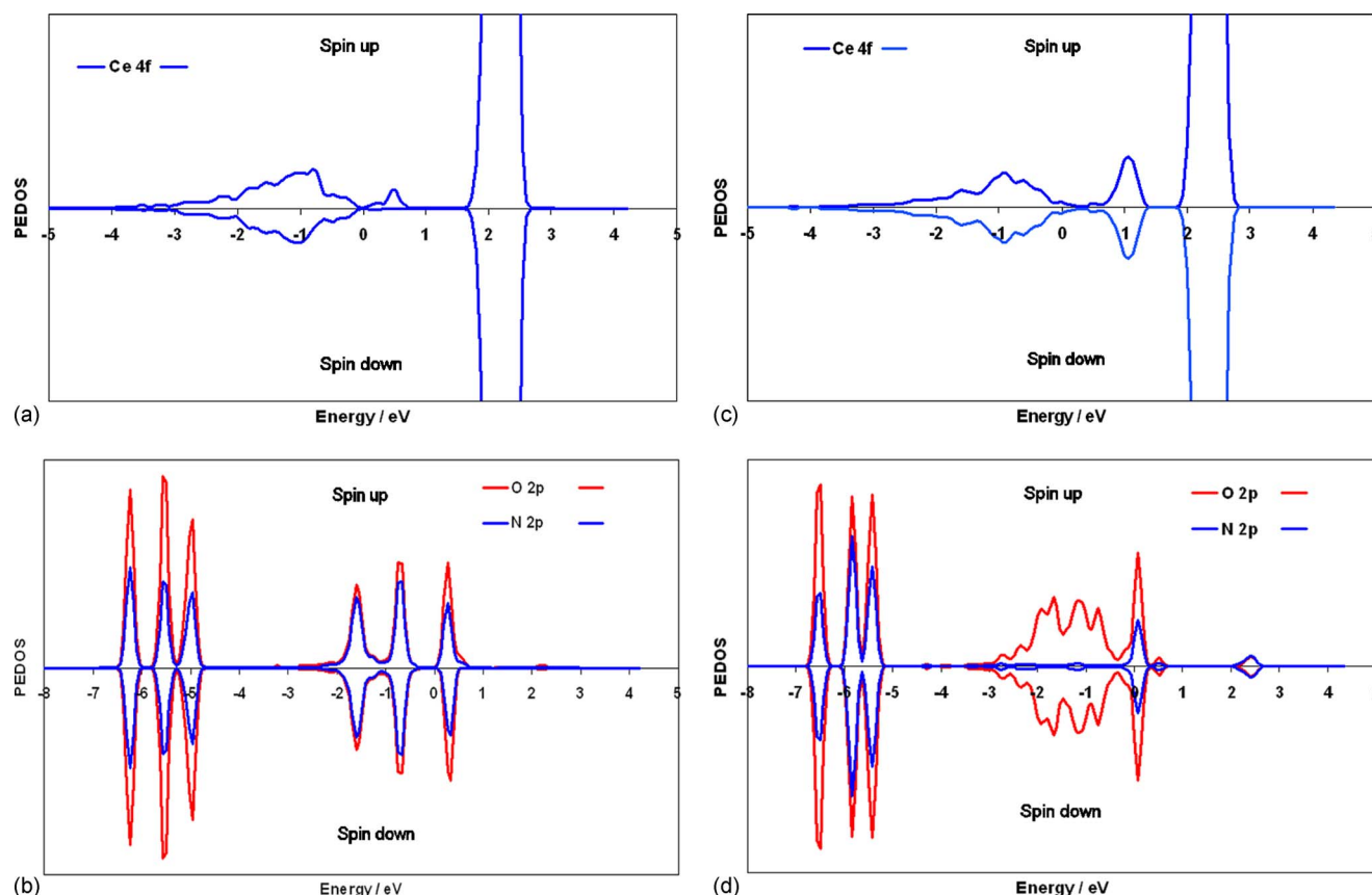
FIG. 7. (Color online) (a) Ce 4 f PEDOS for NO 2 adsorbed on the Au-doped (110) surface, (b) N and O 2 p PEDOS for NO 2 adsorbed on the Au-doped (110) surface, (c) Ce 4 f PEDOS for NO 2 adsorbed on the Au-doped (100) surface, and (d) N and O 2 p PEDOS for NO 2 adsorbed on the Au-doped (100) surface
