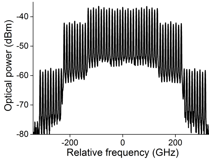
Figure 2.15: Optical spectrum of the 45 line comb generated using the hybrid comb source. First stage composed of the 9 line comb generated by the multi-harmonic comb generator, second stage composed of two cascaded modulators
