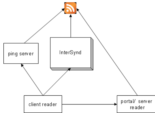
Figure 1. Syndication Middleware
