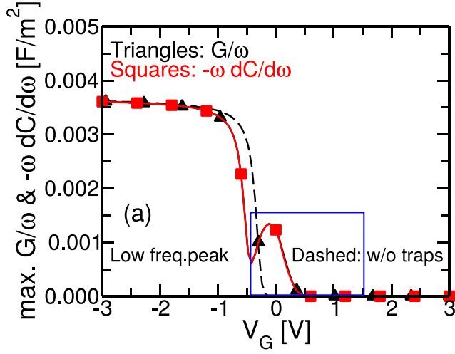
Figure 6. Simulations of the MOS structure in Figs. 1 including the Gaussian DIT profile shown in Figure 5. The peak value of G/\omega and -\omega dC/d\omega versus V_G is shown in (a) and its frequency position in (b). The dashed lines are the simulations results without traps and the blue box indicates the low frequency peak.
