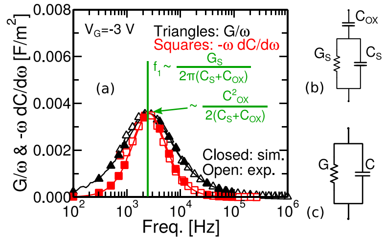
Figure 11. (a) Simulated (closed) and experimental (open) curves at V_G = -3 \text{ V} of G/\omega (triangles) and -\omega dC/d\omega (squares) plotted as a function of frequency. (b) Equivalent electrical circuit of a MOS structure interpreted using a parallel G-C circuit (c).
