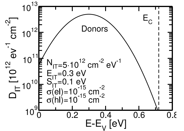
Figure 5. DIT profile of donor traps included in the simulations of Figure 6. The energy is referred to the valence band of InGaAs. The figure reports also the parameter used for the Gaussian distribution and the values of the capture cross section for electron and holes.
