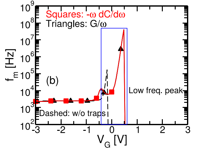
Figure 6. Simulations of the MOS structure in Figs. 1 including the Gaussian DIT profile shown in Figure 5. The peak value of G/\omega and -\omega dC/d\omega versus V_G is shown in (a) and its frequency position in (b). The dashed lines are the simulations results without traps and the blue box indicates the low frequency peak.
