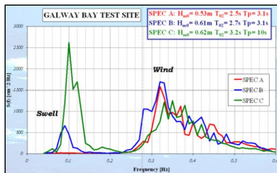
Figure 6. Bimodal Spectra
