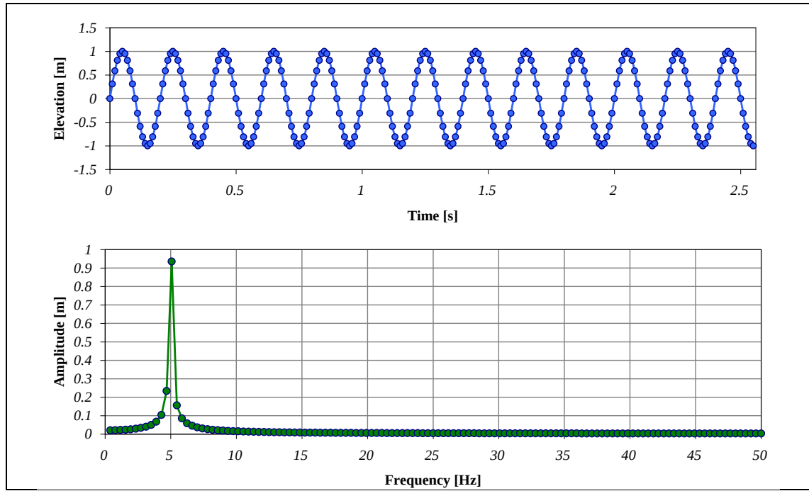
Figure 3.4. Sinusoidal waveform and corresponding frequency spectrum.
