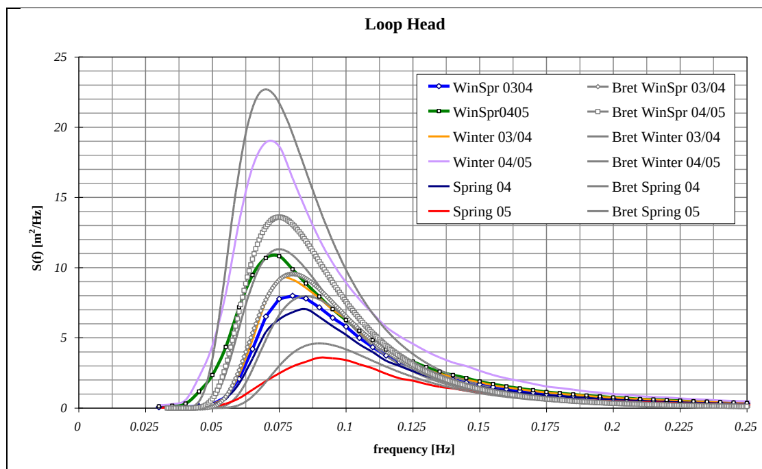
Figure 4.21. Comparison of average spectra and Bretschneider fit.
