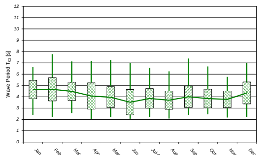
Figure 8. 2007 Monthly Averages, Standard Deviations, Minima and Maxima of Average Wave Period, T_{02} .
