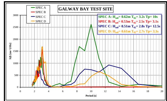
Figure 16: Examples of measured multi-peaked spectra.
