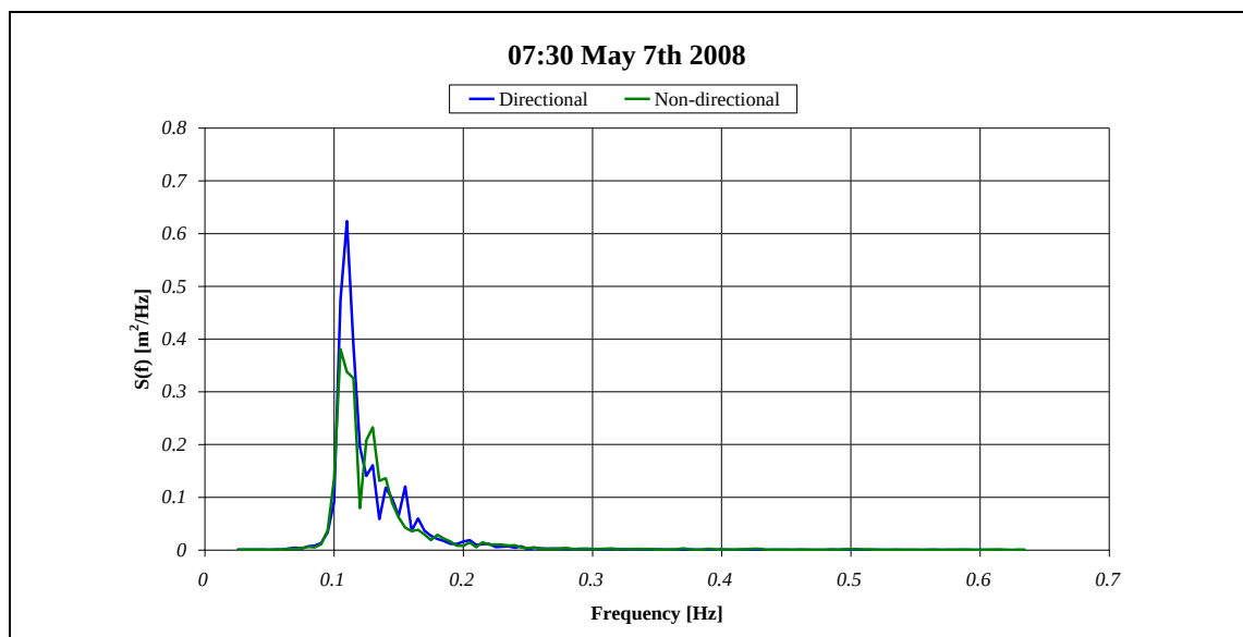
Figure 4.42. Spectra with long average period, T_{02} .
