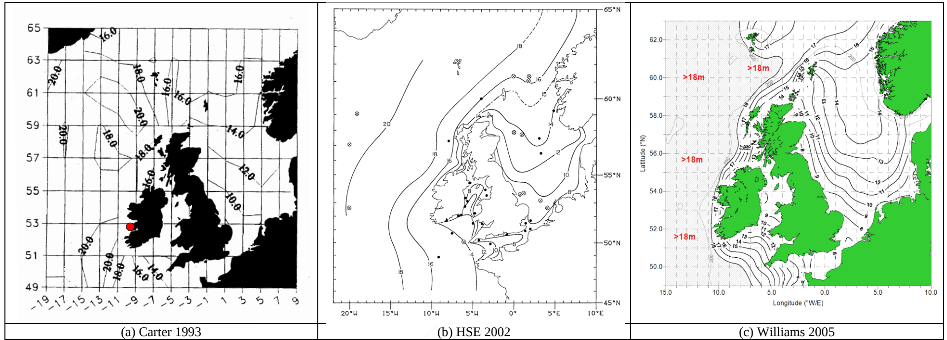
Figure 5.2. 50 year (a & b) and 100 year (c) return values of H_s for North Atlantic.
