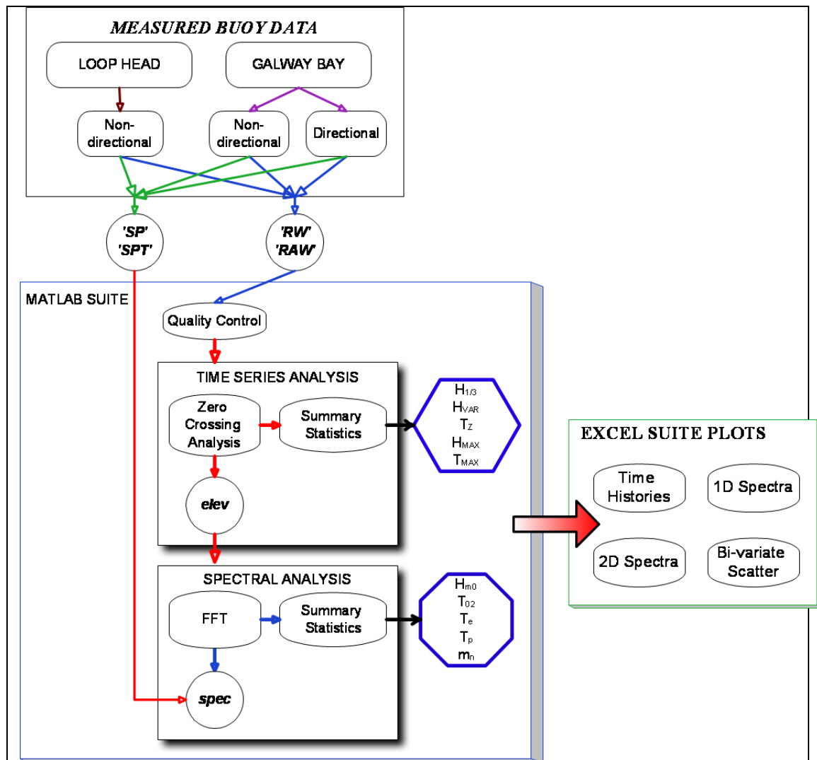
Figure 2.17. Work flow diagram depicting the quality check and analysis procedures for the data sets.
