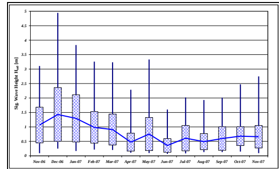
Figure 3. H_{m0} Statistics
