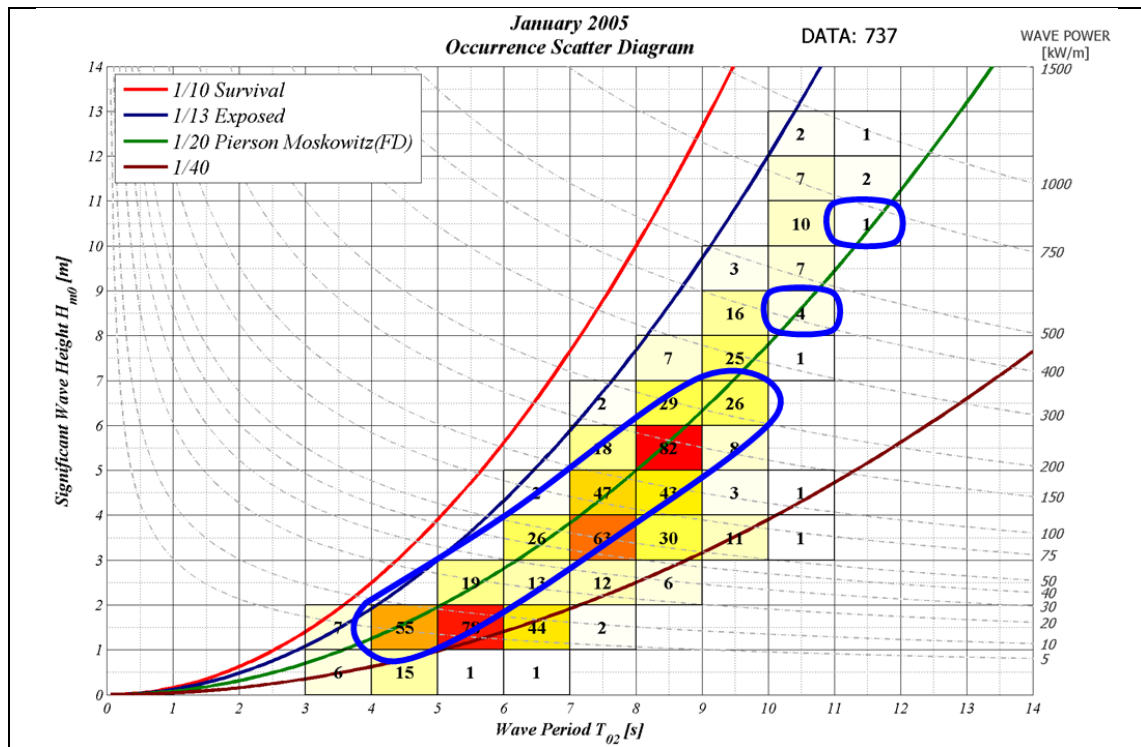
Figure 4.32. January 2005 bi-variate scatter diagram with selected iso-steepness components.
