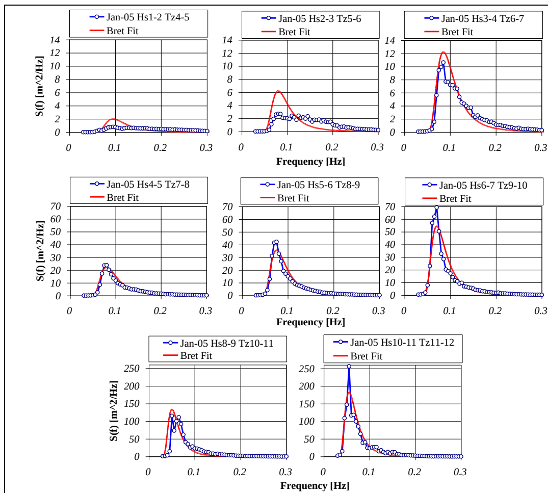
Figure 4.33. Average spectra and Bretschneider fit for iso-steepness scatter elements of Figure 4.32.
