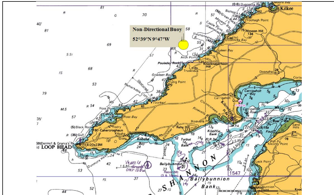
Figure 1.14. Location of non-directional buoy off Loop Head.
