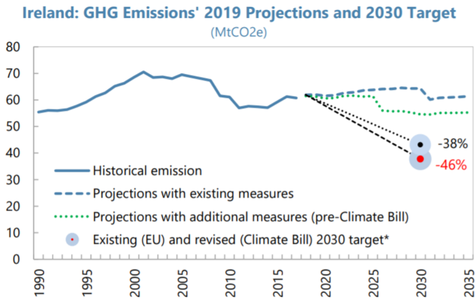
Figure 1: Ireland's GHG emissions and target. 1
