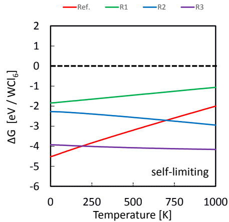
Figure S8: FEPs of the reactions in given in Table S3.
