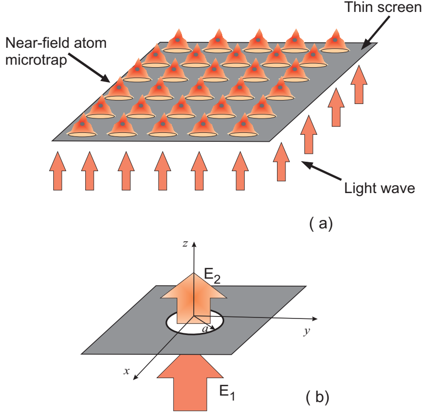
FIG. 1: (a) An array of atom microtraps produced by diffracted optical near-fields; (b) Schematic of a single microtrap formed by a circular aperture of radius a . E_1 represents the incoming light field and E_2 the diffracted near-field.
