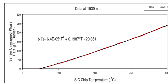
Fig. 3. Sensor Unwrapped Phase Data \phi(T) in Radians versus SiC Chip Temperature (°C) with data taken at 1530 nm. A weak quadratic curve fit is achieved for this data.
