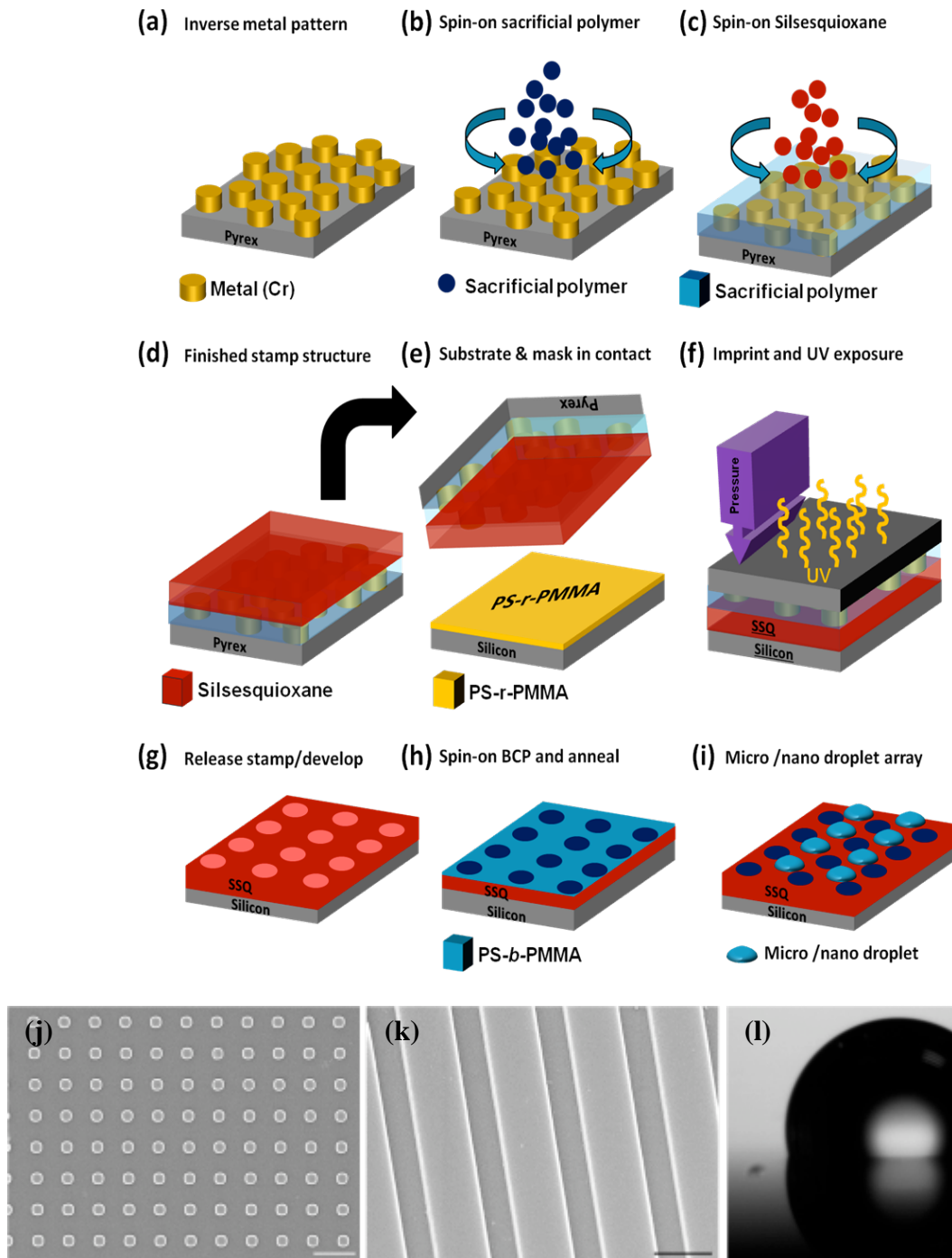
Figure 1: (a)-(i) schematic 3-D diagram process flow for creating patterned PSSQ films by RUV-NIL technique. Top down SEM images of NIL prepared PSSQ (j) via hole arrays and (k) line arrays prior to block copolymer deposition and dewetting and (l) Optical image of contact angle \sim 100^\circ measured on a planar PSSQ surface post UV curing. The scale bars in images (j) and (k) are 2 micron and 1 micron respectively.
