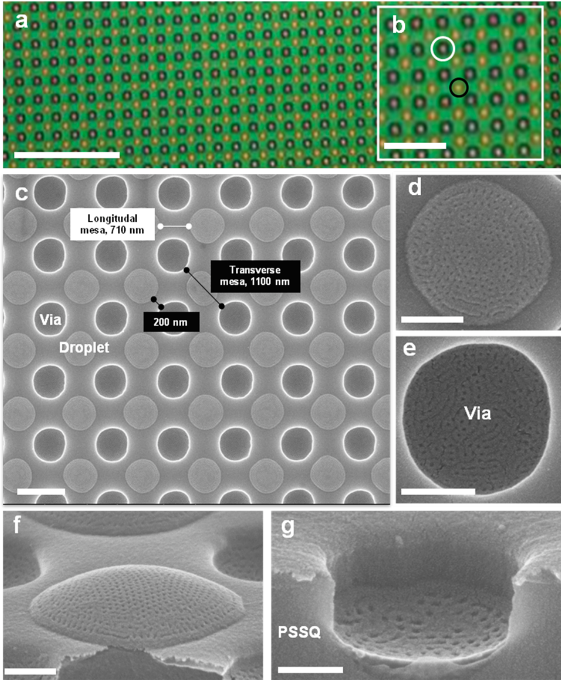
Figure 3: (a), (b) Optical microscopy and (c) SEM images of an extremely regular array of \sim 675 nm micro-droplets forming atop of the transverse mesas between the 600 nm via holes as a result of dewetting processes for a 1% wt. PS-PMMA (46-21 kg/mol) (d) and (e) SEM images of microphase separation within the micro-droplet on the mesa and within the via hole (reservoir) taken from image d. (f) and (g) 70° tilt SEM images of microphase separation within a micro-droplet on PSSQ mesas and via holes. The scale bars are as follows: (a) 10 micron, (b) 4 micron, (c) 1000 nm, (d) 300 nm, (e) 300 nm, (f) 250 nm, (g) 150 nm.
