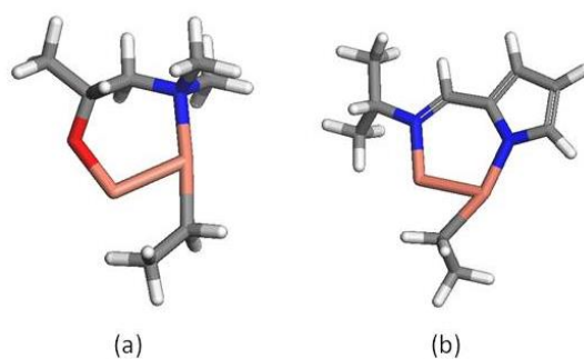
Figure 16: \text{Cu}_2\text{LEt} compounds where (a) \text{L}=\text{dmap} and (b) \text{L}=\text{PyrIm}^{\text{iPr}}
