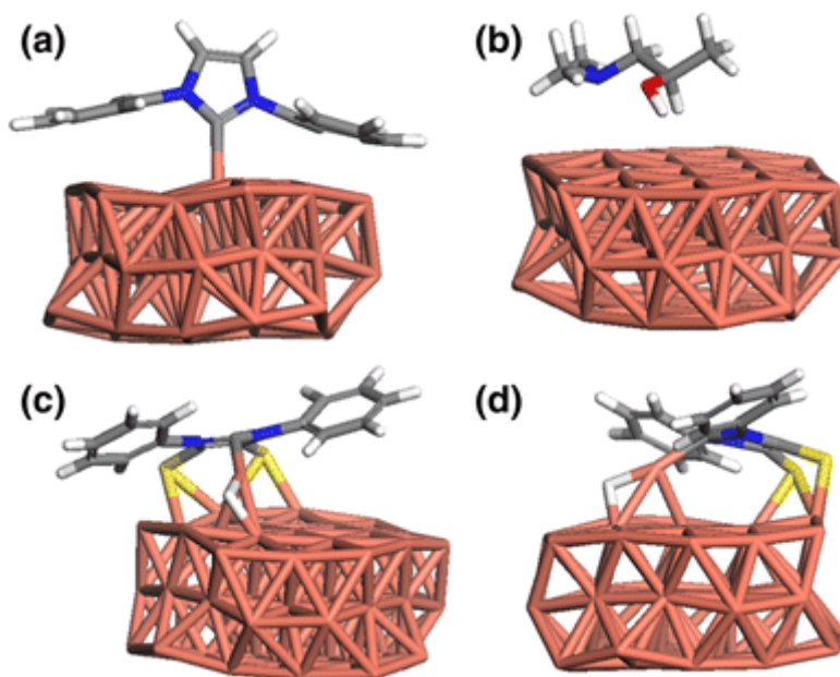
Figure 49: (a) NHC carbene chemisorbed onto the bare copper surface via C. (b) dmapH protonated ligand physisorbed onto the surface. (c) (S-NHC)CuH adsorbed onto the surface via Cu and S. (d) is the same as c from a different viewpoint. Color code: brown copper, white hydrogen, blue nitrogen, gray carbon, yellow sulfur.
