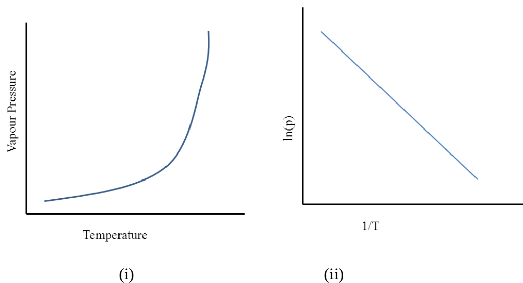
Figure 60: Plots of pressure vs temperature using the Clausius-Clapeyron equation.
