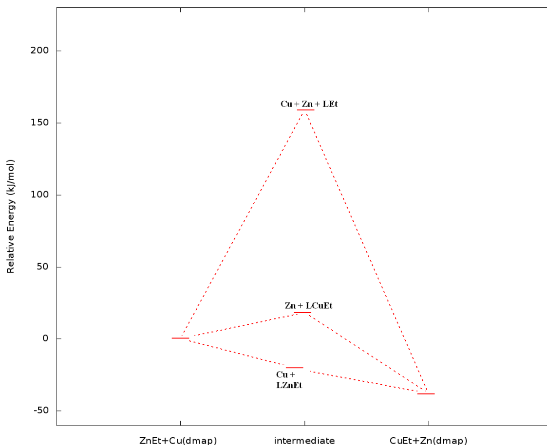
Figure 36: Graph showing the energetics of ligand (L = dmap) exchange between the two metals Cu and Zn following three possible intermediate pathways. It shows that ligand exchange is favourable for dmap ligand as the reaction is downhill. The energy values are presented in the supplementary data present at the end of the chapter.
