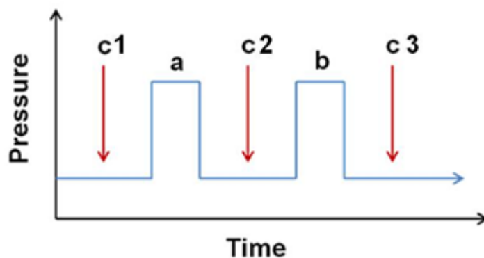
Figure 43: Schematic diagram showing the precursor pulsing sequence for [\text{Cu}(\text{acac})_2] (a), Vanadocene (b) and the three different places for methanol (c) introduction.
