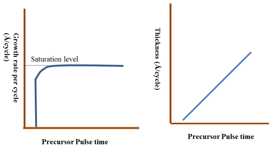
Figure 8: ALD saturation curve (left) vs CVD growth curve (right).
