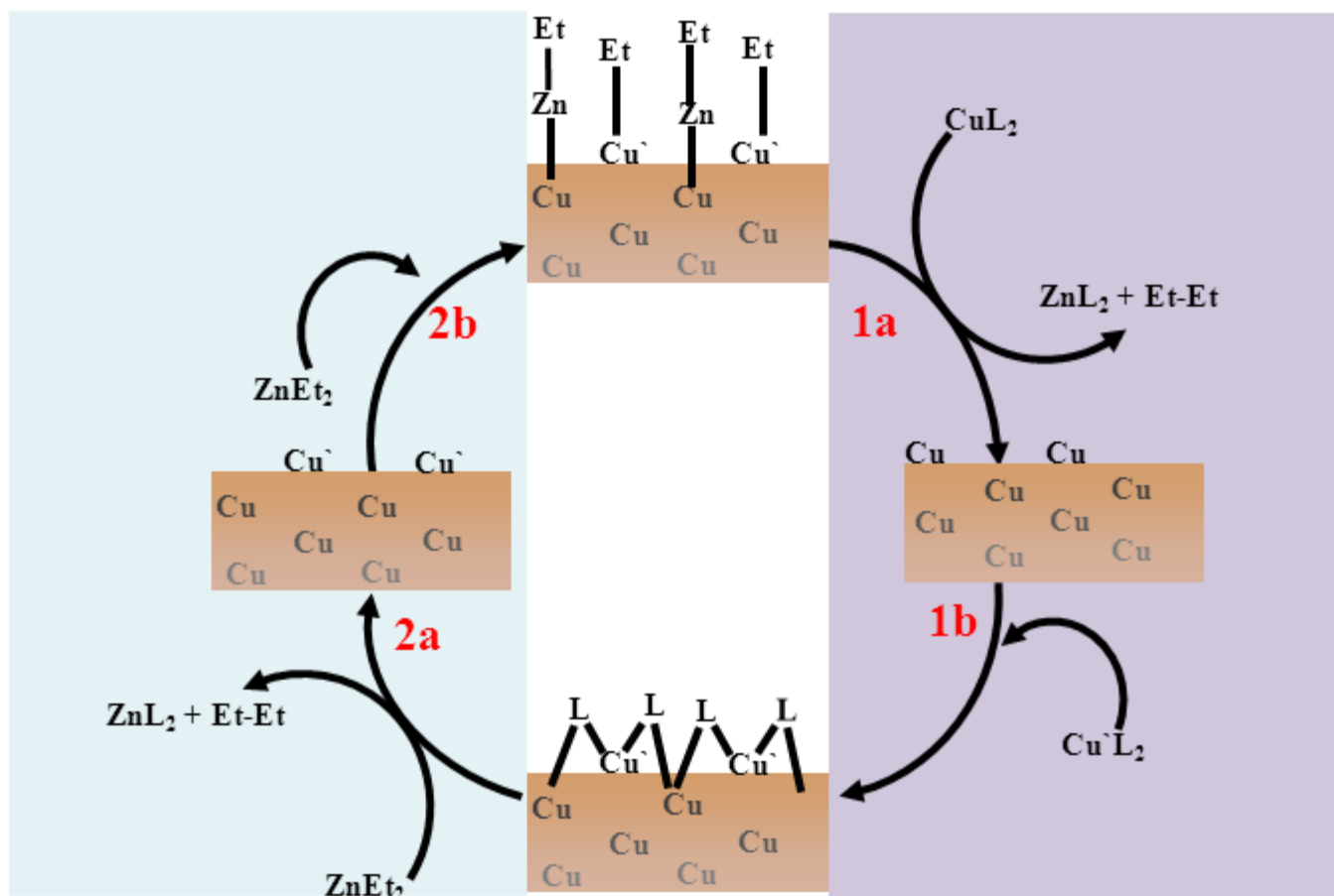
Figure 20: This figure shows various ALD cycle for proposed transmetalation reaction between copper precursor \text{CuL}_2 and reducing agent \text{ZnEt}_2 . Each ALD pulse has been divided conceptually into two halves (a, b). The Cu precursor pulse on the right side with light pink shade is denoted as 1 and the reducing agent pulse on the left side with light blue shade is denoted as 2. Section 1a describes the reaction in a mixed surface between the incoming copper precursor and previously adsorbed Et ligands. Section 1b describes the reaction when the Et ligand has been exhausted and fresh copper precursor adsorbs onto a bare copper surface. Section 2a involves the same reactions as 1a but this is during the reducing agent pulse when incoming \text{ZnEt}_2 interacts with previously adsorbed ligands from the Cu precursor. Section 2b shows the reaction when an excess of reducing agent adsorbs onto a bare copper surface.
