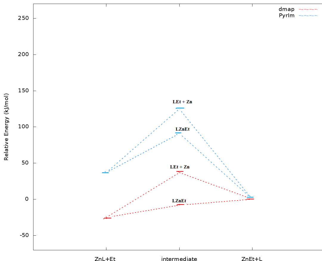
Figure 34: The graph shows the ligand exchange between the \text{Zn} in the reducing agent and copper from the surface for two ligands \text{L} = \text{dmap} and \text{PyrIm}^{\text{iPr}} . The pathway might follow two different intermediates. \text{Zn}(\text{dmap}) is more stable than \text{ZnEt} and \text{ZnEt} is more stable than \text{Zn}(\text{PyrIm}^{\text{iPr}}) in terms of ligand exchange with the copper surface.
