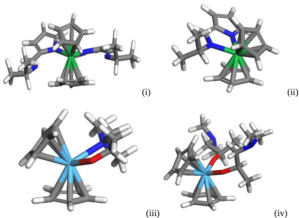
Figure: Stick model of (i) \text{TaCp}_2(\text{PyrIm}^{\text{iPr}})_2 (ii) \text{TaCp}_2(\text{PyrIm}^{\text{iPr}}) . These are the by-products from equation 1 and 2 with tantalocene as the reducing agent and \text{Cu}(\text{PyrIm}^{\text{iPr}})_2 as the precursor. (iii) \text{HfCp}_2(\text{dmap}) (iv) \text{HfCp}_2(\text{dmap})_2 . In (iv) it shows that the dmap ligand opens in the by-product with just the O atoms attached to the Hf. This happens in many by-products. Colour code: Grey – Carbon, White – Hydrogen, Light Grey – Vanadium, Dark Blue – Nitrogen, Green – Tantalum, Light blue – Hafnium, Red – Oxygen.
