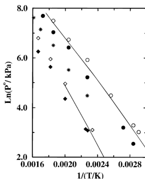
Figure 61: The figure shows the Clausius - Clapeyron equation plot for various alkanes as studied by Martin et al. 223 The solid lines depict the experimental data (upper curve, n-octane; lower curve, n-dodecane). Open circles, filled circles, and stars show the simulation results of the TraPPE, SKS, and OPLS force fields for n-octane, respectively. Open and filled diamonds represent the TraPPE and SKS results for n-dodecane.
