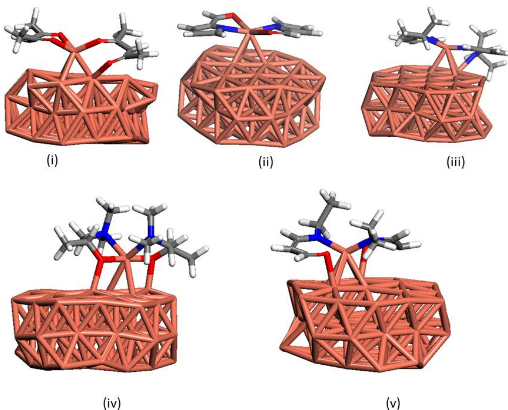
Figure 23: Optimized structures of precursors adsorbed onto the bare copper (111) surface. (i) \text{Cu}(\text{acac})_2 , (ii) \text{Cu}(\text{PyrAld})_2 , (iii) \text{Cu}(\text{PyrIm}^{\text{iPr}})_2 , (iv) \text{Cu}(\text{dmap})_2 , (v) \text{AbaCus}^{\text{(TM)}} . The energetic of the adsorption energy is in Table 12 and the structural changes in the precursor
