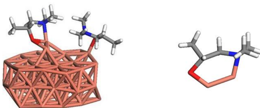
Figure 25: (i) The Cu 2 L 2 (L=dmap) intermediate where there are two ligands, each attached to two adsorbed copper atoms. The corresponding gas phase structure is shown to the right. In the gas phase the distance between the two Cu atoms is |\text{Cu}^{(\text{I})}-\text{Cu}^{(\text{I})}|_{(\text{g})} 2.48 Å and after adsorption onto the surface the distance is |\text{Cu}-\text{Cu}|_{\text{surf}} 3.55 Å. (ii) Cu 2 L + L where the first ligand is attached to two adsorbed copper atoms. The corresponding gas phase structure is also shown. In this case |\text{Cu}-\text{Cu}|_{(\text{g})} = 2.51 Å and |\text{Cu}-\text{Cu}|_{\text{surf}} = 2.67 Å.
