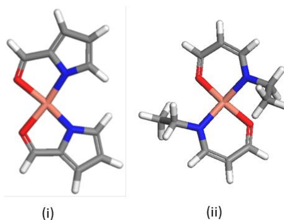
Figure 22: Lowest energy isomer computed in gas phase for potential Cu ALD precursors. (i) \text{Cu}(\text{PyrAld})_2 (ii) \text{AbaCus}^{\text{(TM)}} . Structural parameters are quoted in Table 11. Color code: Red = oxygen, Blue = nitrogen, Grey = carbon, White = hydrogen, Light brown = copper.
