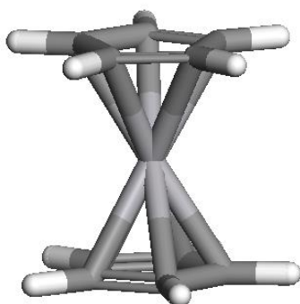
Figure 42: Stick model of (i) Vanadocene. Colour code: Grey – Carbon, White – Hydrogen, Light Grey – Vanadium, Dark Blue – Nitrogen.
