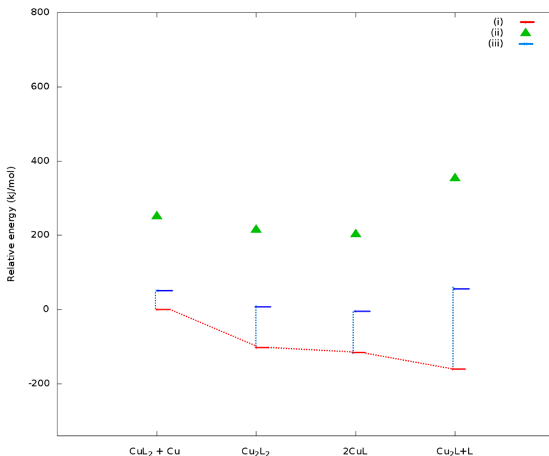
Figure 27: The graph shows similar results to that of Figure 26 but using \text{L} = \text{PyrIm}^{\text{iPr}} as the ligand.
