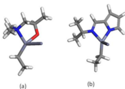
Figure 17: Zn 2 L Et compounds with (a) L=dmap and (b) L=PyrIm iPr .
