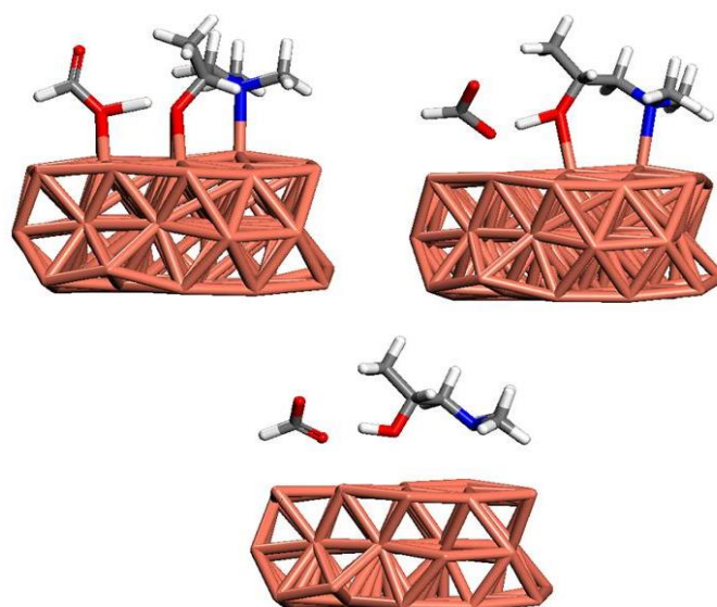
Figure 55: Some snapshots of MD simulation of dmap anion interacting with formic acid in order to form copper formate and dmap-H. The above structures are not optimized. Colour code: brown=Cu, blue=N, red=O, grey=C, white=H.
