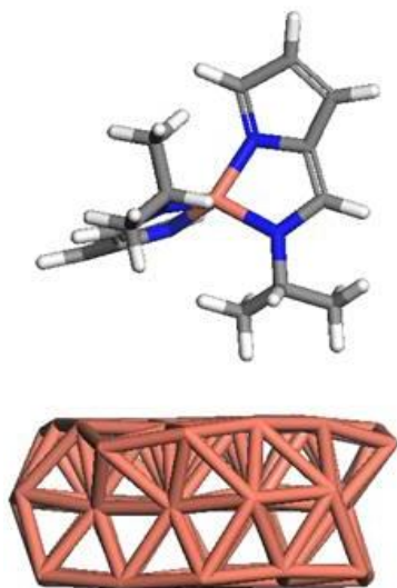
Figure 24: Lowest energy isomer of PyrIm iPr precursor, which does not chemisorb in any orientation onto the copper surface due to steric hindrance (Figure 23 (iii)). Color code: Red = oxygen, Blue = nitrogen, Grey = carbon, White = hydrogen, Light brown = copper.
