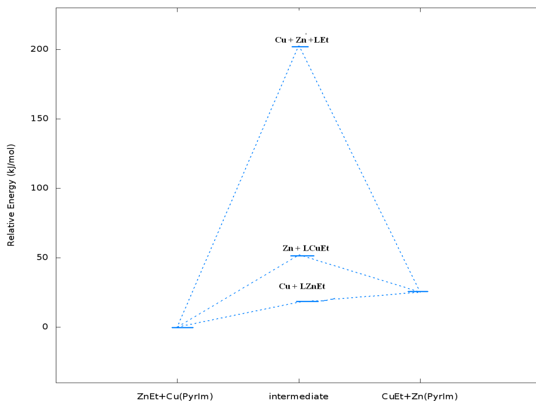
Figure 35: Graph shows the energetics of ligand ( \text{L} = \text{PyrIm}^{\text{iPr}} ) exchange between the two metals Cu and Zn following three possible intermediate pathways. All the intermediates are higher in energy compared to the reactants and products. It shows that ligand exchange is unfavourable for \text{PyrIm}^{\text{iPr}} ligand. The energy values are presented in the supplementary data.
