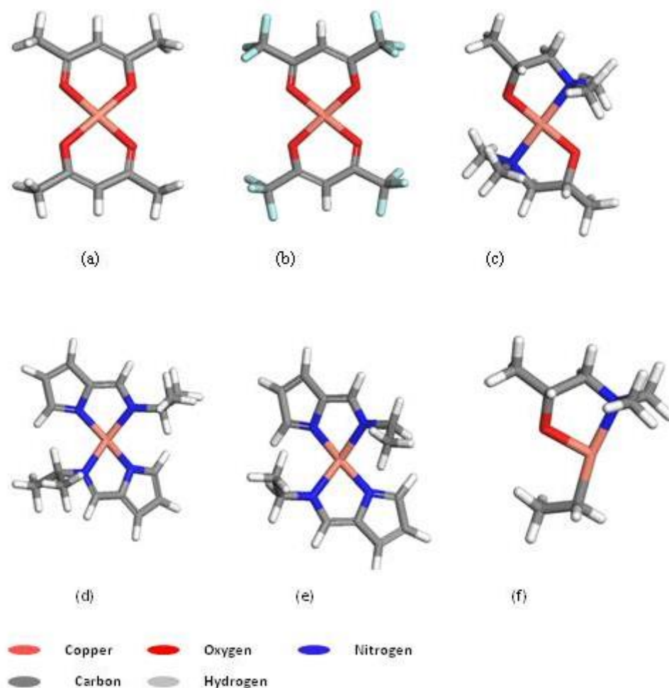
Figure 14: Stick representation of computed structures of precursors and intermediates. (a) \text{Cu}(\text{acac})_2 , (b) \text{Cu}(\text{hfac})_2 , (c) \text{Cu}(\text{dmap})_2 , (d) \text{Cu}(\text{PyrIm}^{\text{iPr}})_2 , (e) \text{Cu}(\text{PyrIm}^{\text{Et}})_2 are the precursors used to understand the mechanism. (f) \text{Cu}(\text{dmap})\text{Et} is a sample intermediate during the course of the reaction. The Zn by-products are similar to these structures, where the Cu atom is replaced with Zn. Quantitative differences in structure between the copper precursor and the zinc by-product are given in Table 6.
