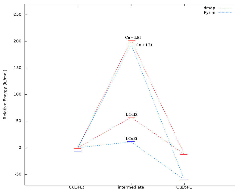
Figure 33: The graph shows the ligand exchange between the copper in the precursor and copper from the surface for two ligands L = \text{dmap} and \text{PyrIm}^{\text{iPr}} . The pathway might follow two different intermediates for each L . It might either form an intermediate redox compound of \text{LCuEt} or else there might be formation of gaseous \text{LEt} with the deposition of \text{Cu} . The two ligand exchanged intermediates have similar energy when L = \text{dmap} . But for L = \text{PyrIm}^{\text{iPr}} the intermediate with the ligand attached to the copper surface is more stable due to downhill in energy.
