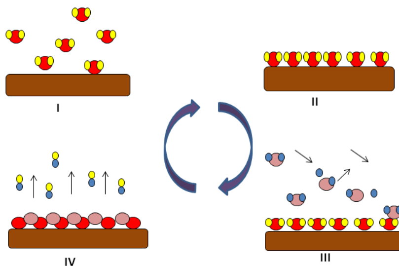
Figure 7: Steps involved in one cycle of Atomic Layer Deposition of a binary compound. Here the two reacting compounds (precursors) are transported to the chamber in two different pulses. It leads to the formation of conformal layers. ‘I’ shows the precursor pulse. ‘II’ shows the adsorbed precursor saturating the surface. ‘III’ shows the incoming co-reagents and ‘IV’ the deposition of the binary material.
