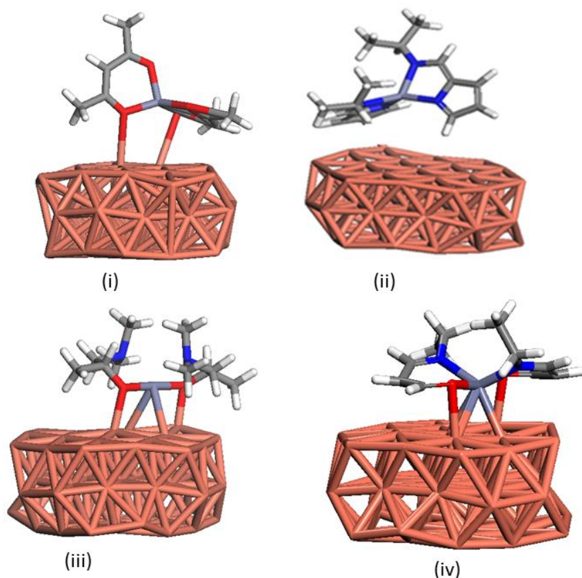
Figure 39: Potential Zn by-products adsorbed on the copper (111) surface. (i) \text{Zn}(\text{acac})_2 , (ii) \text{Zn}(\text{PyrIm}^{\text{iPr}})_2 , (iii) \text{Zn}(\text{dmap})_2 , (iv) AbaZns. Color code: Red = oxygen, Grey = carbon, White = hydrogen, shaded grey = zinc, Blue = nitrogen.
