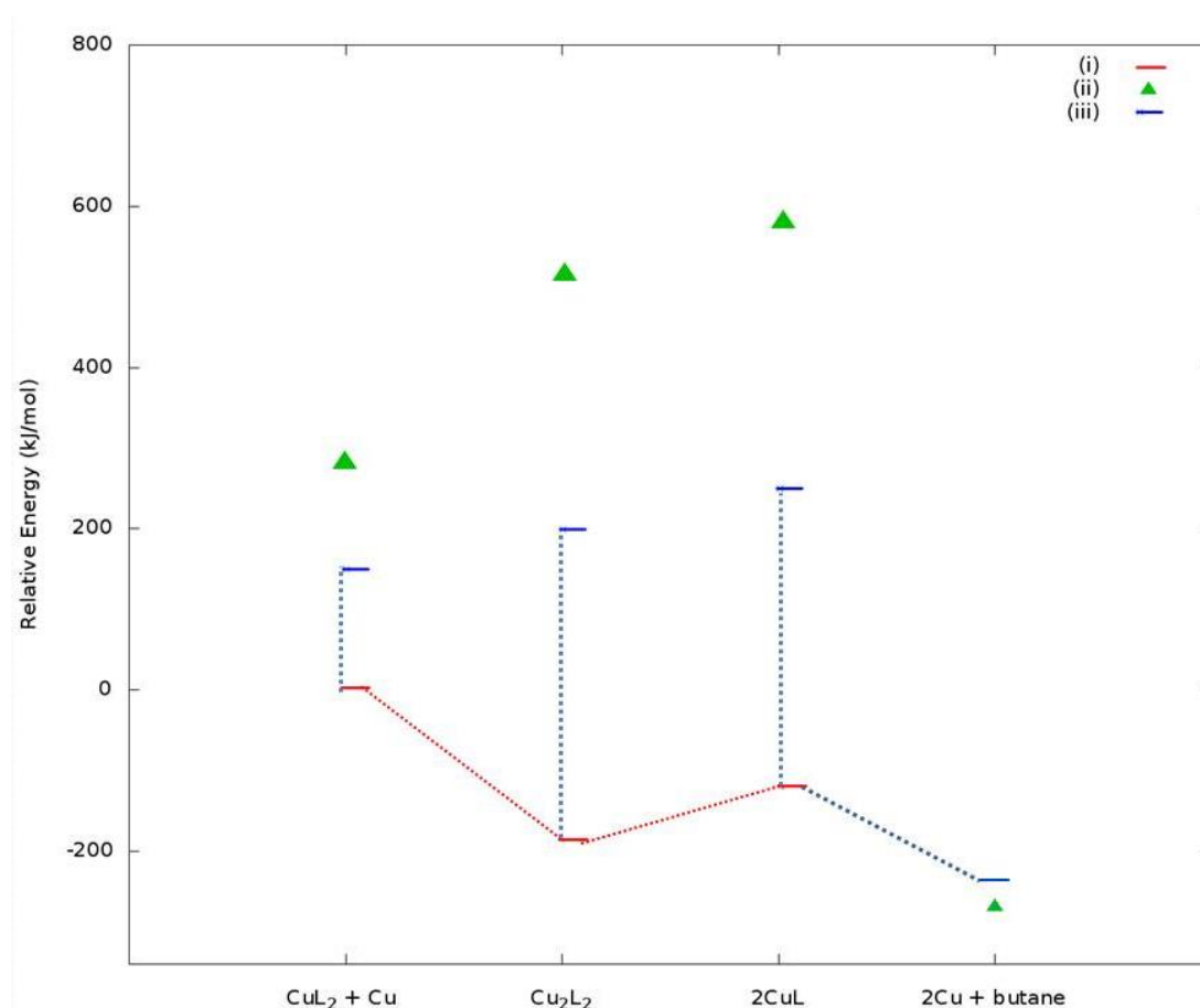
Figure 30: The graph shows similar results to that of Figure 26 but using \text{L} = \text{Et} as the ligand. The most important reaction shown in the graph is the interaction between two \text{CuEt} and formation of butane with deposition of \text{Cu}^{(0)} . The same reaction can also be formed when \text{Cu}_2\text{Et}_2 dimer dissociates. The last intermediate has two new Cu atom adsorbed to the surface and butane in gaseous form.
