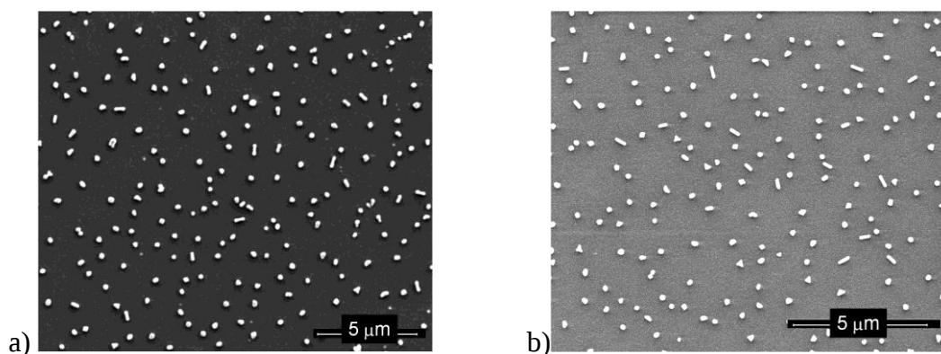
Figure 45: SEM images of experiments grown at 250 °C using ratios of \text{Cu}(\text{acac})_2 :vanadocene of a) 1:1 and b) 1:2 on Si(100) substrate.
