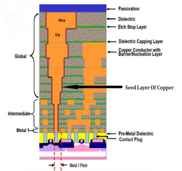
Figure 2: Cross-section of an MPU (Semiconductor Industry Association. The International Technology Roadmap for Semiconductors, 2009 Edition. International SEMATECH: Austin, TX, 2009)
