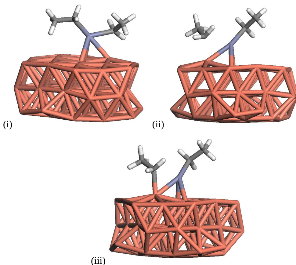
Figure 29: Ab initio Molecular Dynamics study for \text{ZnEt}_2 on \text{Cu}(111) surface. (i) Time t=0 shows \text{ZnEt}_2 attached to the surface. (ii) At time t=1.17 ps breaking of the C-Zn bond is apparent. Distance between C-Zn is 2.38 \text{ \AA} (C from the ethyl group). (iii) At time t=2.17 ps, \text{ZnEt} and Et are separately attached to the copper surface. The above structures are not
