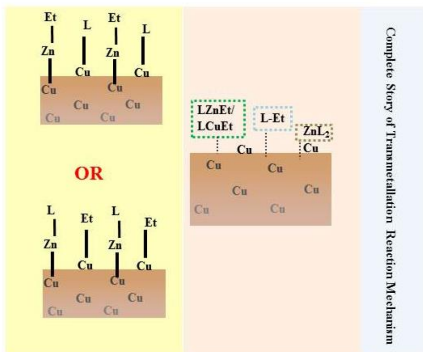
Figure 32: The picture shows the division of parts for this chapter. Here, we are studying the chemistry of a mixed surface that is seen in an ALD chamber after the precursor and \text{ZnEt}_2 pulse. The most stable structure of Cu and Zn atoms attached to precursor ligand L or Et is explored in part 5.3. The desorption energies of the Cu and Zn by-products are seen in part 5.4. The complete story of transmetalation reaction is seen at the end 5.5.
