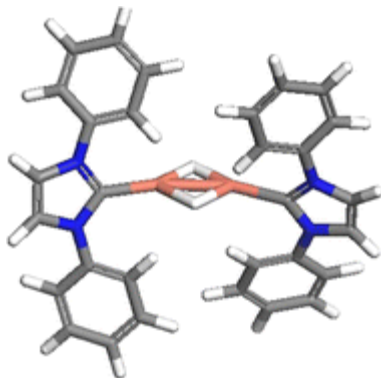
Figure 50: N-heterocyclic - Cu hydride dimer. Color code: brown copper, white hydrogen, blue nitrogen, gray carbon. The computed dihedral angle between C–Cu–Cu–C where the C is from the ligated carbene molecule is 16 °
