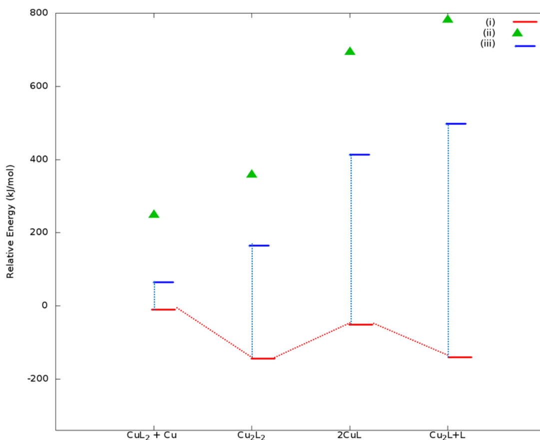
Figure 26: Energetics of surface intermediates during transmetallation when L = dmap is the ligand. The lower the energy in the graph, the more stable the system. (i) Red lines: The energy \Delta E needed to transform the intermediate species into another on a bare copper surface. (ii) Green triangles: The desorption energy ( \Delta E_{\text{des}} ) of the respective species into the gas phase relative to the red line. In the first structure the desorbed molecule is CuL 2 , second Cu 2 L 2 , third CuL, and the last Cu 2 L. (iii) Horizontal Blue lines: The free energy ( \Delta G^{393} ) including the entropy factor at 393 K needed for the species in order to desorb into the gas phase relative to the red line. Any particular intermediate has the probability of either desorption from the surface (red \rightarrow blue) or else can form another surface intermediate (red \rightarrow red). The data are presented in the supplementary information. No barriers have been computed.
