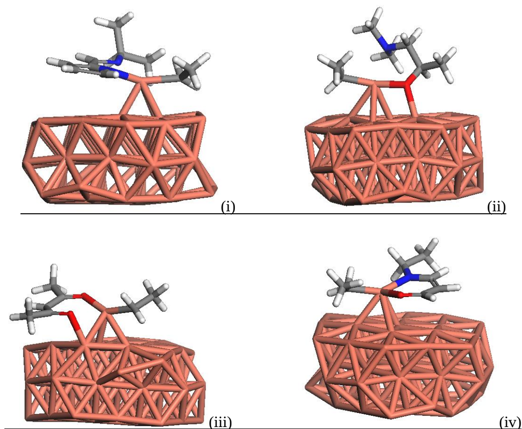
Figure 38: Optimized structures of LCuEt precursors adsorbed onto the bare copper (111) surface. (i) L = PyrIm iPr (ii) L = dmap (iii) L = acac (iv) L = AbaCus (TM) . Structural changes between the gas phase structure and the adsorbed structure are shown in Table 17. Color code: Red = oxygen, Grey = carbon, White = hydrogen, Light brown = copper, Blue = nitrogen.
