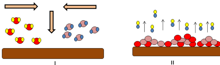
Figure 6: The various steps involved in CVD reactions. Here the two reactants are transported to the system simultaneously. This may lead to the deposition of non-conformal layers.
