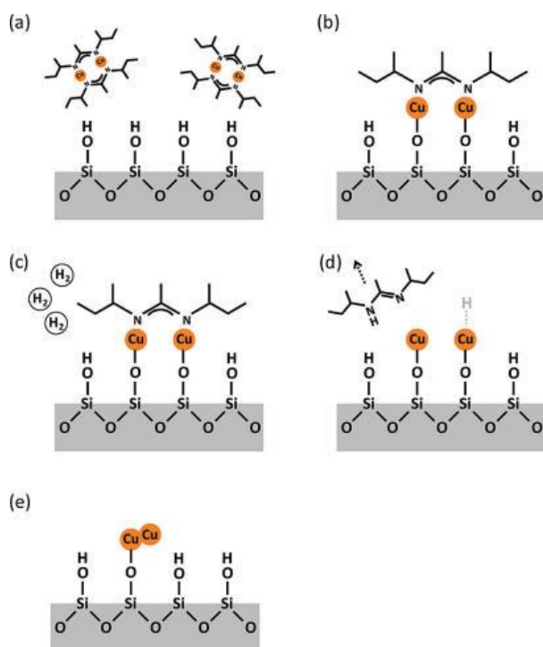
Figure 12: Schematic of reactions of [Cu(sBu-amd)] 2 (a,b) and H 2 (c,d) on the OH-terminated SiO 2 surface. (Reprinted with permission from American Chemical Society. Adapted from Dai et al. 79 )
