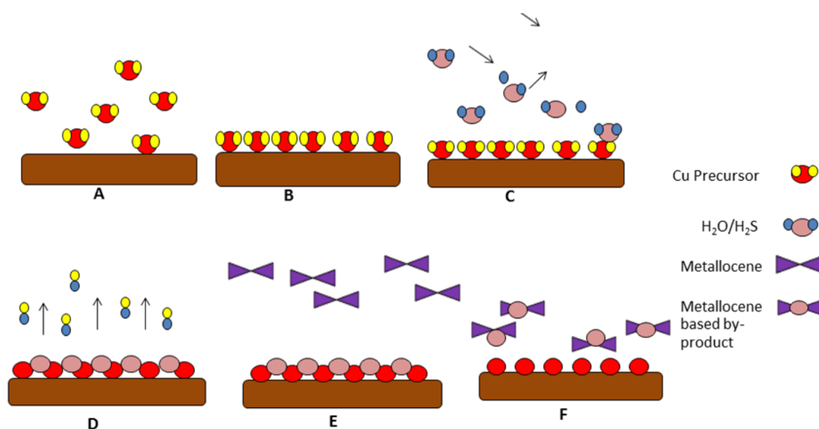
Figure 41: The picture shows the proposed deposition of copper from copper precursor with the intermediate formation of copper sulfide or copper oxide. ‘A’ shows the precursor pulse. ‘B’ shows the saturation of the precursors onto the surface. ‘C’ shows the H 2 O or else H 2 S pulse. ‘D’ shows the formation of oxide or else sulfide. ‘E’ shows the incoming metallocene and ‘F’ the deposition of copper with the formation of substituted metallocene products. Steps C and D can be omitted and there can be direct deposition of copper from the precursor as described in equations 1 and 2.
