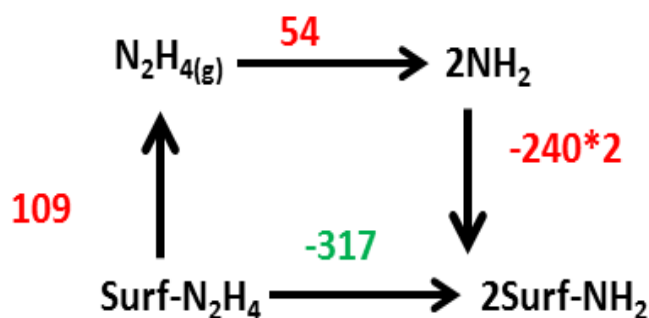
Figure 56: Hess cycle showing the formation of surface adsorbed NH 2 from surface adsorbed N 2 H 4 . All the energies are in kJ/mol of hydrazine.
