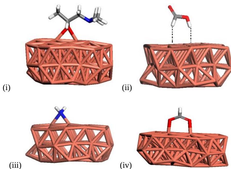
Figure 54: Optimized structure of (i) dmap ligand adsorbed on the smooth model copper surface, (ii) physisorbed formic acid (iii) adsorbed NH 2 radical, (iv) adsorbed formate anion. (Figure 57 for formate adsorption onto a rough surface). Colour code: brown=Cu, blue=N, red=O, grey=C, white=H.
