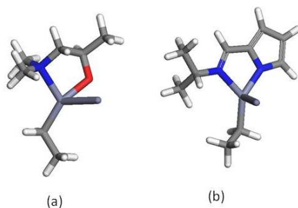
Figure 18 : \text{Zn}_2\text{LEt} compounds with (a) \text{L}=\text{dmap} and (b) \text{L}=\text{PyrIm}^{\text{iPr}} .
