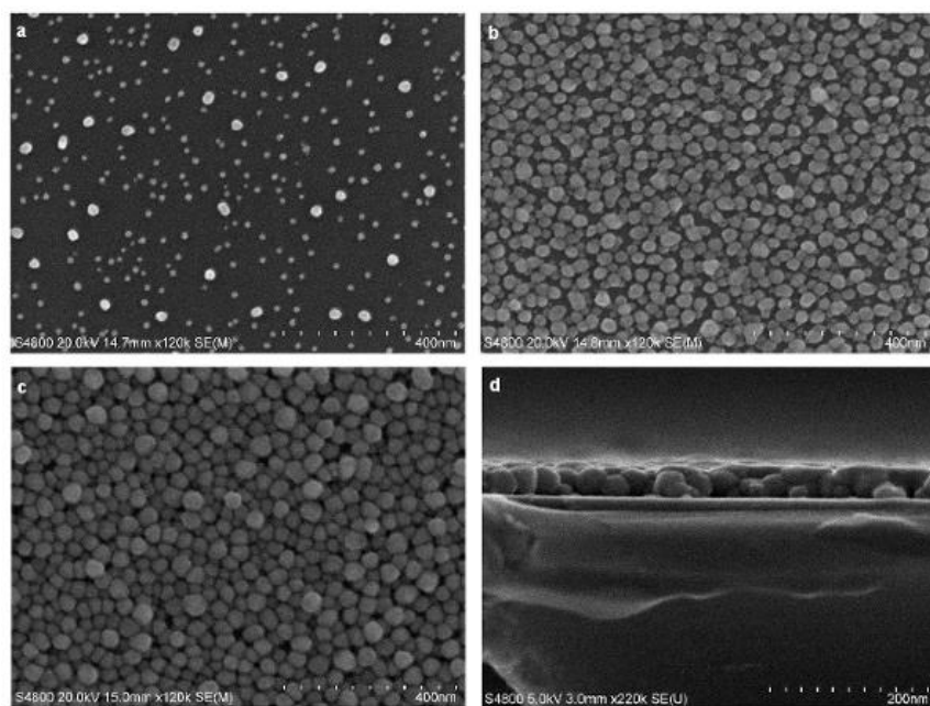
Figure 52: Scanning electron micrographs of deposited copper films. a) Plan view of copper nanoparticles deposited using a 1 s pulse length. b) Plan view of crystalline copper deposited using a 4 s pulse length. c) Plan view of crystalline copper deposited using a 6 s pulse length. d) a profile of crystalline copper deposited using a 6 s pulse length.
