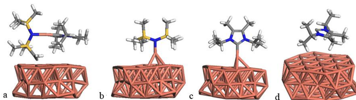
Figure 53: Optimized geometries of (a) 2 molecularly physisorbed on a smooth Cu (111) surface; (b) CuN(SiMe 3 ) 2 chemisorbed on the smooth surface; (c) NHC from 2 chemisorbed onto a rough surface; (d) NHC from 2 physisorbed on the smooth surface.
