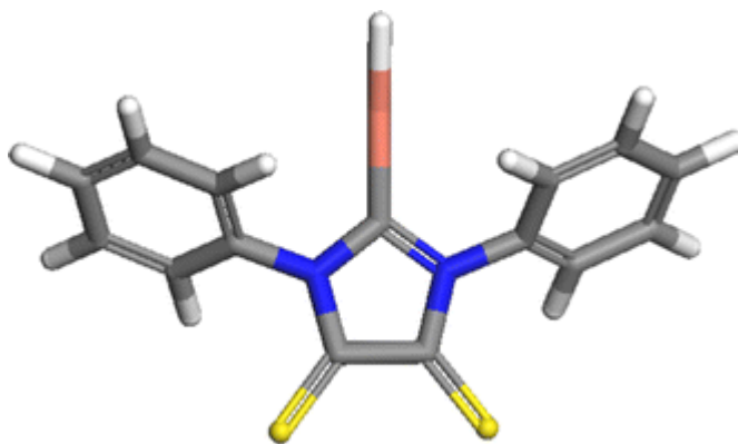
Figure 47: (S-NHC)CuH showing S substituted for H at 4 and 5 positions.
