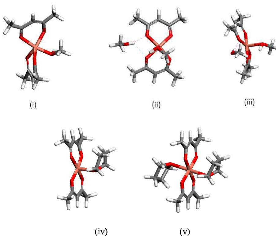
Figure 44: (i) Shows stick model of \text{Cu}(\text{acac})_2(\text{MeOH}) . Here the O from MeOH is coordinatively bonded to the copper in the copper precursor. (ii) shows two MeOH bonded to \text{Cu}(\text{acac})_2 . (iii) shows the side view of (ii). Here, one MeOH is coordinatively bonded to Cu and the other has H-bonding between the H from MeOH and O from the precursor. (iv) shows \text{Cu}(\text{acac})_2 coordinatively bonded to THF. (v) shows \text{Cu}(\text{acac})_2 co-ordinately bonded to two THF molecules.
