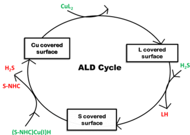
Figure 48: Flowchart showing the three-step ALD cycle for the deposition of Cu with the intermediate formation of CuS layer. L ligand and S sulfide
