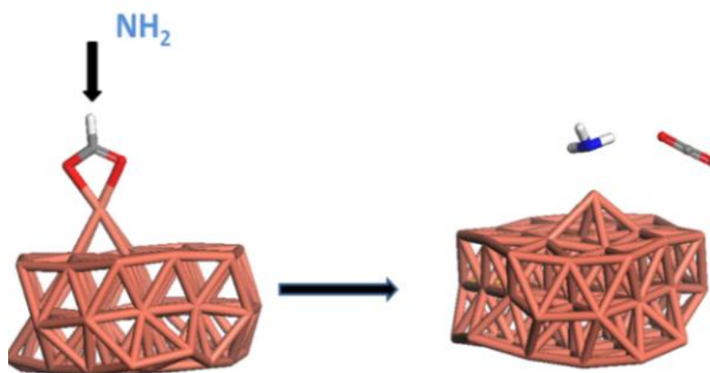
Figure 57: When the \text{NH}_2 radical attacks the H of \text{Cu}(\text{HCOO}) , it forms \text{CO}_2 and \text{NH}_3 as by-products, leaving an atom of copper metal on the surface. Colour code: brown=Cu, blue=N, red=O, grey=C, white=H.
