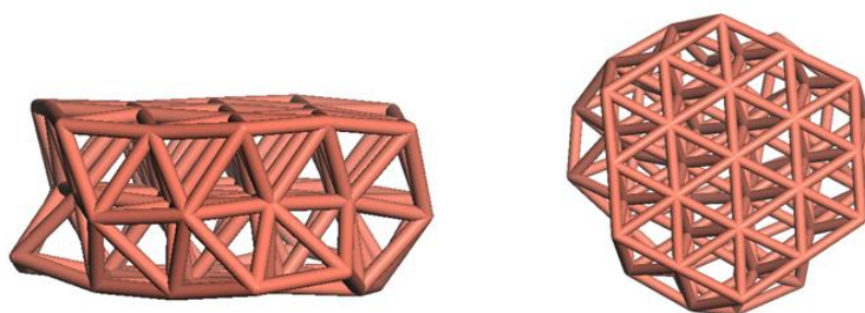
Figure 21: Side view and top view of the 3-layer deep \text{Cu}_{55} cluster, which is used as a model for the \text{Cu}(111) surface to investigate the adsorption of the copper precursors, intermediates and by-products.
