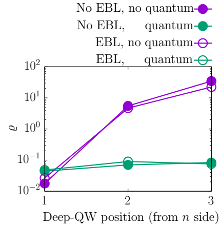
FIG. 4. The ratio of the radiative recombination \varrho [see Eq. (1)] from the shallow wells ( \text{In}_{0.1}\text{Ga}_{0.9}\text{N} ) to recombination from the deep well ( \text{In}_{0.125}\text{Ga}_{0.875}\text{N} ), calculated as a function of the position of the deep well in the MQW stack. Here, \varrho is evaluated using NEXTNANO excluding (purple) and including (green) quantum corrections via a 1-D VCA self-consistent Schrödinger-Poisson drift-diffusion solver; results are shown when excluding (solid, filled circles) and including (dotted, open circles) an \text{Al}_{0.15}\text{Ga}_{0.85}\text{N} blocking layer.
