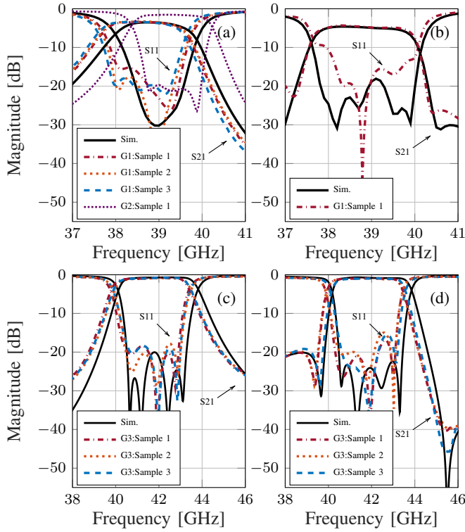
Fig. 1: LMST filters: (a) 4-pole dual-mode Chebyshev (G1 and G2), (b) 6-pole quasi-elliptic (G1), 4-pole single-mode Chebyshev G3 without (c) and with transmission zeros (d).
