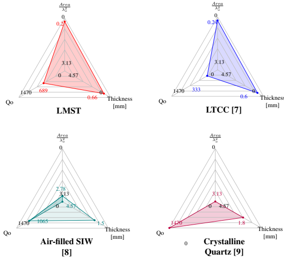
Fig. 4: Relative features comparison between LMST third generation filters and 40 GHz mm-Wave band fabrication technologies [6].
