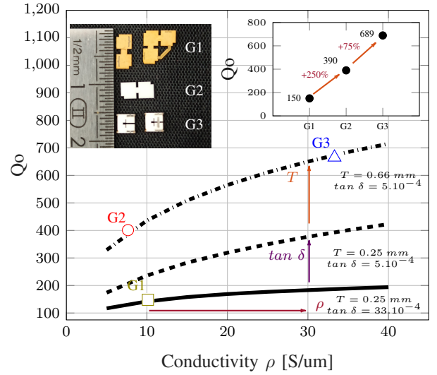
Fig. 2: Quality factor dependency with the substrate loss ( \tan \delta ), electrical conductivity ( \rho ) and thickness ( T ) for a TE_{102} rectangular resonator.
