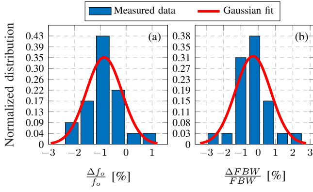
Fig. 3: LMST filters relative frequency shift (a) and fractional bandwidth mismatch (b) statistics and Gaussian distribution.
