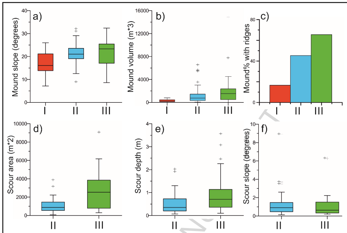
Figure 5 Box & whiskers plots showing the distribution of the minimum, maximum, 1 st quartile, 3 rd quartile and mean values of Type I, II and III mounds for a) slope; b) volume; c) bar chart of percentage that occur with ridge-like features; d) scour area; e) scour depth and; f) slope. Outliers symbolised by "+" symbol.
