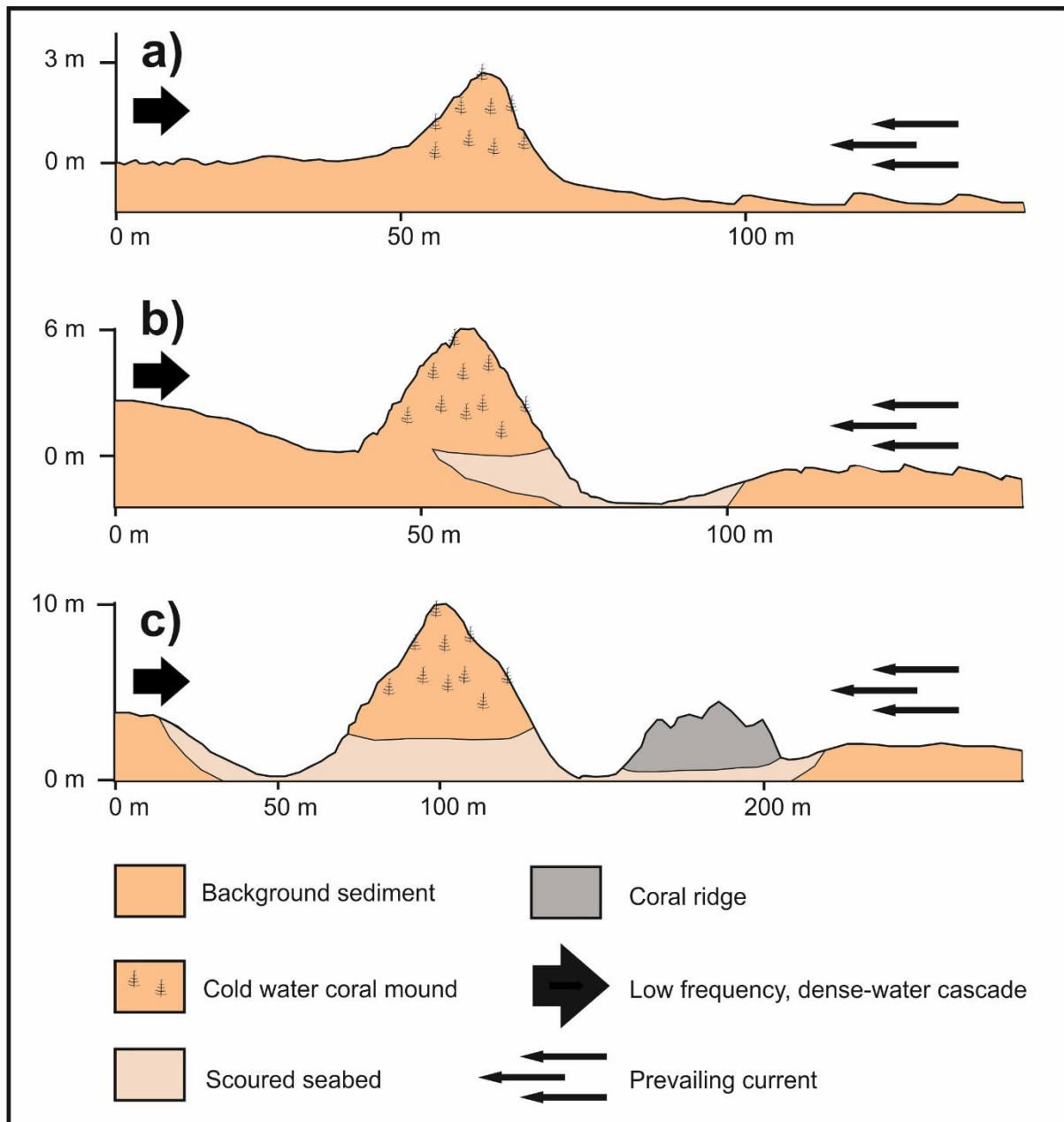
Figure 8a) Schematic of Type I mound local sedimentary environment where the mounds are 3 m in height, with a relatively gentle slope and no scouring; 8b) schematic of Type II mound local sedimentary environment where the mound has now developed to 6 m in height, poorly developed scour occurs at the base of the mounds and the slope has steepened; 8c) schematic of Type III mound local sedimentary environment where the mound has now developed to 10 m in height, the scour is well-developed, encircling the mound and coral ridges have developed within this scour pit.
