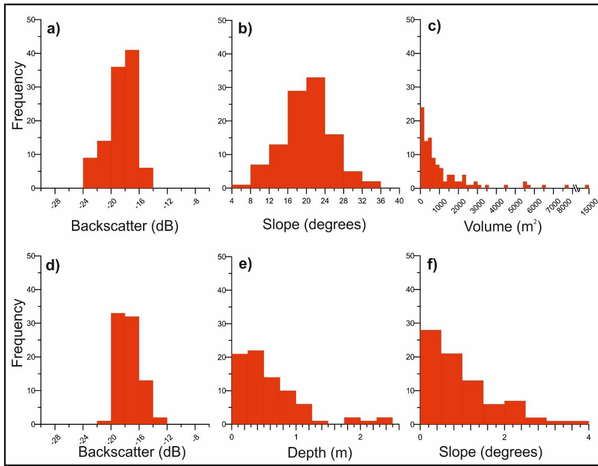
Figure 4 a) Backscatter histogram for the downslope Moira Mounds; b) slope histogram for the downslope Moira Mounds; c) mound volume histogram for the downslope Moira Mounds; d) backscatter histogram for the scour pits; e) depth histogram of the scour pits and; f) slope histogram for the scour pits.
