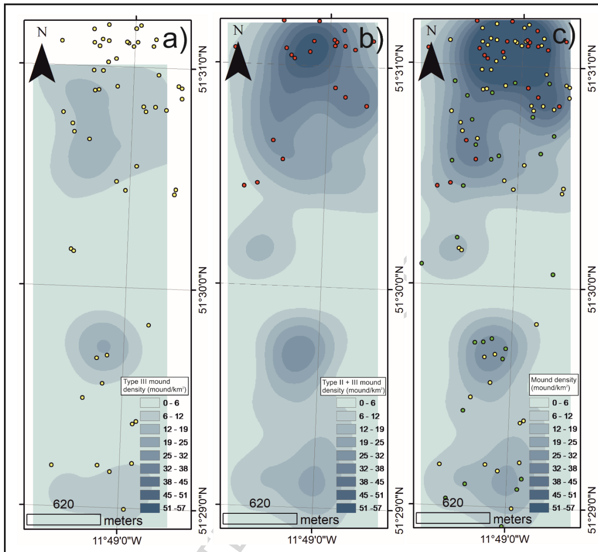
Figure 6 Mound density maps a) Type III mound density raster with Type II mound points overlaid (yellow); b) Type III and type II mound density raster with Type I mound points overlaid (red); c) all mound density raster overlaid by the distribution of all mounds in the study area (yellow = Type II; red = Type I and; green = Type III). Density is expressed as number of mounds per \text{km}^2 over a neighbourhood of 460 m.
