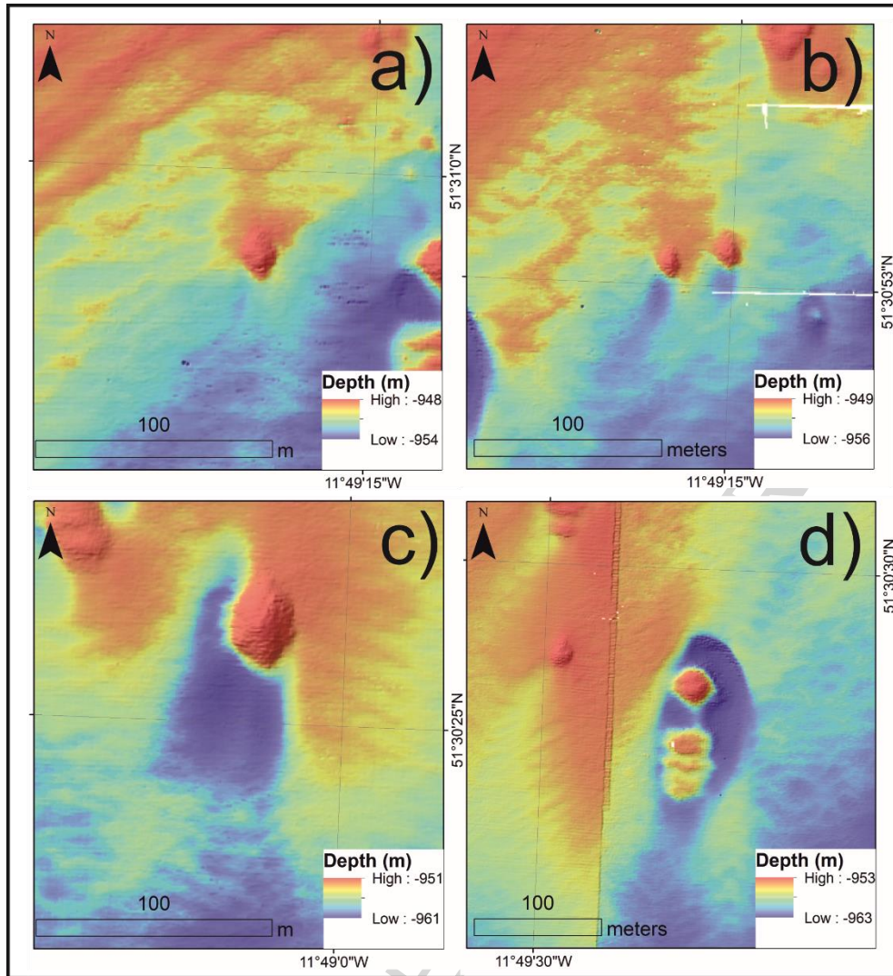
Figure 3 a) Bathymetric data showing a small Moira Mound approx. 3 m in height with no scouring, surrounded by a megarippled seabed; b) bathymetric data showing 2 small Moira Mounds with scour developing at 1 sector of the mound perimeter, surrounded by a megarippled seabed; c) bathymetric data showing a moderately-sized Moira Mound where the mound base has been scoured; d) bathymetric data showing a large Moira Mound with well-developed scour encircling the mound base with ridge-like features formed within the scour pit.
