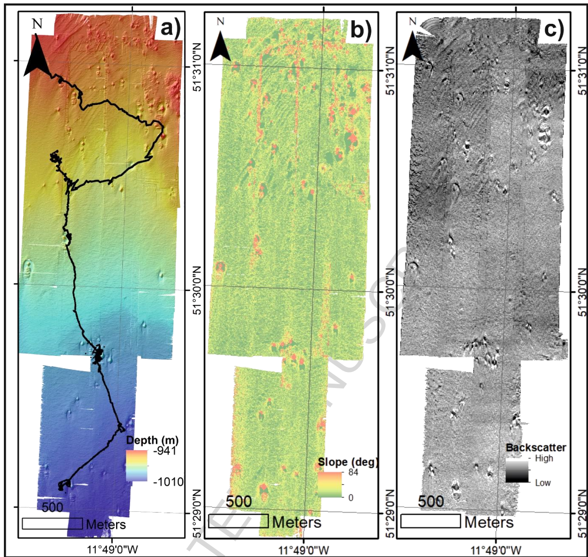
Figure. 2a) Multibeam echosounder bathymetric coverage with the ROV video groundtruthing line shown in black; 2b) seabed slope within the study area (degrees); 2c) multibeam echosounder backscatter (high backscatter in lighter tones, lower in darker tones)
