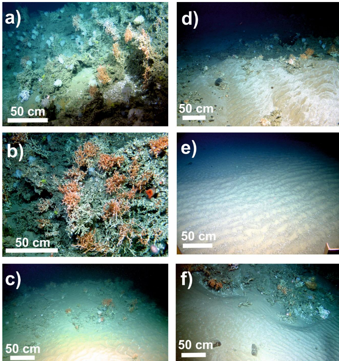
Figure 7 a) Surface of a Moira Mound; b) close up image of large and densely-packed coral colonies, mostly Lophelia pertusa ; c) a small (Type I) Moira Mound showing sparse coral colonies; d) coral ridge within a scour pit; e) off-mound sinuously rippled sands; f) scouring around perimeter of mound.
