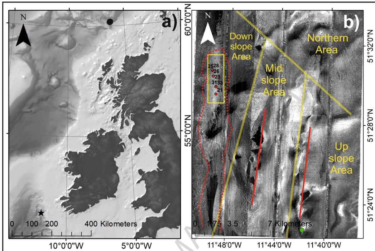
Figure 1a) Locations of the Moira Mounds (star) and of Darwin Mounds (dot); 1b) TOBI 30 kHz sidescan sonar map (after Huvenne et al., 2005) of the Moira Mounds area showing the Challenger Mound (green dot), chains of giant coral carbonate mounds (red lines), margins of blind channel (red dashed line), the 4 Moira Mound areas after Wheeler et al. (2011) (yellow dashed lines), the study site (solid yellow box) and locations of box cores used for this study (red dots).
