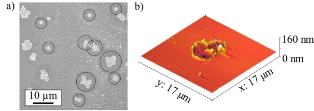
Figure 5. (a) SEM image of the top electrode after the application of a CVS. (b) AFM image of the BD spots showing no alteration of the metal layer outside the crater-like region.
