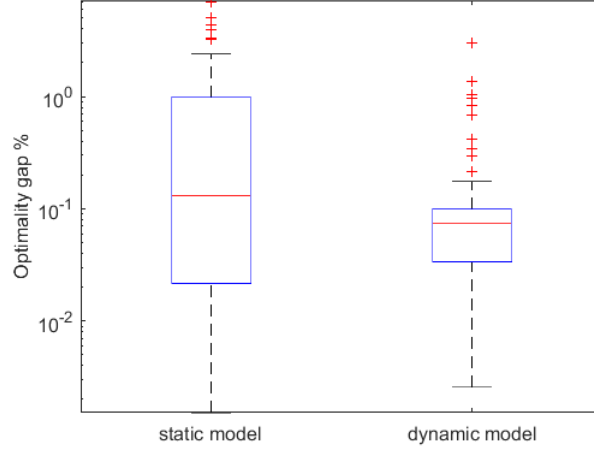
Figure 3: Optimality gaps % of the static method and the dynamic method
