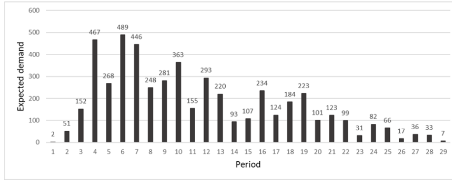
Figure 5: Expected demand of the 29-period example ( K = 300 , c = 0 , h = 1 , b = 5 , cv = 0.1 , and \rho = 0.9 ), for which the cost difference observed when correlation is ignored is 7.90%.
