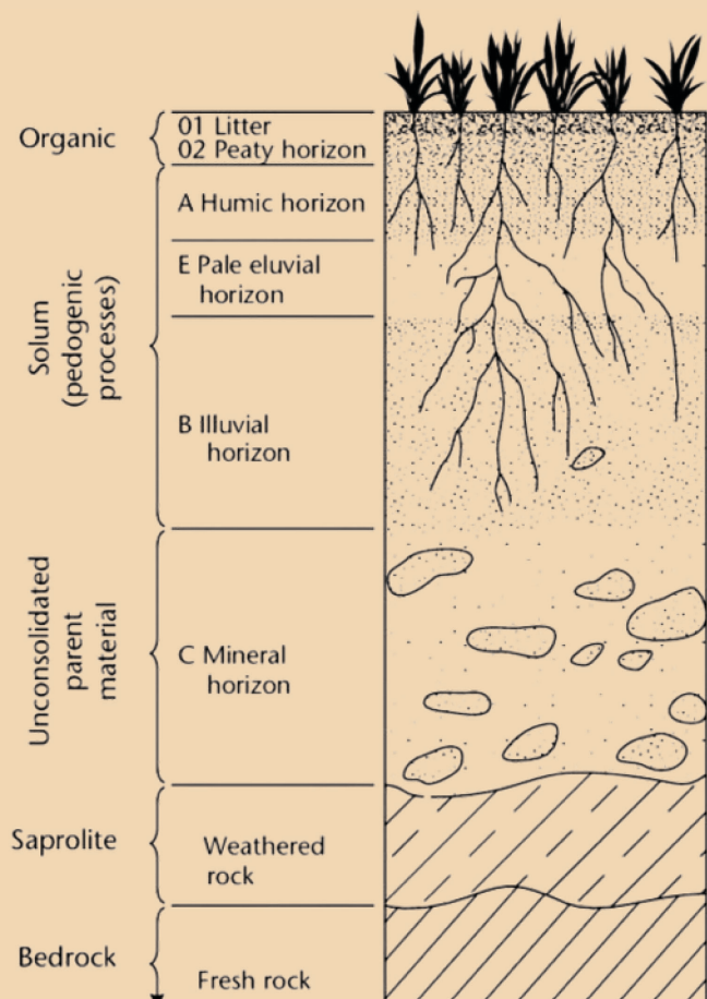
Figure 4. Schematic cross-section of a soil profile showing horizons O, E, A, B, C, saprolite and bedrock, each with distinct structure (McQueen & Scott, 2009).
