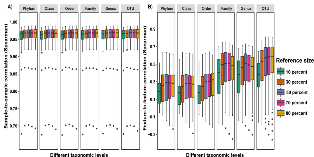
Figure 2 Sample and feature correlation using KEGG pathway abundance at different taxonomic levels and reference dataset size
