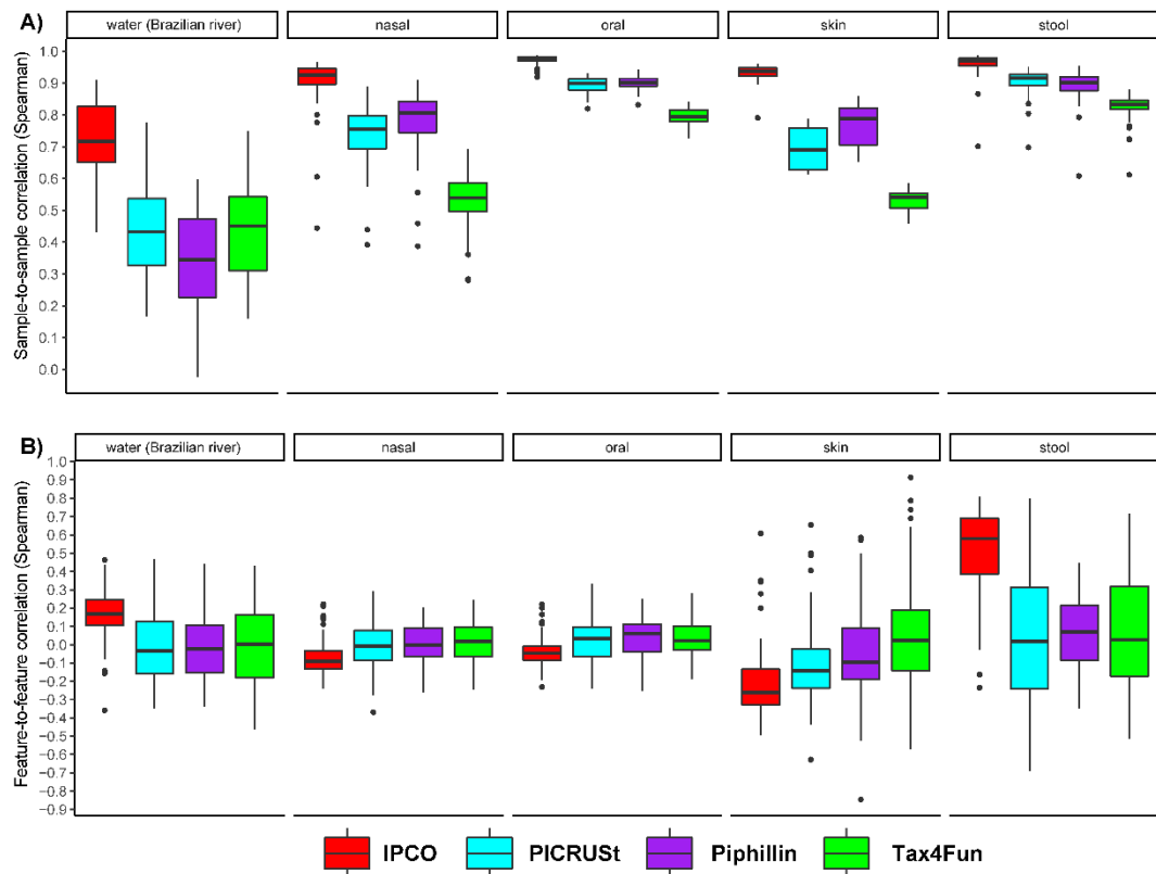
Figure 4 Sample and feature correlations between inferred KO and mWGS KO profiles at different sites and using different methods Boxplots showing the comparison of A) Sample to sample correlations and B) Feature to feature correlations obtained between the inferred KOs and the mWGS KO profiles at different sites using different methods.
