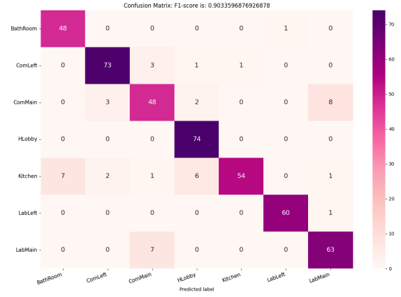
Figure 9. Cross-Session Comparison Results. Third Approach: Transfer Learning, Seven Rooms.
