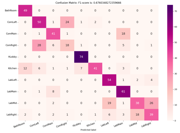
Figure 8. Cross-Session Comparison. Third Approach: Transfer Learning, Ten Rooms. Results: Ten Rooms.
