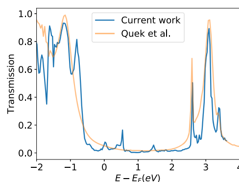
FIG. 2. Comparison of transmission as a function of energy for the junction in Fig. 1 and compared to similar calculations from Ref. 11. Both calculations use the NEGF + DFT calculation on similar geometries using similar electronic structure approximations.
