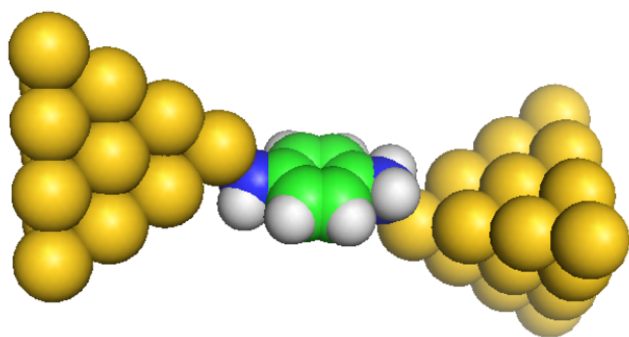
FIG. 1. Explicit atomic model of the MTJ: a single benzene diamine molecule linked by amine groups to two pyramidal gold clusters. Yellow: gold, green: carbon, blue: nitrogen, and white: hydrogen. The junction axis is taken to run between the two gold electrode tips in the diagram.
