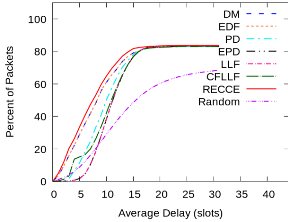
FIGURE 11. CDF of avg. Packet delay ( N = 20 (Scenario set No.6), PDR from 0.7 to 1.0).
