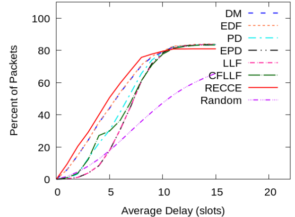
FIGURE 5. CDF of avg. Packet delay ( N = 10 (Scenario set no.2), M = 1 ).
