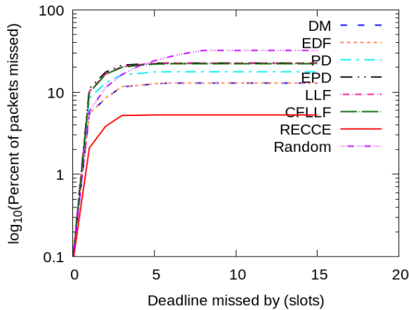
FIGURE 6. CDF of packet delay for missed packets ( N = 10 (Scenario set no. 2), M = 1 ).
