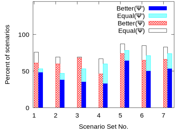
FIGURE 13. Performance of RECCE for scenarios unseen during training.
