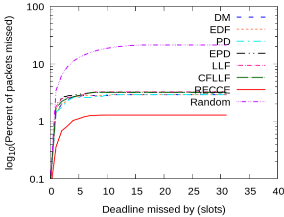
FIGURE 12. CDF of packet delay for missed packets ( N = 20 (Scenario set no. 6), PDR from 0.7 to 1.0).
