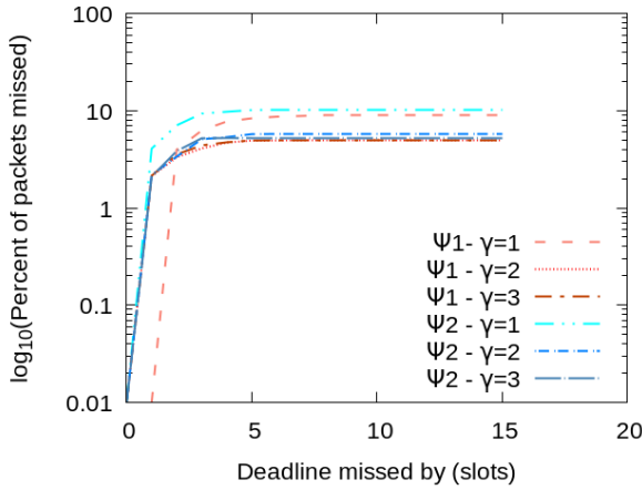
FIGURE 3. CDF of packet delay for missed packets with the number of routes ( N = 10 , scenario set nos. 1 and 2).
