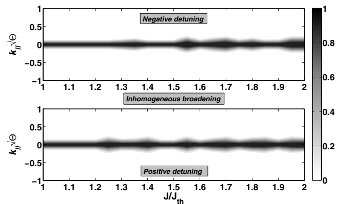
FIG. 14. Nonthermal regime: far field at different pump levels in an inhomogeneously broadened ( \sigma_D=3 ) gain media for both signs of detuning ( \Omega=\pm 0.1 ). The far field remains single lobed until twice threshold.
