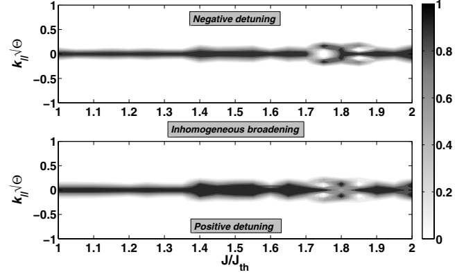
FIG. 13. Nonthermal regime: pump-dependent far field in moderately inhomogeneously broadened ( \sigma_D=1.5 ) gain medium for both signs of detuning ( \Omega=\pm 0.1 ). Difference between negatively detuned homogeneously broadened medium is already evident.
