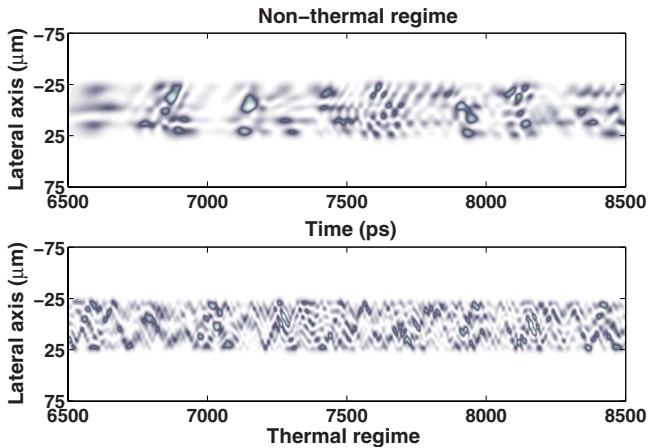
FIG. 19. (Color online) Time-resolved near field (6.5–8.5 ns after laser switch on) for positively detuned ( \Omega=0.1 ) homogeneously broadened ( \sigma_D=0 ) gain medium for both thermal and nonthermal regimes. The negatively detuned case gives qualitatively similar profiles.
