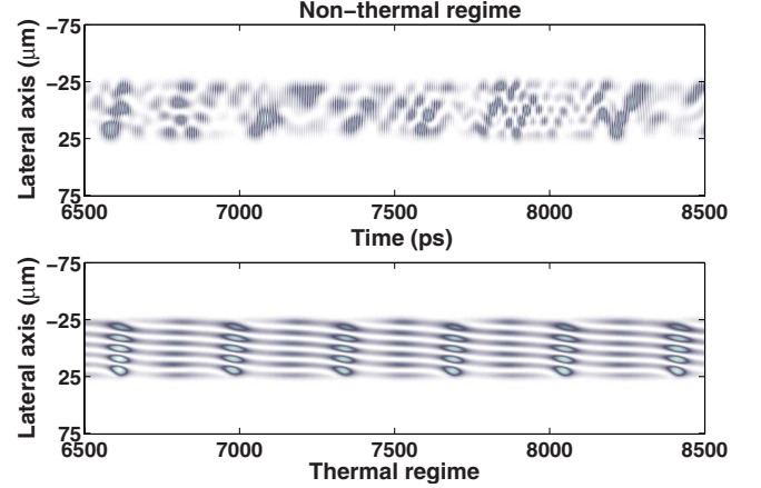
FIG. 20. (Color online) Time-resolved near field (6.5–8.5 ns after laser switch on) for positively detuned ( \Omega=0.1 ) inhomogeneously broadened gain medium ( \sigma_D=3 ) for both thermal and nonthermal regimes. Negative detuning gives qualitatively similar profiles.
