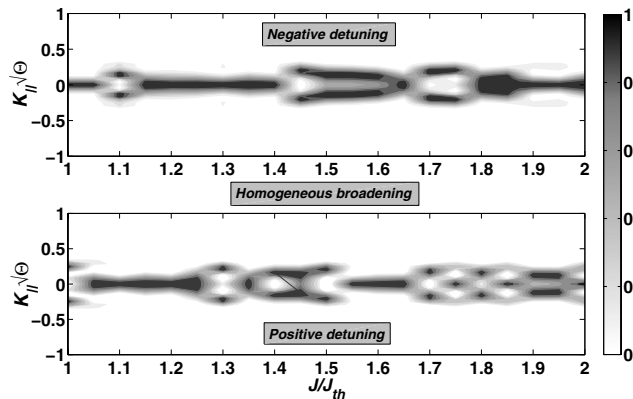
FIG. 12. Nonthermal regime: far-field profiles in a homogeneously broadened ( \sigma_D=0 ) gain media for both signs of detuning ( \Omega=\pm 0.1 ) at different pump levels. The far-field profile moves between single and double lobes.
