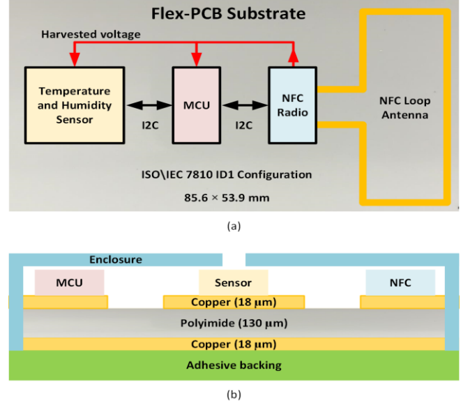
Figure 2. (a) Block diagram, (b) System architecture of the proposed NFC temperature/humidity sensor.
