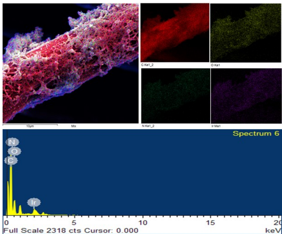
Fig. S3. EDX mapping of \text{IrO}_2 -PANI/CFC electrode.
