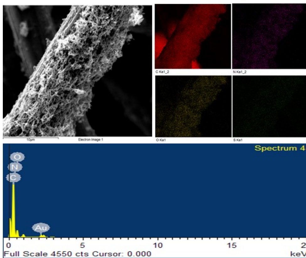
Fig. S2. EDX mapping of PANI modified CFC electrode.
