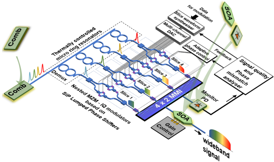
Figure 5.2: Proposed schematic design of a photonic integrated spectrally sliced coherent transmitter ( N=4 ). SiP: silicon photonic; SOA: semiconductor optical amplifier.
