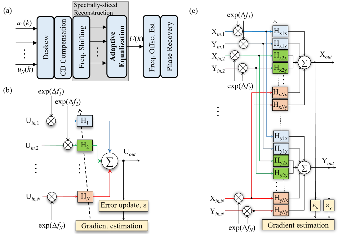
Figure 3.5: (a) Functional blocks in a spectrally sliced receiver DSP. The schematic of reconstruction DSP is based on FIR filters for (b) single-polarization, and (c) dual-polarization modulation.
