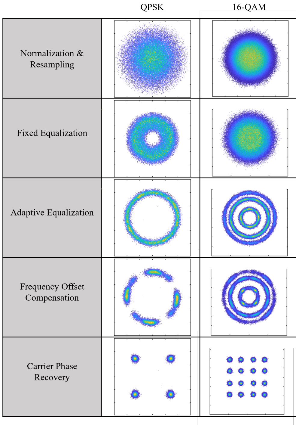
Figure 2.7: Digital signal processings flow to compensate for impairments and to recover the data stream. Constellation diagrams of both QPSK and 16QAM modulation signals were taken after the associated DSP blocks to illustrate the data processing.
