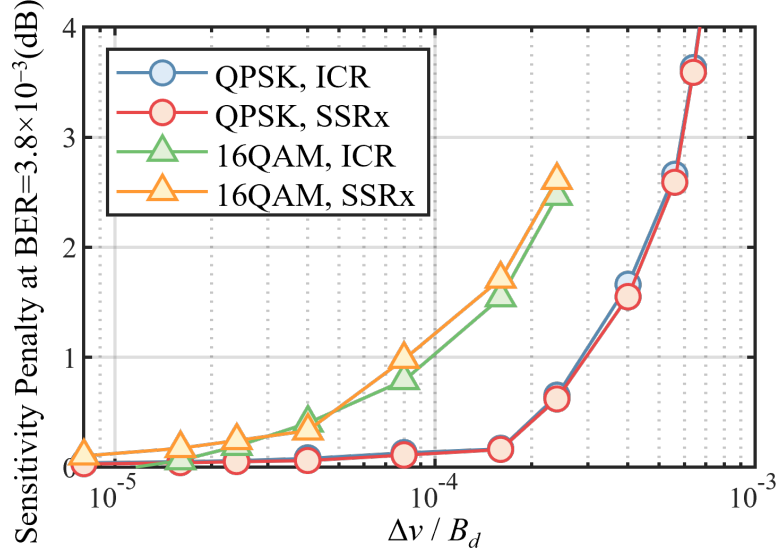
Figure 4.6: Simulated sensitivity penalty as a function of the product of the laser linewidth \Delta\nu and symbol duration 1/B_d for two different modulation formats.
