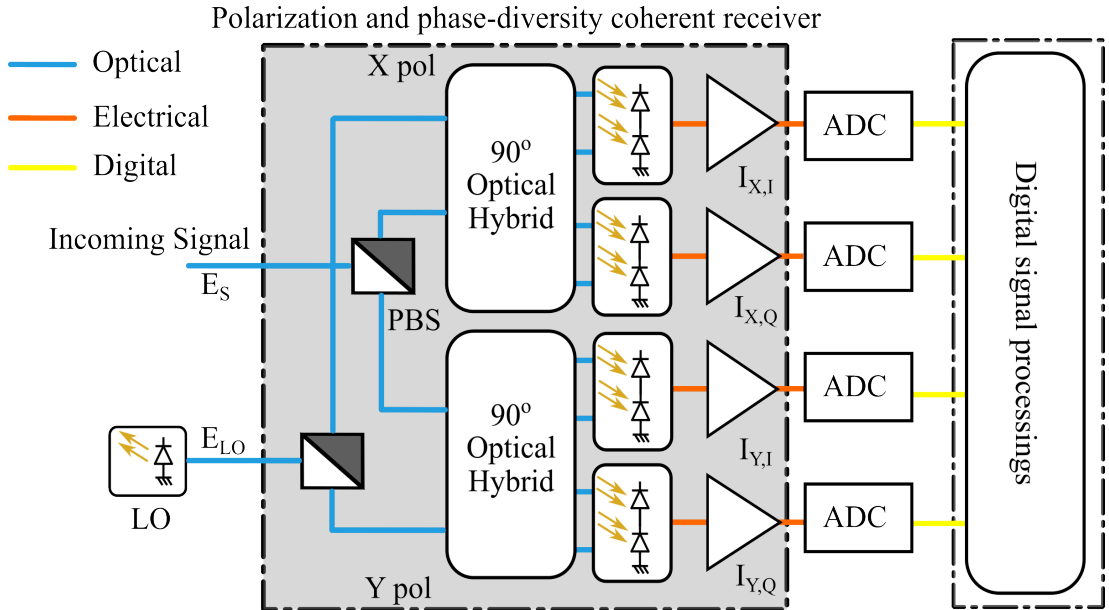
Figure 2.4: Configuration of a phase and polarization diversity optical coherent receiver
