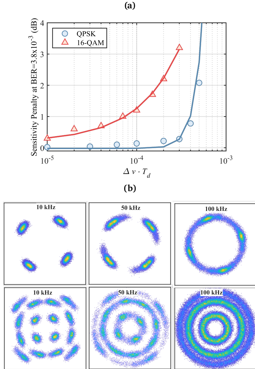
Figure 2.22: (a) Sensitivity penalty versus combined linewidths symbol duration products for QPSK and 16QAM modulation formats. (b) Constellation diagram without phase domain equalization using QPSK (top) and 16QAM (bottom) for different combined laser linewidths.
