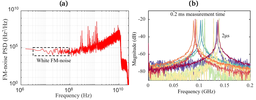
Figure 2.6: (a) Example FM-noise spectrum of a semiconductor laser using a delayed self-heterodyne setup. (b) Field spectra of beat tones between two ECLs in an experimental setup where the two ECLs were connected to the coherent receiver inputs and the output waveform was taken within 0.2 \text{ms} time window; each spectra plotted here has a span of 2 \mu\text{s} .
