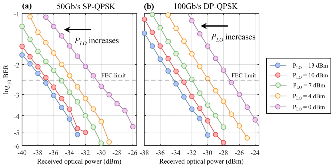
Figure 2.19: Experimental results of the ICR sensitivity performance of a single-carrier 25 Gbaud QPSK signals employing single-pol (left) and dual-pol (right) in a back-to-back link.
