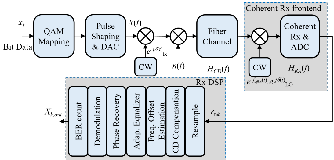
Figure 2.15: Block diagram of a coherent simulation setup.
