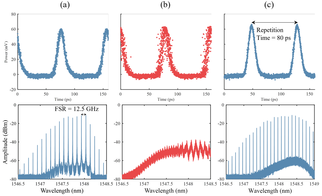
Figure 4.10: Top: The pulse sampling of the optical frequency comb in the time-domain, bottom: Optical spectrum captured with the spectral resolution of 20 MHz for different gain-switching configurations. (a) DFB laser driven at 12.5 GHz sinusoidal RF signal with +5 dBm amplitude, (b) DFB laser driven by +20 dBm RF signal, and (c) DFB laser driven at +20 dBm RF signal with applied injection locking from an ECL laser.
