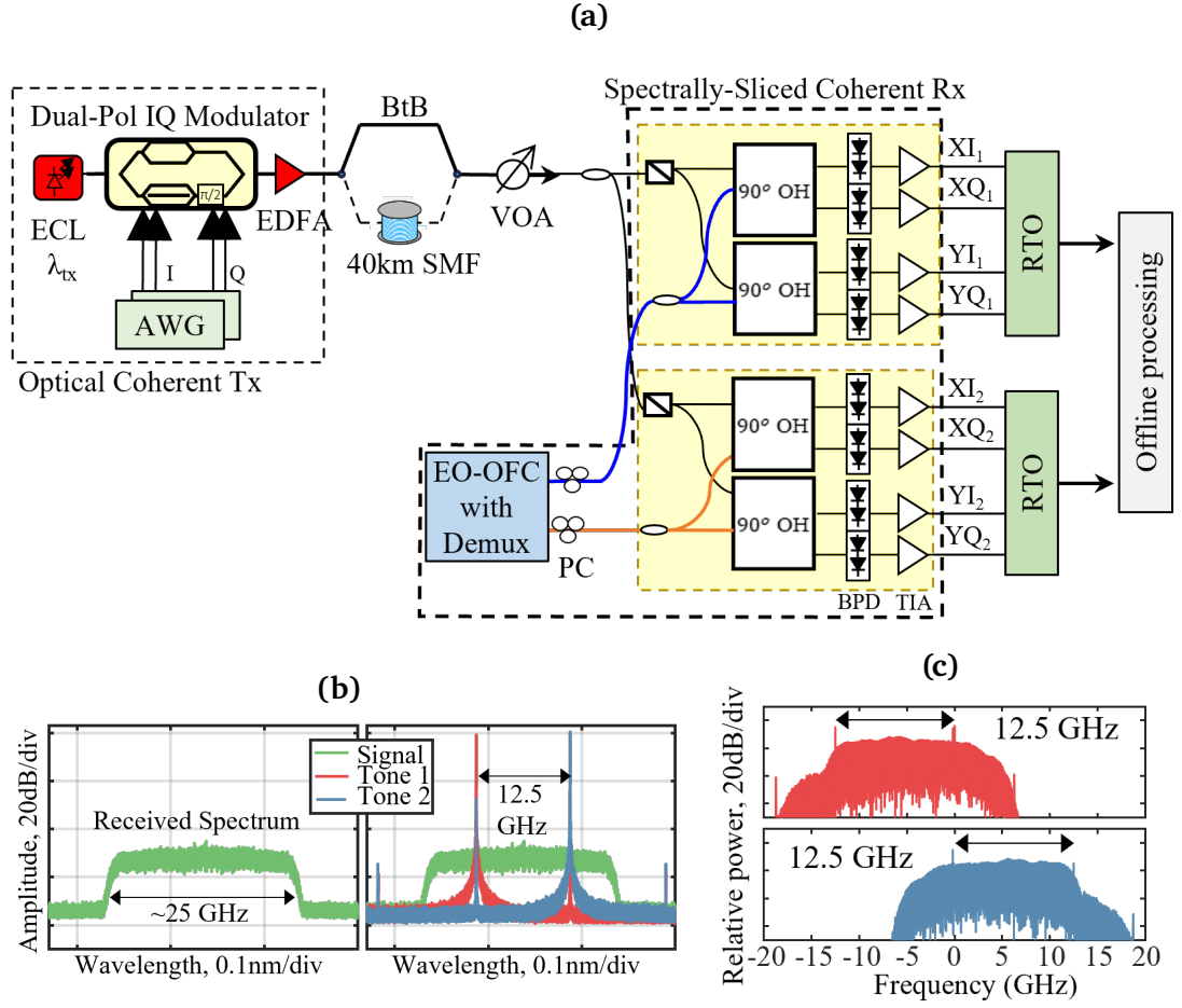
Figure 3.13: (a) Experimental setup for proof-of-concept of 25 Gbaud signal transmission. Spectrally-sliced coherent receiver diagram with two slicing operations ( N=2 ) on two different modulation schemes: SP-QPSK and DP-QPSK. The spectra in (b) illustrate the comb tones aligned to the signal spectrum, subsequently reduced into two smaller spectra, each known as a 'slice', shown in (c).
