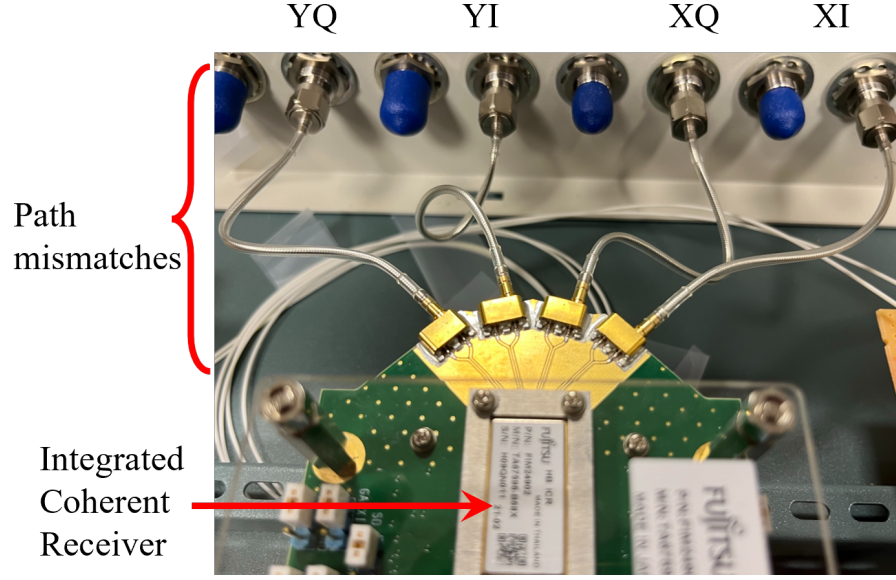
Figure 2.8: An example of the I-Q channel imbalance induced due to the path mismatches of the RF cables connecting from an integrated coherent receiver to the oscilloscopes
