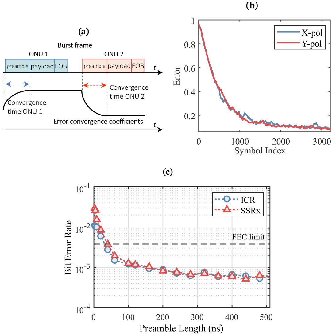
Figure 3.20: (a) Illustrative signal frame design operating in burst mode. EOB: End of burst. (b) Error convergence versus the symbol length in the equalization training in SSRx ( N=2 ). (c) BER performance of 100 Gb/s DP-QPSK using the SSRx scheme versus the preamble length at a received power of -29 dBm.
