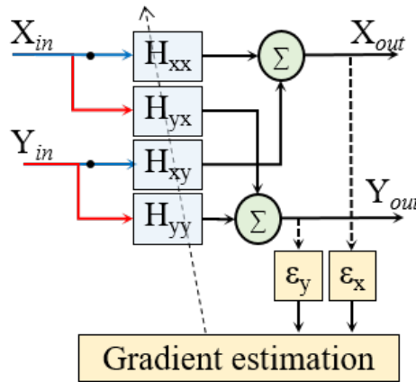
Figure 2.10: Basic structure of 2 \times 2 MIMO adaptive FIR filters.
