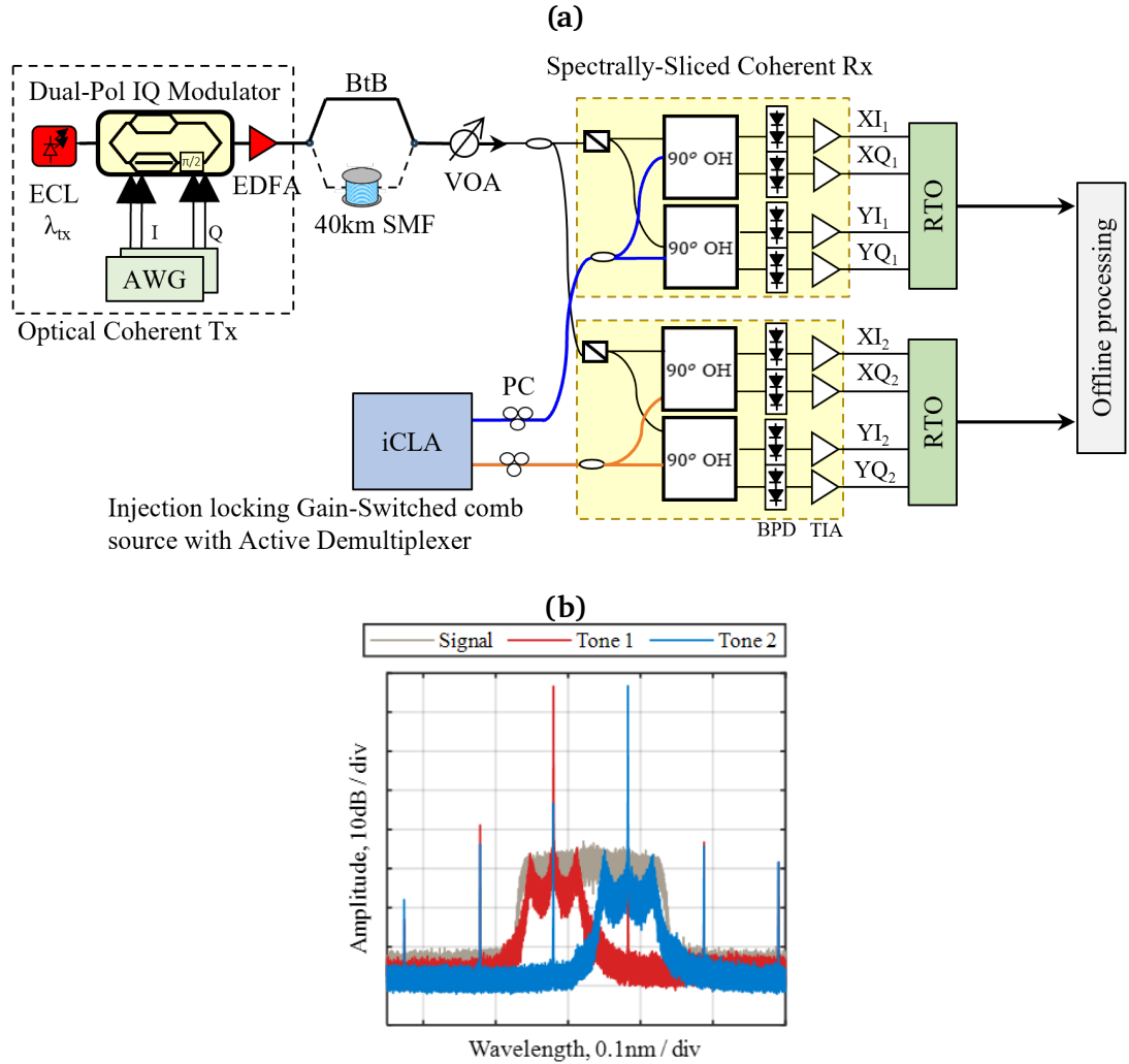
Figure 4.18: (a) Experimental setup for 100 Gb/s DP-QPSK with ( N=2 ) SSRx utilizing iCLA. (b) optical spectrum of the transmitted 100 Gb/s signal with two demultiplexed comb lines which each directly mixing with portion spectrum of the received signal.
