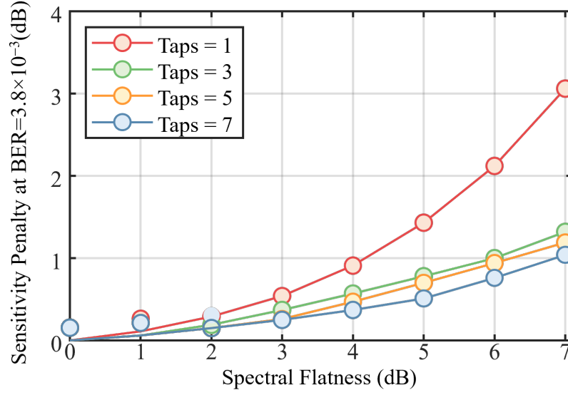
Figure 4.5: Simulated sensitivity penalty versus the spectral flatness generated by comb source relative to the spectral flatness of 0 dB.
