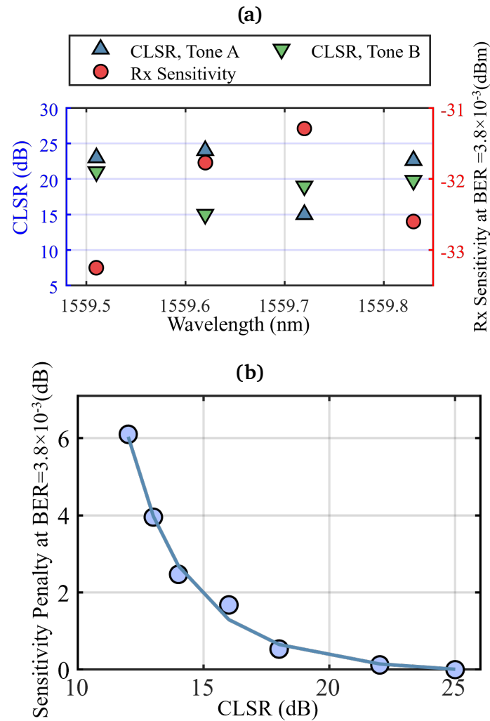
Figure 4.15: (a) Measured receiver sensitivity performance of the SSRx obtained with the IL-GS OFC. The red marker (right y-axis) represents the measured receiver sensitivity of the SSRx for four sets of comb pairs, while the CLSR measured for the demultiplexed comb tones in each pair is represented by the blue and green markers (left y-axis). (b) Sensitivity penalty measured versus CLSR of SSRx obtained with EO-OFC.
