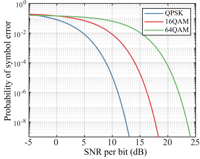
Figure 2.2: Probability of a symbol error for different QAM
