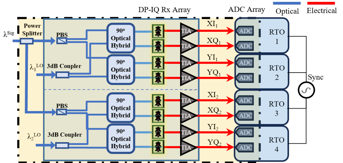
Figure 3.3: Schematic of two DP-I-Q coherent receivers configured in parallel, generating XI_n(t) , XQ_n(t) , YI_n(t) and YQ_n(t) components to the oscilloscopes.
