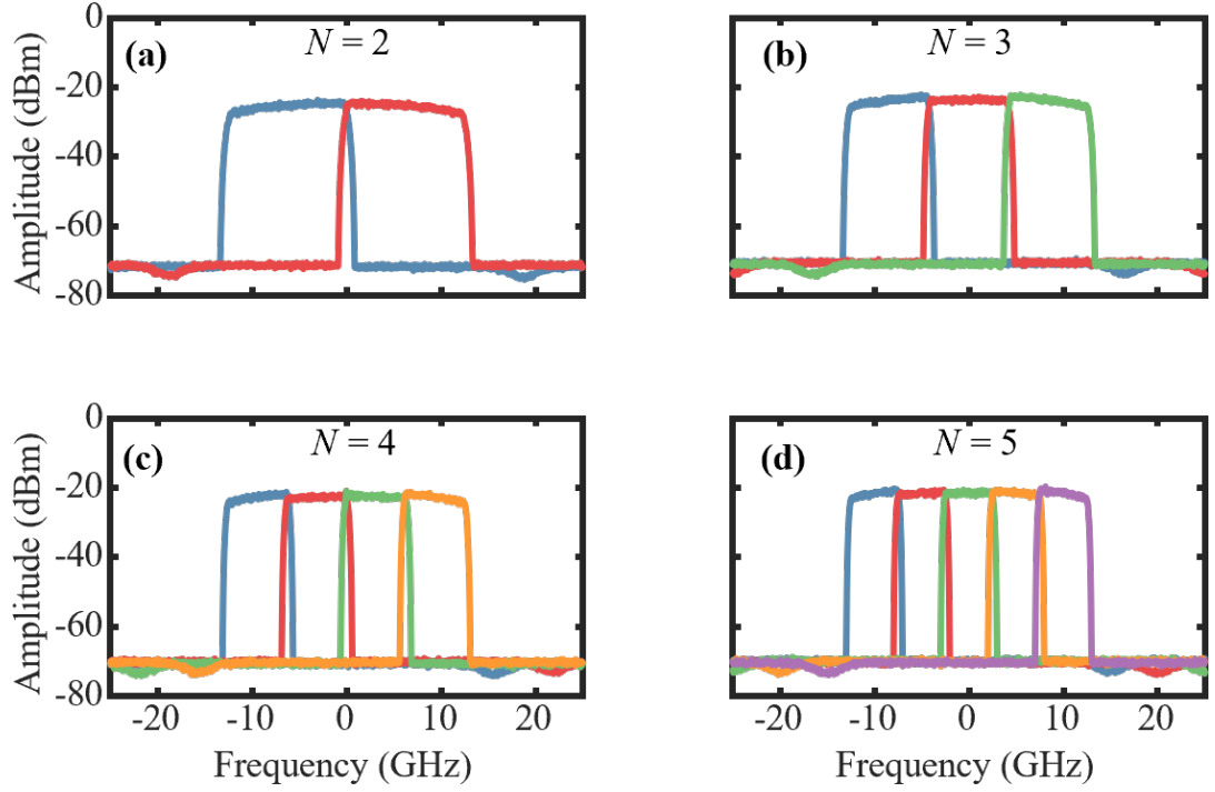
Figure 3.8: Visualisation of the stitching process of the frequency-shifted signal sliced on a 25 Gbaud signal. (a) N=2 , (b) N=3 , (c) N=4 , and (d) N=5 .
