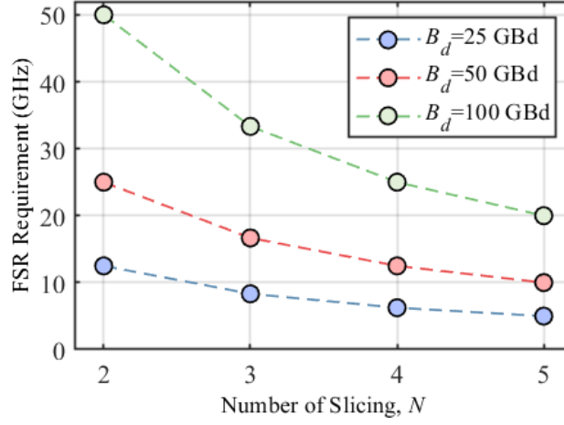
Figure 4.1: Free spectral range requirement of a comb source in spectral slicing.
