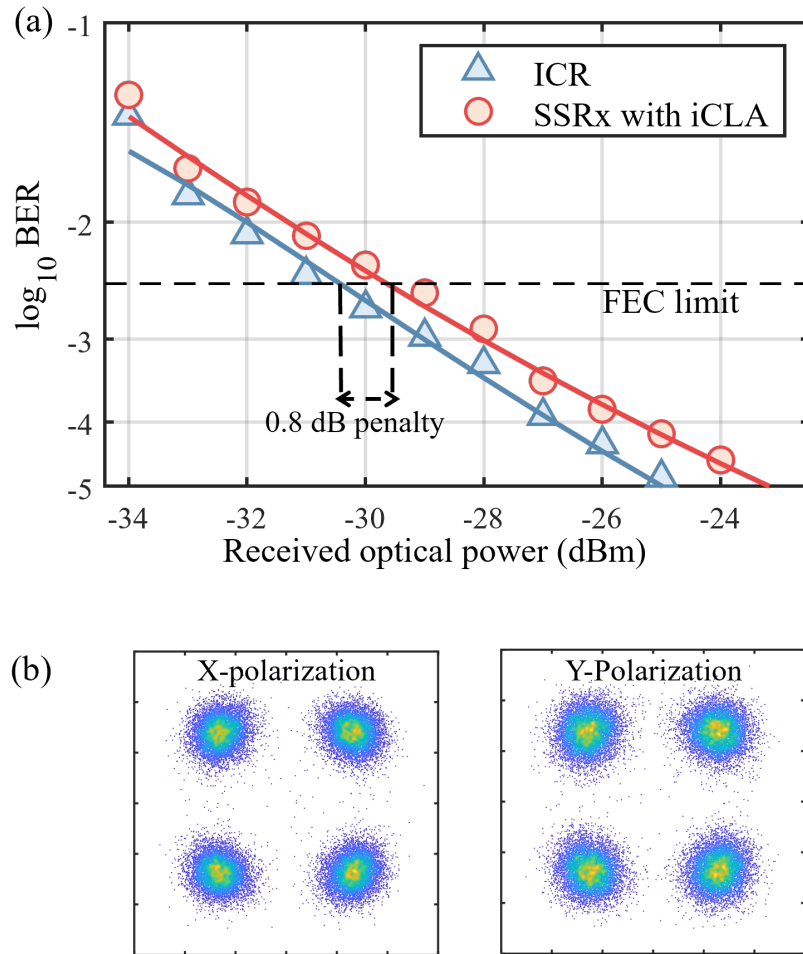
Figure 4.19: (a) 100 Gb/s DP-QPSK BER versus ROP performance over 40 km transmission distance. (b) Constellation diagram of SSRx captured at receive power of -20 dBm.
