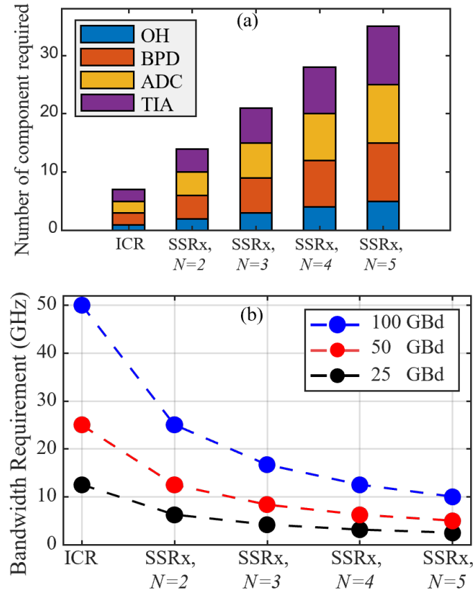
Figure 3.12: (a) The quantity of component required in the front-end receiver. (b) Receiver front-end bandwidth requirement.
