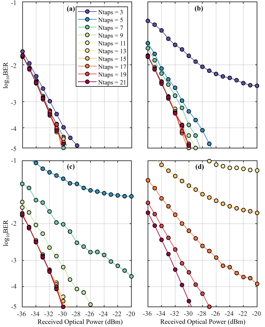
Figure 3.10: The performance of BER versus ROP with (a) 0 ps, (b) 50 ps, (c) 100 ps, and (d) 150 ps delay between slice 1 and slice 2.
