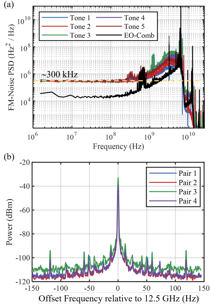
Figure 4.12: (a) Calculated FM-noise spectrums for both EO-OFC tones and for IL-GS OFC (all five main tones). (b) RF beat tones generated between the pair of comb lines for all four IL-GS OFC pairs captured at 12.5 GHz offset frequency.
