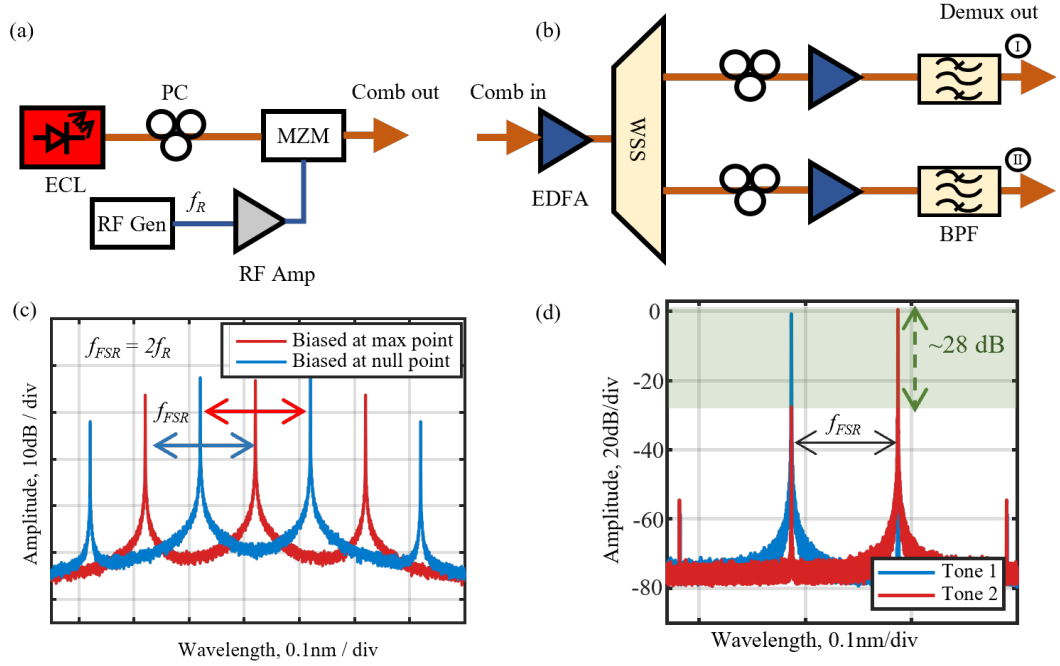
Figure 3.2: (a) Experimental setup of an optical frequency comb based on a single-drive MZM. RF Gen.: RF Source Generator. (b) The experimental setup for comb signal demultiplexing using the wavelength selective switch based on liquid crystal on silicon technology. (c) The optical spectrum of the OFC was captured using an optical spectrum analyzer (OSA) with resolution bandwidth of 20 MHz. The two traces represent two different bias settings of the EO-modulator to generate the frequency comb. (d) The optical spectrum of the comb after demultiplexing. The comb line suppression ratio is measured based on the difference between the peak power of the demultiplexed comb line with the adjacent lines.
