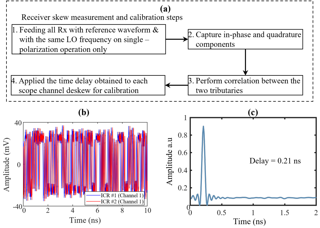
Figure 3.4: (a) Block diagram of processing steps performed to calibrate timing delay between receiver channels. (b) Captured experimental waveforms of channel 1 (in-phase tributary) from the two separate coherent receivers. (c) Cross-correlation response of the captured waveforms between coherent receivers in each lane.
