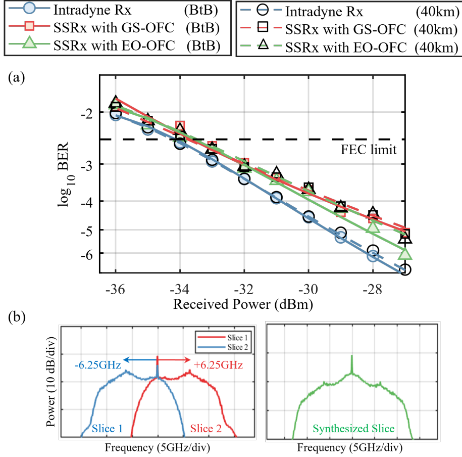
Figure 4.14: (a) Receiver power sensitivity performance of the conventional and proposed SSRx for 25 Gbaud QPSK signals. (b) Digitized and frequency-shifted by \pm 6.25 GHz spectral slices (red, blue) and synthesized 25 Gbaud data signal (green) spectra.
