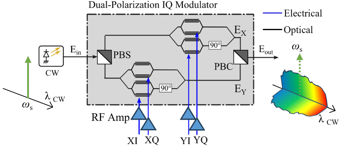
Figure 2.3: General structure of a multi-format optical coherent transmitter employing amplitude and phase modulations in two polarizations of lightwave. Inset: Illustration of modulated signal on a carrier frequency spectrum.
