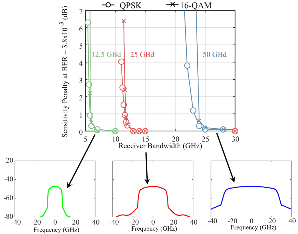
Figure 2.21: The receiver sensitivity tolerance with varied receiver bandwidths for three different baud rate operation. Insets show the associated spectra of the signal from each operating baud rate.
