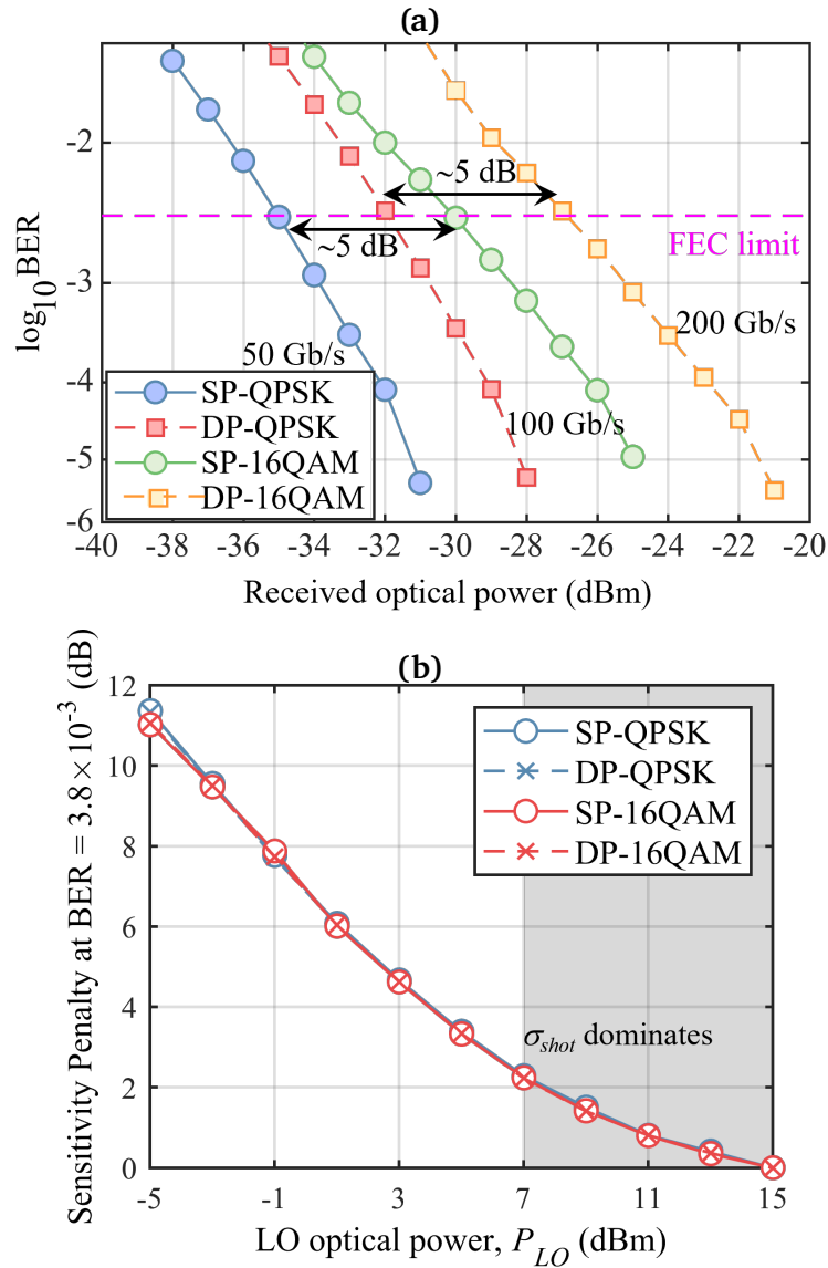
Figure 2.16: (a) BER versus received optical power for QPSK and 16QAM modulation formats on different transmission links with single-polarization, and dual-polarization operation. (b) Sensitivity penalty as a function of the LO power ( P_{LO} ) in the BtB link for different modulation formats.
