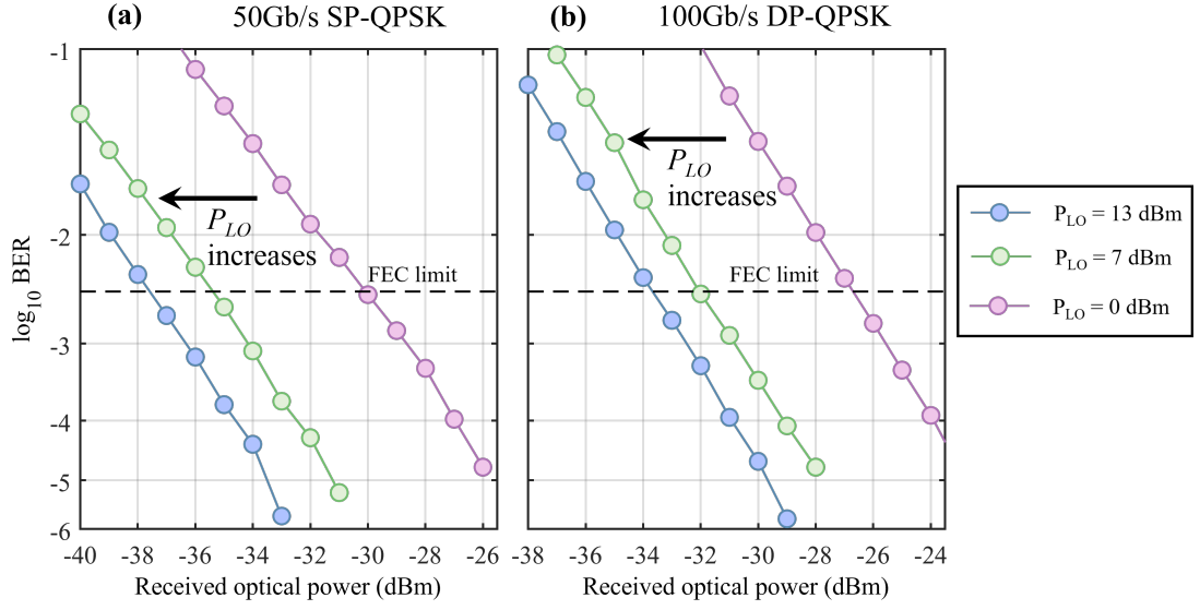
Figure 2.20: Experimental results of the ICR sensitivity performance over 40 km G.652 standard optical fiber.
