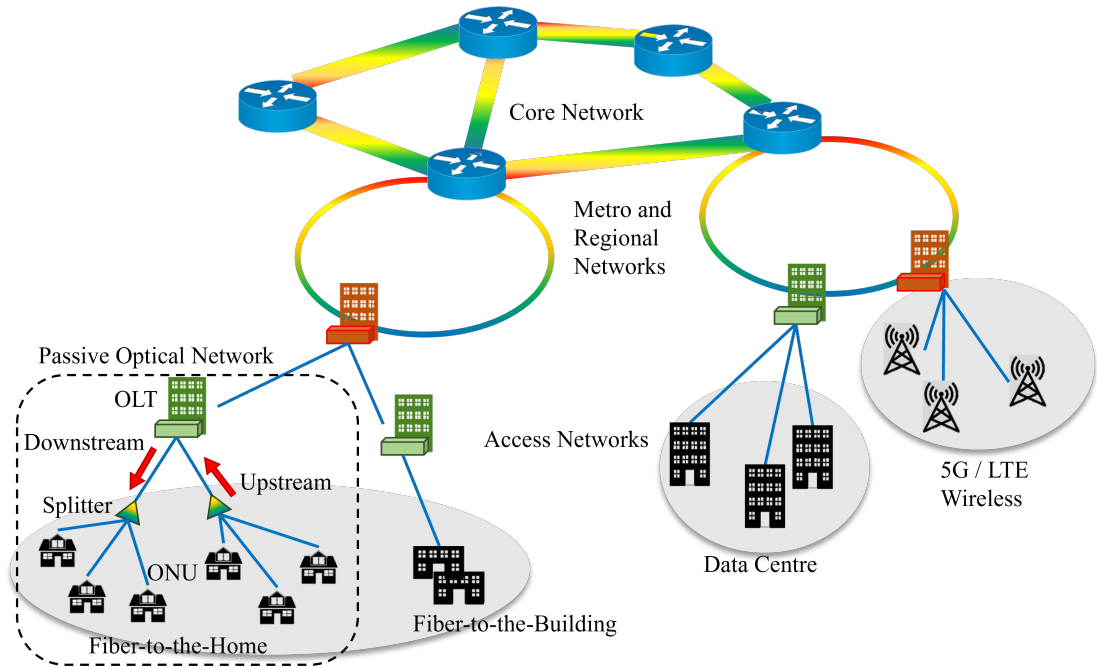
Figure 1.1: Optical fiber communication topology including core, metropolitan, data centre interconnect, and access network. OLT: Optical line terminal, ONU: Optical network unit, 5G: Fifth Generation, LTE: Long-term evolution.
