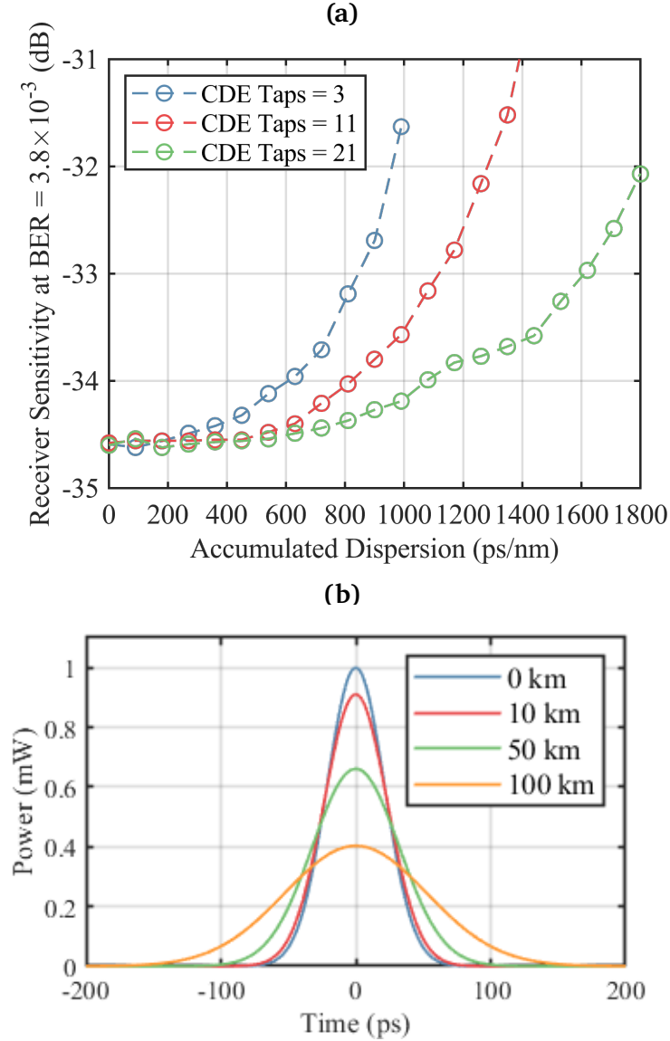
Figure 2.17: (a) Performance of the coherent receiver sensitivity against accumulated CD with varied number of taps of chromatic dispersion equalizer. (b) Dispersion-induced broadening of a Gaussian pulse in a fiber transmission at different fiber lengths.
