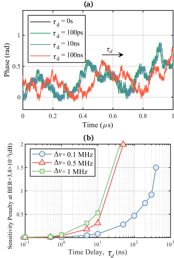
Figure 4.7: (a) Phase noise traces of comb line ( \Delta\nu=100 kHz) with delayed versions of itself. (b) Simulated sensitivity penalty versus applied time delay for three different linewidths.
