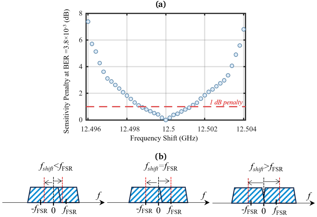
Figure 3.15: (a) Receiver sensitivity measured as a function of frequency shift for signal reconstruction. (b) Illustration of the impacts of frequency shift on the reconstructed spectra.
