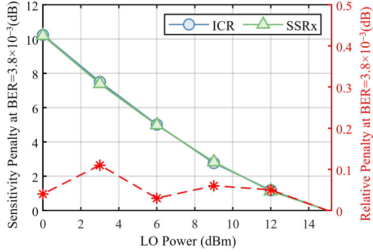
Figure 4.4: Simulated receiver sensitivity penalty as a function of local oscillator power. The red curve indicates the relative sensitivity penalty between the ICR and SSRx detection schemes.
