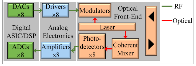
Figure 1.3: Simplified diagram of the building blocks of a fully coherent transceiver
