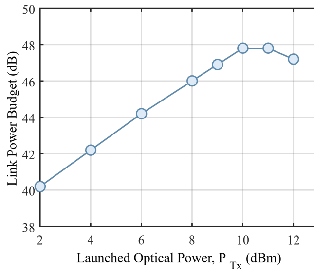
Figure 2.23: Optical link budget as a function of launch power.
