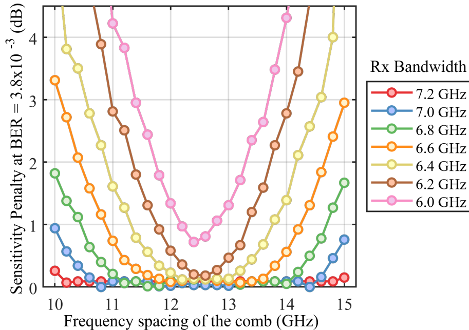
Figure 3.11: Receiver sensitivity penalty performance in 25 Gbaud QPSK signal transmission versus the frequency spacing of the comb with varied receiver's bandwidth.
