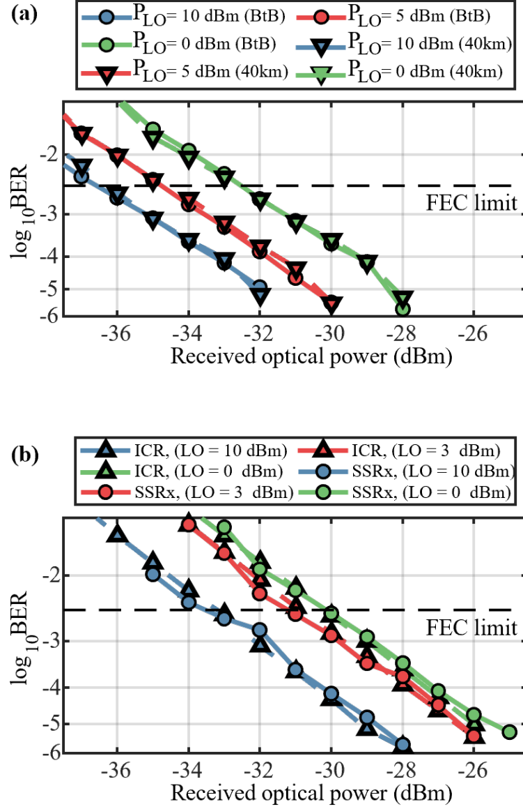
Figure 3.14: (a) Experimental results of BER performance versus ROP for the different optical power per comb line. (a) 50 Gb/s SP-QPSK comparing the SSRx performance over BtB and 40 km fiber link. (b) 100 Gb/s DP-QPSK over 40 km fiber comparing the ICR with SSRx detection scheme.
