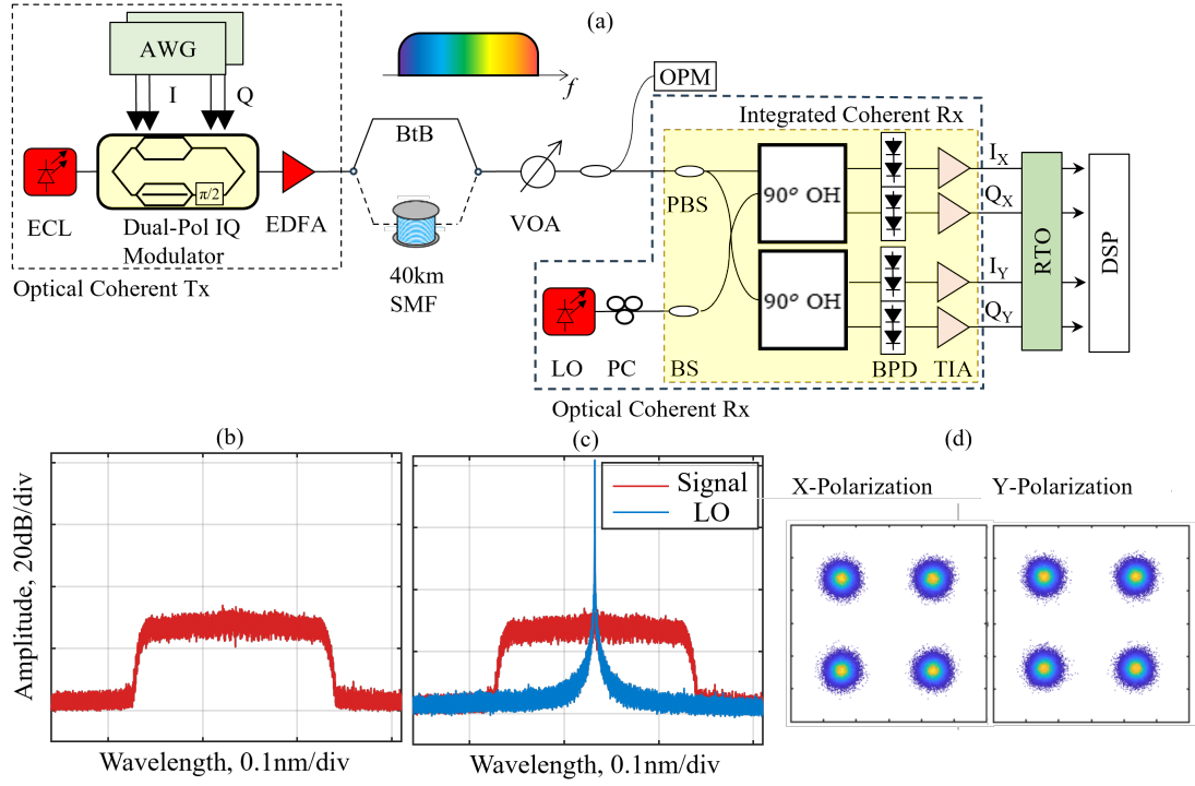
Figure 2.18: (a) Experimental setup for optical coherent transmission system of 50 and 100 Gb/s of single- and dual-polarization QPSK respectively. (b) Captured optical spectrum of transmitted signal centered at 1553.1 nm wavelength. (c) Optical spectrum used for comparison between transmitted signal with LO. (d) Recovered constellation of DP-QPSK at -22 dBm receive power.
