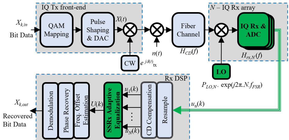
Figure 3.6: Block diagram of an SSRx simulation system setup.
