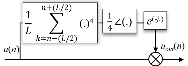
Figure 2.13: Block processing of CPR based on feed-forward estimation. \angle(\cdot) represents the phase of complex number.
