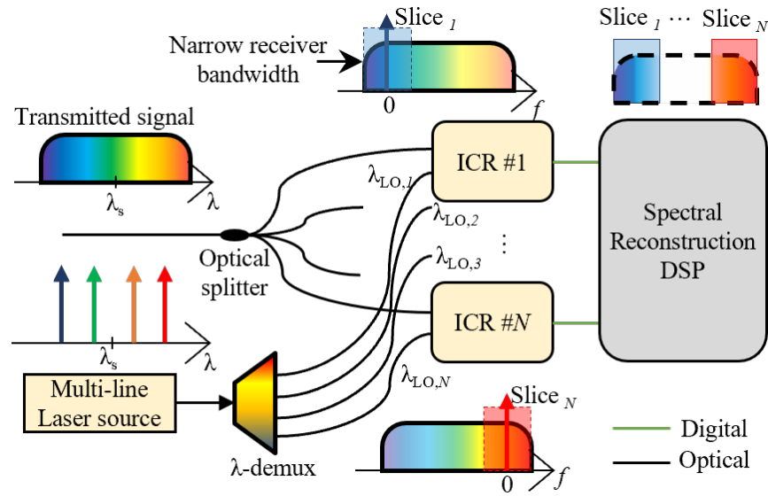
Figure 3.1: Schematic diagram of a spectrally-sliced optical coherent receiver. The received signal is split by a factor of N via an optical splitter and fed into an array of N -integrated coherent receivers. The multi-optical lines are separated by a wavelength de-multiplexer and act as LO that mixes with a portion of signal frequencies. After sub-signal photodetection and ADC readout inside the ICRs, N -complex signal slices are generated. Following the sub-ADC sampling, the whole signal spectrum can be reconstructed by "stitching" together each sampled slice using DSP; thus recovering the received signal.
