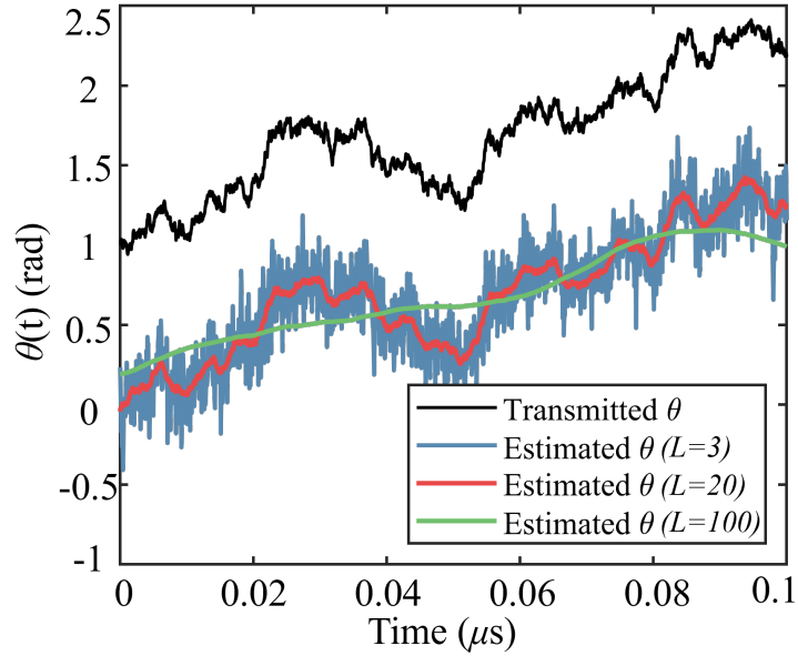
Figure 2.14: Simulated Wiener laser phase noise by using system modelling presented in Section 2.4.1 later. The total linewidth of the system was set to 100 kHz as shown in black trace. The estimated phase was generated by using the Viterbi-Viterbi algorithm with different symbols averaging L .
