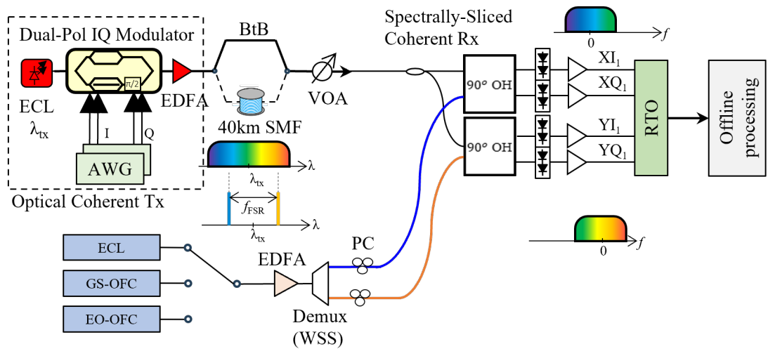
Figure 4.13: (a) Experimental setup for 50 Gb/s SP-QPSK with ( N=2 ) SSRx over 40 km of SMF. The GS-OFC used in this experiment is based on Pilot Photonics LYRA-OCS-1000, while the Finisar Waveshaper (WSS) is used as the comb de-multiplexer.
