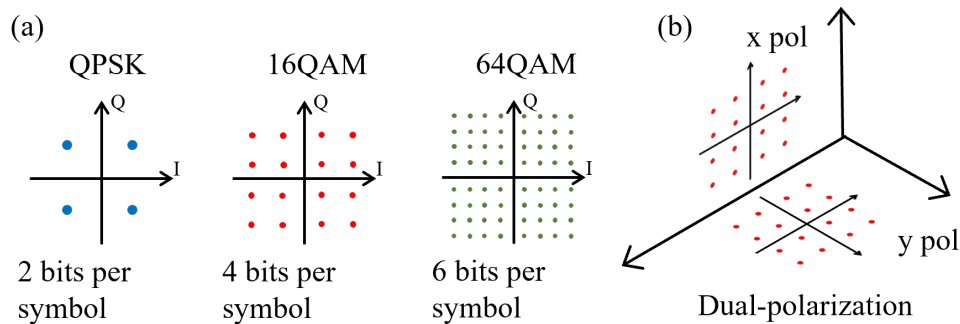
Figure 2.1: Constellation diagrams showing the bit-rate scaling in various dimensions, including (a) advanced modulation formats by employing more bits in a symbol, and (b) capacity doubling by multiplexing the signal in dual-polarization of the lightwave.
