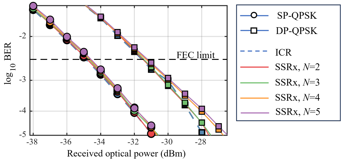
Figure 3.7: Simulated BER versus ROP for 50 Gb/s SP-QPSK and 100 Gb/s DP-QPSK. Solid lines refer to a spectral slicing receiver with different number of slicing operation N , and the dashed lines refer to a conventional coherent receiver, ICR.
