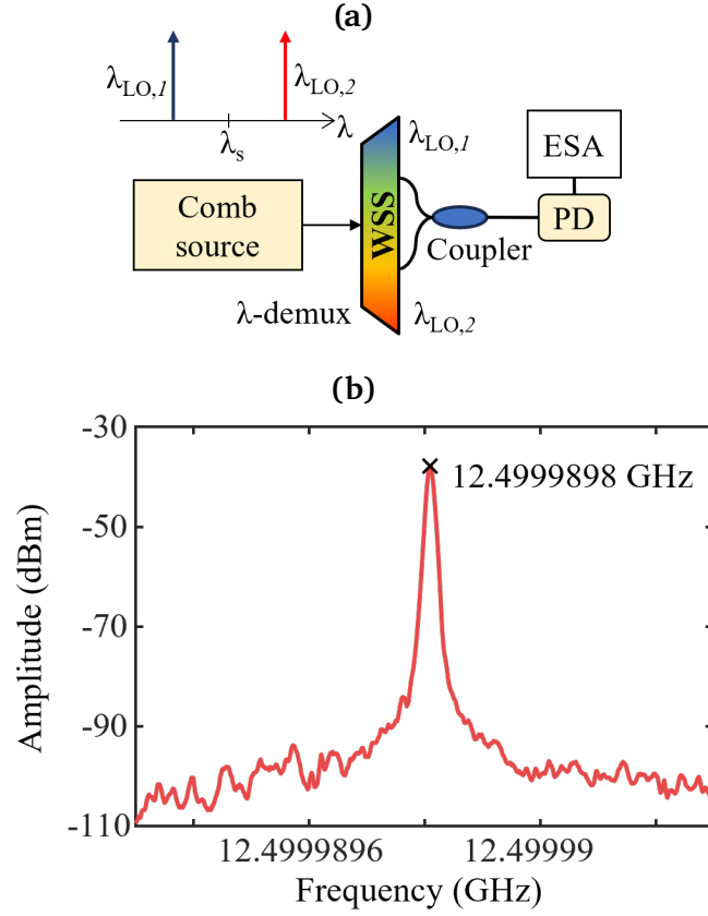
Figure 3.16: (a) Setup for measuring the free spectral range of the comb. (b) The spectra of the beating tone captured by an ESA operating at the resolution bandwidth of 3 Hz.
