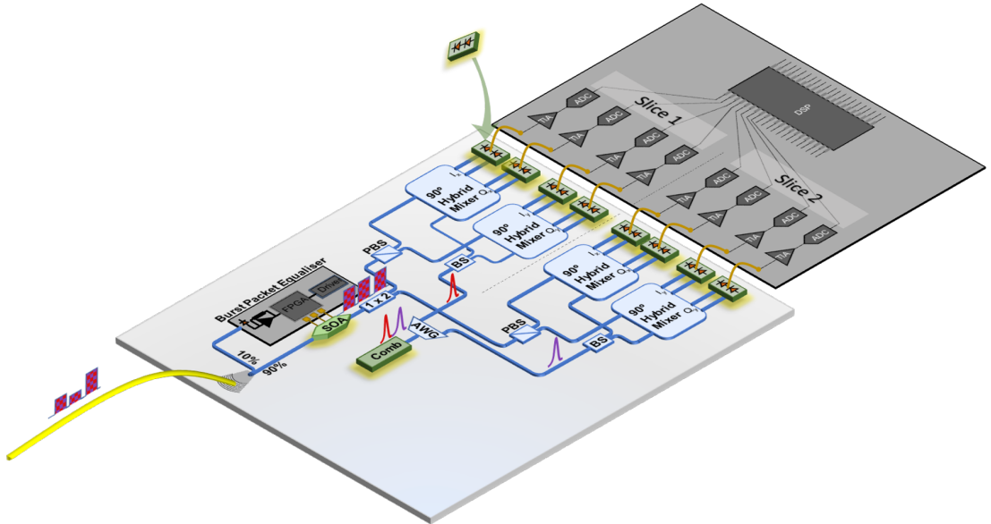
Figure 5.1: Schematic of an integrated spectrally sliced coherent receiver ( N=4 ) envisioned for PON upstream transmission.
