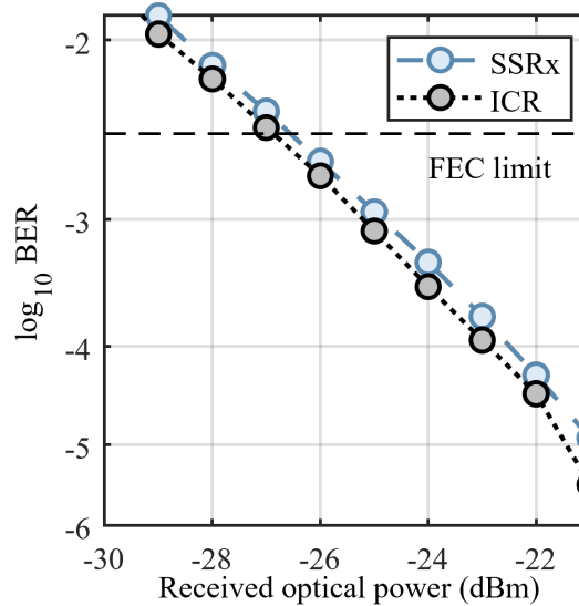
Figure 3.21: Sensitivity for 200 Gb/s DP-16QAM employing SSRx (N=2) over 40 km.
