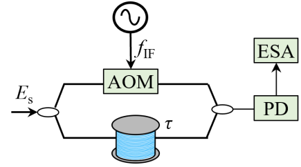
Figure 2.5: Delayed self-heterodyne method to measure the FM-noise of a laser. AOM: Acousto-optic modulator. ESA: Electrical spectrum analyzer.
