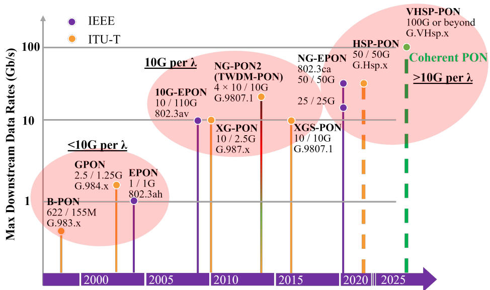
Figure 1.2: Evolution of PON standardized technology.
