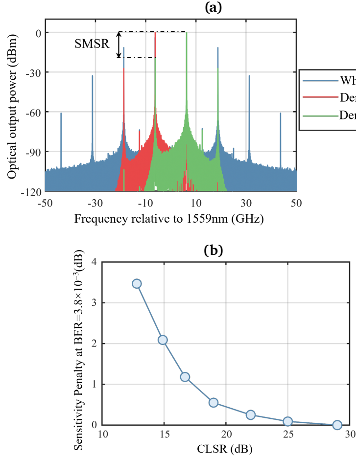
Figure 4.8: (a) Spectra were captured for the whole frequency comb (blue) and two isolated combs filtered by de-multiplexer with finite bandwidth (red and green traces). (b) Simulated sensitivity penalty versus CLSR for SSRx detection.
