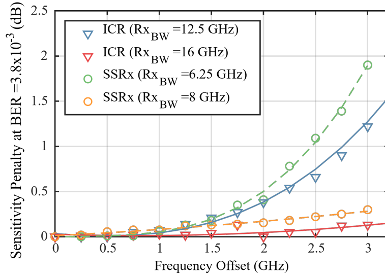
Figure 3.19: Tolerances to frequency offsets with varied bandwidth of the receiver.
