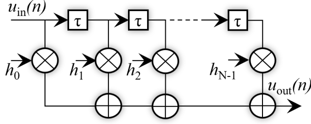
Figure 2.9: Basic structure of an FIR filter with a length of N taps
