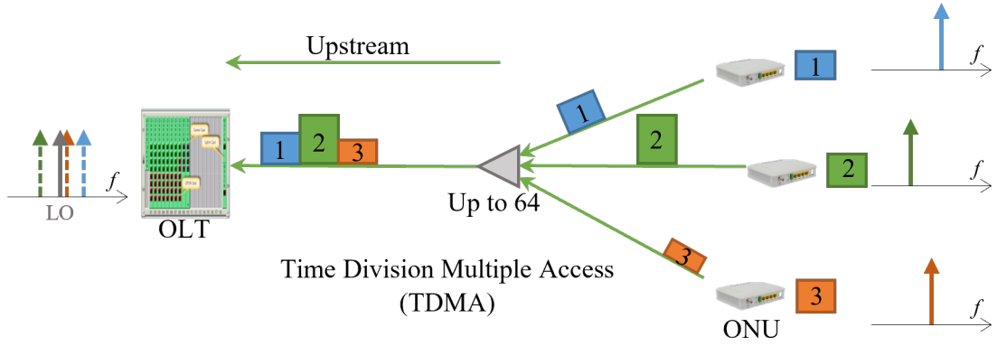
Figure 3.18: Implementation diagram of multipoint-to-point link transmission of PON according to ITU-T standard.
