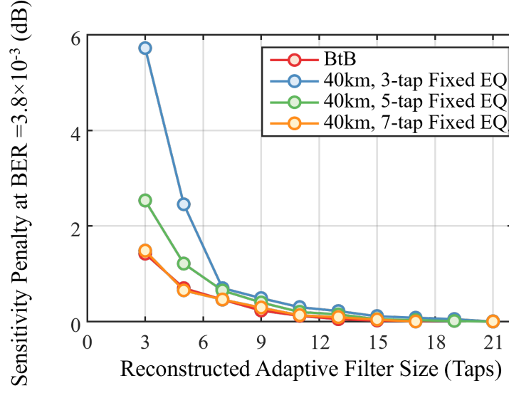
Figure 3.17: Receiver sensitivity penalty as a function of the number of taps required for the reconstruction adaptive equalizer in BtB and over 40km fiber link.
