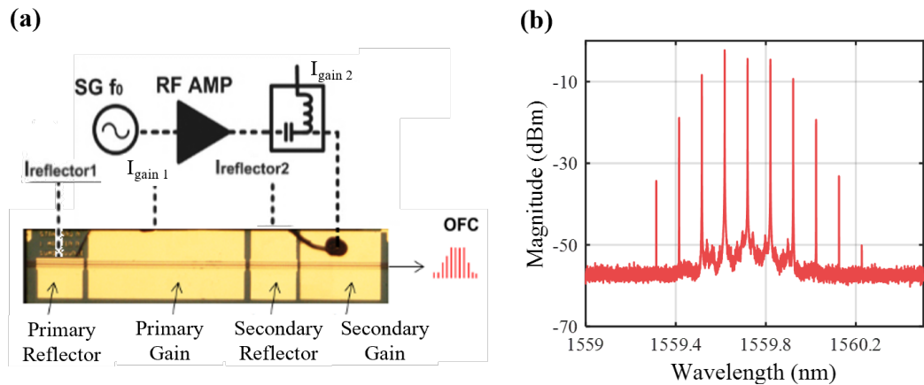
Figure 4.11: (a) Schematic diagram of an injection-locking gain-switched Fabry-Pérot (FP) laser-based frequency comb. (b) The output optical spectrum of the comb source with 12.5 GHz frequency spacing.
