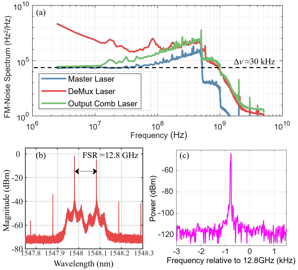
Figure 4.17: (a) Phase noise measurements comparing the comb signal with the primary laser, (b) optical spectrum of the output comb signals with frequency spacing of 12.8 GHz and each having CLSR of more than 30 dB, (c) resultant beating tone between the two output tones generated at a frequency of 12.8 GHz.
