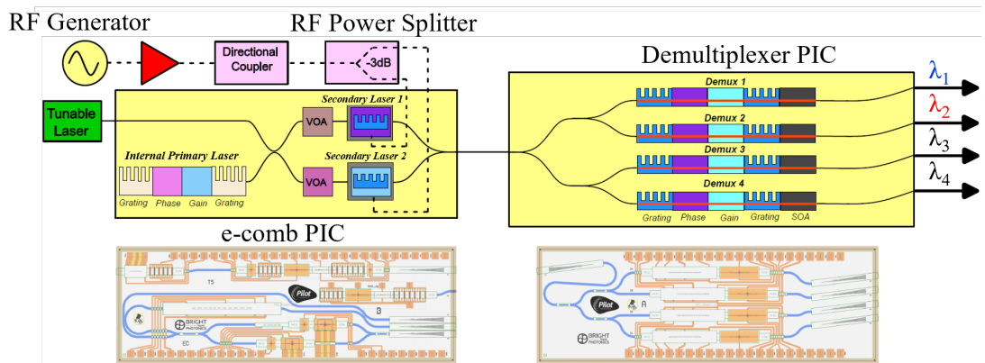
Figure 4.16: The schematic and fabricated PIC layout of both comb source and de-multiplexer respectively.
