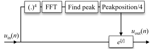
Figure 2.11: Block processing of frequency offset estimation technique based on peak power search.
