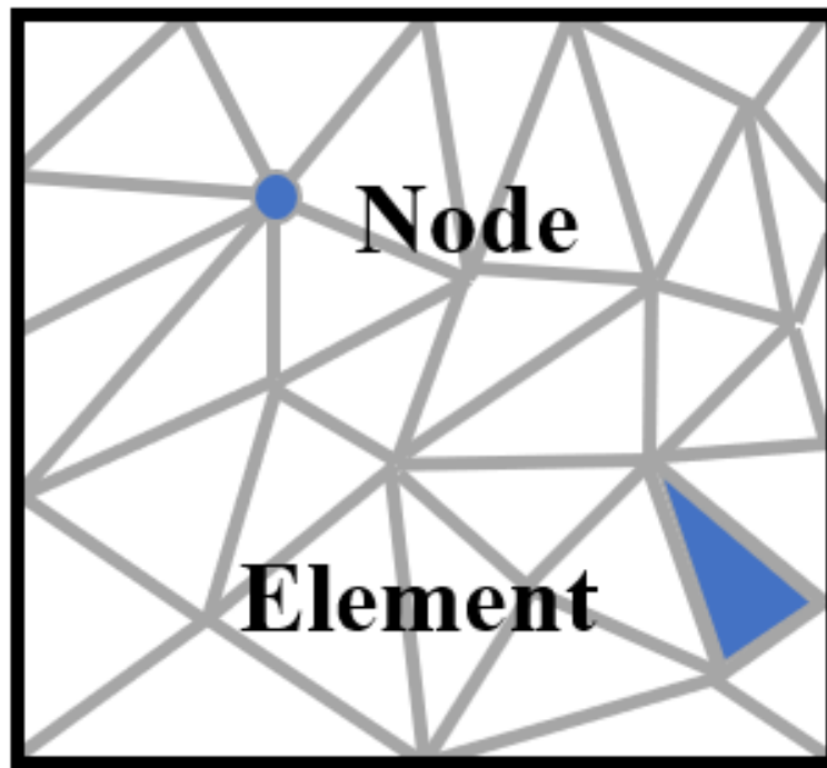
Figure 1.12 Schematic representation of a typical triangular mesh used in a 2D domain.
