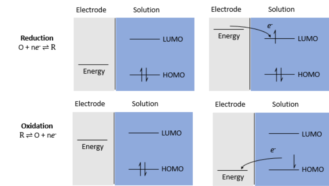
Figure 1.3 Diagram of electron transfer and energy levels at an electrode/solution interface for reduction and oxidation processes. LUMO is the lowest unoccupied molecular orbital and HOMO is the highest occupies molecular orbital. An applied voltage is required to surmount the energy barrier and allow electron transfer.
