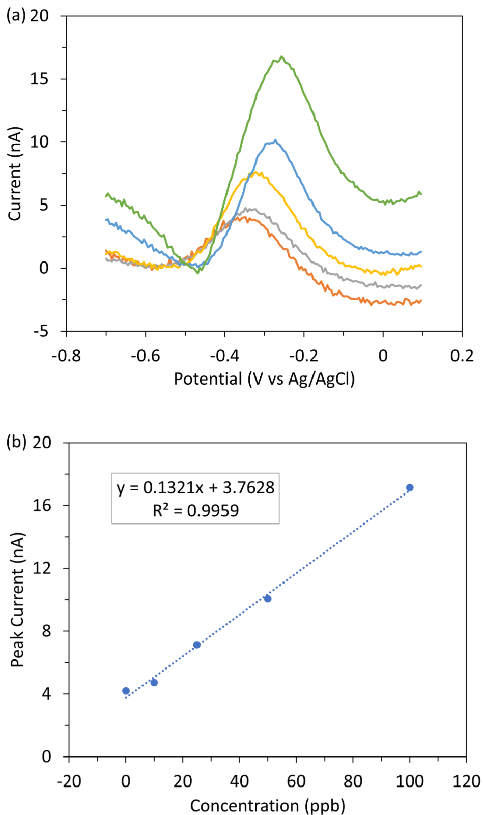
Figure 4.6 (a) Square wave stripping voltammogram for varied concentration of lead nitrate in unmodified tap water at gold IDE arrays where the protonator was held at 1.55 V. (b) Calibration plot of lead stripping peak current vs. lead concentration.
