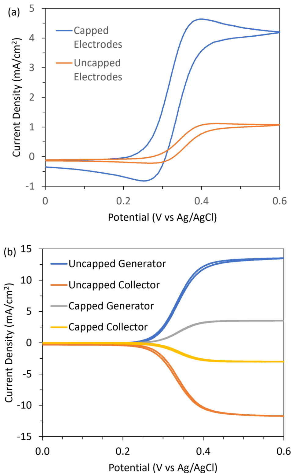
Figure 2.17 Typical CVs of 1 mM FCA in 10 mM PBS from 0.0 to 0.6 V vs Ag/AgCl (sat. KCl) at 50 mV s -1 at 2 \mu m gold bands with 2 \mu m inter-electrode gaps uncapped and capped electrode where (a) the Collector electrode is left unconnected while the Generator is swept from 0 to 0.6 V vs Ag/AgCl (sat. KCl), Non GC Mode, and (b) the Collector is held at 0.1 V Ag/AgCl (sat. KCl) while the Generator is swept from 0 to 0.6 V Ag/AgCl (sat. KCl), GC Mode.
