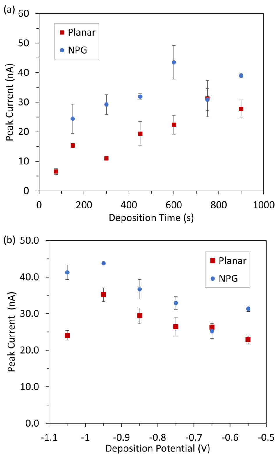
Figure 3.7 SWV peak current responses for 10 ppb Lead Nitrate in 0.1 M Acetate Buffer pH 4.6 for (a) deposition at -0.95 V vs Ag/AgCl (sat. KCl) with varied time and (b) deposition for 600 s with varied deposition potential at planar and NPG-modified 20 \mu m gold micro-disc arrays.
