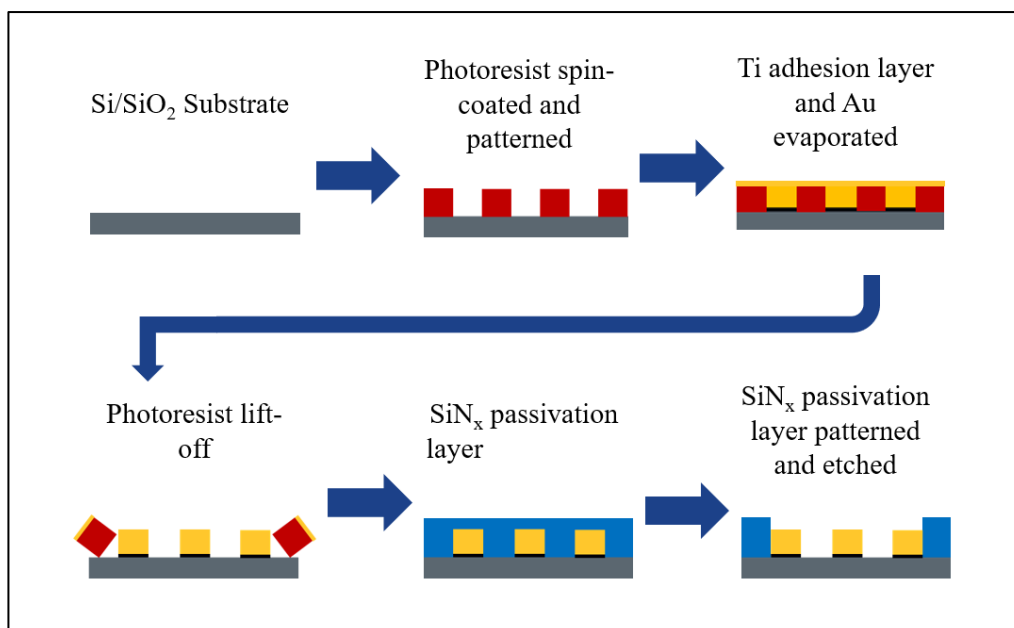
Figure 2.2 Process flow diagram for the fabrication of gold microbands using photolithographic techniques.
