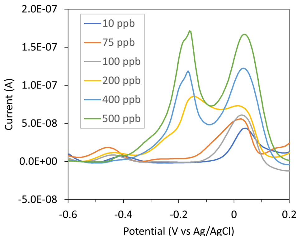
Figure 3.6 SWV of 10 ppb - 500 ppb lead(II) nitrate in 0.1 M acetate buffer pH 4.6 deposited at -0.95 V vs Ag/AgCl (sat. KCl) for 600 s at NPG-modified 20 \mu m micro-disc arrays.
