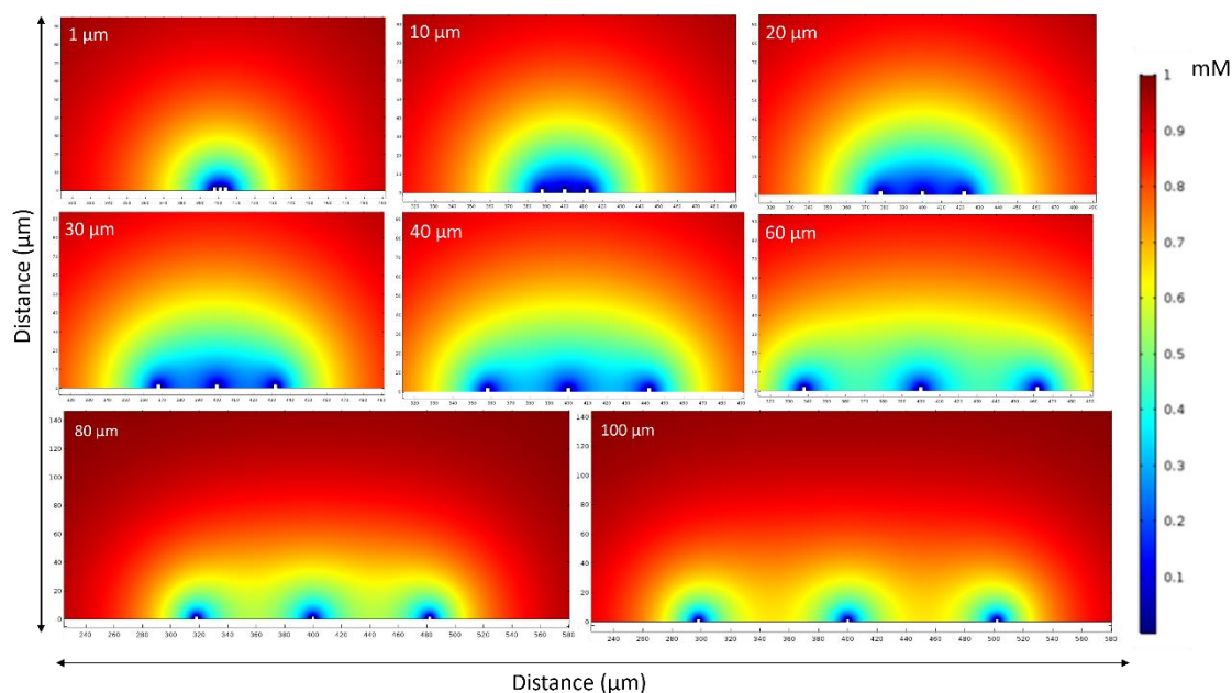
Figure 2.4 Cross-sectional view of 2D simulations of 1 mM FCA in 10 mM PBS diffusion profiles corresponding to CVs with 3 \times 2 \mu\text{m} bands with varied inter-band spacing indicated in each tile. The images represent the condition at the end of a sweep to the potential 0.6 V vs Ag/AgCl (sat. KCl) at 50 \text{ mV s}^{-1} . The scale bar on the right-hand side of the figure represents the concentrations of \text{Fe}^{2+} and \text{Fe}^{3+} , where 1 mM (red) is \text{Fe}^{2+} in the bulk solution and as it is oxidised at the electrode surface it is converted to \text{Fe}^{3+} (blue).
