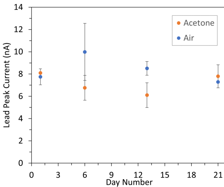
Figure 4.8 Plot of lead peak currents from SWV voltammograms following analysis in 10 ppb lead nitrate in tap water where the protonator was held at 1.55 V for arrays aged in acetone and air. Each measurement was carried out in triplicate at the same array.
