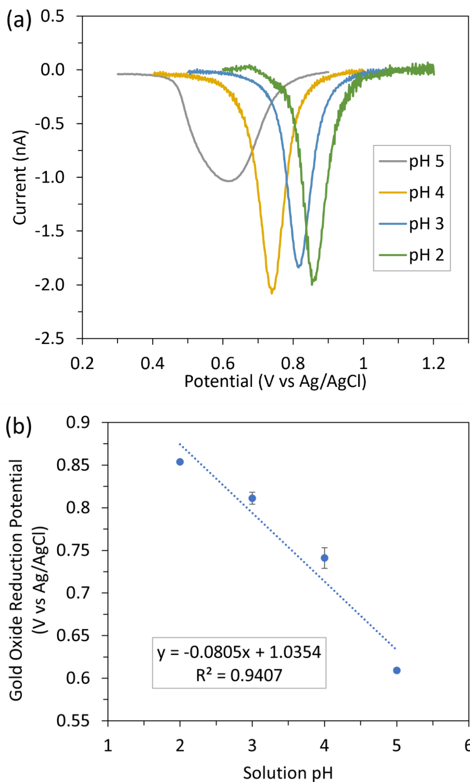
Figure 4.1 (a) The gold oxide reduction peak in CVs recorded from 0.0 V to 1.5 V vs Ag/AgCl (sat. KCl) at 50 mV s -1 at gold IDE arrays in a series of pH buffers. For these scans, only one side of the IDE array was used, the other was left unbiased. (b) Calibration plot of gold oxide reduction peak vs. solution pH.
