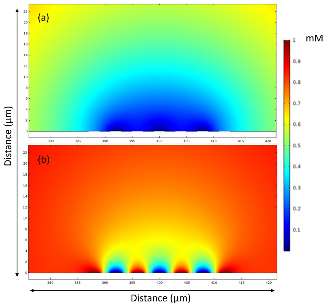
Figure 2.9 Cross-sectional view of 2D simulations of 1 mM FCA in 10 mM PBS diffusion profiles corresponding to CVs in (a) non GC mode where the generator electrode was swept from 0.0 V to 0.6 V while the collector electrode was unconnected and (b) GC mode where the generator was swept from 0.0 V to 0.6 V vs Ag/AgCl (sat. KCl) at 50 \text{ mV s}^{-1} while the collector was held at 0.1 V vs Ag/AgCl (sat. KCl). The images represent the condition at the end of a sweep to the potential 0.6 V vs Ag/AgCl (sat. KCl). The scale bar on the right hand side of the figure represents the concentrations of \text{Fe}^{2+} and \text{Fe}^{3+} , where 1 mM (red) is \text{Fe}^{2+} in the bulk solution and as it is oxidised at the electrode surface it is converted to \text{Fe}^{3+} (blue).
