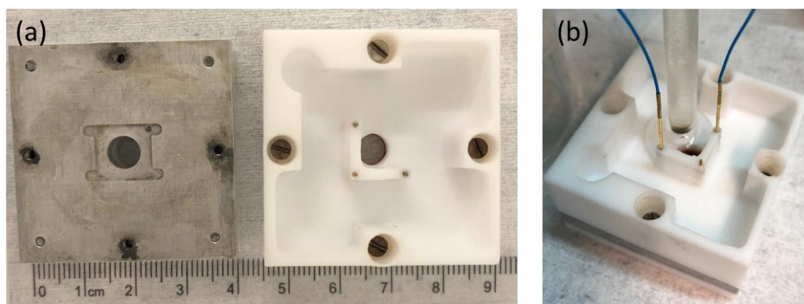
Figure 2.3 Image of a typical electrochemical cell set-up: (a) Cell components with measurements and (b) Cell in use with pins connecting to the working and counter electrodes and an external Ag/AgCl (sat. KCl) reference electrode
