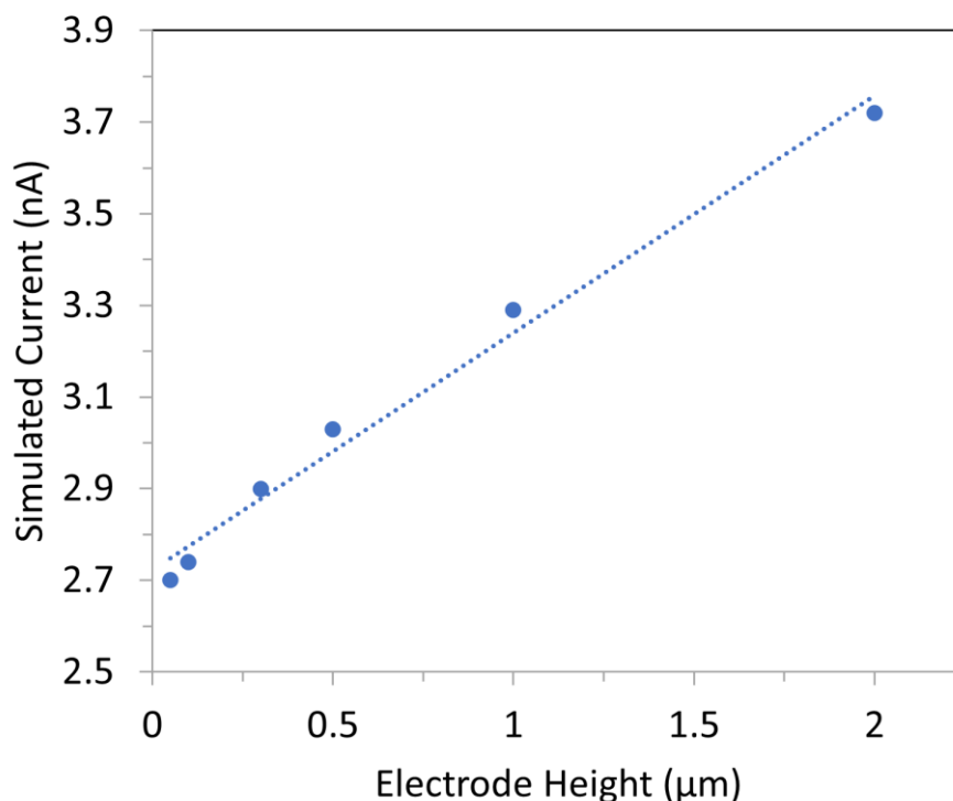
Figure 2.8 Plot of simulated limiting current for various electrode height of 2 \mu\text{m} bands in an array with 100 \mu\text{m} inter-electrode gaps. Simulated current data point were taken from the limiting current of simulated CVs swept from 0 V to 0.6 V vs Ag/AgCl (sat. KCl) at 50 \text{mV s}^{-1} .
