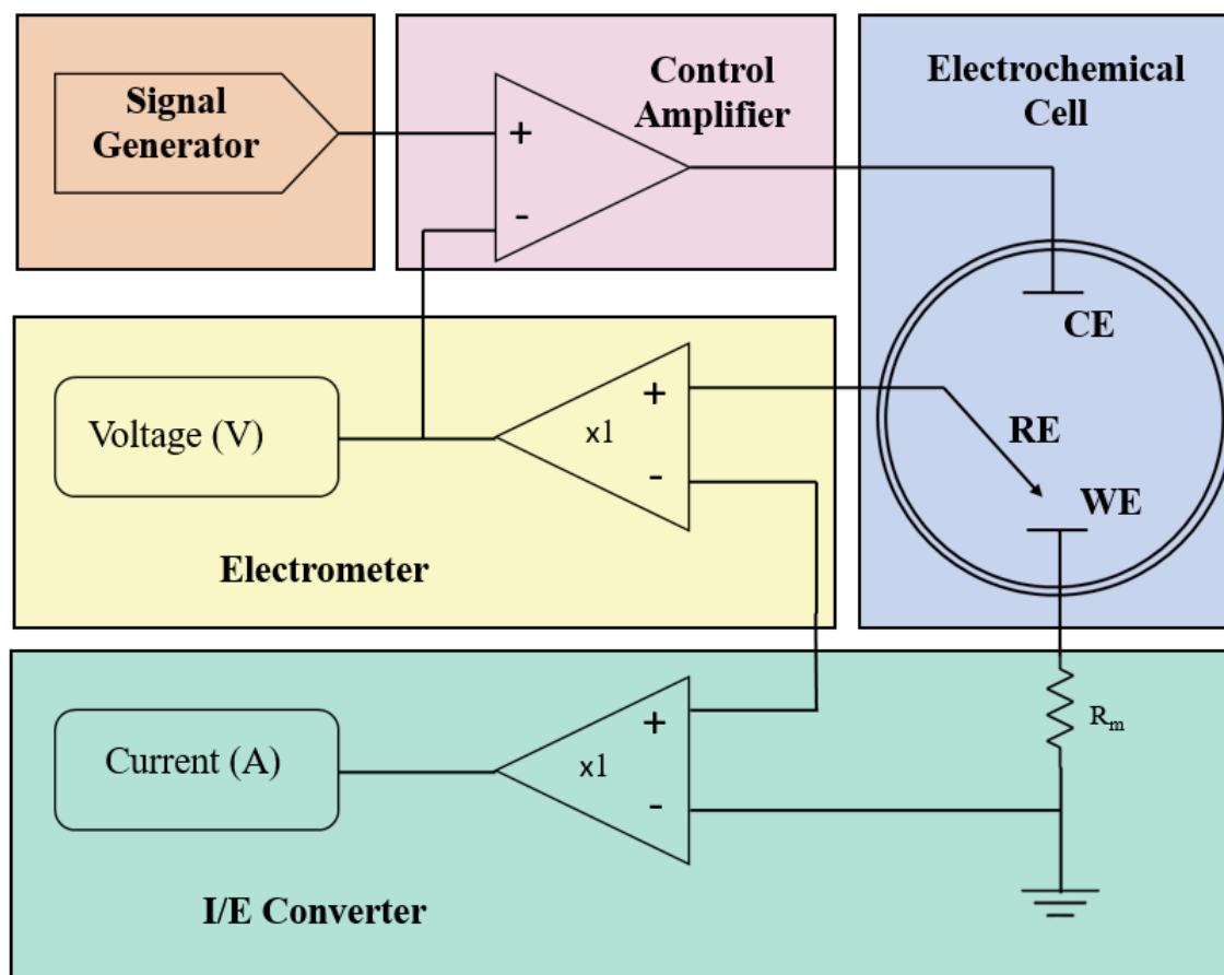
Figure 1.2 A simplified schematic diagram of a potentiostat for a three-electrode set-up, reproduced from 14 .
