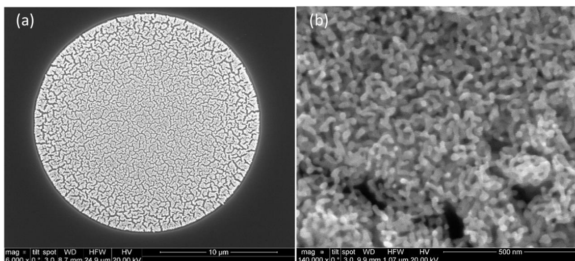
Figure 1.17 SEM Images of (a) NPG deposited at a 20 \mu\text{m} micro-disc electrode and (b) high mag of NPG deposited in 20 \mu\text{m} micro-disc electrodes
