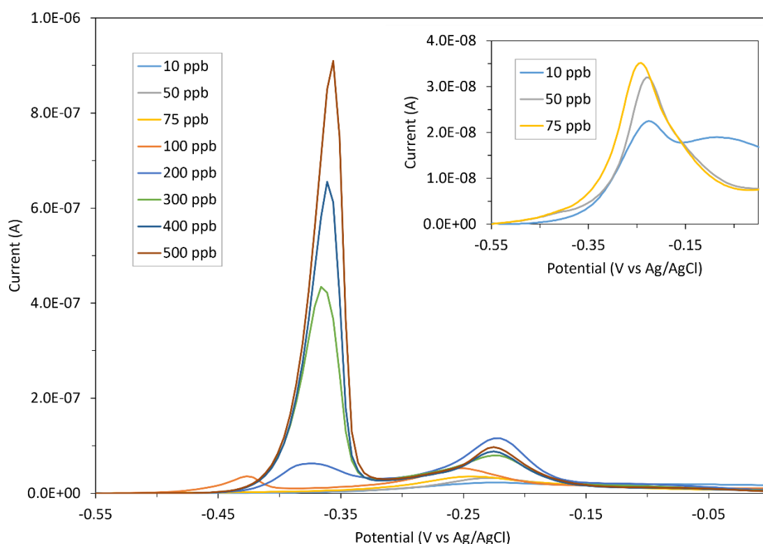
Figure 3.4 SWV of 10 ppb - 500 ppb lead(II) nitrate in 0.1 M acetate buffer pH 4.6 deposited at -0.95 V vs Ag/AgCl (sat. KCl) for 600 s at planar gold 20 \mu m micro-disc arrays. Insert highlights the response of the lower concentration range of 10 ppb – 75 ppb lead(II) nitrate.
