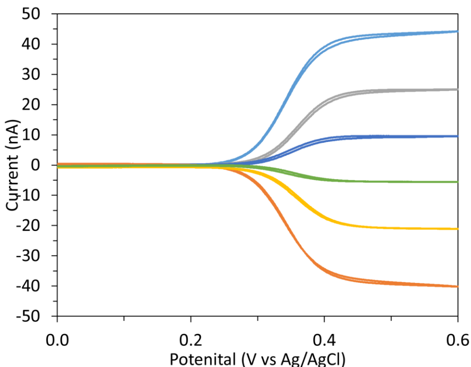
Figure 2.16 Typical CV of 1 mM FCA in 10 mM PBS from 0.0 to 0.6 V vs Ag/AgCl (sat. KCl) at 50 \text{ mV s}^{-1} at 1 \text{ }\mu\text{m} gold bands with various spacing where the Generator is swept between 0.0 to 0.6 V Ag/AgCl (sat. KCl) and the Collector was held at 0.1 V Ag/AgCl (sat. KCl). The scans were carried out at 1 \text{ }\mu\text{m} electrode bands with 1 \text{ }\mu\text{m} inter-electrode gaps generator (light blue) and collector (orange), 1 \text{ }\mu\text{m} electrode bands with 2 \text{ }\mu\text{m} inter-electrode gaps generator (grey) and collector (yellow), and 1 \text{ }\mu\text{m} electrode bands with 5 \text{ }\mu\text{m} inter-electrode gaps generator (dark blue) and collector (green).
