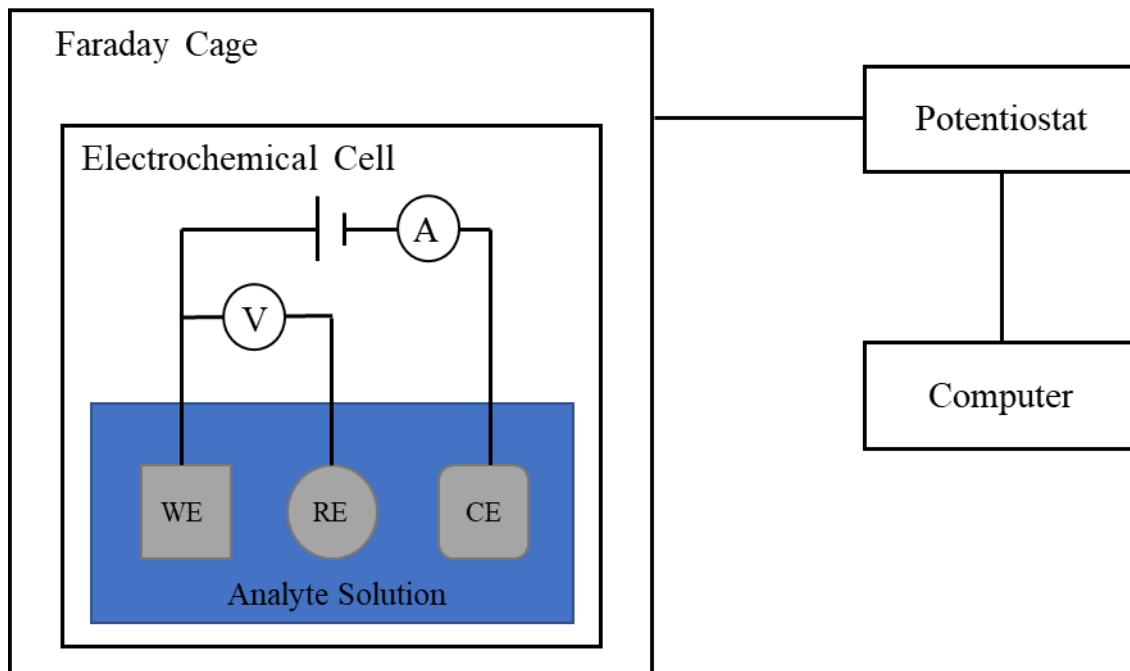
Figure 1.1 Schematic diagram of a standard three-electrode electrochemical cell within a Faraday cage, connected to a potentiostat and a computer. WE, RE and CE are the working, reference, and counter electrodes, respectively.
