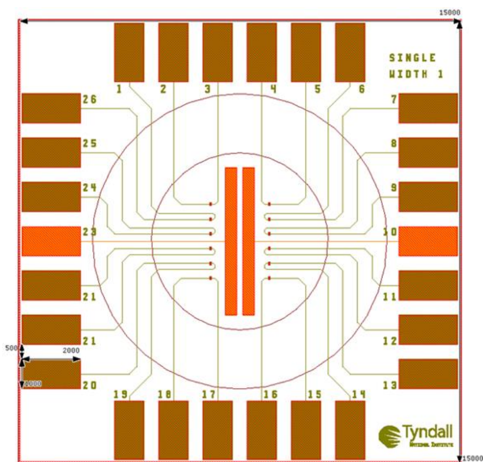
Figure 2.1 Mask design schematic for the chip fabrication process.
