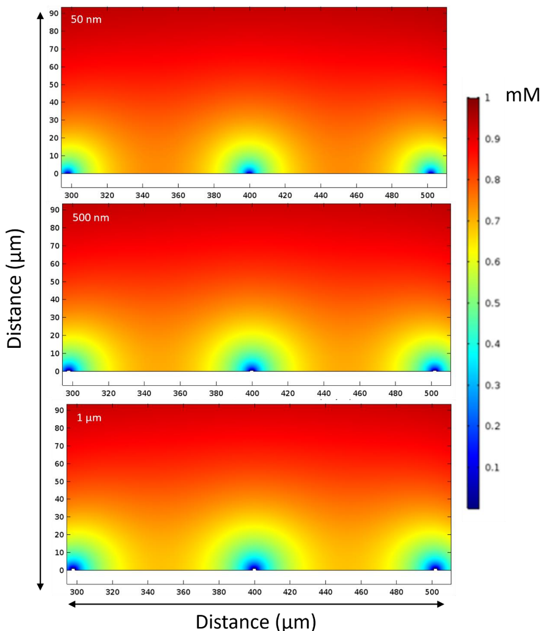
Figure 2.7 Cross-sectional view of 2D simulations of 1 mM FCA in 10 mM PBS diffusion profiles corresponding to CVs with 3 \times 2 \mu\text{m} bands with 100 \mu\text{m} inter-electrode spacing and varied electrode height, as indicated on the tiles. The images represent the condition at the end of a sweep to the potential 0.6 \text{ V} vs \text{Ag/AgCl} (sat. \text{KCl} ) at varied scan rates of 1 , 10 , and 100 \text{ mV s}^{-1} as indicated on each tile. The scale bar on the right hand side of the figure represents the concentrations of \text{Fe}^{2+} and \text{Fe}^{3+} , where 1 \text{ mM} (red) is \text{Fe}^{2+} in the bulk solution and as it is oxidised at the electrode surface it is converted to \text{Fe}^{3+} (blue).
