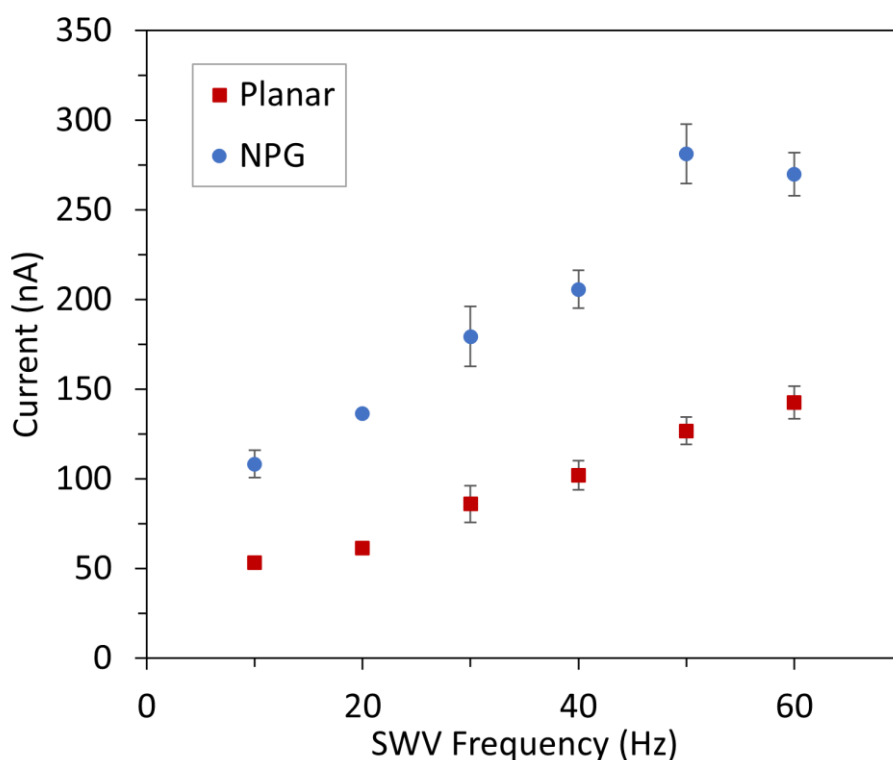
Figure 3.8 SWV peak current responses for 10 ppb Lead Nitrate in 0.1 M Acetate Buffer pH 4.6 deposited at -0.95 V vs Ag/AgCl (sat. KCl) for 600 s with varied frequency in the SWV stripping step at planar and NPG-modified 20 \mu\text{m} gold micro-disc arrays.
