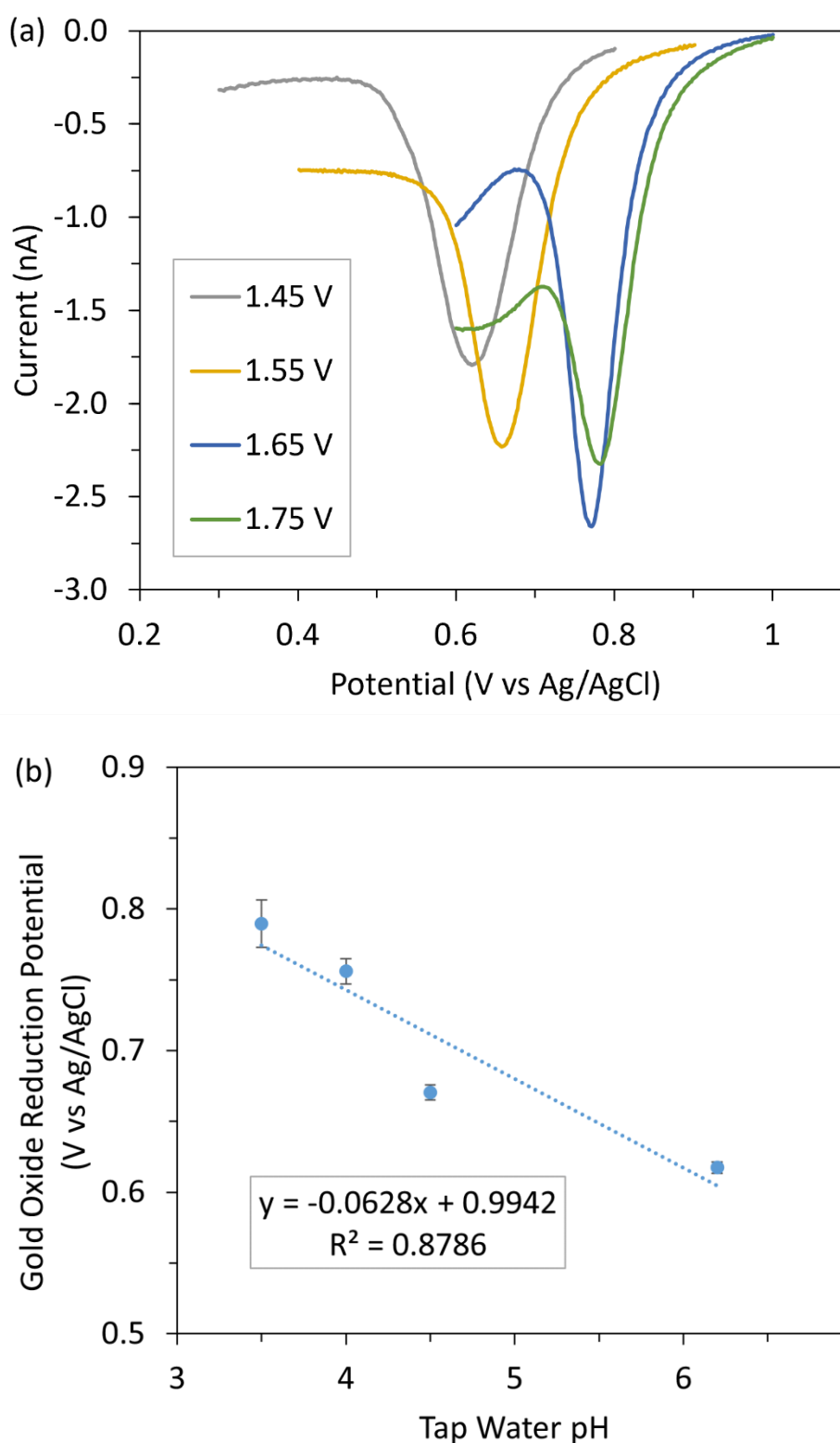
Figure 4.2 (a) The gold oxide reduction peak in CVs recorded from 0.0 V to 1.5 V at 50 mV s -1 at gold IDE arrays in artificial drinking water. At the opposing side of the array, the protonator, the potential was biased at various potentials to electrochemically impose a local pH change at the IDE arrays. (b) Calibration plot of gold oxide reduction peak potential vs. solution pH.
