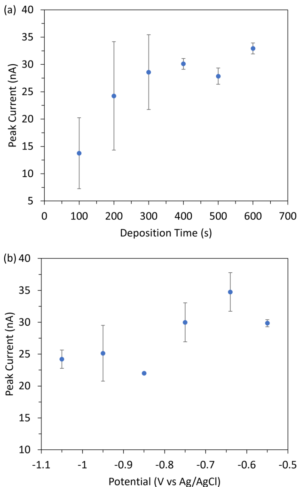
Figure 3.13 SWV peak current responses for 10 ppb Lead Nitrate in 0.1 M Acetate Buffer pH 4.6 for (a) deposition at -0.75 V vs Ag/AgCl (sat. KCl) with varied time and (b) deposition for 300 s with varied deposition potential at NPG-modified 3 \mu m gold IDEs with a 3 \mu m inter-electrode gap. Each measurement was carried out in triplicate with a new array used for each measurement.
