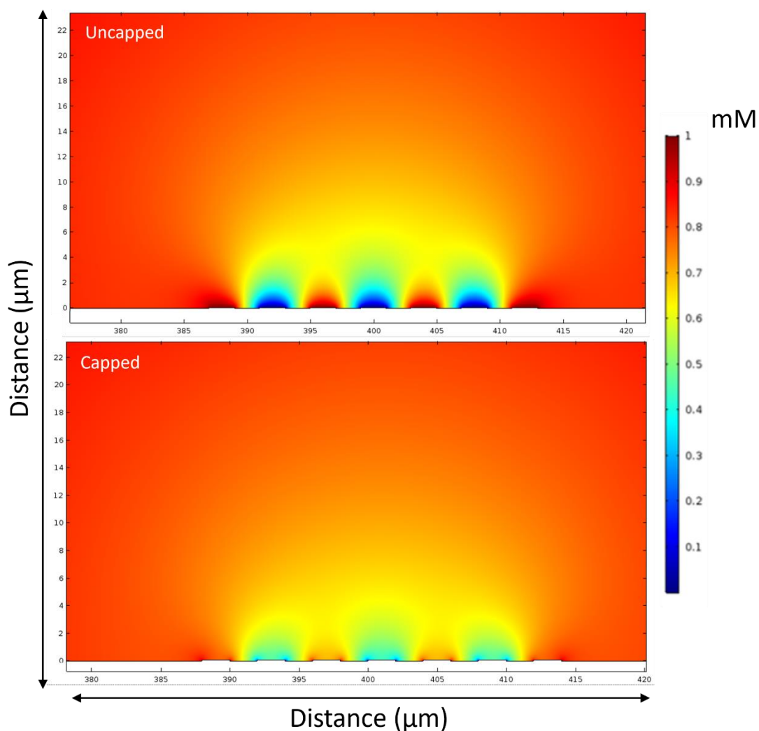
Figure 2.12 Cross-sectional view of 2D simulations 1 mM FCA in 10 mM PBS diffusion profiles corresponding to CVs when the potential at the generator electrode was swept from 0.0 V to 0.6 V vs Ag/AgCl (sat. KCl) at 50 \text{ mV s}^{-1} while the collector was held at 0.1 V vs Ag/AgCl (sat. KCl) for uncapped and capped electrodes, as indicated on the tiles. The images represent the condition at the end of a sweep to the potential 0.6 V vs Ag/AgCl (sat. KCl). The scale bar on the right-hand side of the figure represents the concentrations of \text{Fe}^{2+} and \text{Fe}^{3+} , where 1 mM (red) is \text{Fe}^{2+} in the bulk solution and as it is oxidised at the electrode surface it is converted to \text{Fe}^{3+} (blue).
