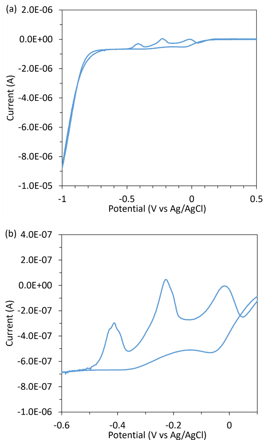
Figure 3.5 Typical CV of 10 ppm lead nitrate in 0.1 M acetate buffer pH 4.6 swept from 0.5 V to -1.0 V vs Ag/AgCl (sat. KCl) at 50 and at 100 mV s -1 at 20 \mu m gold micro-disc array, where (a) is the full CV range and (b) is highlighting the depositions and stripping peaks in the 0.1 to -0.6 V range.
