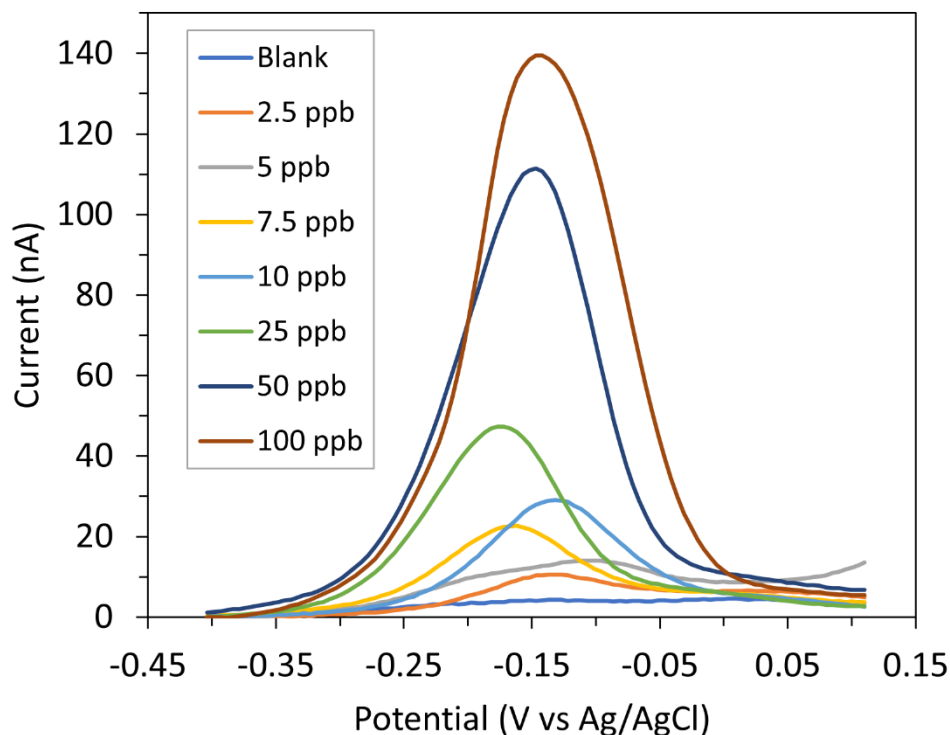
Figure 3.14 SWV for lead nitrate in 0.1 M acetate buffer pH 4.6 at NPG-modified 3 \mu m gold IDEs with a 3 \mu m inter-electrode gap. Each measurement was carried out in triplicate with a new array used for each measurement.
