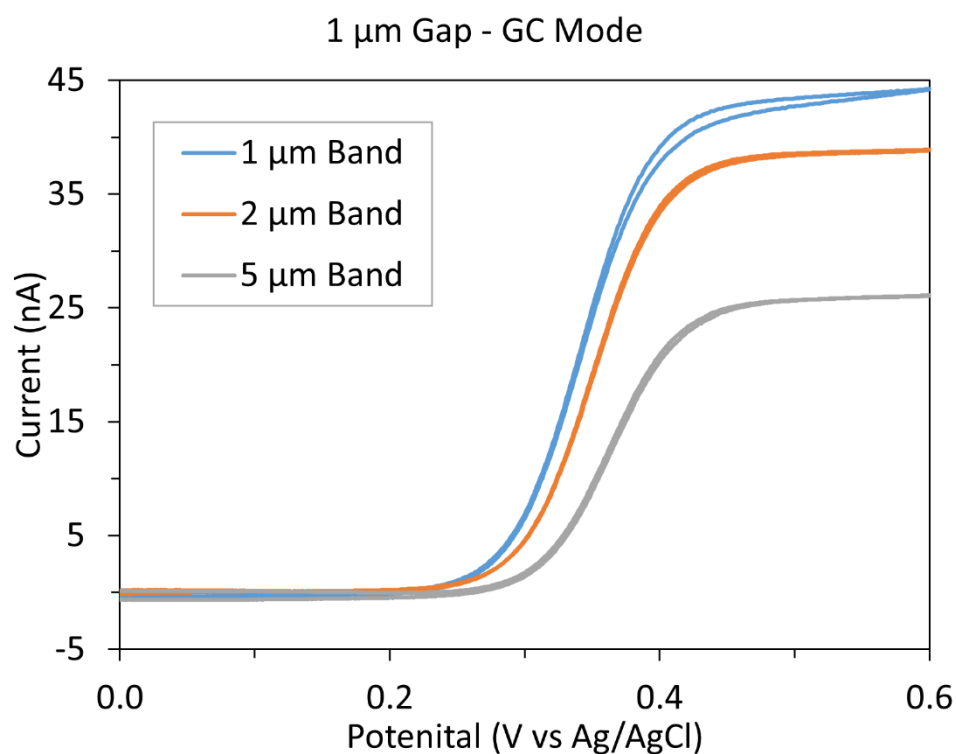
Figure 2.15 Typical cyclic voltammetric response of 1 mM FCA in 10 mM phosphate buffer from 0.0 to 0.60 V vs Ag/AgCl (sat. KCl) at 50 \text{mV s}^{-1} for IDE arrays with a 1 \mu\text{m} inter-electrode gap where the electrode band width was varied between 1 \mu\text{m} , 2 \mu\text{m} , and 5 \mu\text{m} as indicated by the legend.
