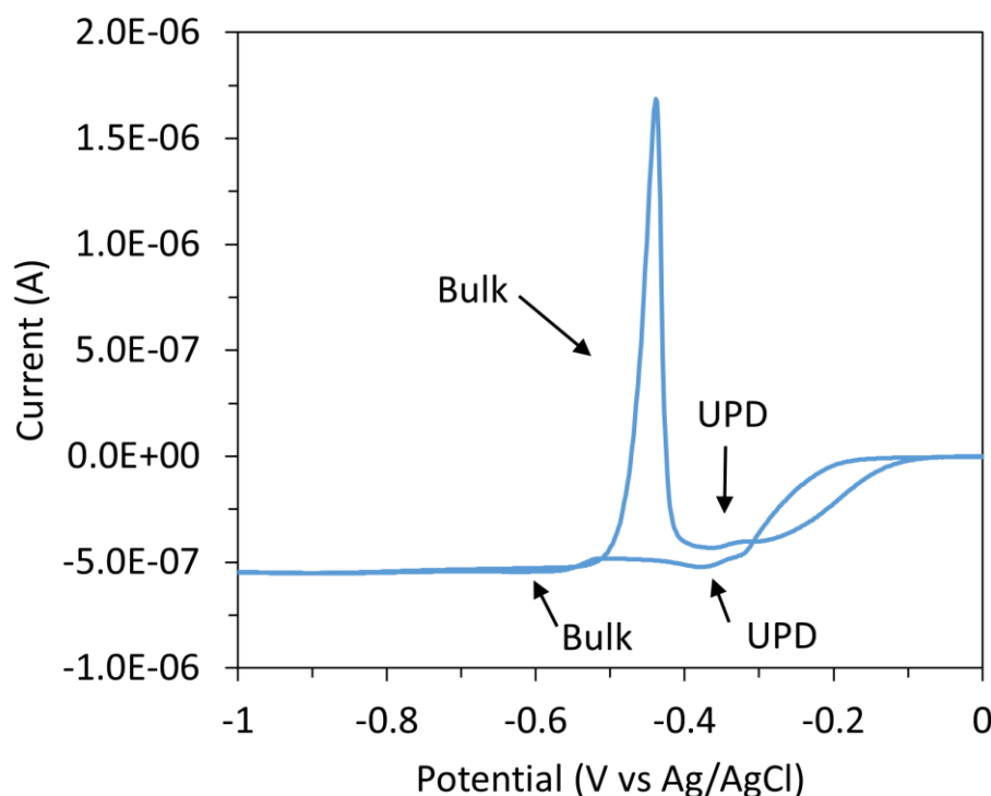
Figure 3.3 Typical CV of 10 ppm lead nitrate in 0.1 M acetate buffer pH 4.6 swept from 0.0 V to -1.0 V vs Ag/AgCl (sat. KCl) at 100 mV s -1 at 20 \mu m gold micro-disc array, highlighting the deposition and stripping peaks attributed to UPD and bulk.
