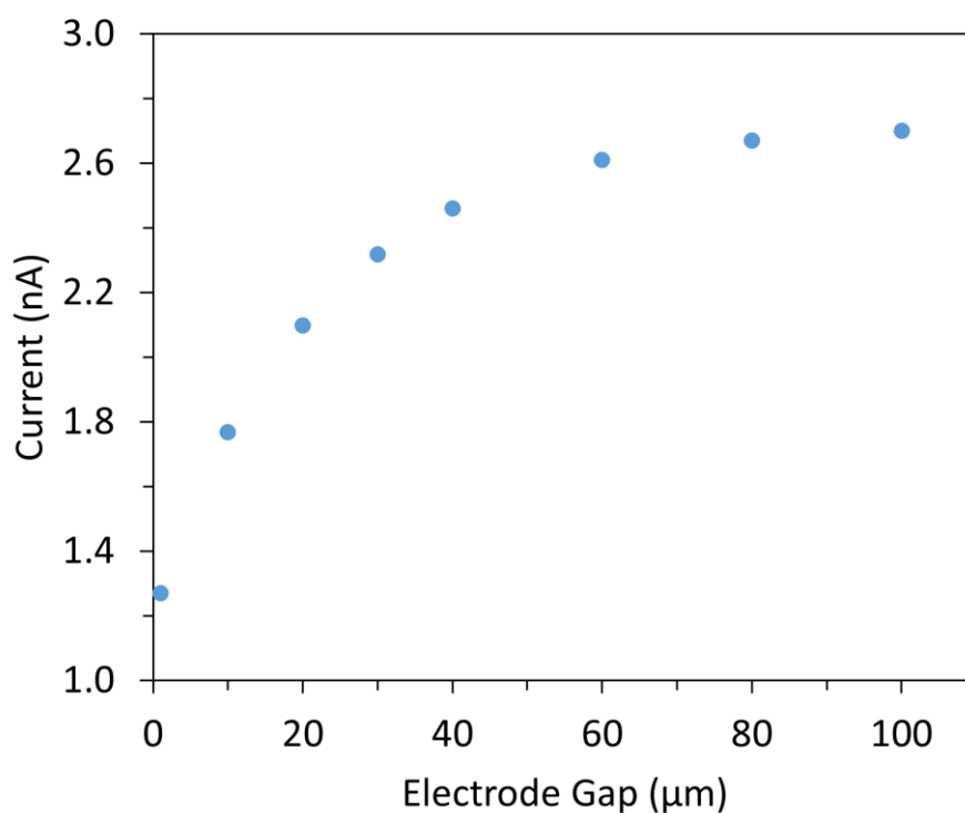
Figure 2.5 Plot of simulated current values for 2 \mu\text{m} band 3 electrode arrays with varied inter-electrode gap. Simulated current data point were taken from the limiting current of simulated CVs swept from 0 V to 0.6 V vs Ag/AgCl (sat. KCl) at 50 \text{mV s}^{-1} .
