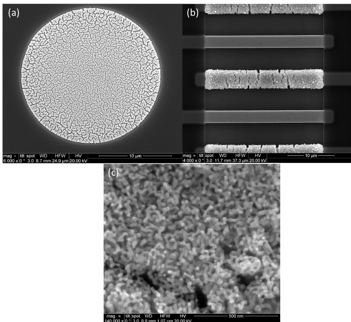
Figure 3.2 SEM Images of (a) NPG deposition in an individual 20 \mu\text{m} diameter micro-disc, (b) NPG deposited on several 3 \mu\text{m} wide micro-band electrodes in an IDE array (c) high magnification image of NPG deposit.
