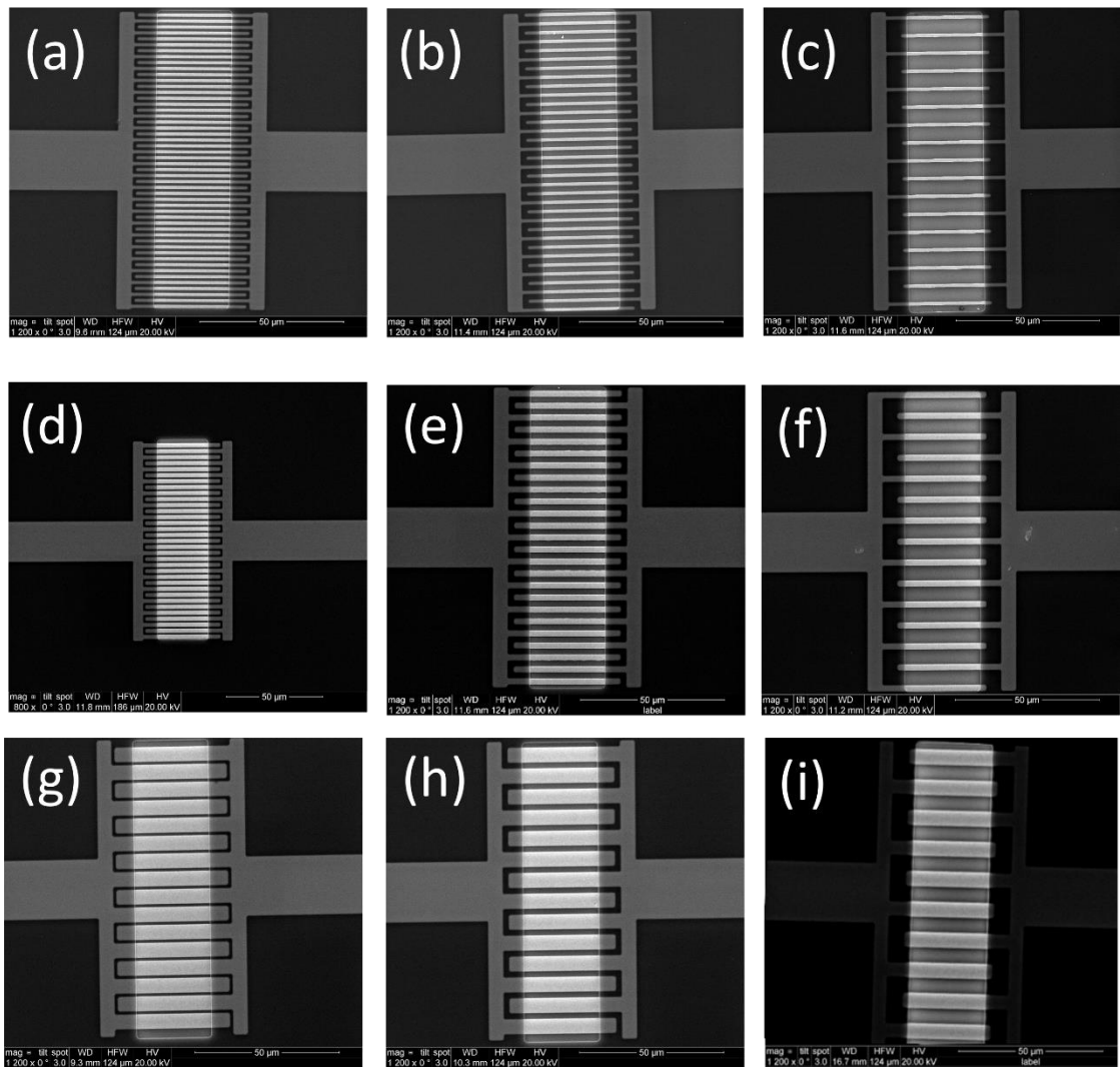
Figure 2.13 SEM of each array design; 1 \mu\text{m} bands with 1 \mu\text{m} (a), 2 \mu\text{m} (b) and 5 \mu\text{m} (c) spacing, 2 \mu\text{m} bands with 1 \mu\text{m} (d), 2 \mu\text{m} (e) and 5 \mu\text{m} (f) spacing, and 5 \mu\text{m} bands with 1 \mu\text{m} (g), 2 \mu\text{m} (h) and 5 \mu\text{m} (i) spacing.
