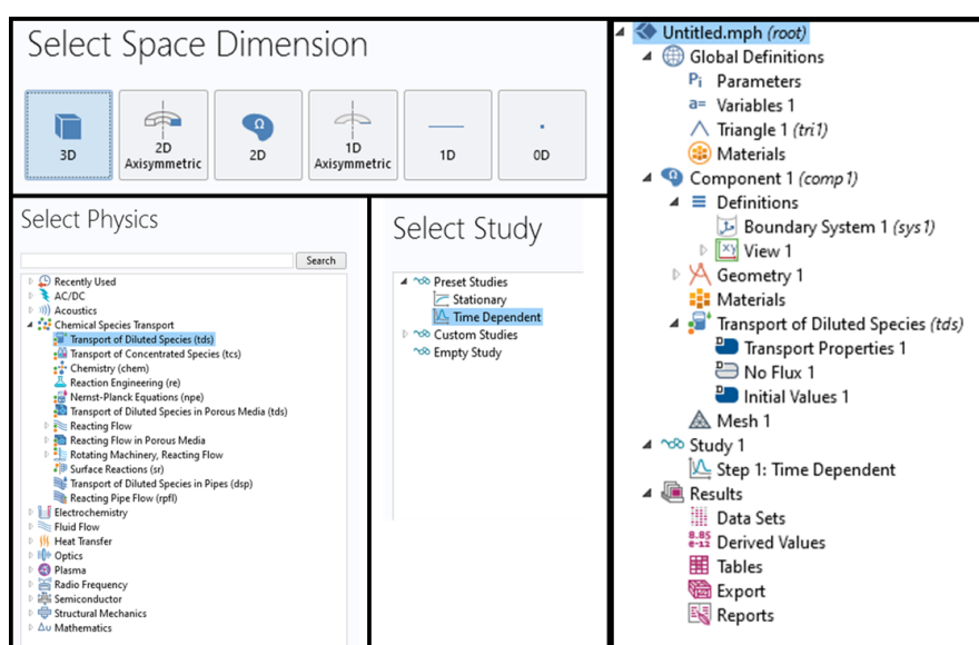
Figure 1.9 Screenshots of steps for building, solving and processing a model in COMSOL Multiphysics® 5.2.
