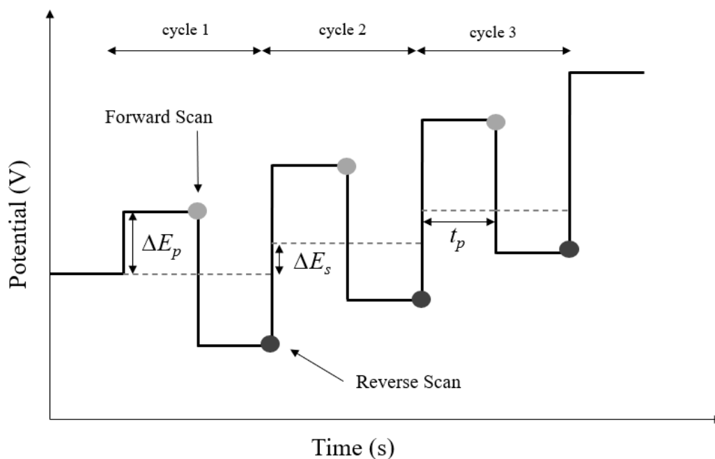
Figure 1.7 Schematic diagram of the potential in square wave voltammetry. Each cycle comprises a forward pulse and a reverse pulse, which are characterised by a pulse height ( \Delta E_p ), a pulse increment ( \Delta E_s ) and a pulse width ( t_p ).
