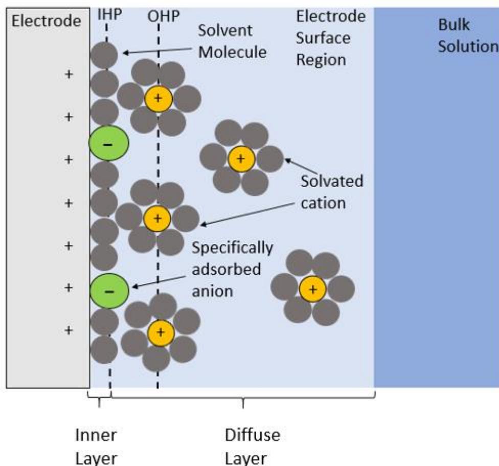
Figure 1.4 Simplified Model of the double layer region with specifically adsorbed anions and solvent molecules in the inner layer, and solvated cations in the diffuse layer. IHP and OHP are the inner and outer Helmholtz planes, respectively.
