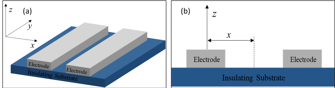
Figure 1.11 Schematic representation of (a) a 3D microelectrode domain and (b) a 2D cross section through the x,z plane, representing one unit cell for the diffusion domain approach
