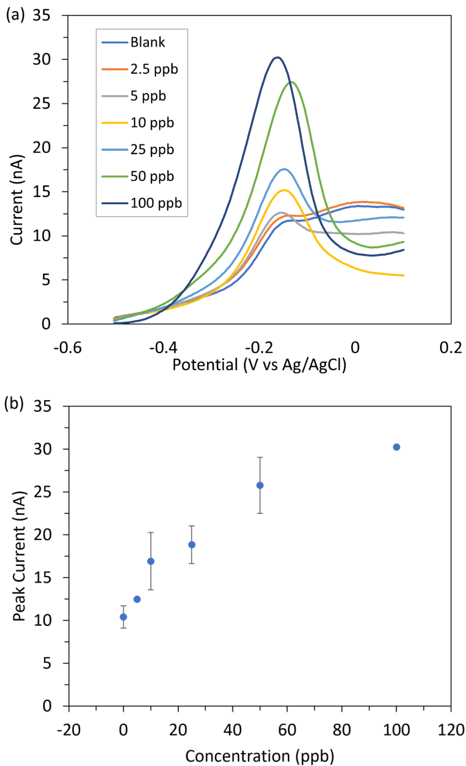
Figure 4.5 (a) Square wave stripping voltammogram for varied concentration of lead nitrate in tap water pH 4.6 at NPG-modified IDE arrays. (b) Calibration plot of lead stripping peak current vs. lead concentration.
