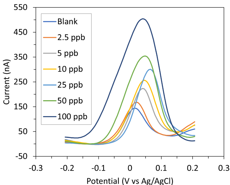
Figure 3.11 SWV of for varied concentrations of lead nitrate in 0.1 M acetate buffer pH 4.6 at NPG-modified 20 \mu\text{m} gold micro-disc arrays. Each measurement was carried out in triplicate with a new array used for each measurement.
