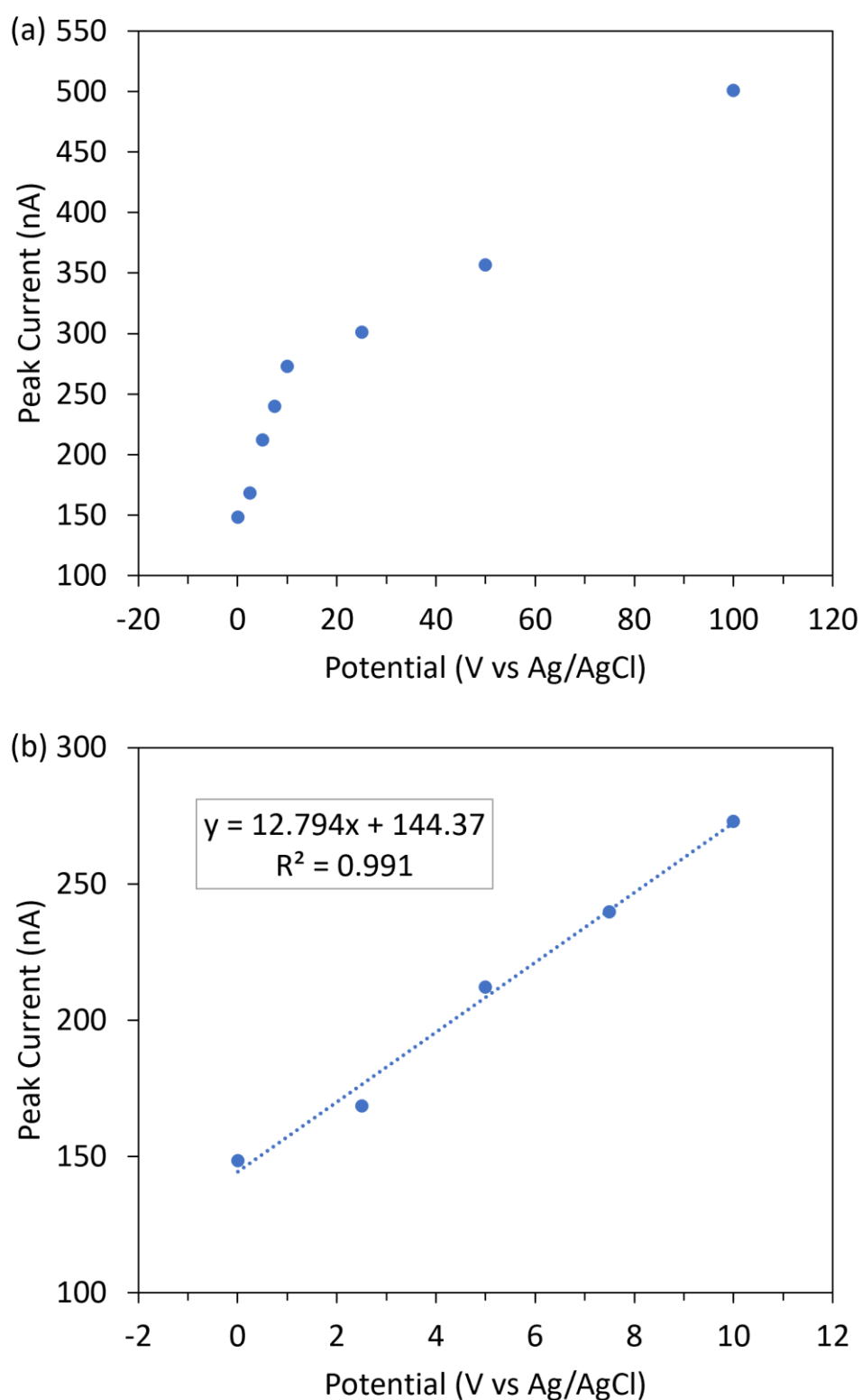
Figure 3.12 Calibration plots of lead peak stripping current at NPG modified 20 \mu\text{m} micro-disc arrays for (a) 0 to 100 ppb and (b) 0 to 10 ppb. Each measurement was carried out in triplicate with a new array used for each measurement.
