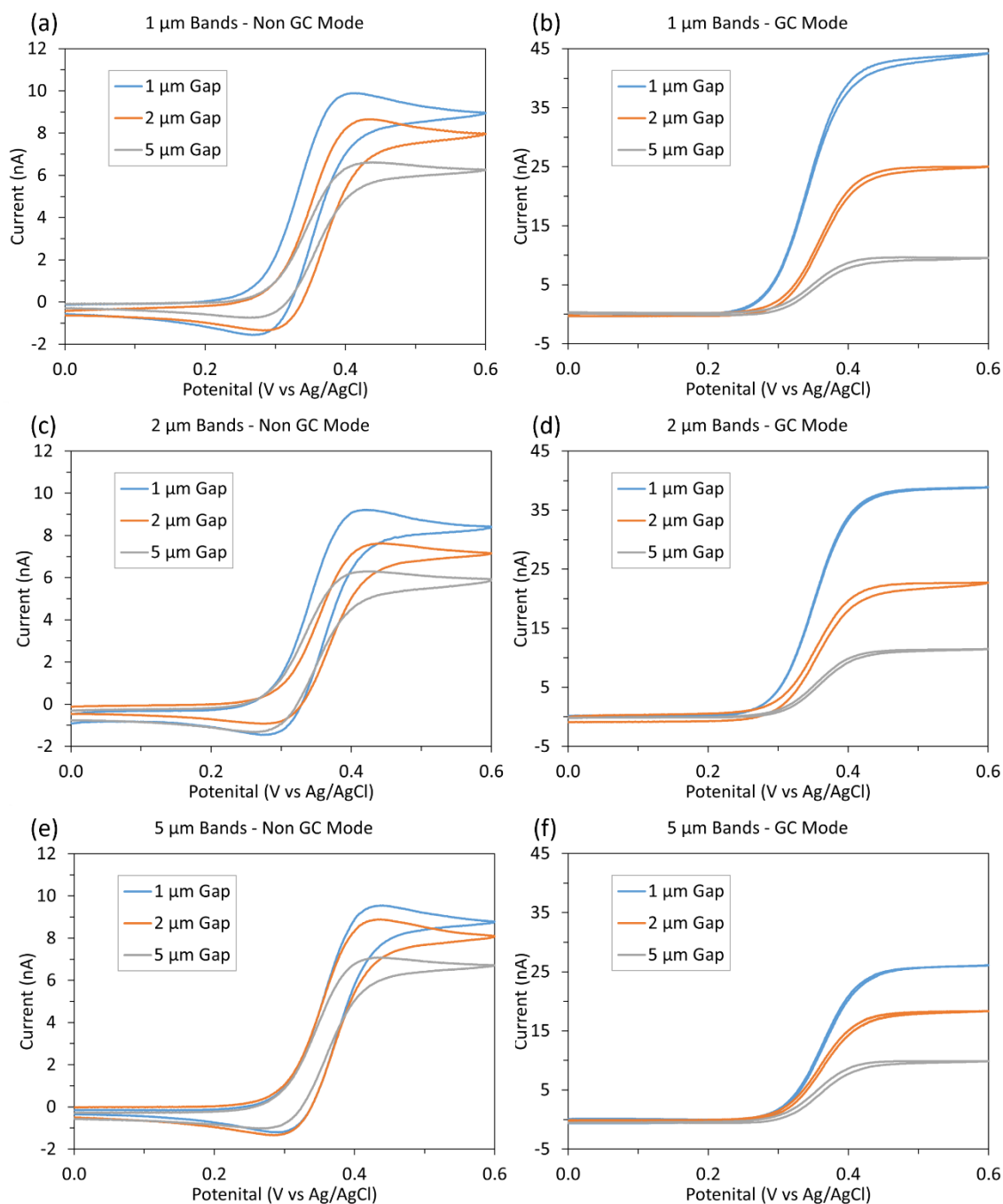
Figure 2.14 Typical cyclic voltammetric response of 1 mM FCA in 10 mM phosphate buffer from 0.0 to 0.60 V vs Ag/AgCl (sat. KCl) at 50 \text{ mV s}^{-1} for (a) 1 \text{ } \mu\text{m} bands with a 1 \text{ } \mu\text{m} , 2 \text{ } \mu\text{m} , and 5 \text{ } \mu\text{m} gap in Non GC mode, (b) 1 \text{ } \mu\text{m} bands with a 1 , 2 and 5 \text{ } \mu\text{m} gap in GC Mode, (c) 2 \text{ } \mu\text{m} bands with a 1 , 2 and 5 \text{ } \mu\text{m} gap in Non GC mode, (d) 2 \text{ } \mu\text{m} bands with a 1 , 2 and 5 \text{ } \mu\text{m} gap in GC Mode, (e) 5 \text{ } \mu\text{m} bands with a 1 , 2 , and 5 \text{ } \mu\text{m} gap in Non GC mode, (f) 5 \text{ } \mu\text{m} bands with a 1 , 2 and 5 \text{ } \mu\text{m} gap in GC Mode.
