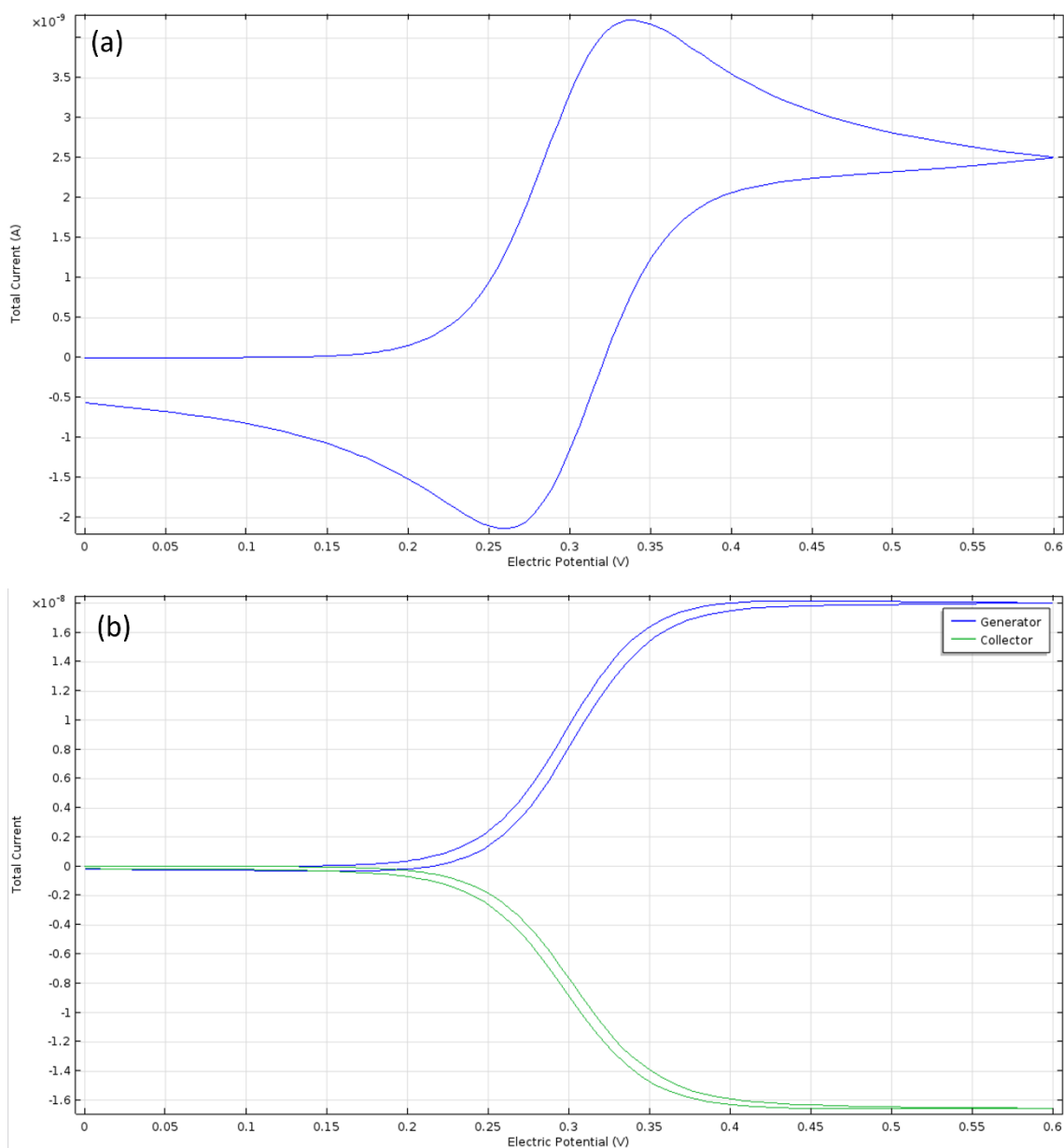
Figure 2.10 Simulated CV for 1 mM FCA from 0 to 0.6 V vs Ag/AgCl (sat. KCl) at 50 \text{ mV s}^{-1} for 2 \text{ }\mu\text{m} bands with 2 \text{ }\mu\text{m} inter-electrode gaps for (a) the Collector left unconnected as the Generator was swept from 0.0 to 0.6 V vs Ag/AgCl (sat. KCl), Non GC Mode, and (b) the Collector was held at 0.1 V vs Ag/AgCl (sat. KCl) while the Generator was swept from 0.0 to 0.6 V vs Ag/AgCl (sat. KCl), GC Mode.
