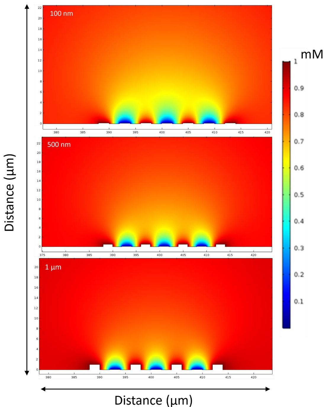
Figure 2.11 Cross-sectional view of 2D simulations of 1 mM FCA in 10 mM PBS diffusion profiles corresponding to CVs in GC mode with three 2 \mu\text{m} bands generator electrodes 50 nm in height and four 2 \mu\text{m} collector electrode with varied height as indicated on the individual tiles. The images represent the condition at the end of a sweep to the potential 0.6 V vs Ag/AgCl (sat. KCl) at 50 \text{mV s}^{-1} . The scale bar on the right hand side of the figure represents the concentrations of \text{Fe}^{2+} and \text{Fe}^{3+} , where 1 mM (red) is \text{Fe}^{2+} in the bulk solution and as it is oxidised at the electrode surface it is converted to \text{Fe}^{3+} (blue).
