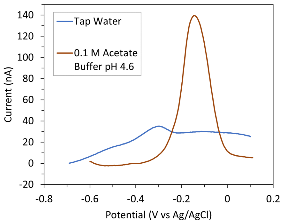
Figure 3.18 Square wave stripping voltammograms of for 100 ppb lead nitrate at NPG-modified interdigitated electrode arrays in 0.1 M acetate buffer pH 4.6 and tap water. Each measurement was carried out in triplicate with a new array used for each measurement.
