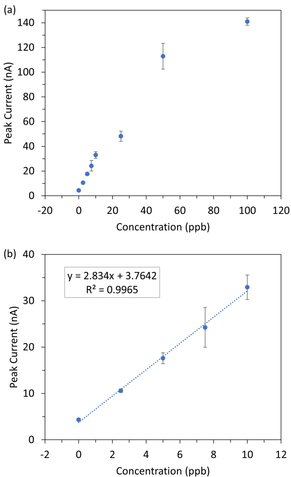
Figure 3.15 Calibration plots of lead peak stripping current at NPG-modified interdigitated electrodes arrays for (a) 0 to 100 ppb and (b) 0 to 10 ppb. Each measurement was carried out in triplicate with a new array used for each measurement.
