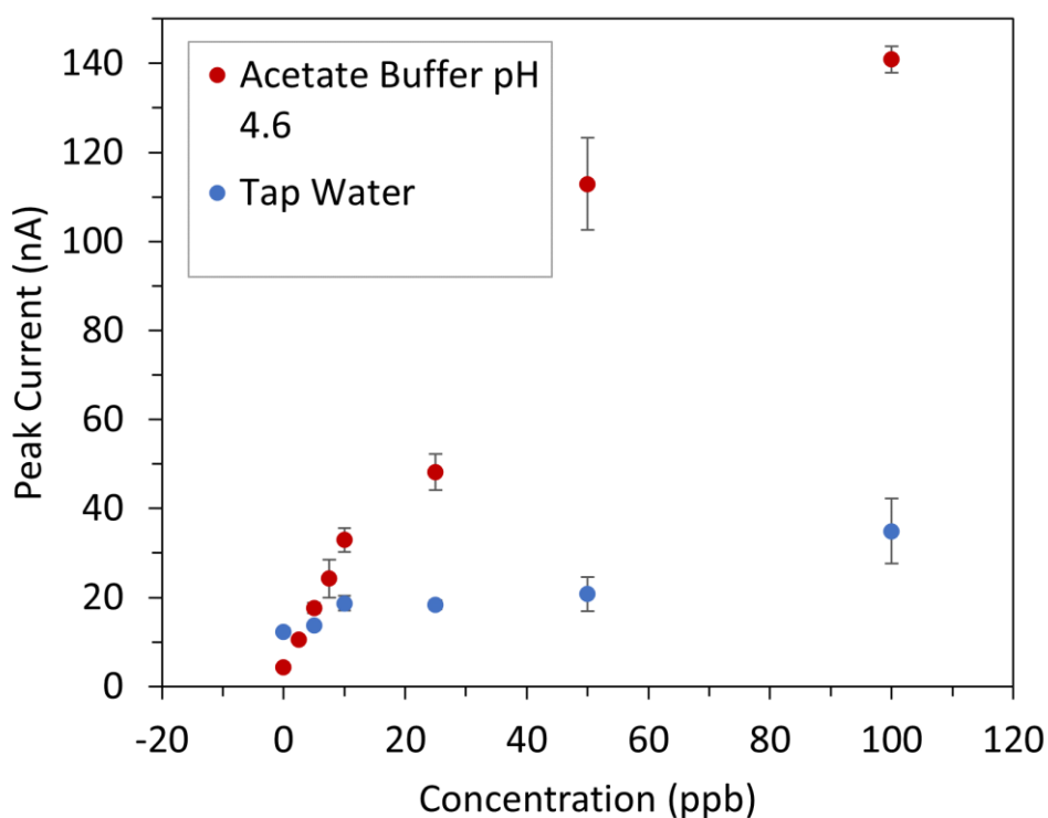
Figure 3.17 Calibration plot of the lead stripping peak current versus varied lead concentrations using NPG modified IDE arrays in acetate buffer pH 4.6 (red) and tap water (blue). Each measurement was carried out in triplicate with a new array used for each measurement.
