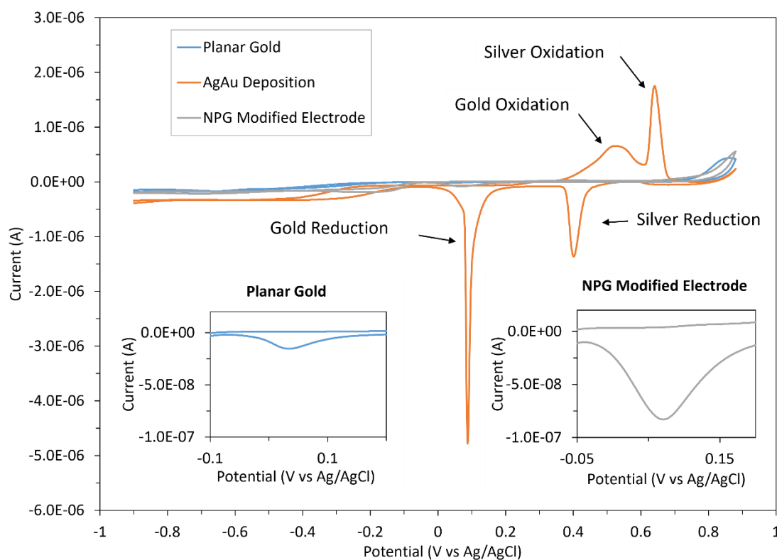
Figure 3.1 CVs in 1 M NaOH recorded from -0.90 to 0.88 V vs Ag/AgCl (sat. KCl) at 10 \text{ mVs}^{-1} recorded at a gold micro-disc array (blue), after \text{Au}_{0.18}\text{Ag}_{0.82} electrodeposition (orange) and at an NPG modified array (grey). Inserts show gold oxide reduction peaks at planar gold and NPG modified arrays (left and right, respectively)
