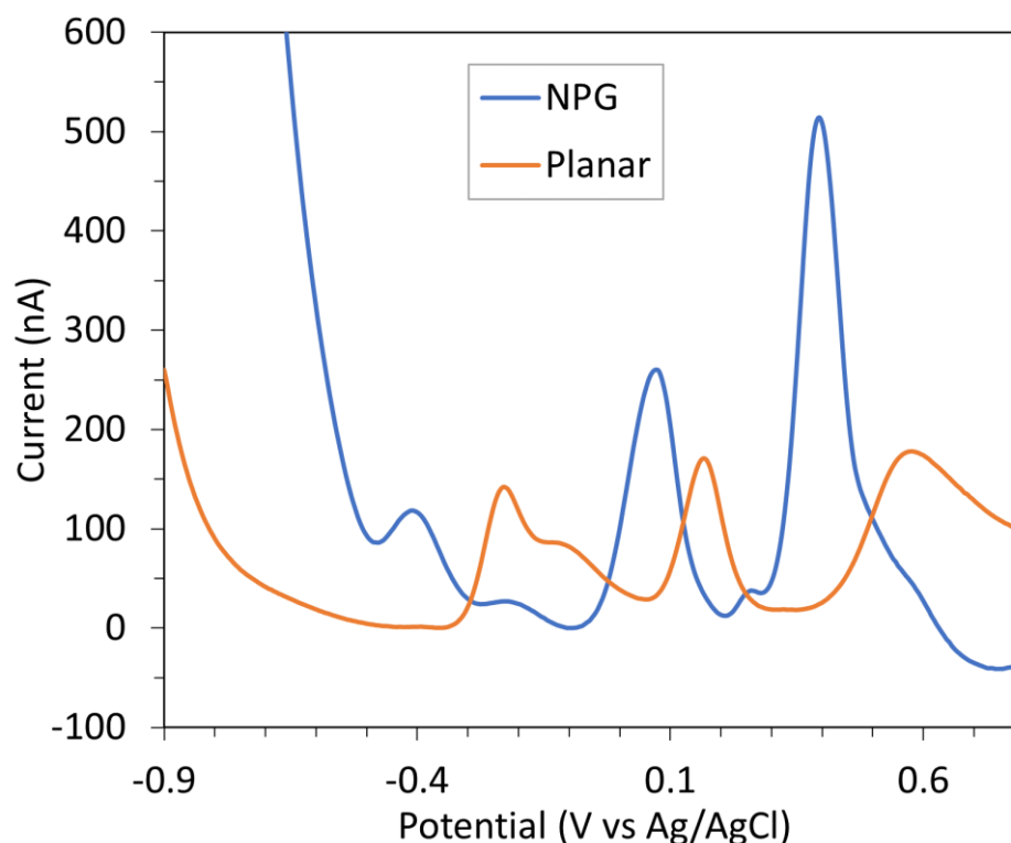
Figure 3.9 SWV current peaks for 10 ppb Lead Nitrate in 0.1 M Acetate Buffer pH 4.6 at unmodified 20 \mu\text{m} micro-disc arrays (red) and NPG modified 20 \mu\text{m} micro-disc arrays (blue)
