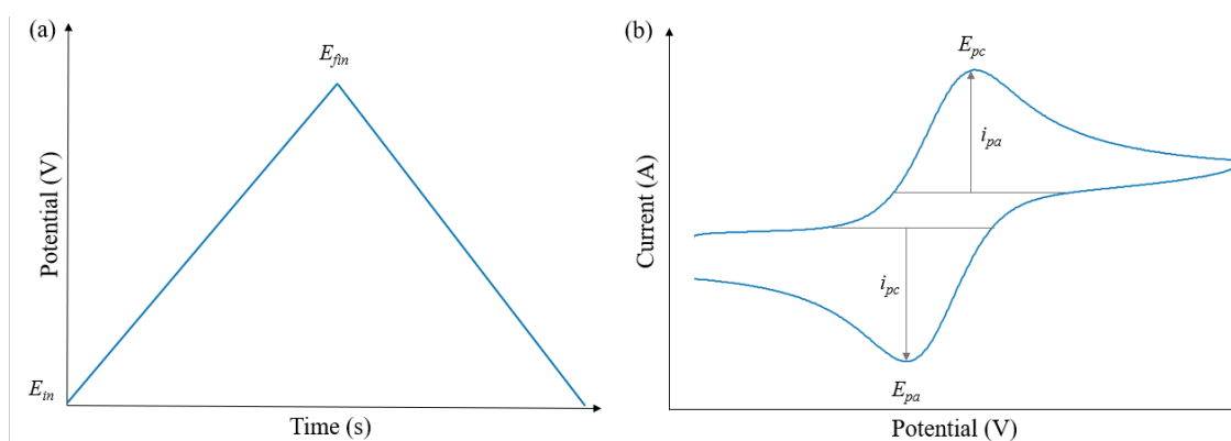
Figure 1.6 Schematic diagrams of (a) the potential wave form of cyclic voltammetry and (b) the resulting cyclic voltammogram.
