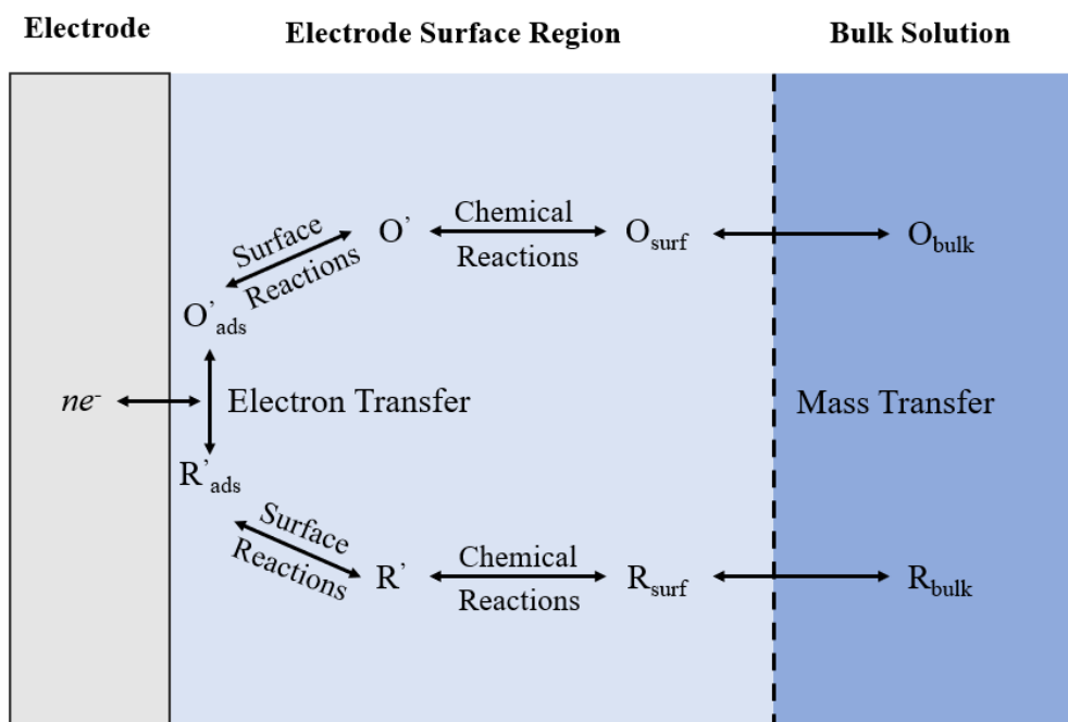
Figure 1.5 Schematic of the steps involved in a Faradaic reaction. O and R are a species in an oxidised and reduced state, respectively. O_{bulk} is oxidised in the bulk solution, O_{surf} is oxidised species at the electrode surface, O' is oxidised species that has been chemically changed and O'_{ads} is oxidised species that is absorbed on the surface. The same notation applies to R the reduced species.
