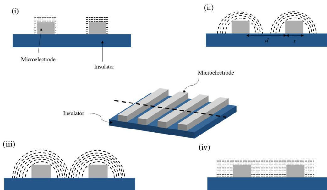
Figure 1.10 Schematic diagram of the four categories a diffusion profile may belong to for an array of microelectrodes. (i) \delta \ll r , planar diffusion to each electrode, (ii) \delta = r < d , radial diffusion to each electrode, (iii) r < \delta \leq d , transition zone and (iv) \delta \gg d , planar diffusion to the entire array.
