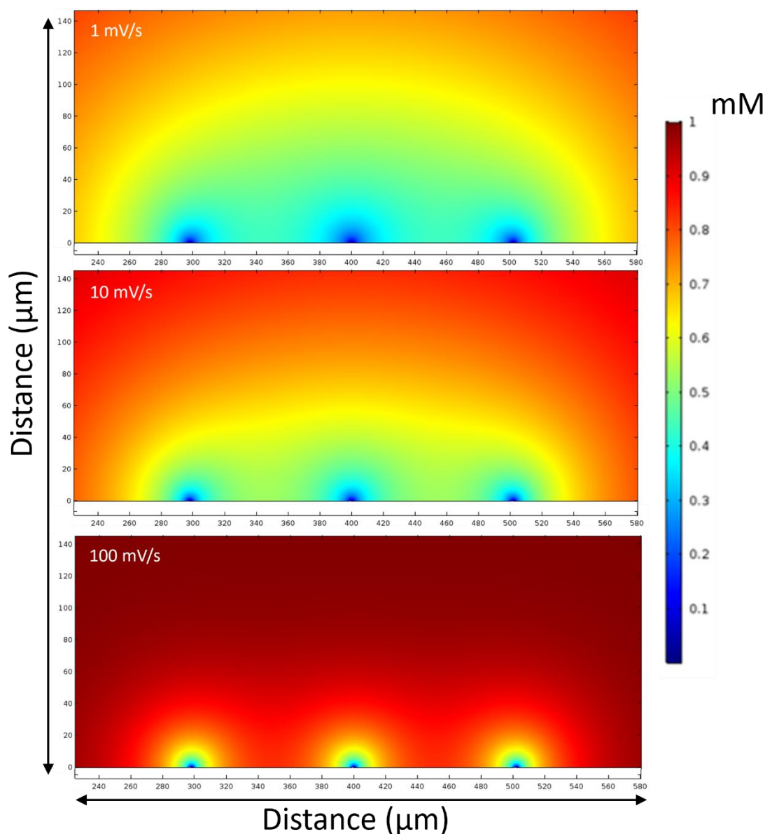
Figure 2.6 Cross-sectional view of 2D simulations of 1 mM FCA in 10 mM PBS diffusion profiles corresponding to CVs with 3 \times 2 \mu\text{m} bands with 100 \mu\text{m} inter-electrode spacing. The images represent the condition at the end of a sweep to the potential 0.6 V vs Ag/AgCl (sat. KCl) at varied scan rates of 1, 10, and 100 \text{ mV s}^{-1} as indicated on each tile. The scale bar on the right hand side of the figure represents the concentrations of \text{Fe}^{2+} and \text{Fe}^{3+} , where 1 mM (red) is \text{Fe}^{2+} in the bulk solution and as it is oxidised at the electrode surface it is converted to \text{Fe}^{3+} (blue).
