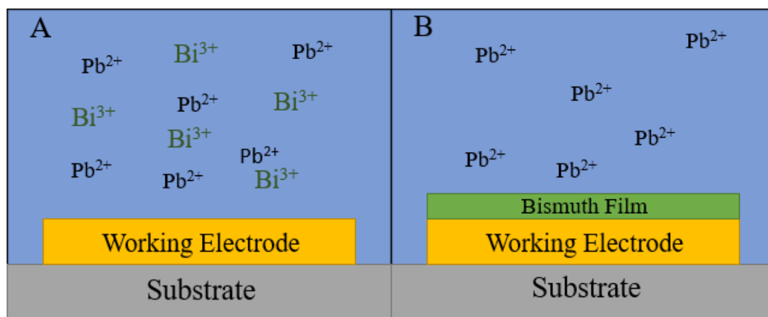
Figure 1.15 Principles of (A) In situ and (B) Ex situ bismuth electrodes for the detection of lead in water
