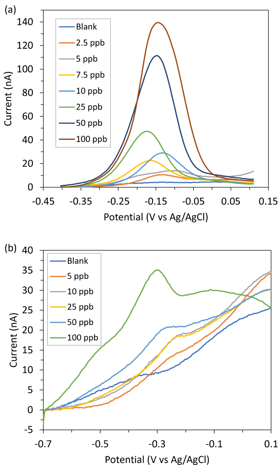
Figure 3.16 Square wave stripping voltammograms of for varied concentrations of lead nitrate at NPG modified gold interdigitated electrode arrays in (a) 0.1 M acetate buffer pH 4.6 and (b) tap water. Each measurement was carried out in triplicate with a new array used for each measurement.
