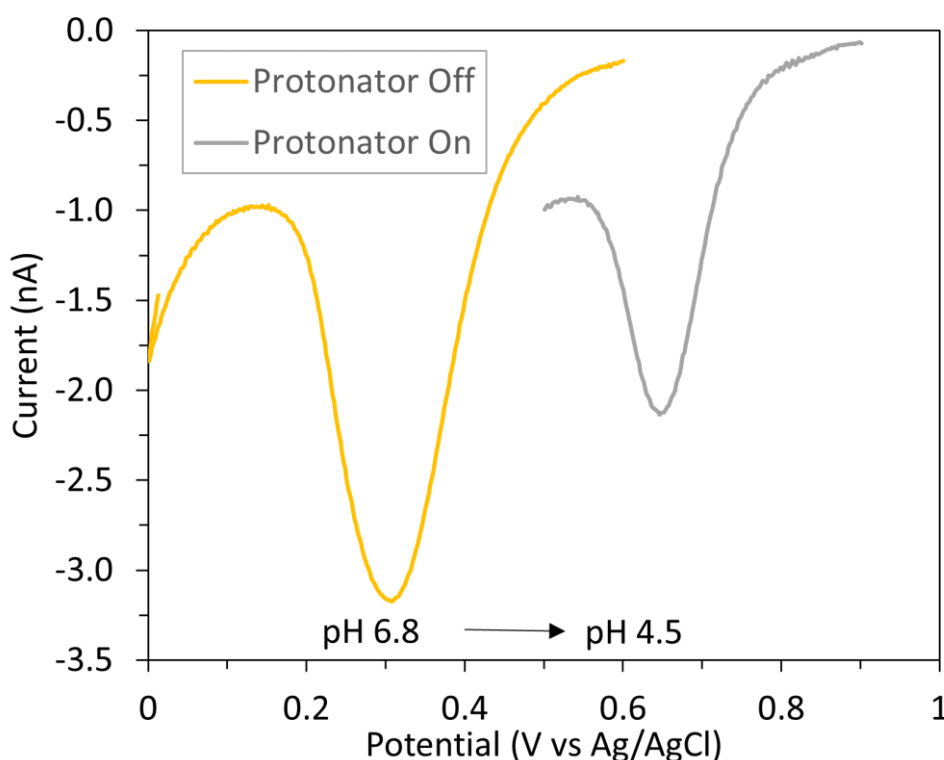
Figure 4.3 The gold oxide reduction peaks in tap water in CVs recorded from 0.0 V to 1.5 V vs Ag/AgCl (sat. KCl) at 50 \text{ mV s}^{-1} at gold IDE arrays while the protonator was initially left unbiased and then held at 1.55 V vs Ag/AgCl (sat. KCl).
