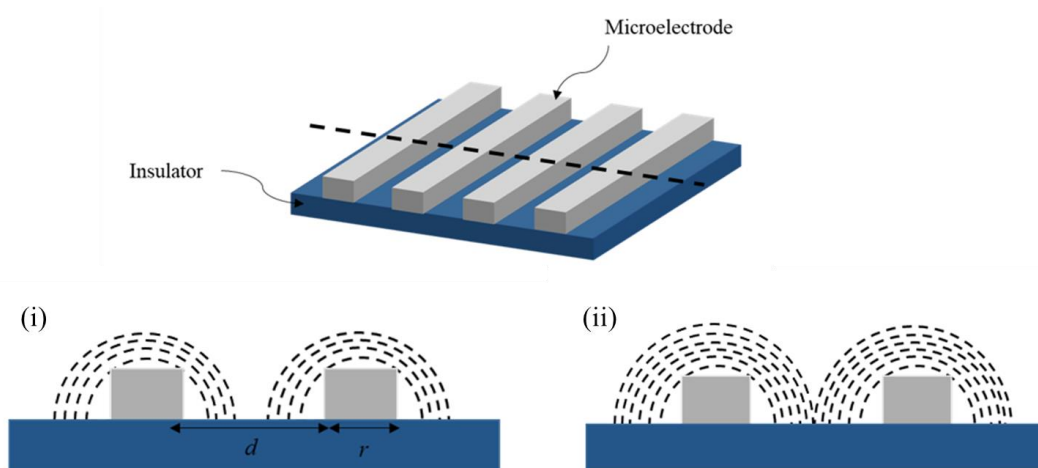
Figure 1.8 Schematic diagram of the diffusion layers where (i) the electrodes are diffusionally independent and (ii) the diffusion layers are diffusionally dependent.
