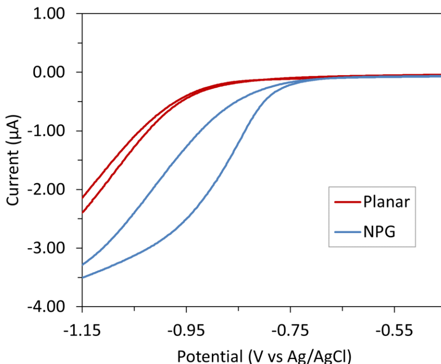
Figure 3.10 Typical CV at 10 \text{ mVs}^{-1} of planar and NPG modified 20 \mu\text{m} micro-disc array in 0.1 M acetate buffer pH 4.6 from -0.45 V to -1.15 V vs Ag/AgCl (sat. KCl) highlighting the onset of hydrogen evolution.
