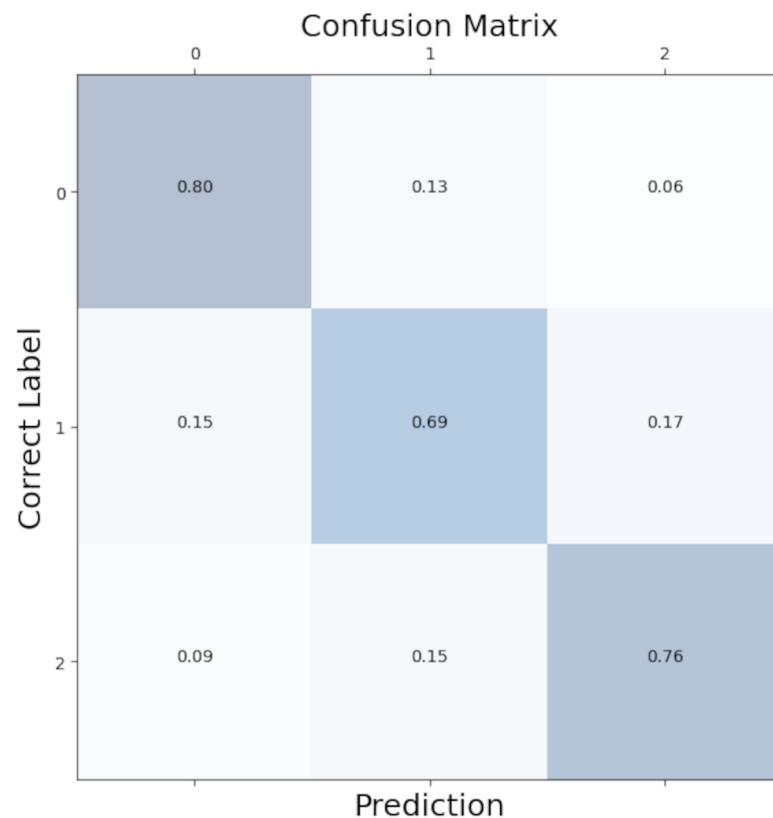
Figure 5. Confusion matrix for the Convolutional Neural Network. 0: no anxiety; 1: mild anxiety; 2: severe anxiety.
