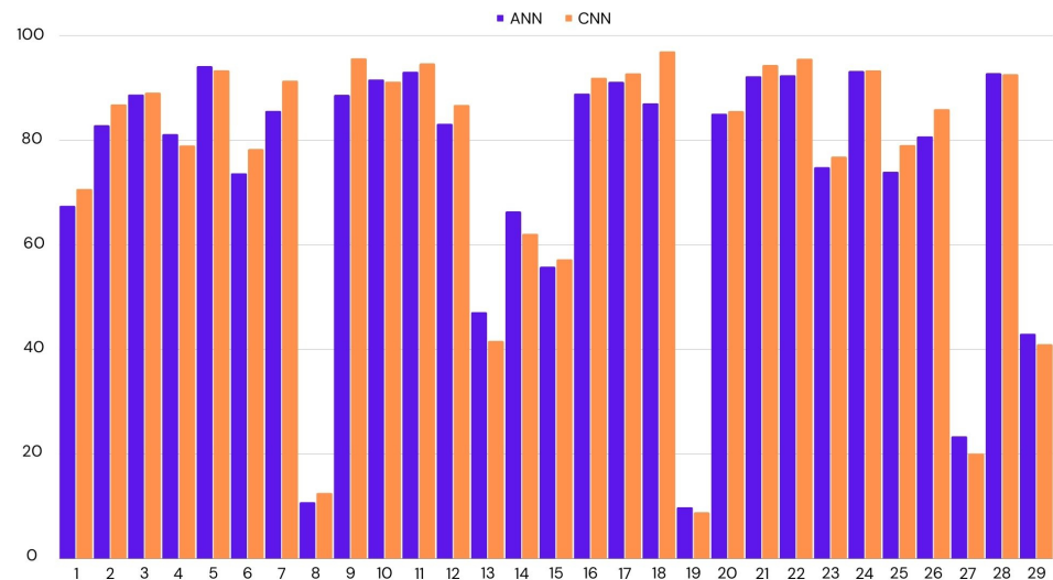
Figure 4. Classification accuracy for the each participant using leave-one-out cross-validation. ANN: Artificial Neural Network; CNN: Convolutional Neural Network.
