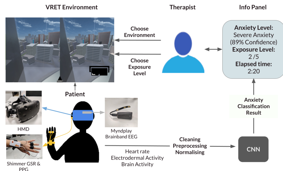
Figure 1. Framework diagram. CNN: Convolutional Neural Network; EEG: electroencephalogram; GSR: Galvanic Skin Response; HMD: head-mounted display; PPG: photoplethysmogram.
