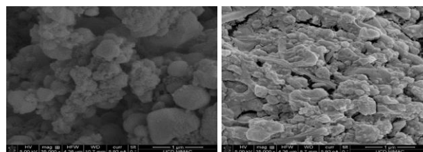
Figure 7. SEM for HKUST 1 powder (a) and pellet (b)
