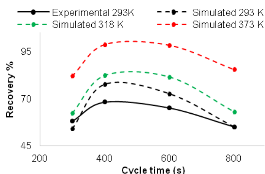
Figure 10. Experimental and simulated PSA recovery for zeolite 13X.
