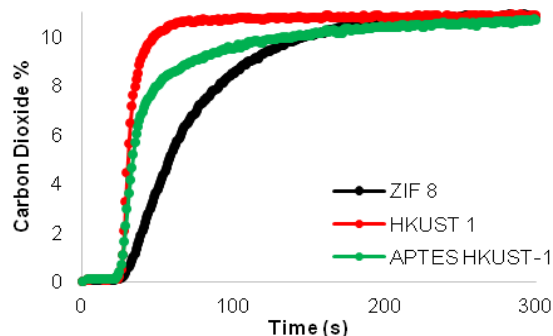
Figure 6. Adsorption capacity of MOFs
