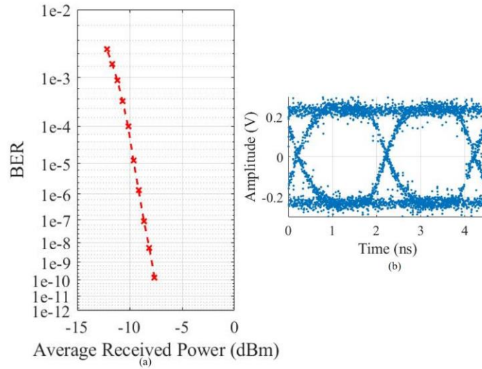
Figure 8 (a) BER performance of the DS link (500 Mb/s) using REAM as the optical receiver operating at 1520nm. Error free operation was observed at -7dBm. (b) Obtained eye diagram at -7dBm for REAM based optical receiver operating at 1520nm.
