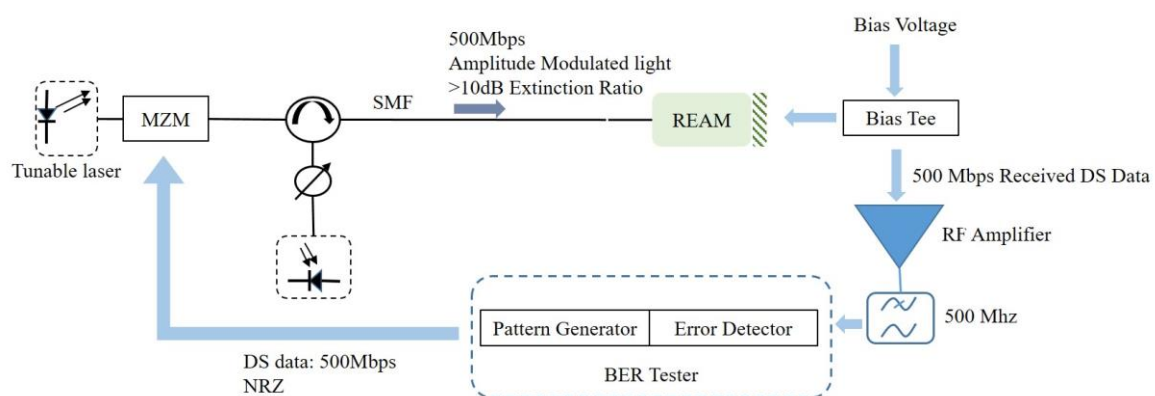
Figure 7 Experimental setup for emulating the DS link for 500Mb/s. The REAM is operating in the receive mode at 1520nm using zero-bias voltage. The photocurrent was amplified using a commercially available RF amplifier and the BER performance was measured using a BER tester. The REAM based optical receiver does not incorporate a transimpedance amplifier as in commercially available optical receivers.
