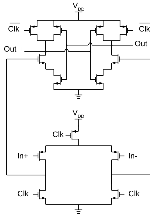
Figure 3.24: Schematic of double-tail dynamic latch comparator with preamplifier.
