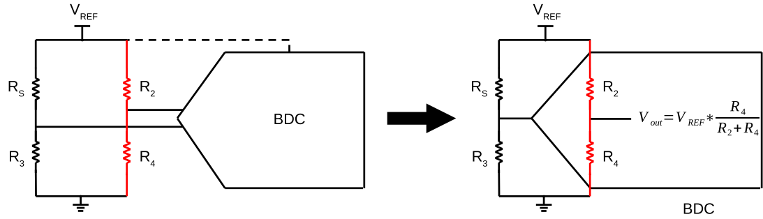
Figure 3.1: Block diagram of the modified Wheatstone Bridge.
