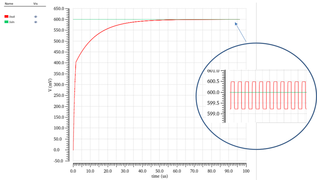
Figure 3.21: Simulated DAC output.
