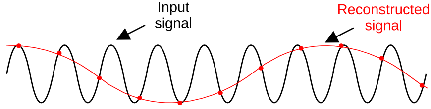
Figure 2.3: The aliasing effect, where the reconstructed signal (red) appears to be a sine wave of a lower frequency than the input signal (black).
