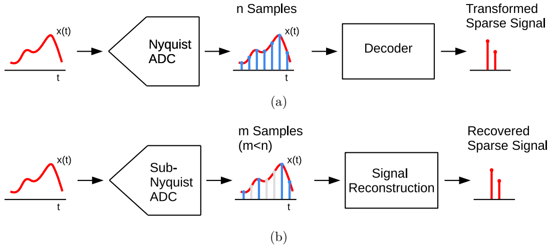
Figure 2.22: A high-level diagram of Nyquist sampling (a) and analog-to-information conversion (b) [43].
