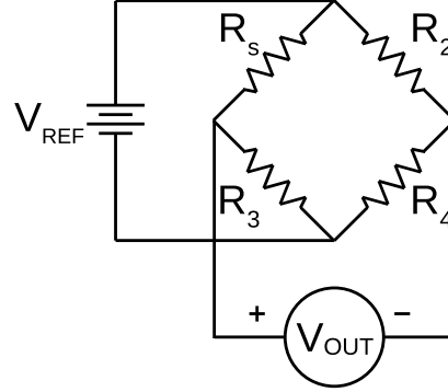
Figure 2.35: Typical Wheatstone Bridge configuration.
