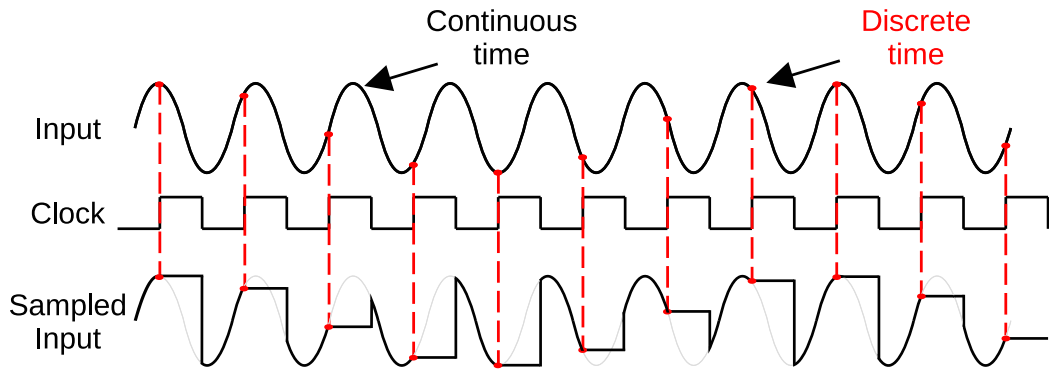
Figure 2.2: Sampling of an input signal. The voltage signal is first tracked during the sampling phase and then held at a constant amplitude for the duration of the conversion.
