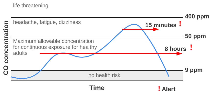
Figure 4.1: Example of carbon monoxide concentration levels and their impact on an individual's health.
