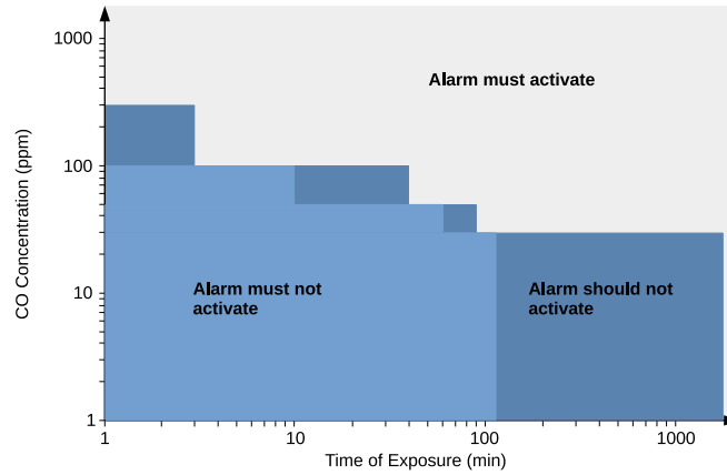
Figure 1.1: Example of carbon monoxide (CO) concentration levels [5].
