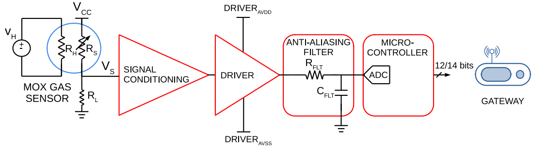
Figure 1.3: System diagram of a gas readout system.
