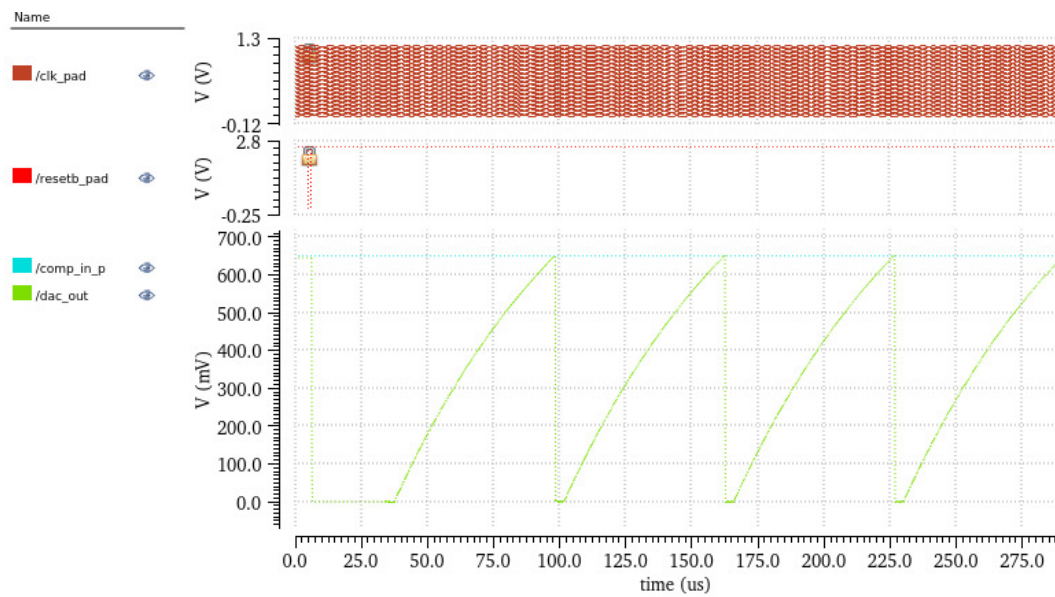
Figure 5.6: Simulation of post-layout extracted BDC with IO ring showing ramp-up mode.
