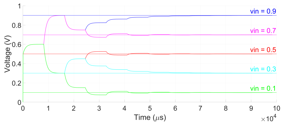
Figure 3.6: Matlab model of the BDC's successive approximation plotted across a range of inputs.
