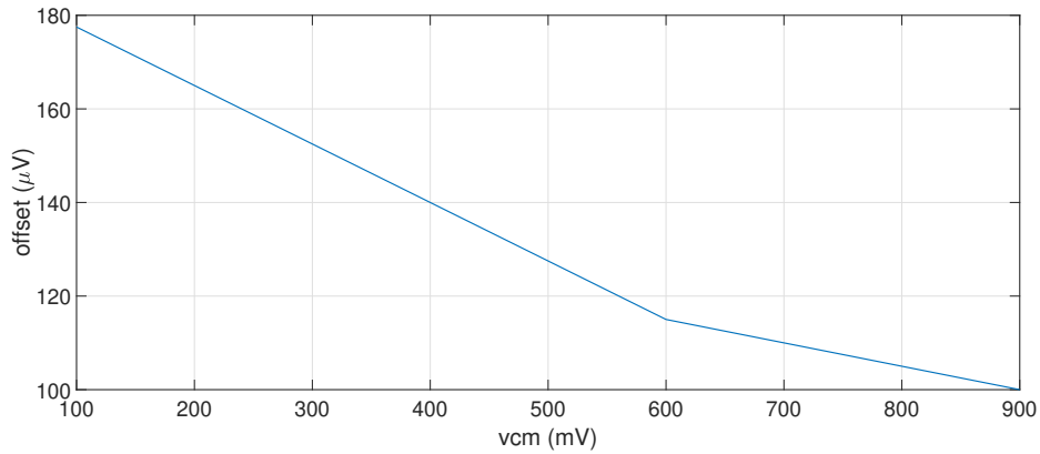
Figure 3.28: Extracted simulations showing a maximum offset of 178 \mu V across the input common mode.
