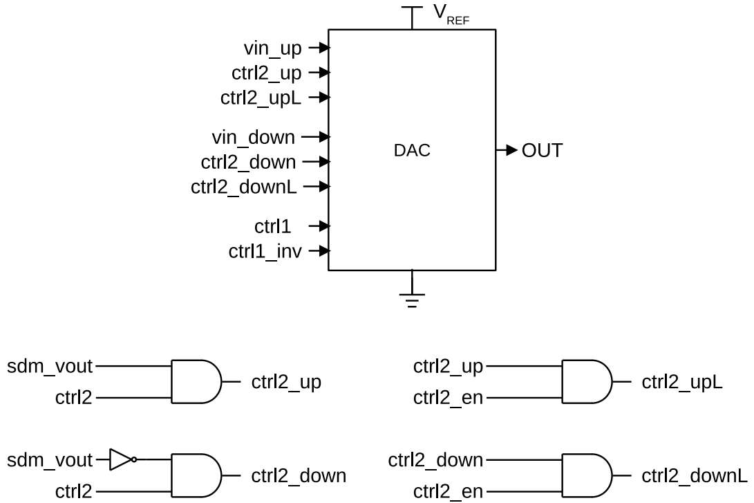
Figure 3.13: Top level schematic of Delta-Sigma DAC.
