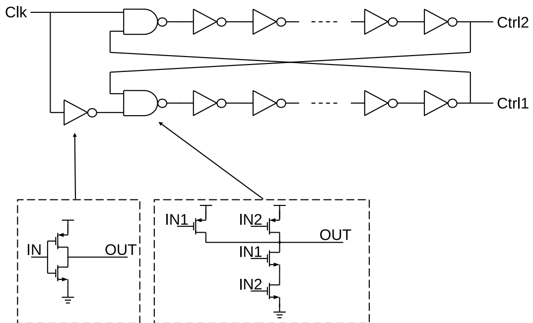
Figure 3.18: Schematic of the non-overlapping clock (NOC) generation circuit.
