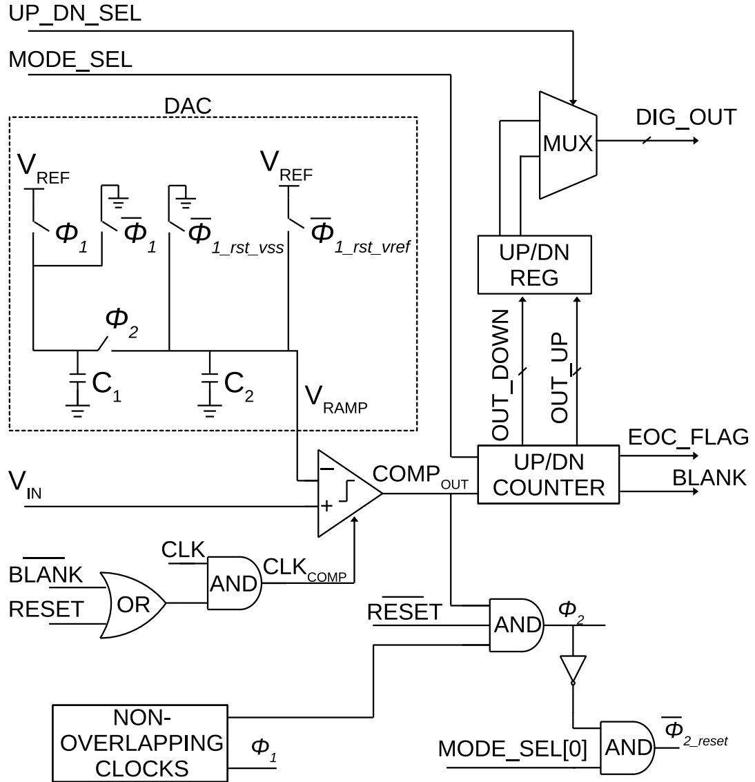
Figure 5.1: Block diagram of the digital ramp ADC.
