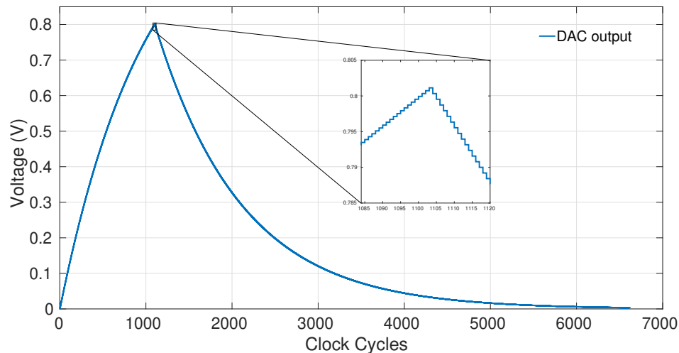
Figure 5.3: DAC sweep.
