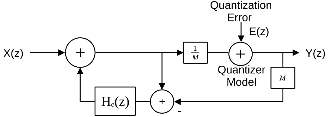
Figure 2.21: Linear model of a 1 st -order error feedback modulator.
