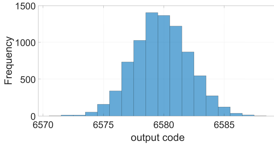
Figure 5.10: Histogram of the repeatability test results.
