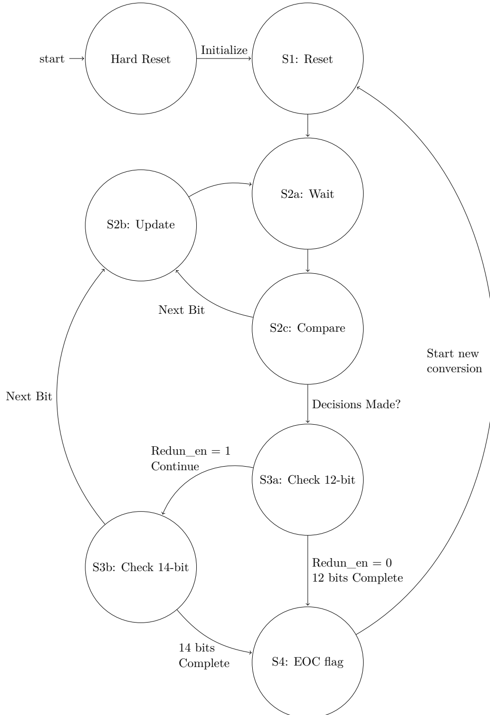
Figure 3.32: Representative diagram of the state machine of the operation of the BDC
