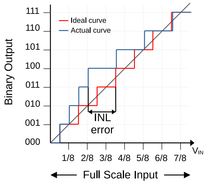
Figure 2.5: Representation of the integral non-linearity, showing the deviation from a straight line.
