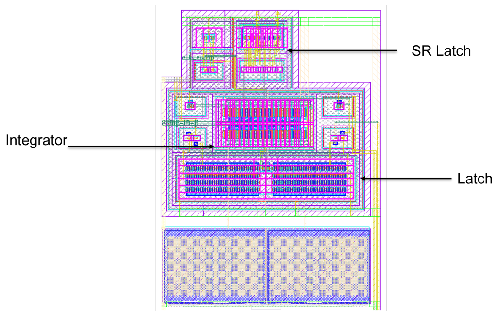
Figure 3.25: Comparator layout with main sub-blocks indicated.
