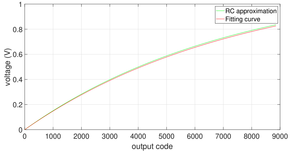
Figure 5.9: Output conversion, RC approximation and fitting curve.
