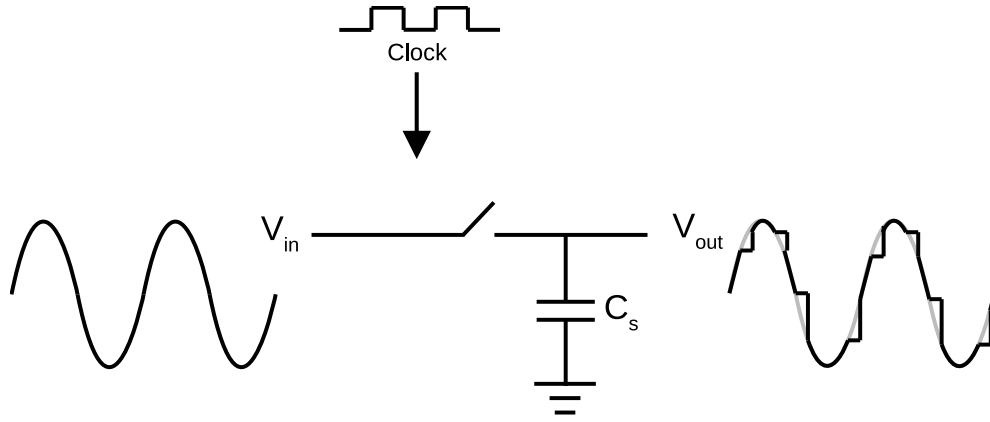
Figure 2.9: Simplified diagram of a sampling circuit.
