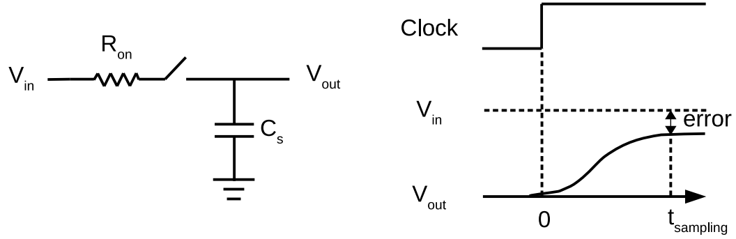
Figure 2.11: Sampling error due to RC charging time.
