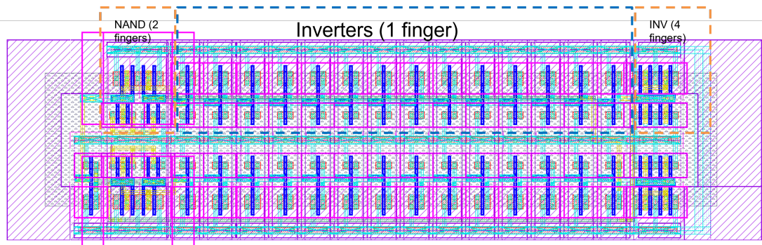
Figure 3.19: Layout of the non-overlapping clock (NOC) circuit.
