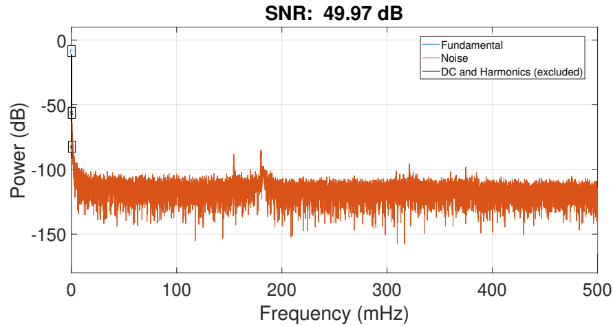
Figure 5.12: Measured output spectrum at full-scale input.
