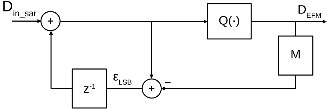
Figure 3.16: Block diagram of implemented 1 st -order EFM.
