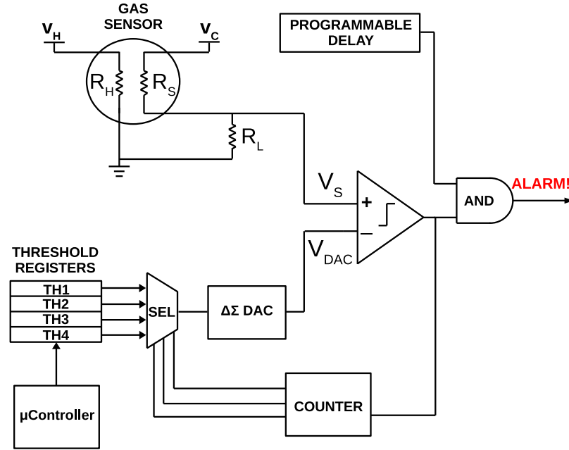
Figure 4.2: Block diagram representing the proposed threshold detection based ADC concept, whereby the input generated by the resistor divider is compared against the 4 different levels.
