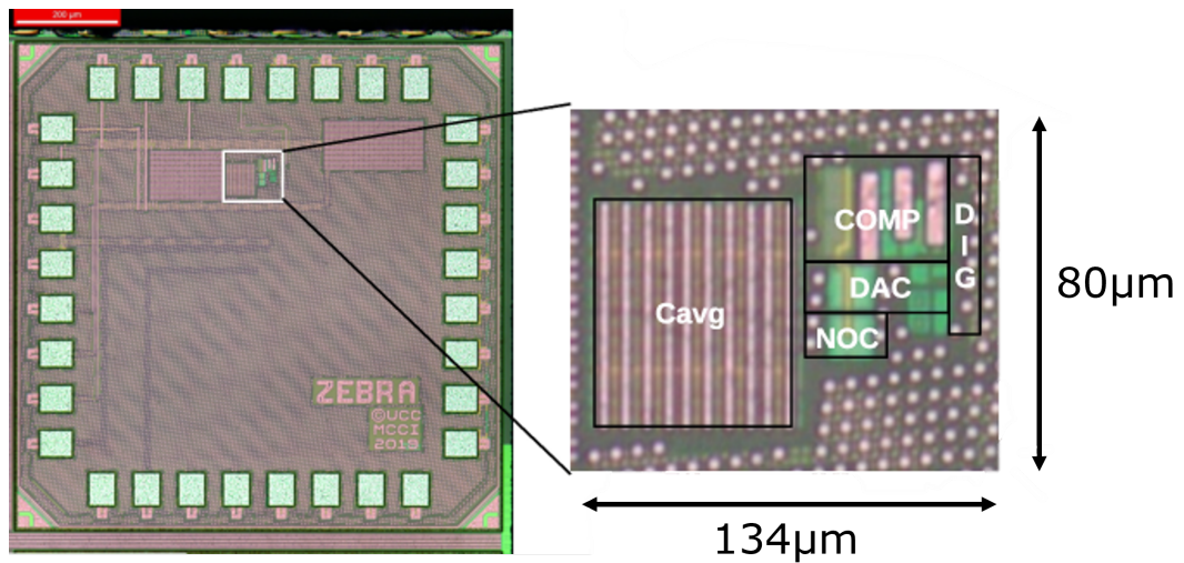
Figure 3.36: Die photograph with a zoomed view of a core BDC occupying 0.01\text{mm}^2 .
