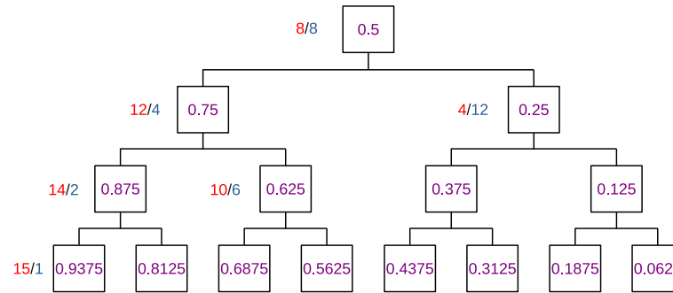
Figure 3.5: SAR approximation represented by resistance ratios.
