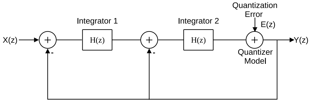
Figure 2.20: Linear model of a 2 nd -order \Delta\Sigma modulator.
