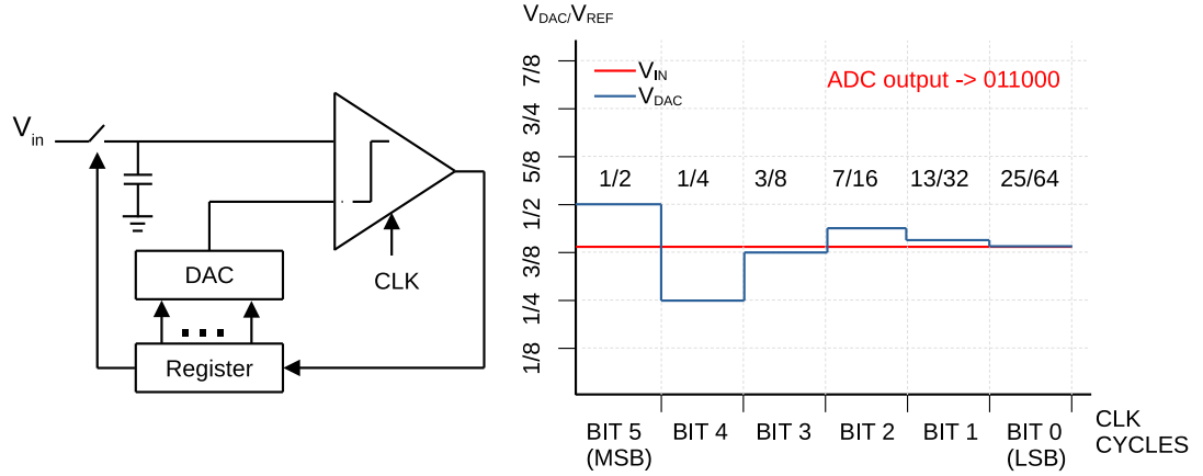
Figure 2.15: Simplified block diagram of a single-ended SAR ADC and sample approximation of 6-bit ADC.
