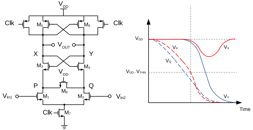
Figure 2.33: Transistor level diagram of a StrongArm latch comparator, with its associated voltage levels during amplification and regeneration stages.
