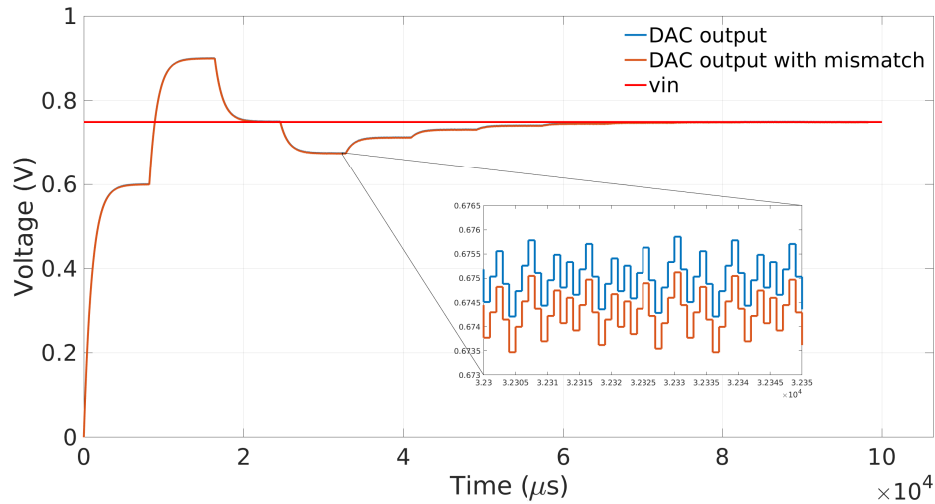
Figure 3.10: DAC output error for a 0.05 fF mismatch
