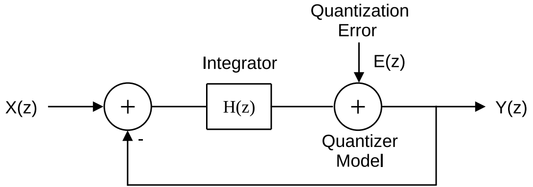
Figure 2.19: Linear model of a 1 st -order \Delta\Sigma modulator.
