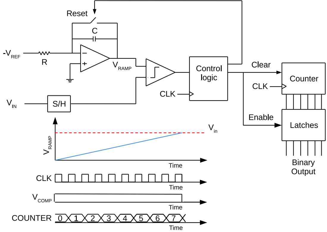
Figure 2.24: Simplified diagram of a conventional single-slope-based ADC with a timing diagram.
