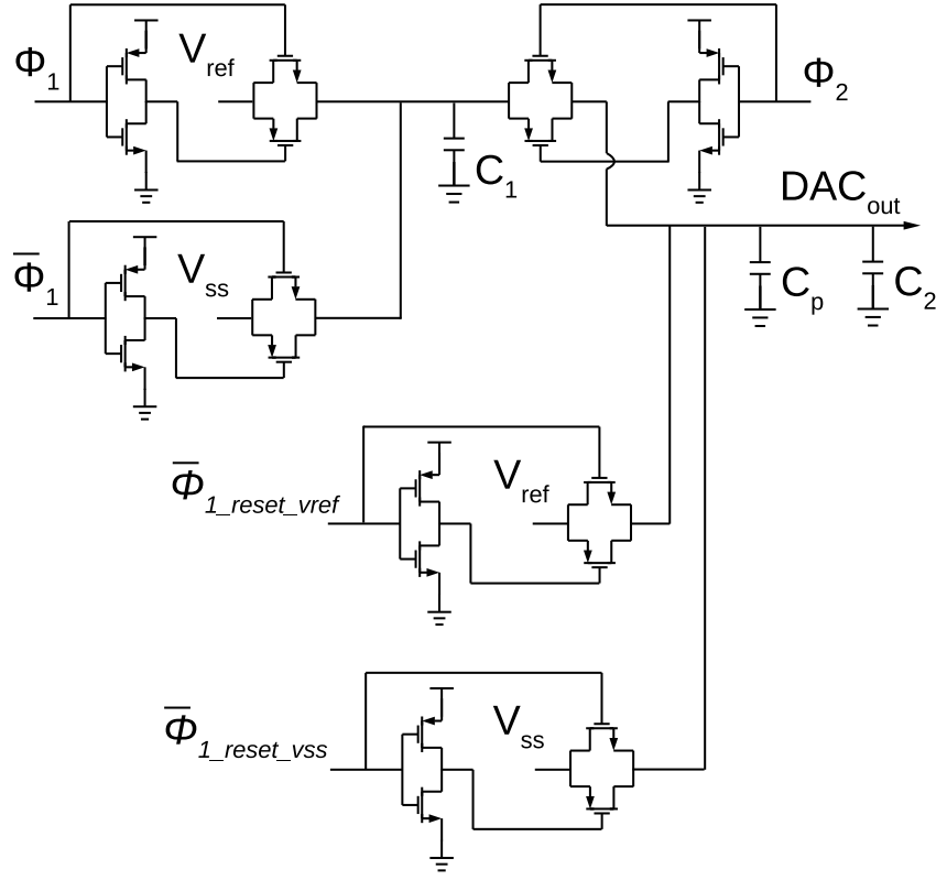
Figure 5.2: Transistor level implementation of the DAC including parasitic capacitor C_p and illustrating both ramp up and ramp down capability.
