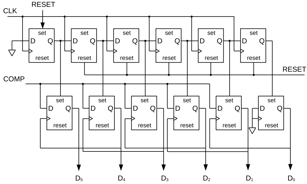
Figure 2.34: SAR logic for a 6-bit converter.
