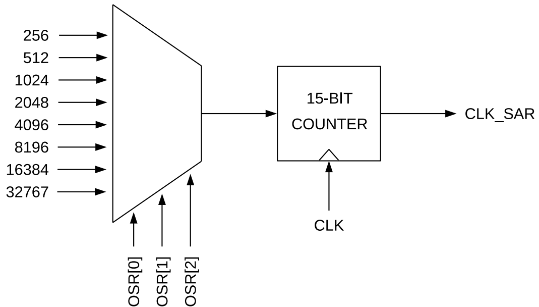
Figure 3.33: Clock Divider.
