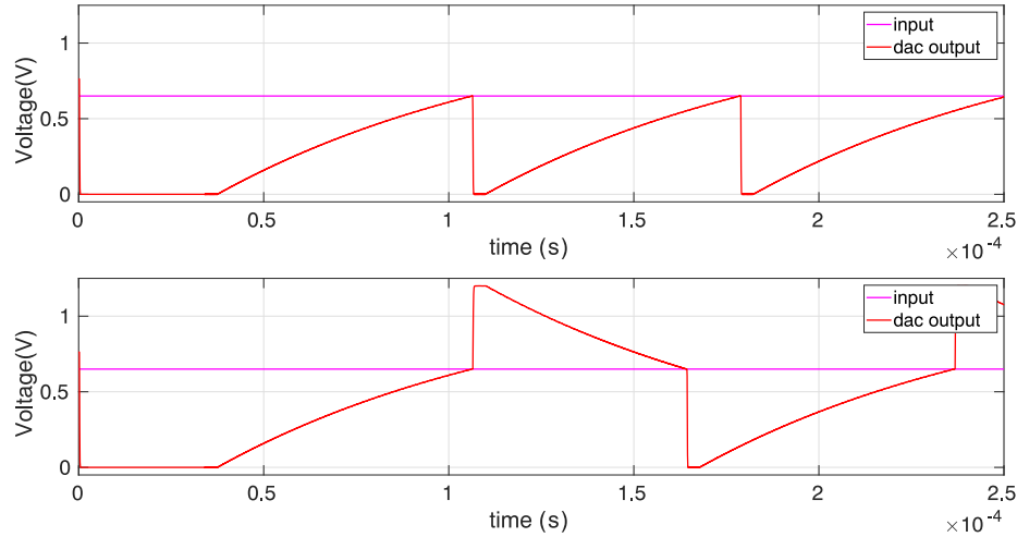
Figure 5.4: Modes of operation illustrated. Ramping up only (top) and Ramping up then ramping down (bottom).
