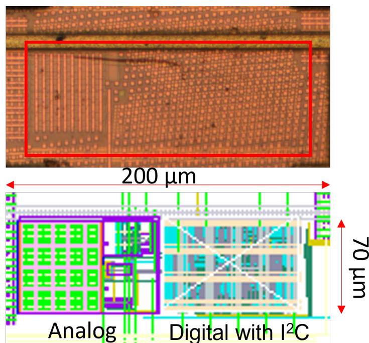
Figure 5.7: Die micrograph.
