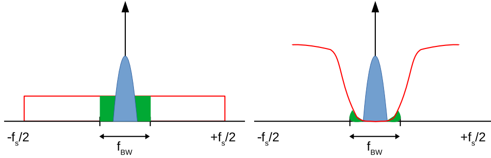
Figure 2.17: Noise shaping of the quantisation noise.
