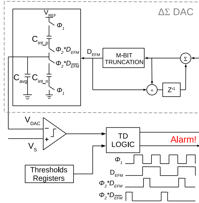
Figure 4.4: Schematic of the proposed Threshold Detection based ADC with a timing diagram.
