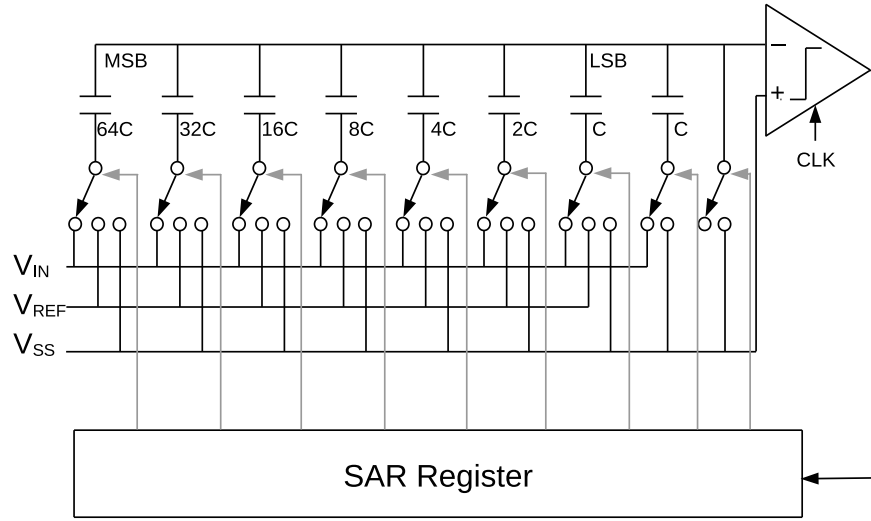
Figure 2.28: Conventional implementation of DAC in single-ended ADCs.
