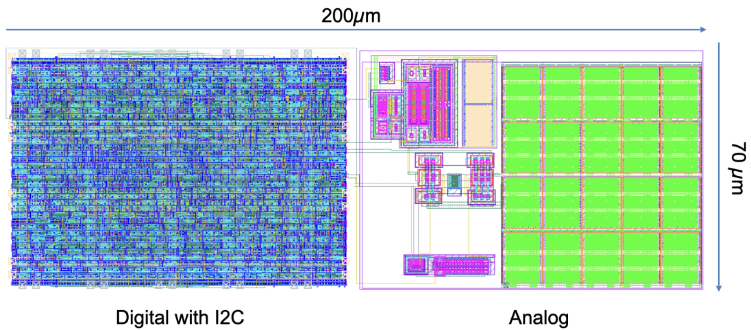
Figure 5.5: Layout of the implemented counting BDC.
