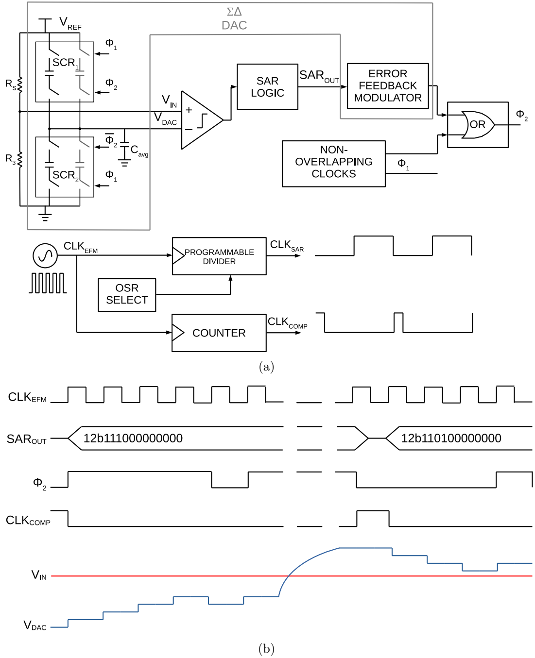
Figure 3.11: Detailed view of the proposed architecture including internal clock generation (a) and system timing diagram (b).
