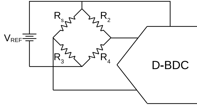
Figure 2.38: System diagram of a Direct Bridge-to-Digital Converter.
