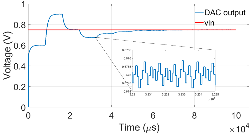
Figure 3.8: Simulated DAC settling and the concomitant ripple (inset).
