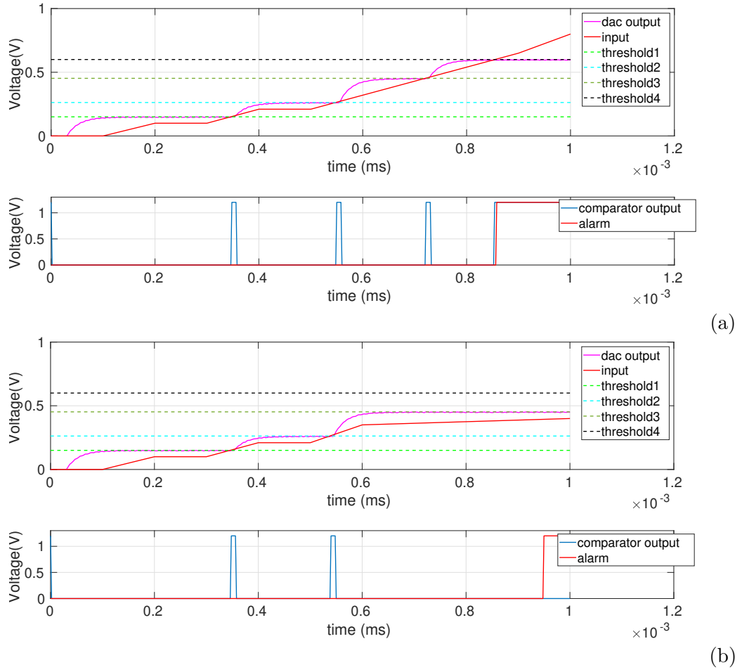
Figure 4.6: The post-layout simulation results of the Threshold Detection ADC operation for (a) threshold triggered alarm and (b) delay triggered alarm scenario.
