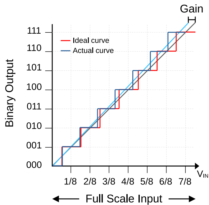
Figure 2.8: Representation of the gain error, showing the deviation from the ideal transfer function.
