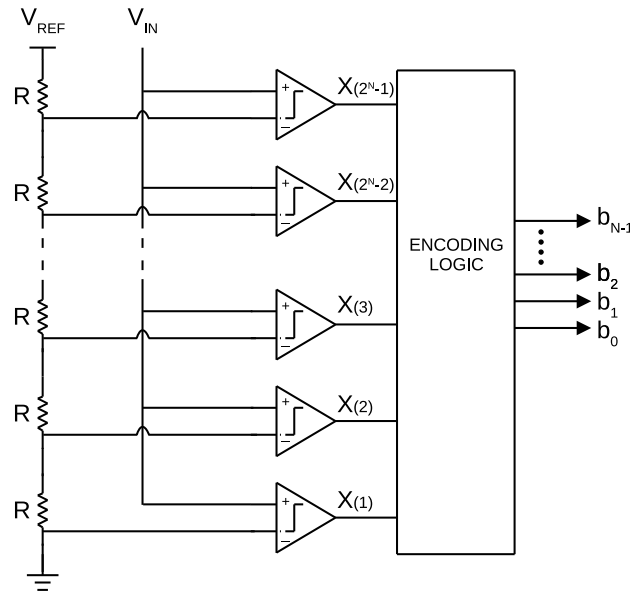
Figure 2.14: Simplified block diagram of a Flash ADC.
