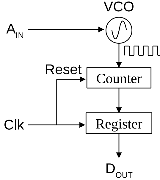
Figure 2.27: VCO-based quantizer.
