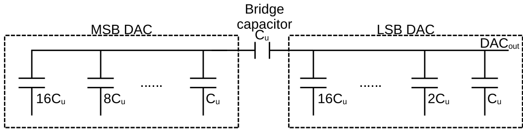
Figure 2.29: Diagram of a 5-5 split-capacitor DAC.
