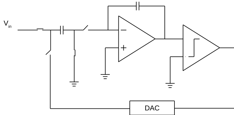
Figure 2.18: Simplified block diagram of a noise-shaping ADC.
