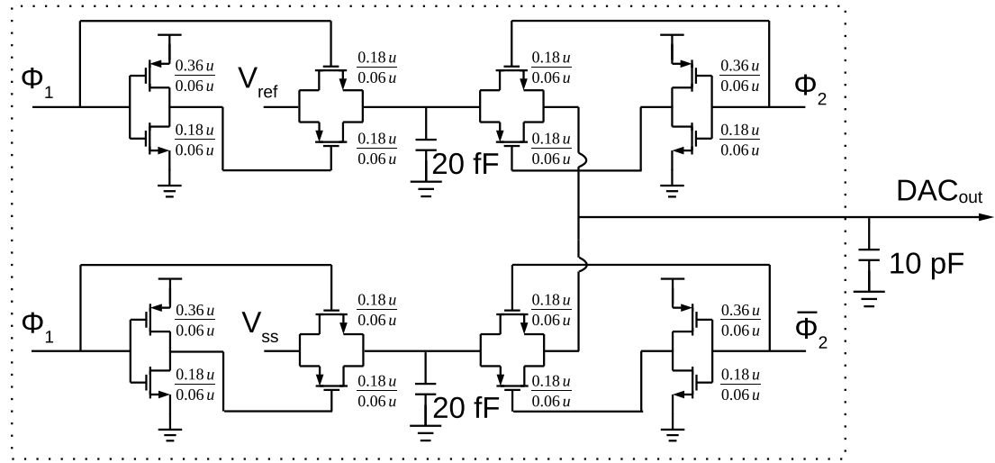
Figure 3.14: Transistor level diagram of the switched capacitor resistor cells with the unit capacitors.
