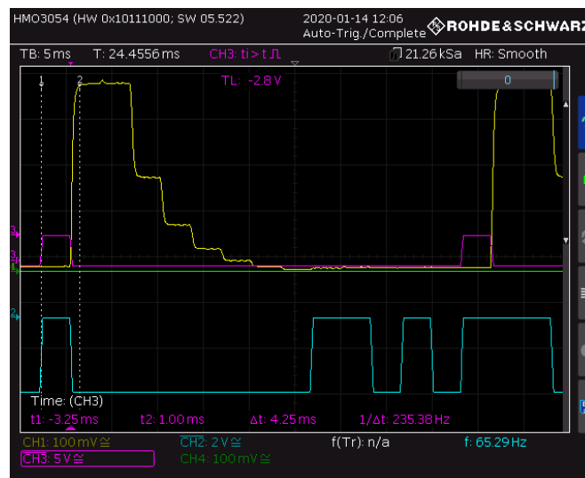
Figure 3.39: DAC convergence for 0V input.
