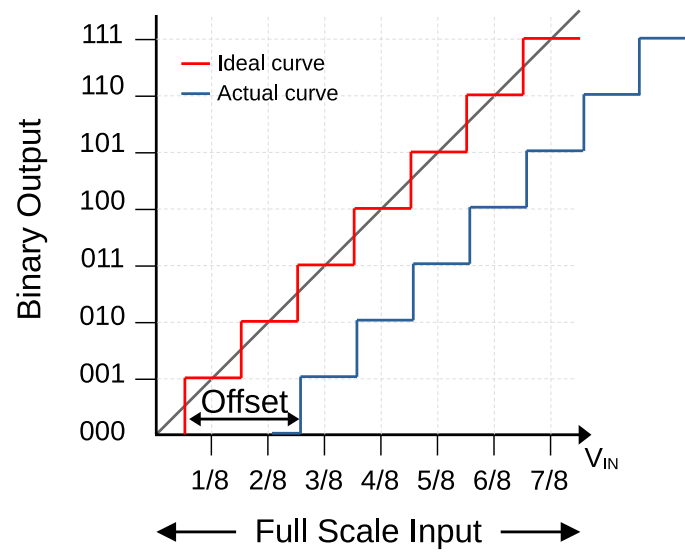
Figure 2.7: Representation of the offset error, shown as the distance from the ideal transfer function.
