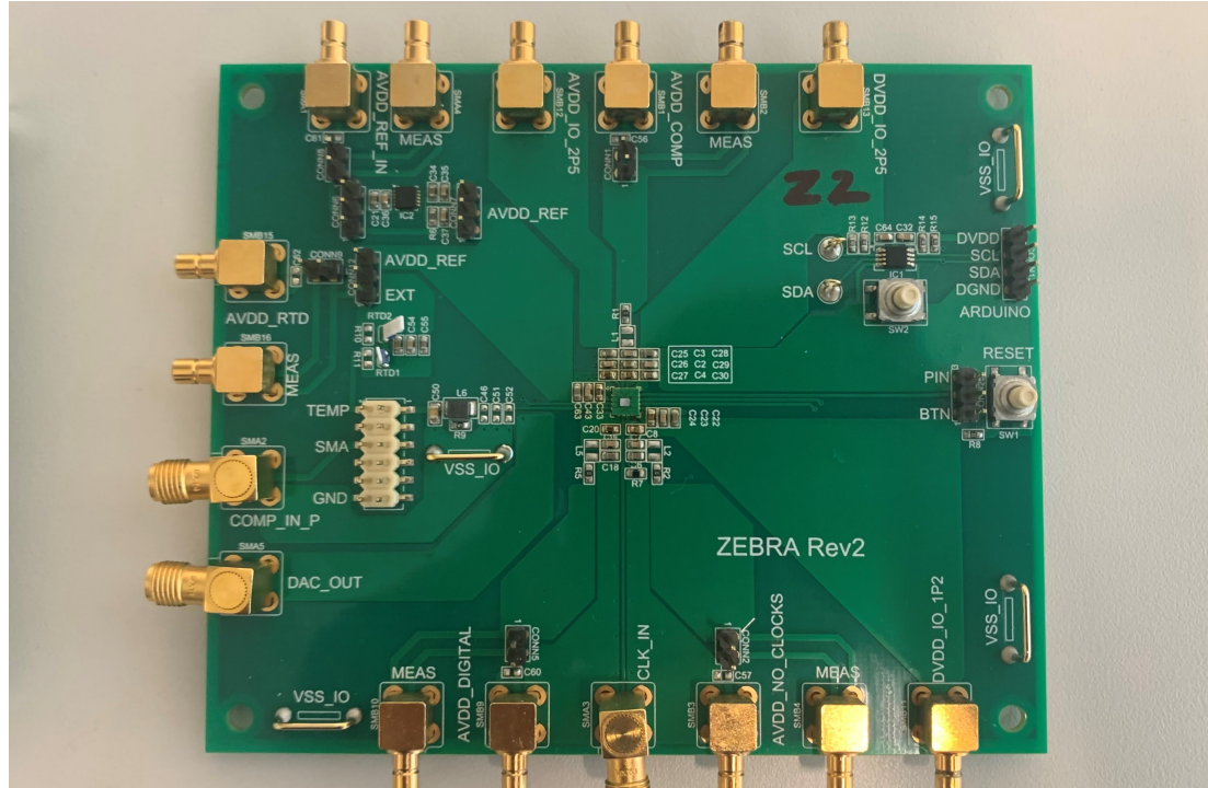
Figure 5.8: Photograph of a PCB board with an interposer.
