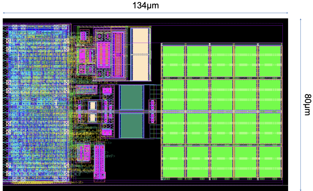
Figure 3.12: Top level layout of the BDC.
