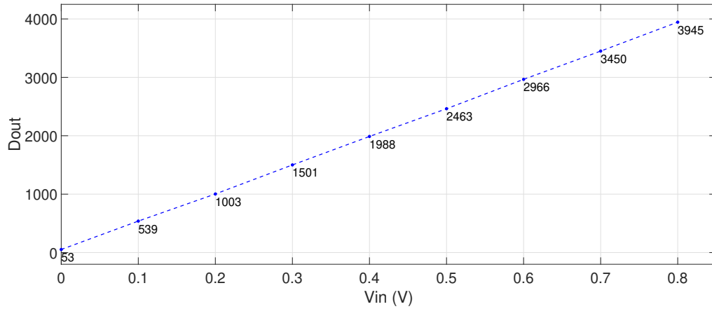
Figure 3.41: Plot of an output code vs the input voltage.
