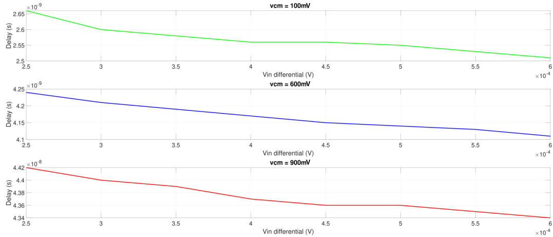
Figure 3.26: Extracted results showing a maximum comparator delay of 45 ns across the input common mode.
