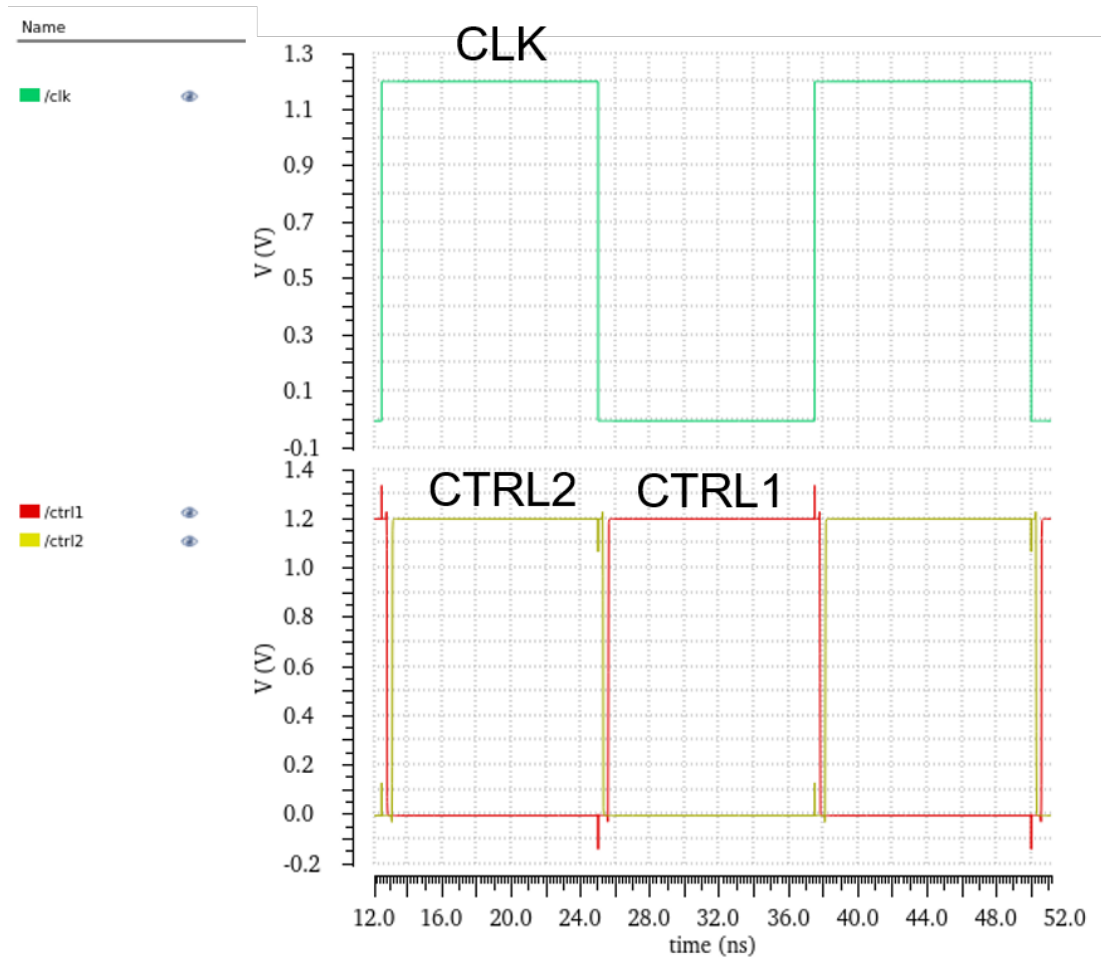
Figure 3.20: Extracted (post layout) simulation of non-overlapping clocks.
