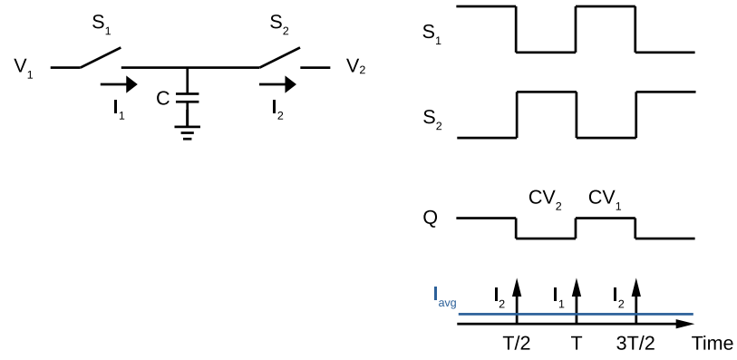
Figure 3.3: Switched capacitor resistor with timing diagram [110].
