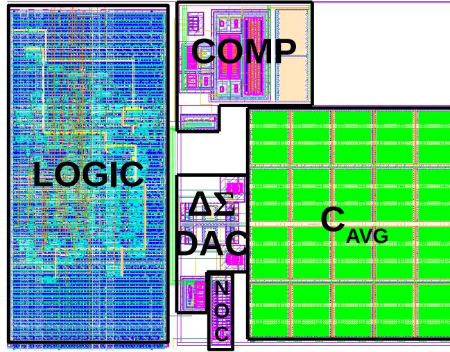
Figure 4.5: Layout of the Threshold Detection ADC occupying 0.012 \text{ mm}^2 in 65 nm CMOS.
