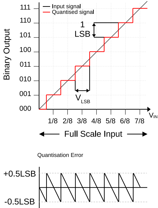
Figure 2.4: ADC transfer characteristics. LSB definition and quantisation error (for 3-bit ADC).
