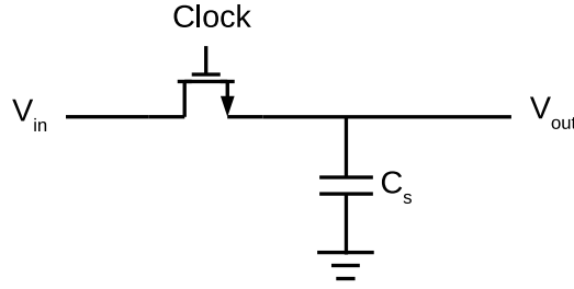
Figure 2.10: Sampling switch implemented with MOS.
