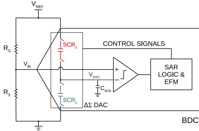
Figure 3.4: Top level block diagram of the SAR based BDC.
