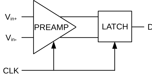
Figure 2.32: Main building blocks of a dynamic comparator, consisting of preamplifier and a latch.
