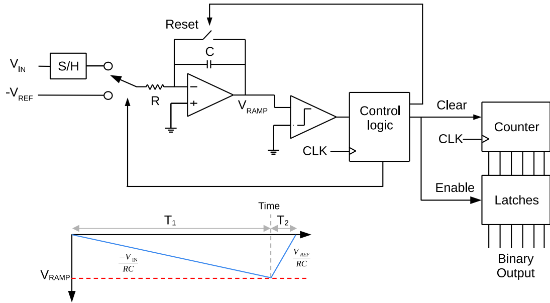
Figure 2.25: Simplified diagram of a conventional dual slope-based ADC with a timing diagram.
