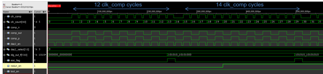
Figure 3.30: Simulated sample configuration of the BDC showing 12 and 14-bit decision cycles.
