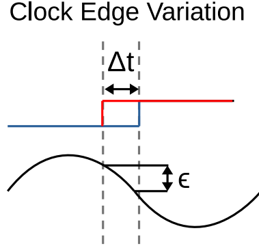
Figure 2.12: Sampling errors due to clock jitter.
