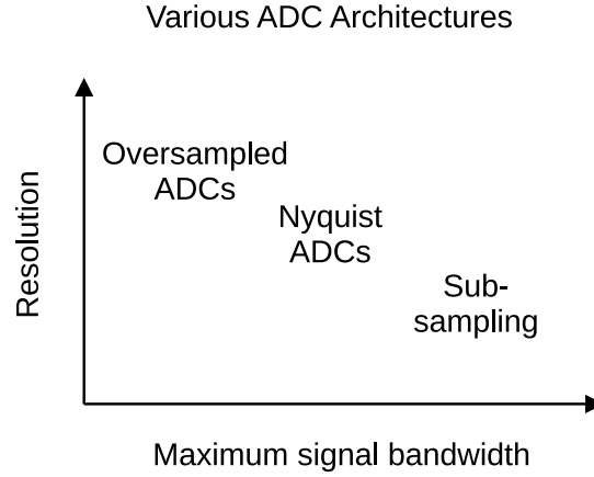
Figure 2.13: A representation of the resolution vs maximum signal bandwidth of three different types of ADCs.
