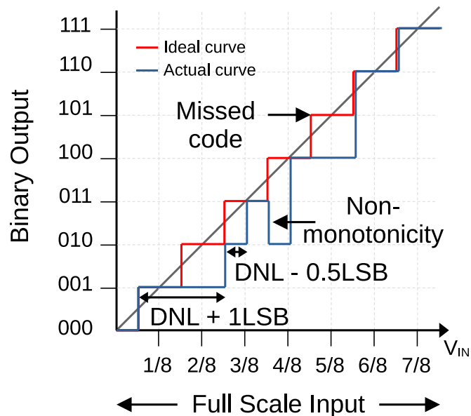
Figure 2.6: Representation of the differential linearity, illustrating disparities between ideal and actual curves.
