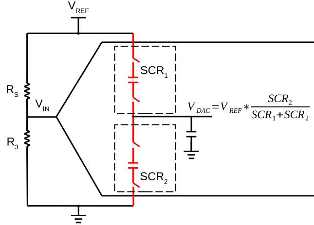
Figure 3.2: WhB with switched capacitor resistors.
