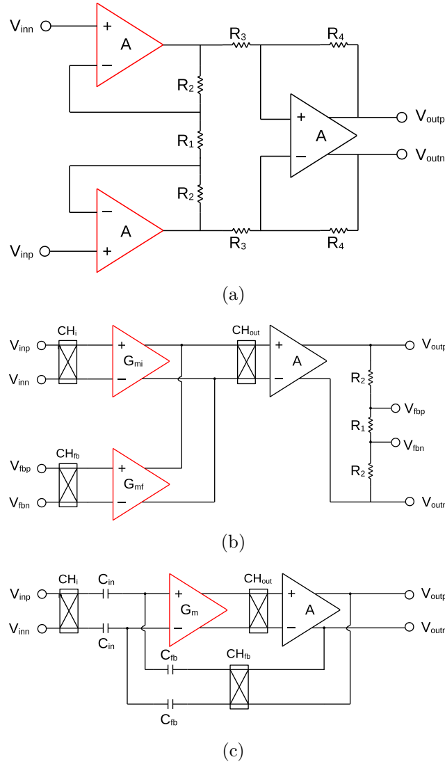
Figure 2.37: Standard architectures of three-opamp (a), CFIA (b) and CCIA (c) instrumentation amplifiers. CFIA and CCIA both employ chopping.
