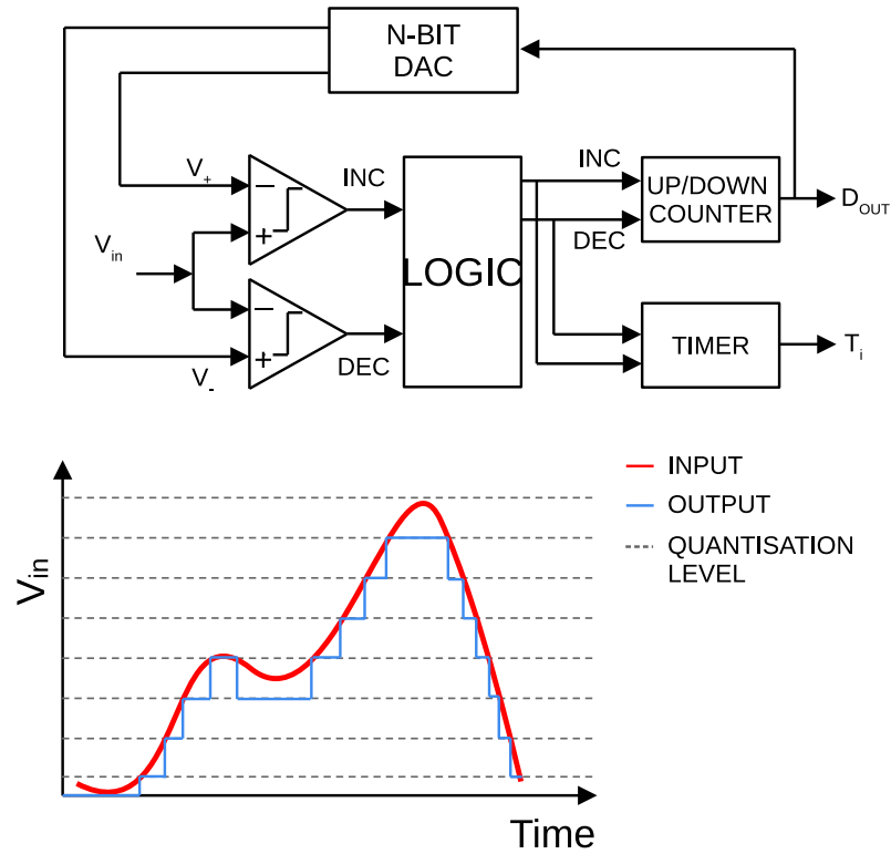
Figure 2.23: Diagram of Level crossing ADC with conversion levels.
