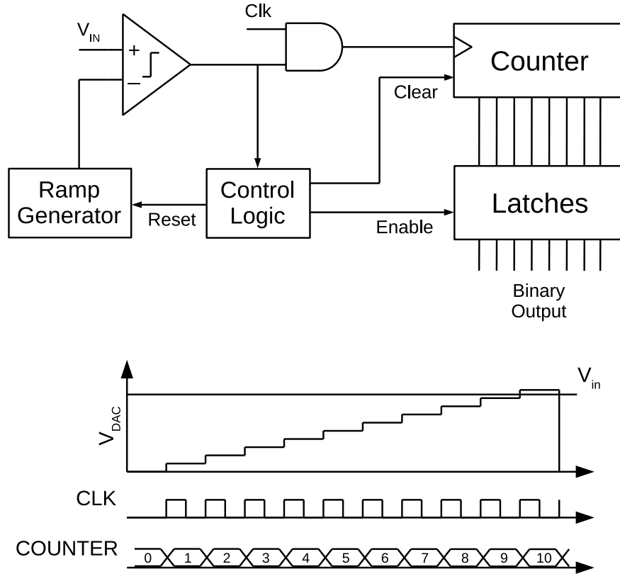
Figure 2.26: Block diagram of a counter ADC with a timing diagram
