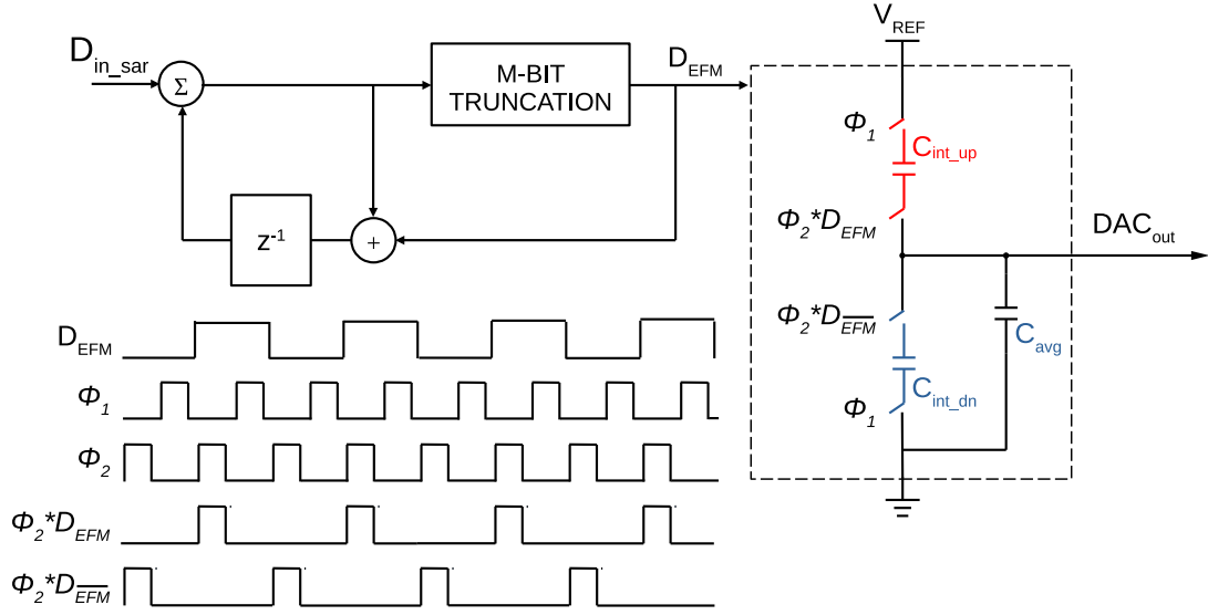
Figure 3.7: A block diagram of an error-feedback modulator driving switched capacitor resistors.
