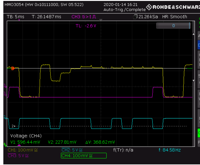
Figure 3.40: DAC convergence for 0.6 V input.
