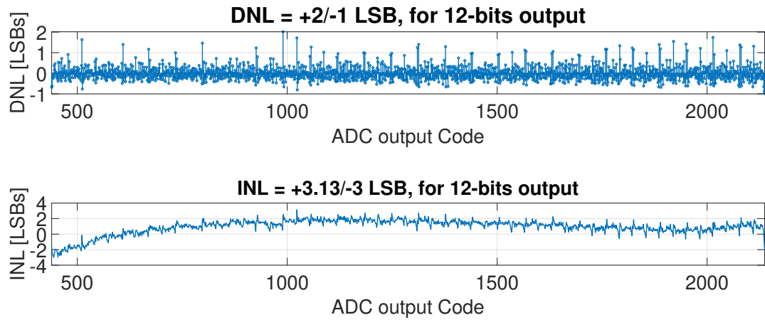
Figure 3.42: Measured DNL and INL for ramp input.
