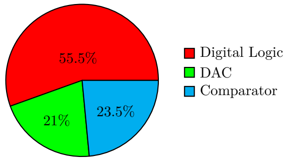
Figure 3.45: Power consumption breakdown of the BDC operating at a 10 MHz clock frequency and 32768 OSR.
