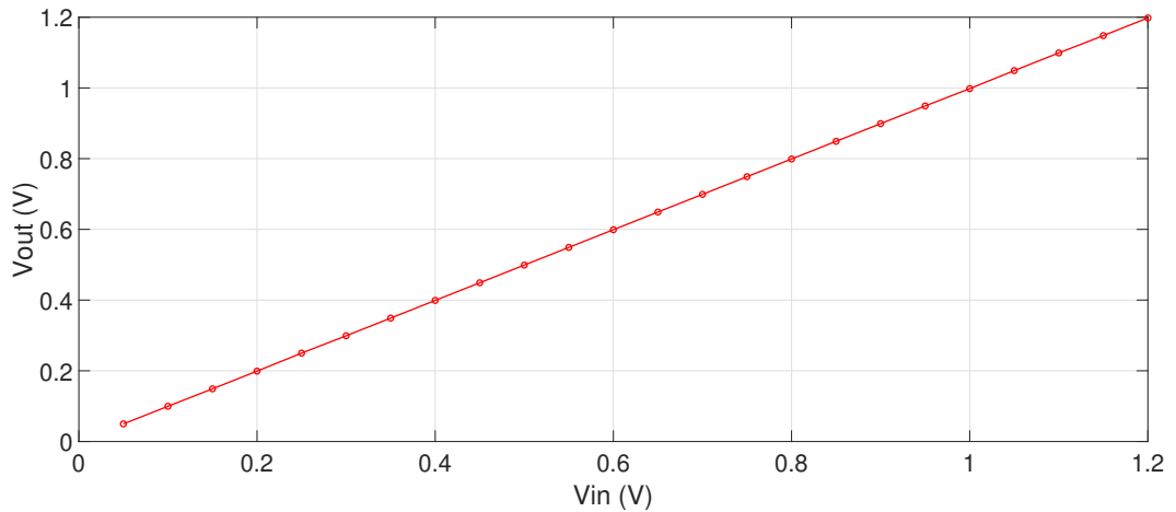
Figure 3.17: EFM output versus input.
