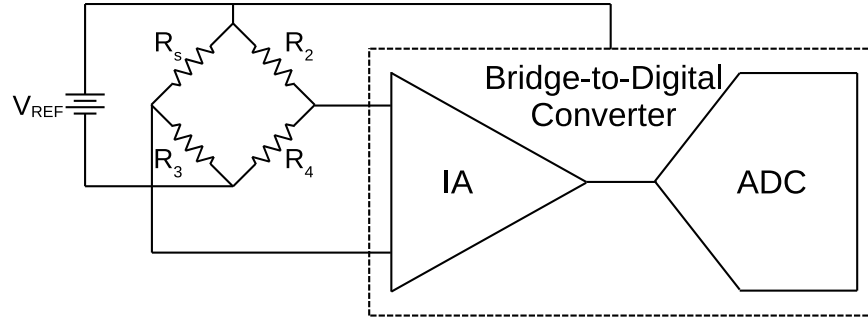
Figure 2.36: System diagram of a conventional Bridge-to-Digital Converter.
