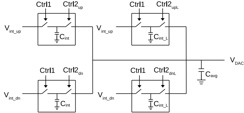
Figure 3.9: Schematic of a DAC showing implemented SCRs with their control signals.
