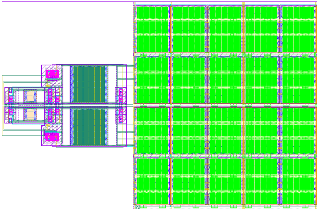
Figure 3.15: Layout of the switched capacitor resistor cells and the averaging capacitor.
