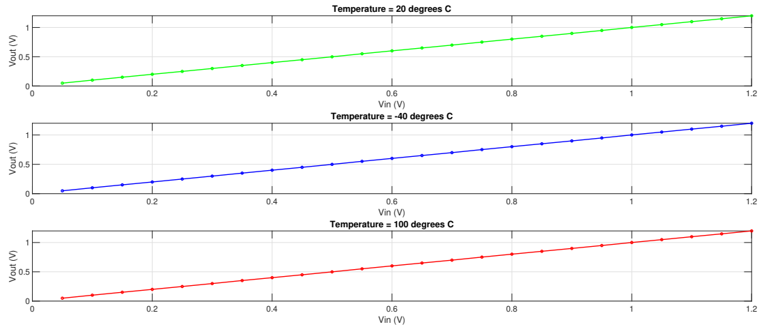
Figure 3.23: DAC linearity for temperature range.
