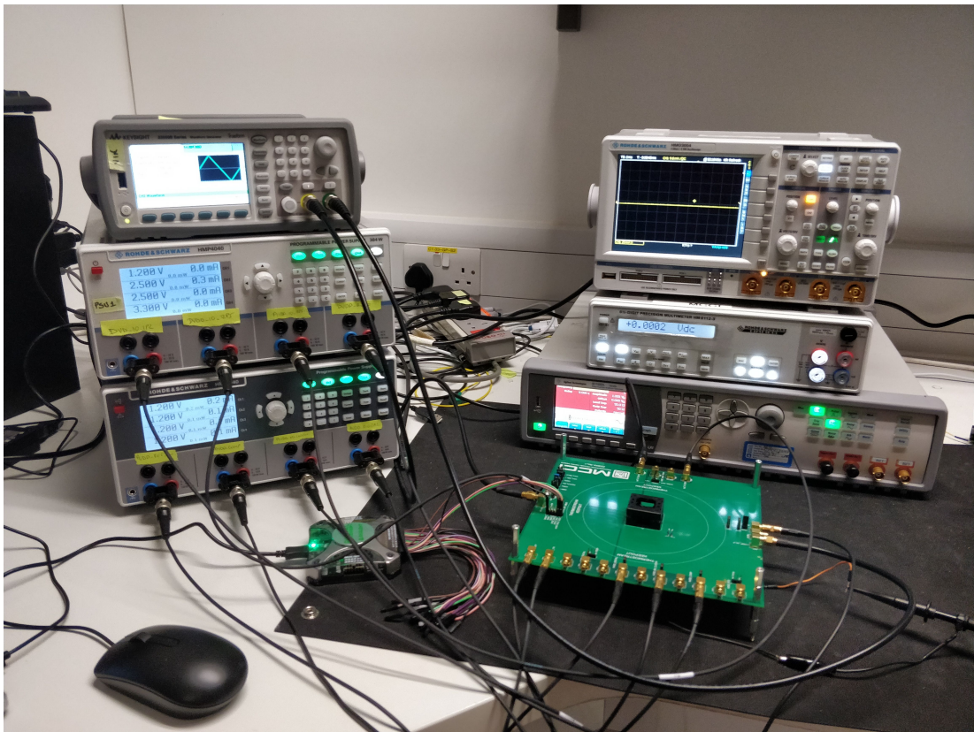
Figure 3.38: Photograph of laboratory setup.
