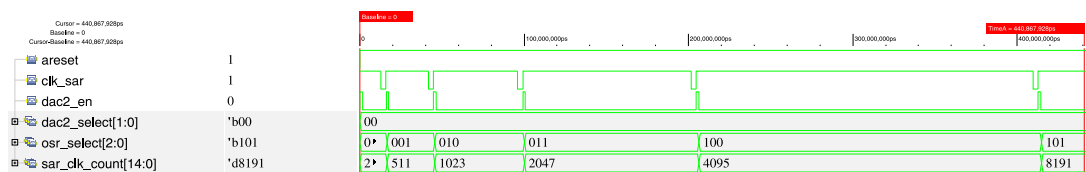
Figure 3.34: Operation of the 8:3 multiplexer.
