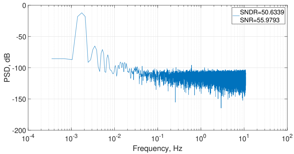
Figure 3.44: Measured output spectrum (65 536 points).
