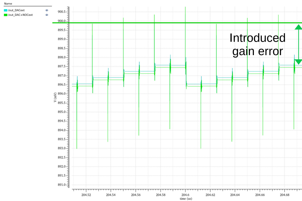
Figure 3.22: The extracted results showing introduced gain error that is due to layout related mismatch.
