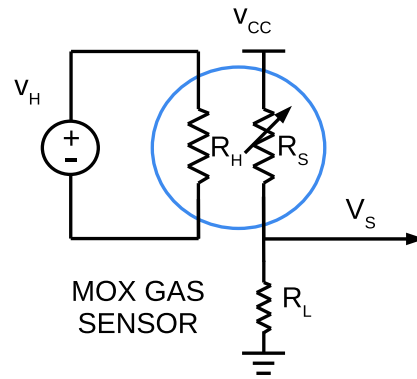
Figure 1.2: An equivalent circuit diagram of a MOX sensor.
