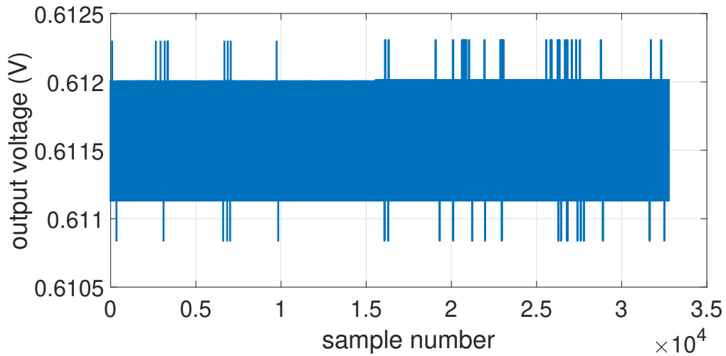
Figure 3.43: Repeatability test for a 600 mV input signal.
