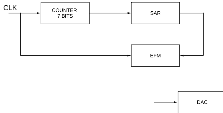
Figure 3.29: Representation of blocks implemented within the logic.
