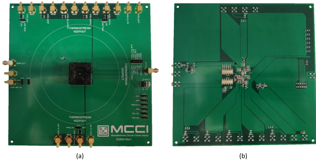
Figure 3.37: Designed PCB. Front (a) and back (b).
