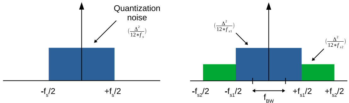
Figure 2.16: Quantisation noise inside and outside the band of interest.
