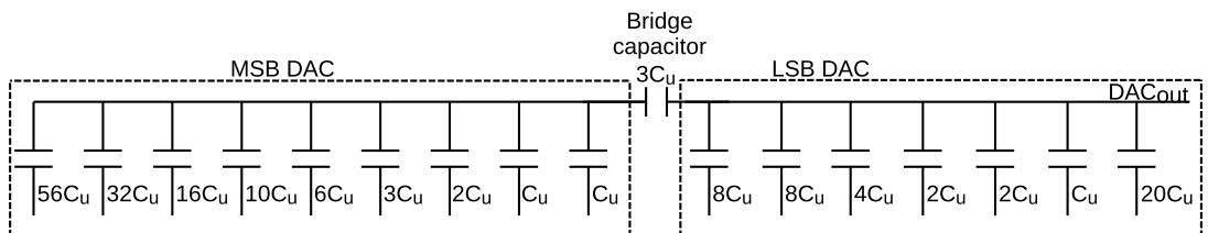
Figure 2.30: Schematic of a split-capacitor DAC array with redundancy [75].
