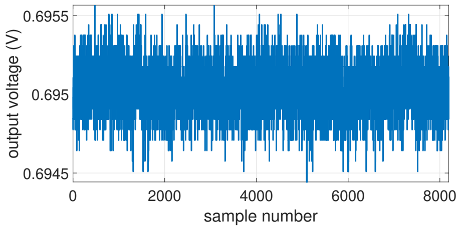
Figure 5.11: Repeatability test results showing rms noise of 0.15 mV.
