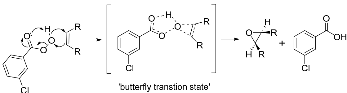
Scheme 2.59
