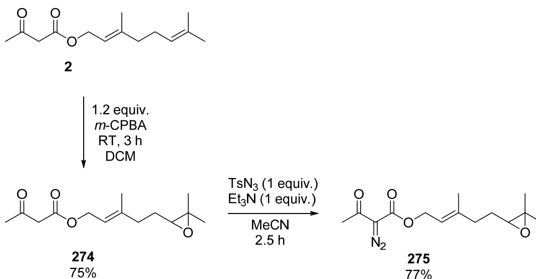
Scheme 2.63
