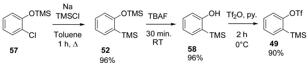
Scheme 2.11
