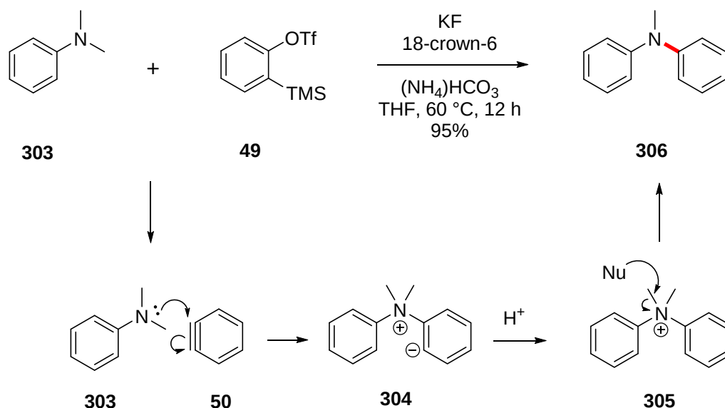
Scheme 2.77
