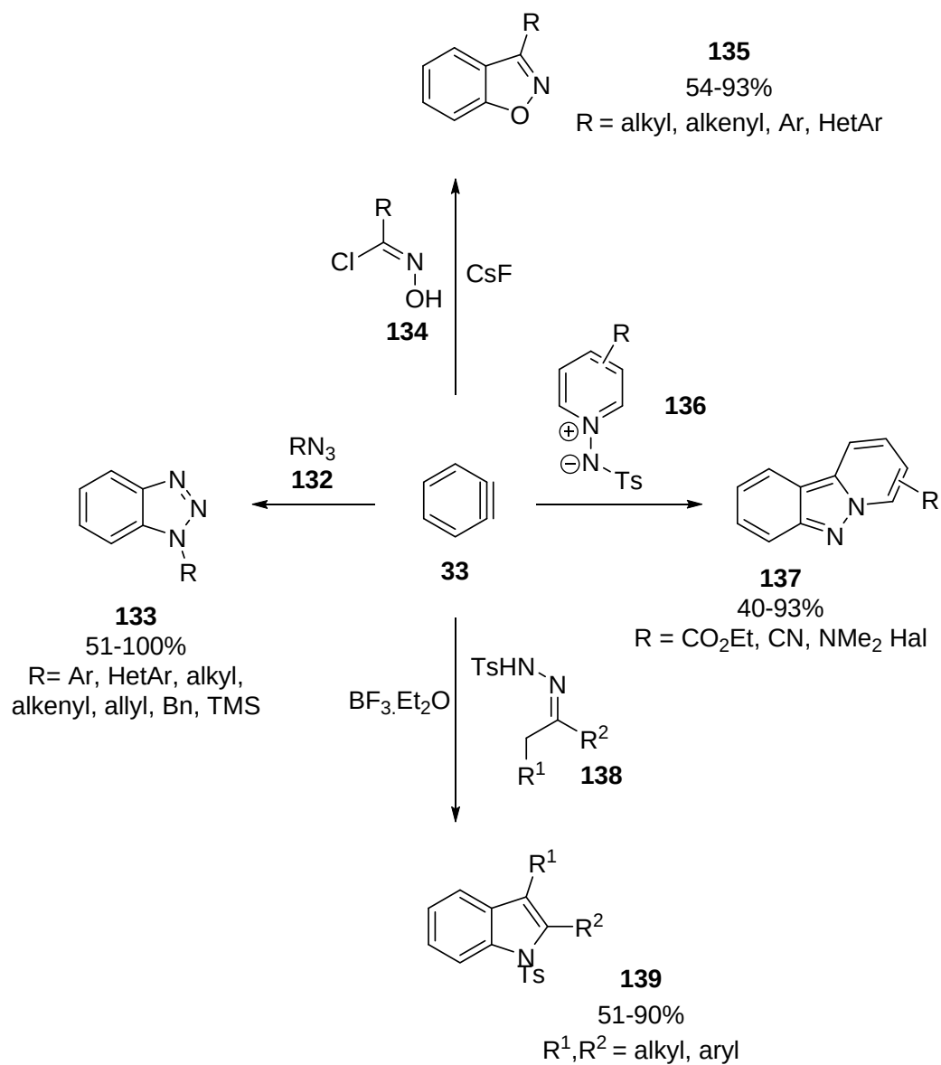
Scheme 1.35
