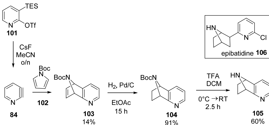
Scheme 1.24
