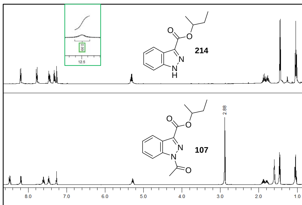
Figure 2.52 ^1\text{H} NMR spectra comparison 1-acetyl-indazole 107 vs 1H-indazole 214
