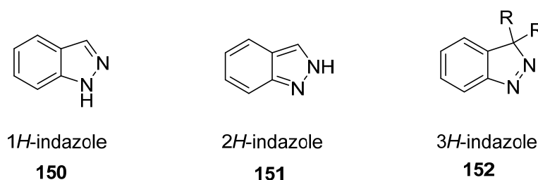
Figure 1.11 Indazole tautomer forms
