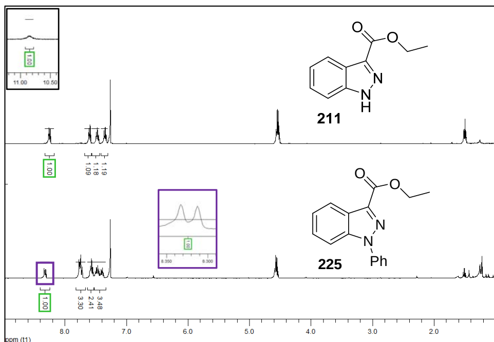
Figure 2.54 1 H NMR spectra of aryl region of 225 vs 211
