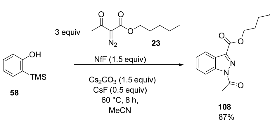
Scheme 2.39
