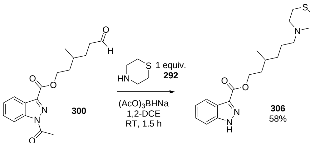
Scheme 2.78
