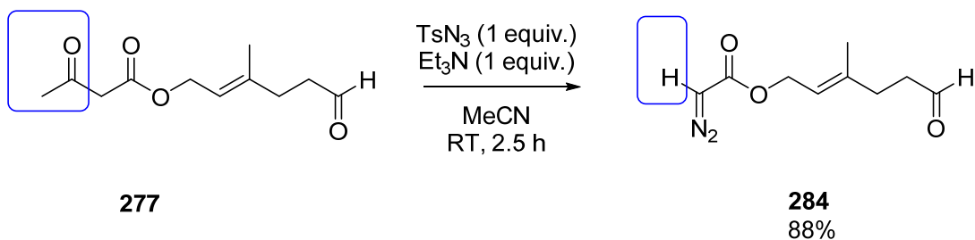
Scheme 2.67
