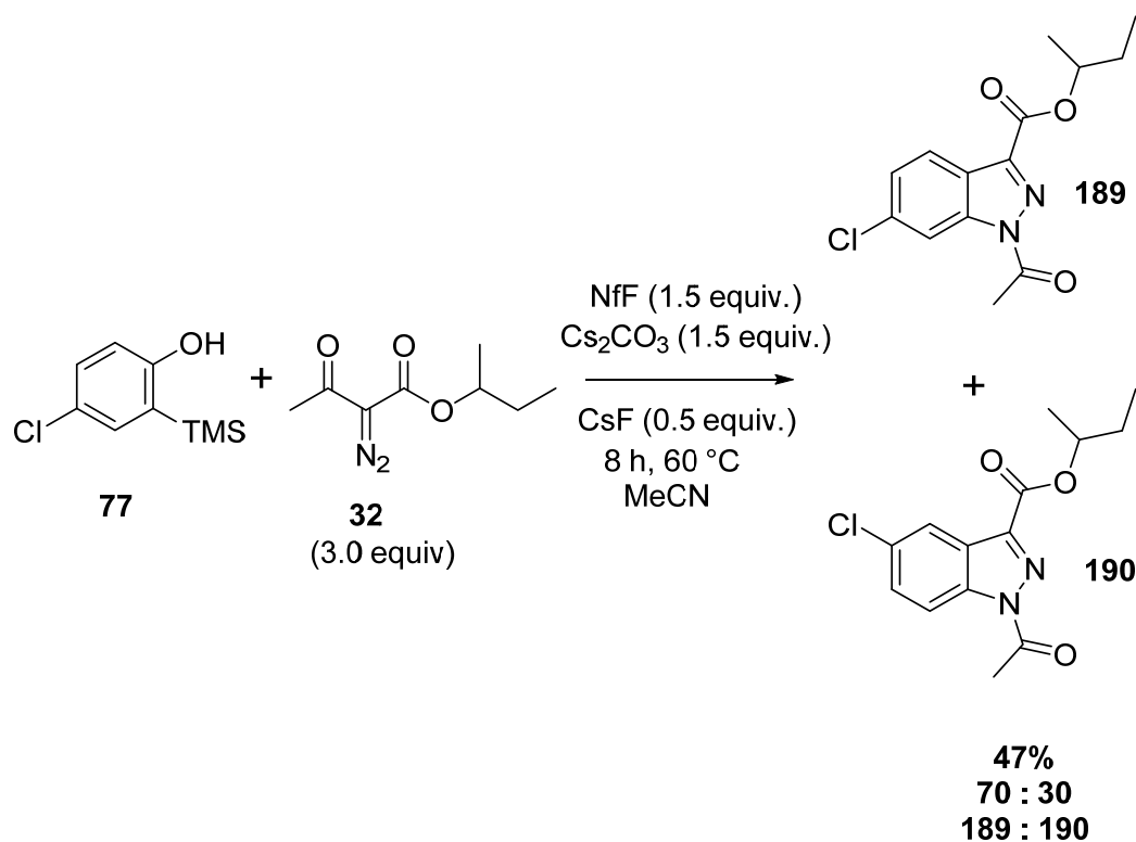
Scheme 2.41
