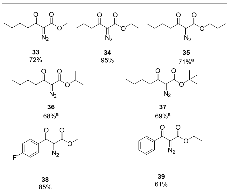
Figure 2.4 Summary of lengthened ketone side-chain \alpha -diazo- \beta -ketoester derivatives
