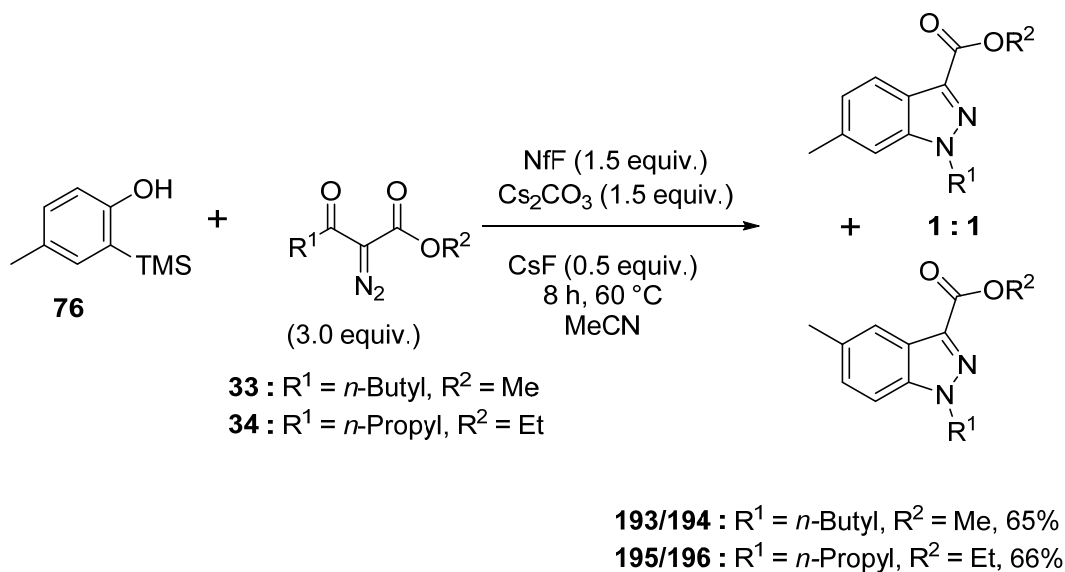
Scheme 2.43
