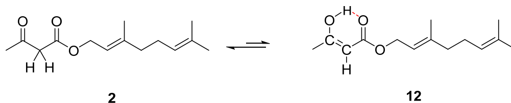
Scheme 2.4
