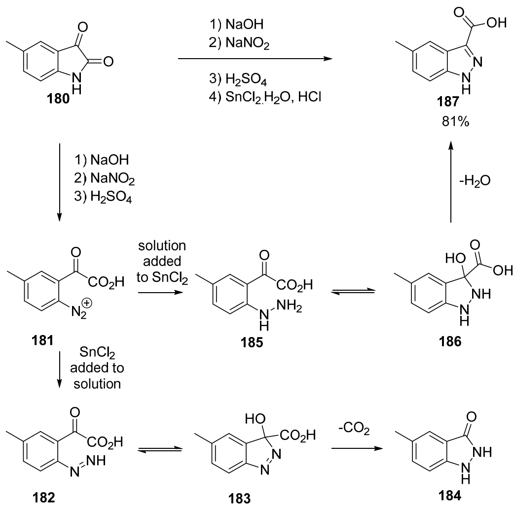
Scheme 1.45
