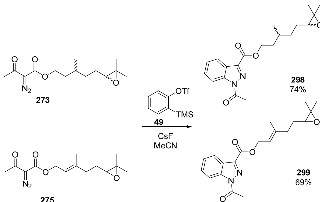
Scheme 2.73
