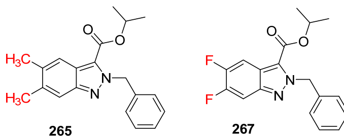
Figure 2.101 Derivatives possibly sharing mechanism of action
