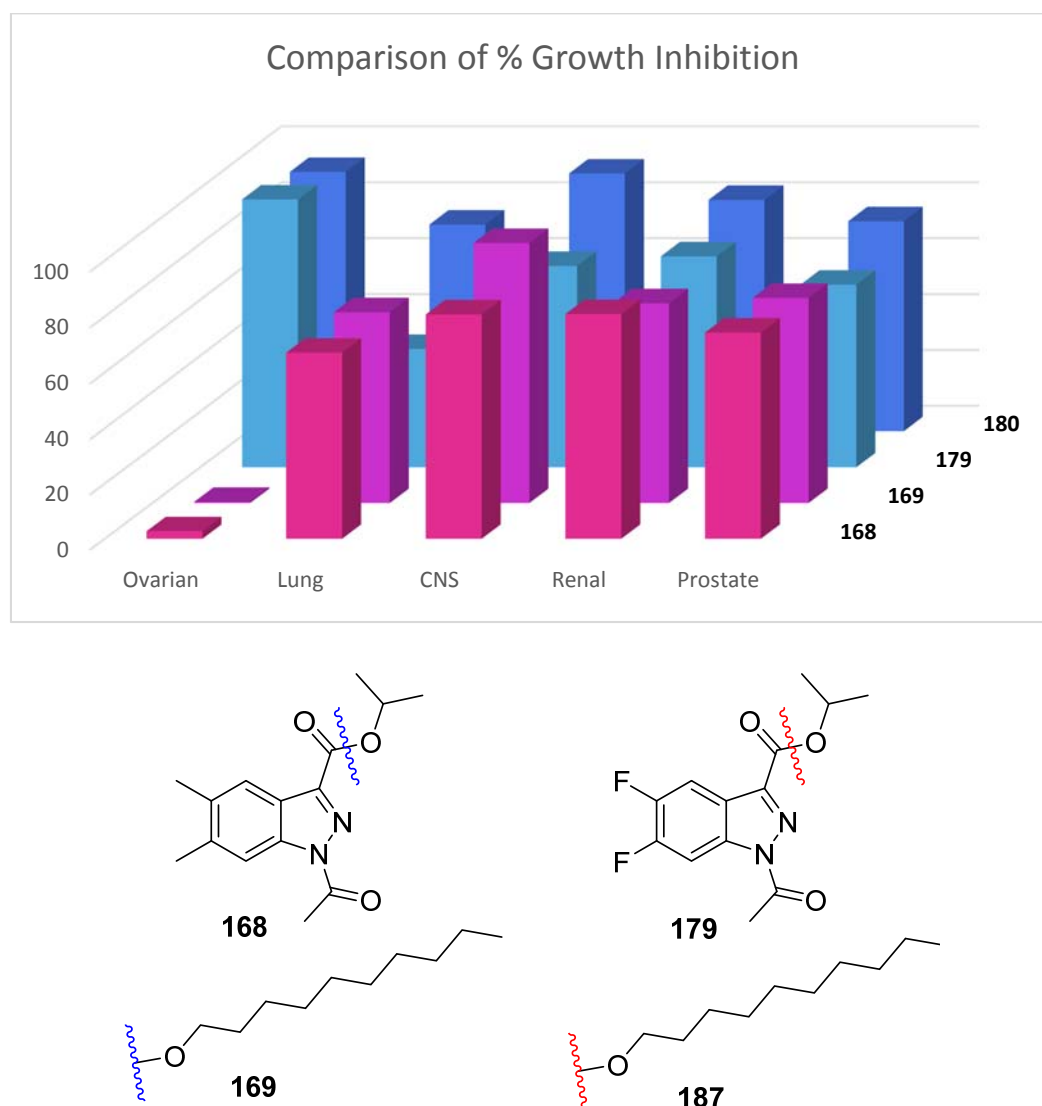
Figure 2.95 Comparison of dimethyl and difluoro indazoles
