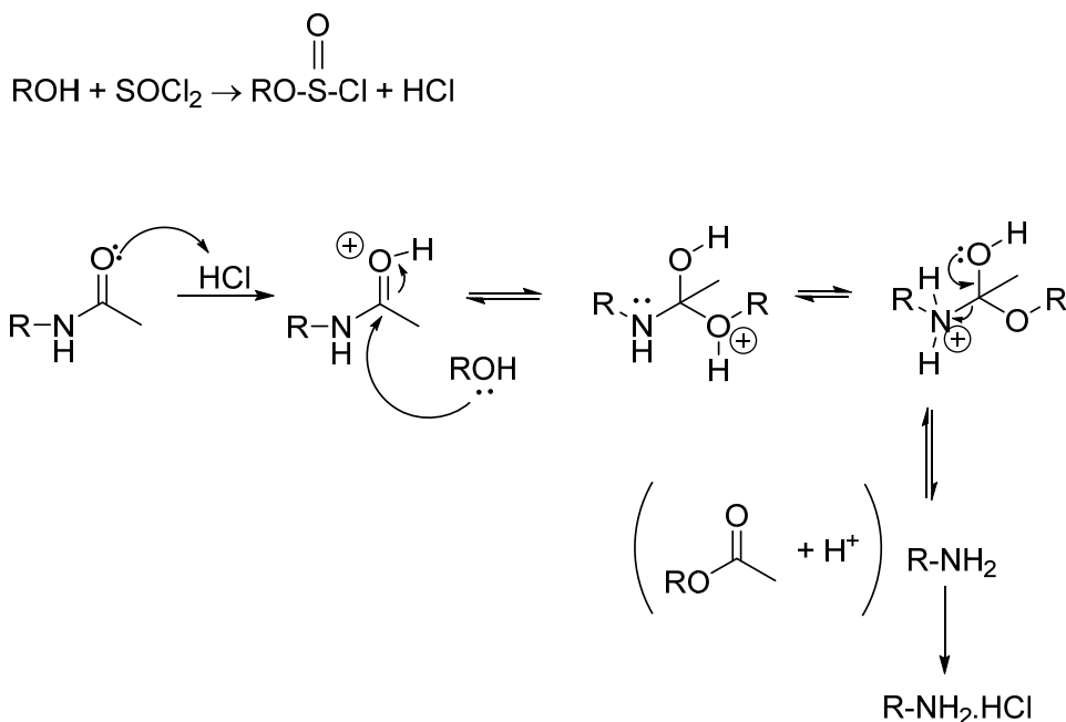
Scheme 2.48
