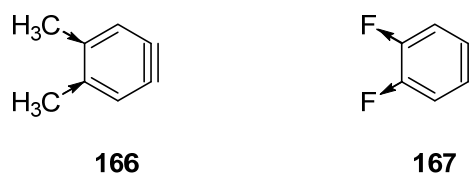
Figure 2.38 Symmetrical aryne precursors with EDG and EWG
