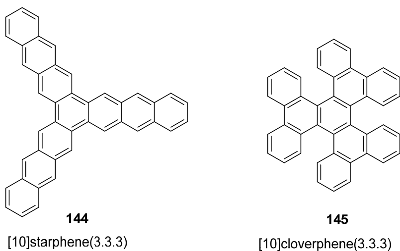
Figure 1.9 Benzyne-derived polycyclic aromatic hydrocarbons
