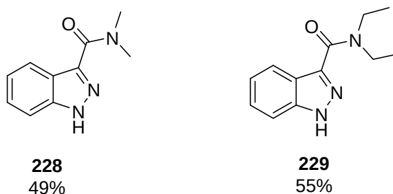
Figure 2.56 1 H -indazole carboxamide derivatives
