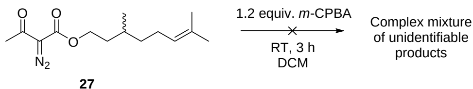
Scheme 2.62
