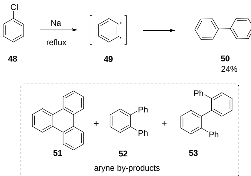
Scheme 1.14
