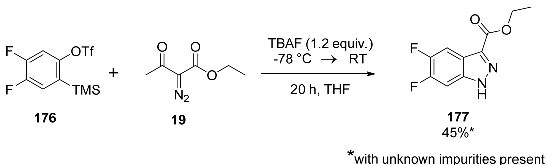
Scheme 2.40 Larock's only example of a difluoro indazole
