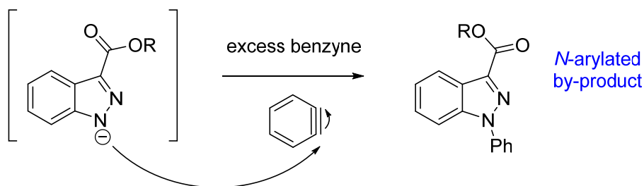
Scheme 2.25
