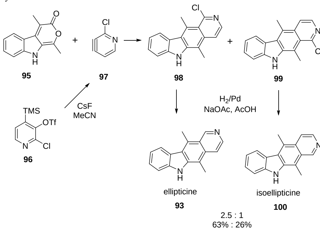
Scheme 1.23
