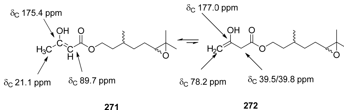
Figure 2.72 Evidence of both enol forms in ^{13}\text{C} NMR spectrum
