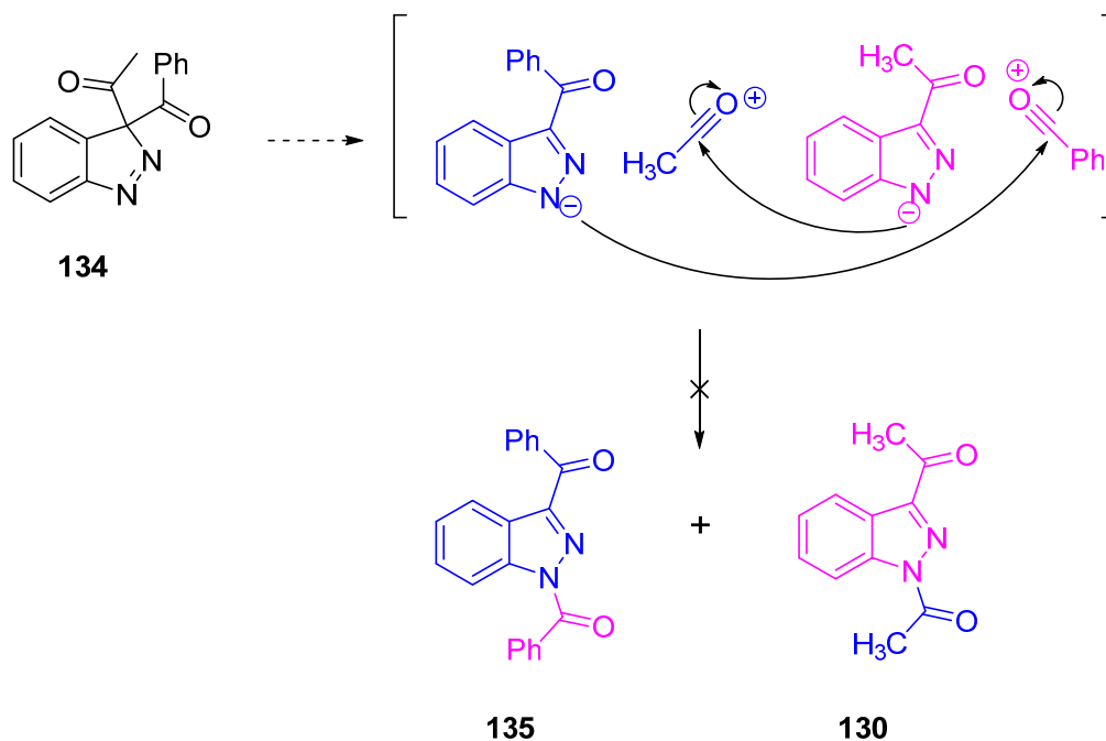
Scheme 2.28
