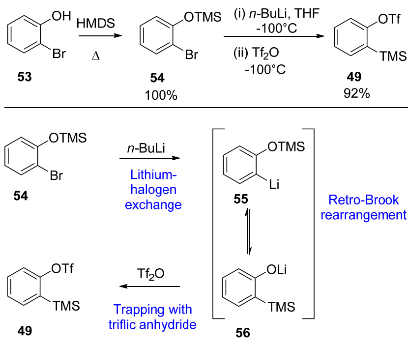
Scheme 2.10
