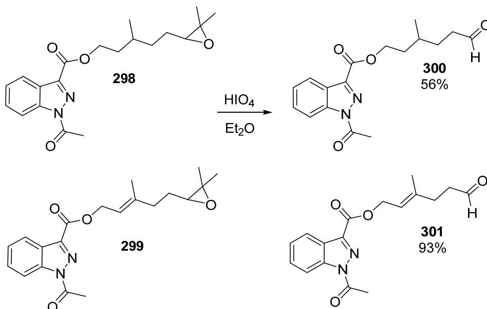
Scheme 2.75
