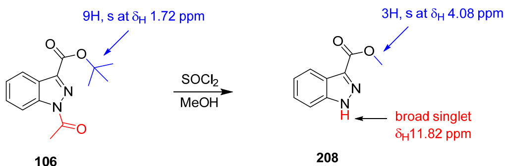
Scheme 2.49
