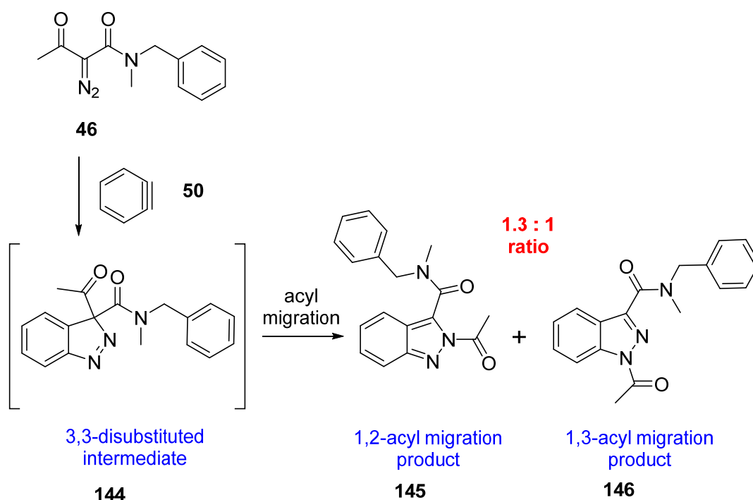
Scheme 2.33
