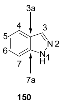
Figure 1.10 1 H -Indazole numbering convention
