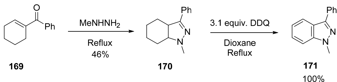
Scheme 1.42
