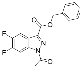
benzyl 1-acetyl-5,6-difluoro-1 H -indazole-3-carboxylate 181
