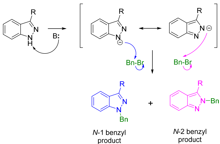
Scheme 2.55
