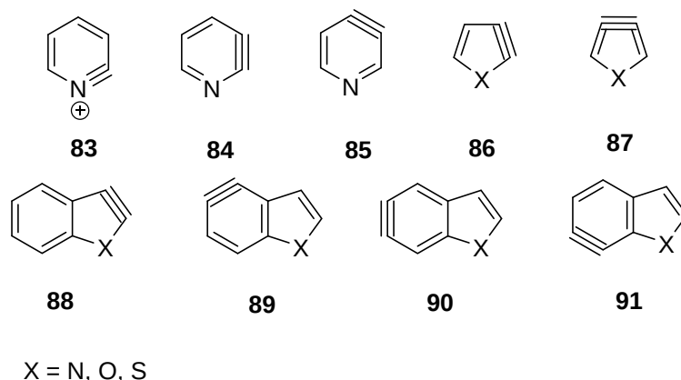
Figure 1.7 Well-known and postulated hetaryne intermediates
