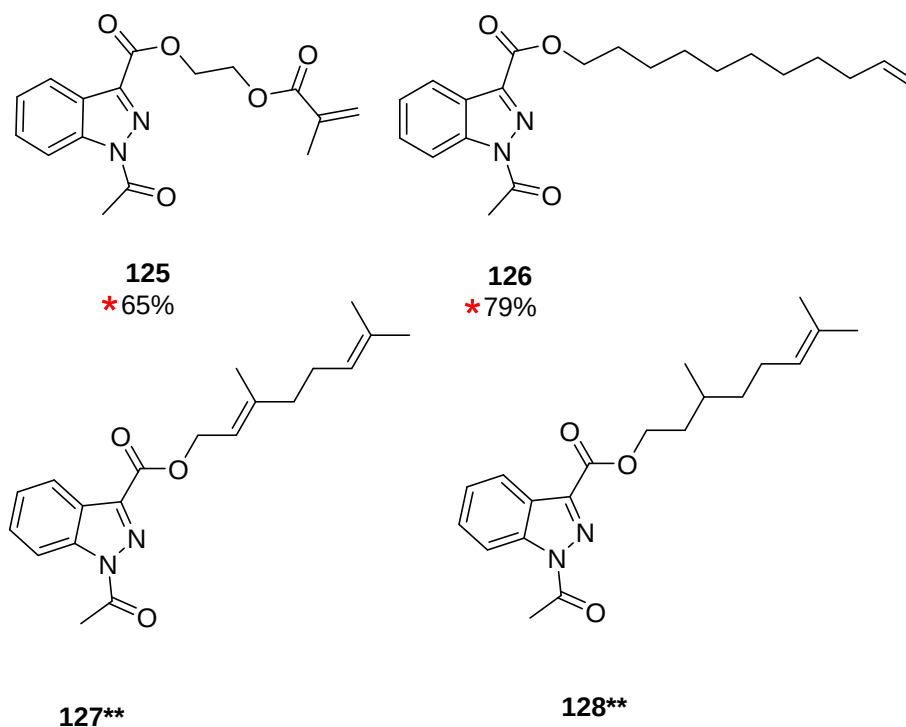
Figure 2.24 Further indazole derivatives prepared
