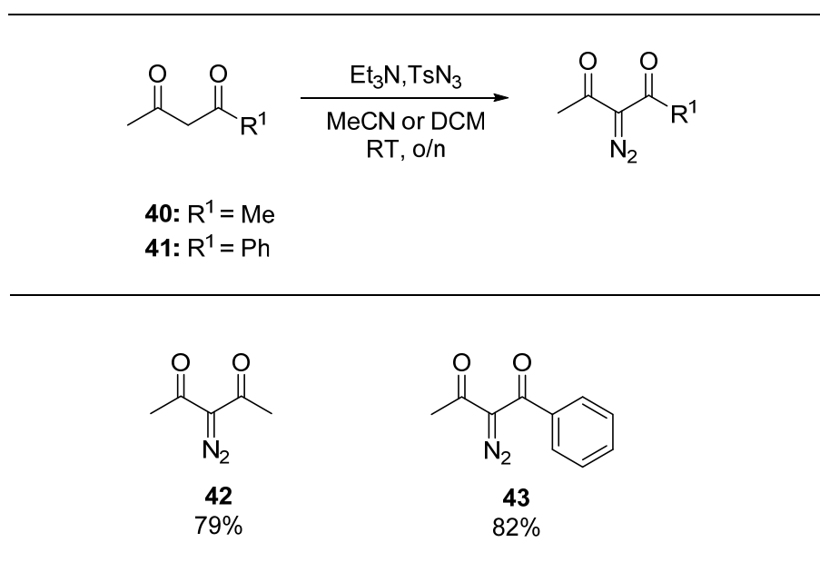
Figure 2.5 Summary of \alpha -diazo- \beta -diketone derivatives
