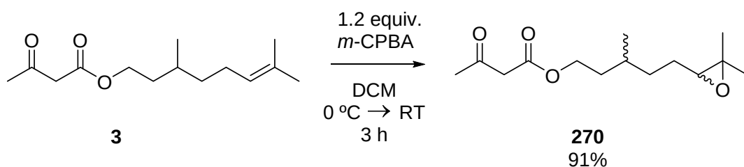
Scheme 2.60
