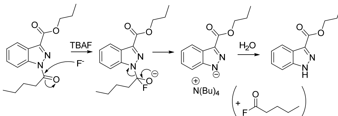
Scheme 2.52
