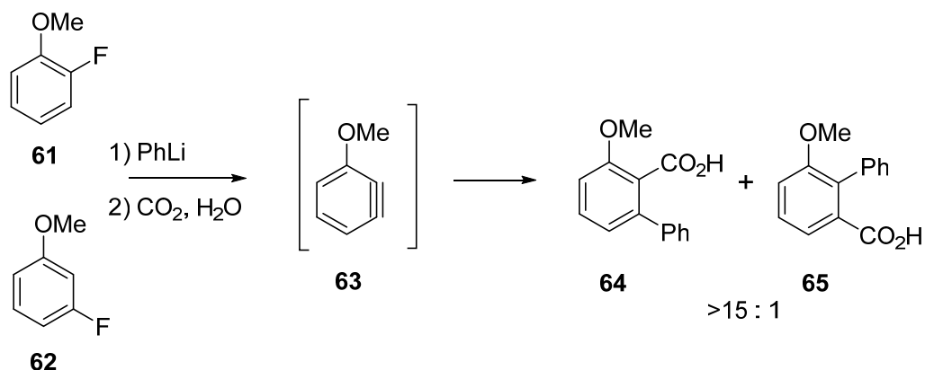
Scheme 1.17
