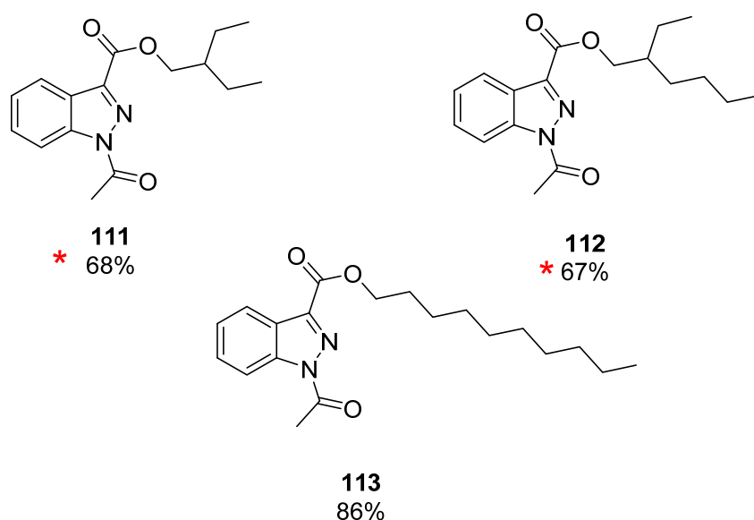
Figure 2.16 Extending the length of the ester side chains
