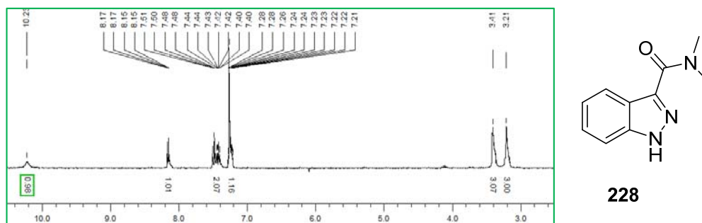
Figure 2.57 ^1\text{H} NMR spectrum of 228
