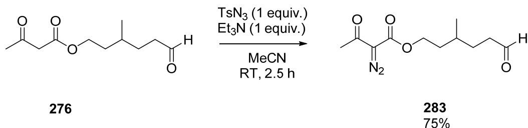
Scheme 2.66
