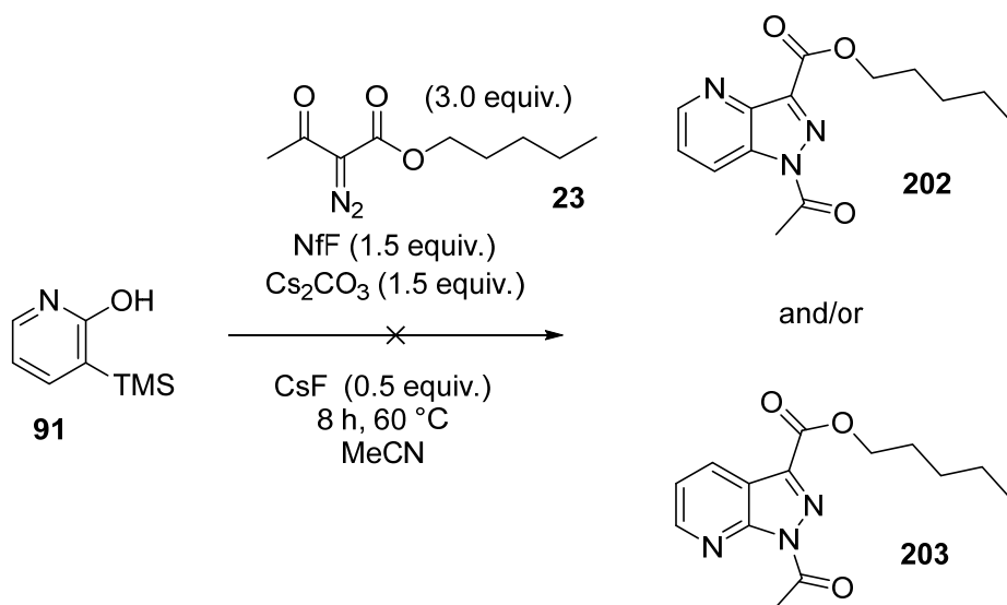
Scheme 2.46
