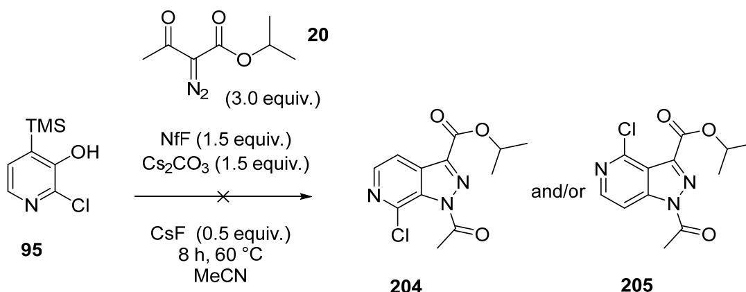
Scheme 2.47
