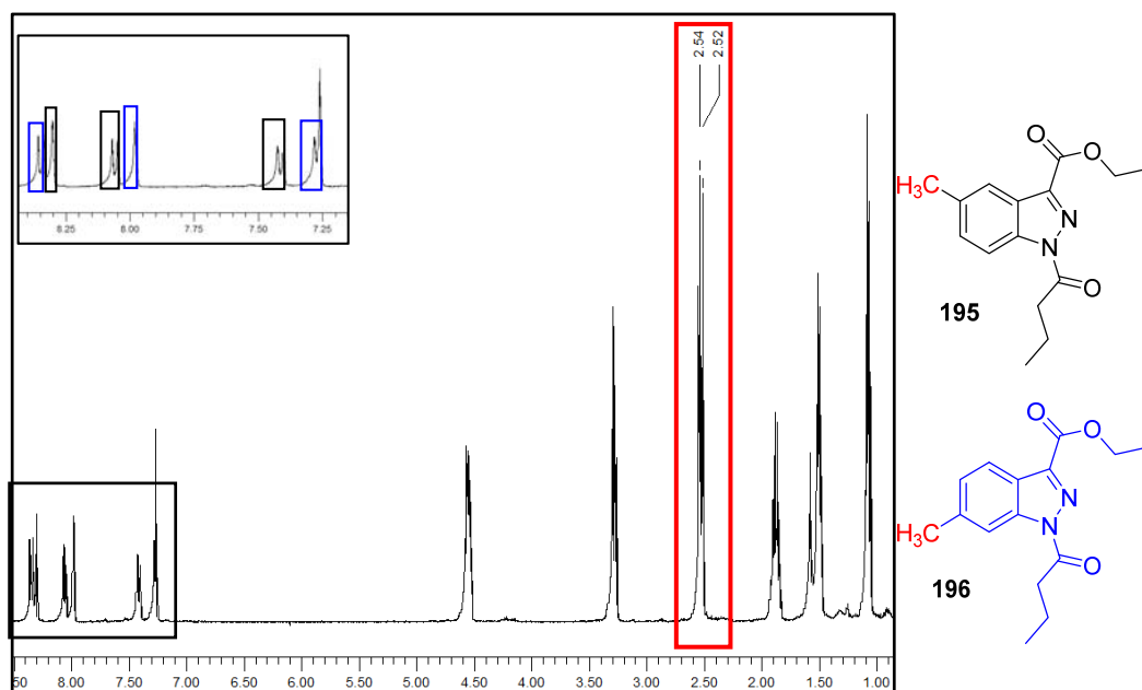
Figure 2.49 1 H NMR spectra of 195/196
