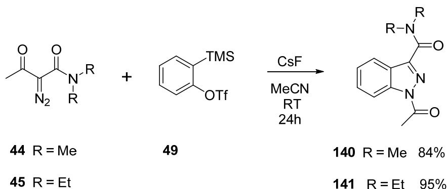
Scheme 2.32
