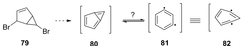
Scheme 1.21
