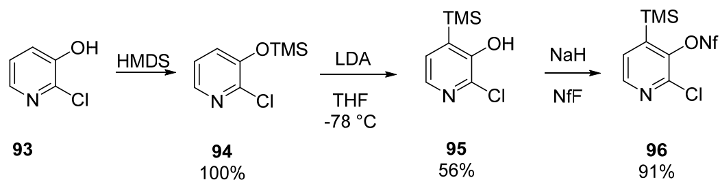
Scheme 2.20
