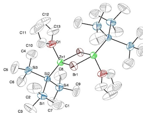
Figure 1. Perspective views of 2 with thermal ellipsoids at the 50% level. Selected bond lengths (Å) and angles (deg): Zn-Br 2.5030(6), Zn-Br' 2.5382(6), Zn-Si2 2.352(1), Zn-O1 2.101(3), Zn-Br-Zn' 81.16(2), Br-Zn-Br' 93.84(2), Br-Zn-Si2 124.52(3), Br-Zn-Br' 121.70(3), Br-Zn-O 96.88(9), Br'-Zn-O 94.56(9).
