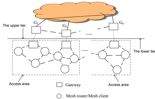
Fig. 4. An example of the two-tier integrated architecture .
