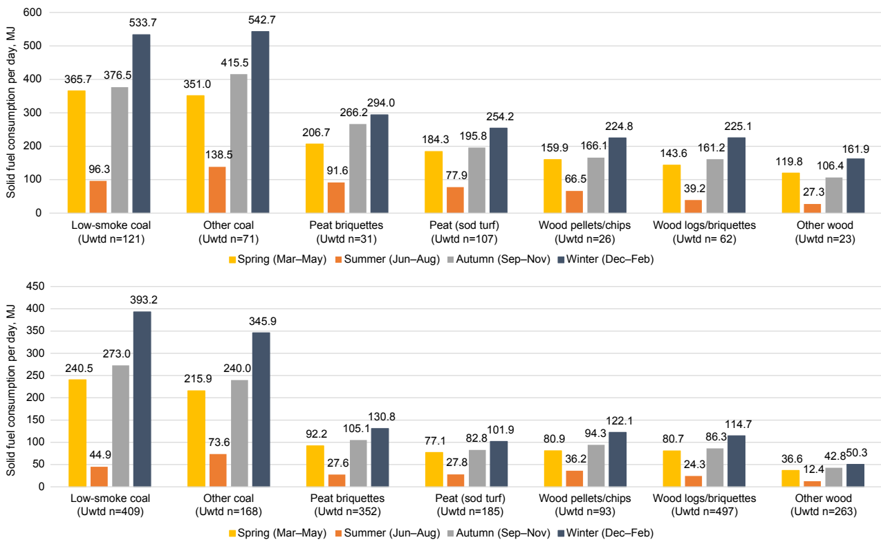
Figure 3.5. Average daily household consumption of individual solid fuels by season and by primary (top) and supplementary (bottom) solid fuel user (MJ).
