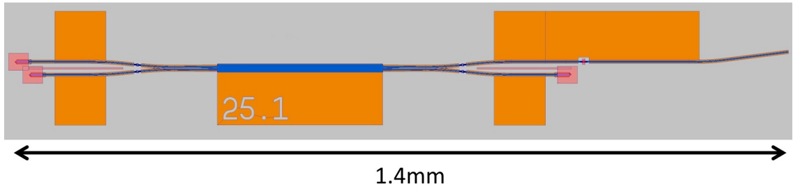
Figure 5.3: Schematic of a second generation 2x2 MMI slotted laser with \Delta L = 25\mu\text{m} and k = 1 - the slot is placed on the output arm to increase feedback and to modify the reflection profile
