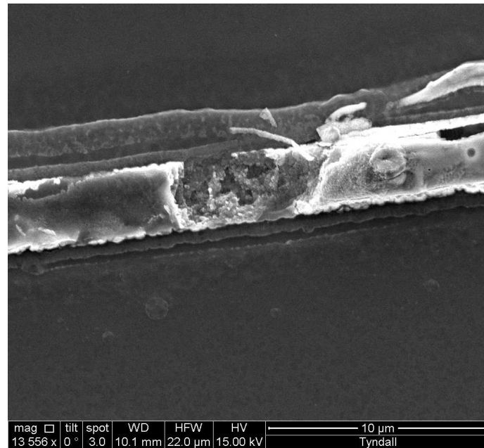
Figure 3.21: SEM picture of a ridge damaged by excessive current density
