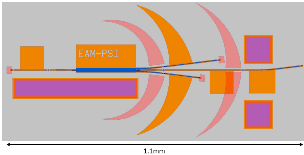
Figure 8.3: Schematic of a proposed intra-cavity reflector of width 1.35\mu\text{m}
