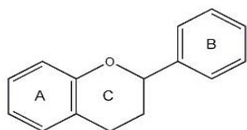
Figure 1. Structure of a typical flavonoid consisting of A, B and C ring.
