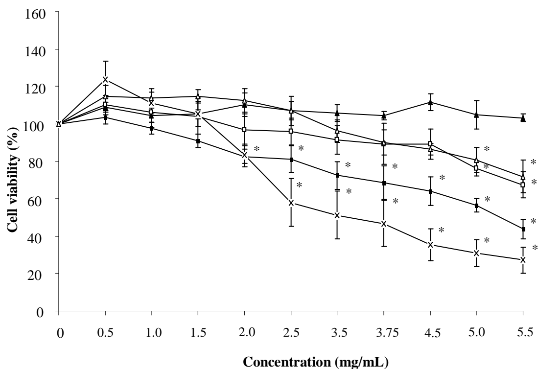
Figure 1. Viability of Caco-2 cells following addition of increasing levels (mg/mL) of Ascophyllum nodosum (-■-), Laminaria hyperborea (-▲-), Pelvetia canaliculata (-□-), Fucus vesiculosus (-×-) and Fucus serratus (-Δ-). Data are the means of four independent experiments, with standard errors represented by vertical bars. * Mean value was significantly different from that of control cells ( P < 0.05 ). n = 4 independent experiments.
