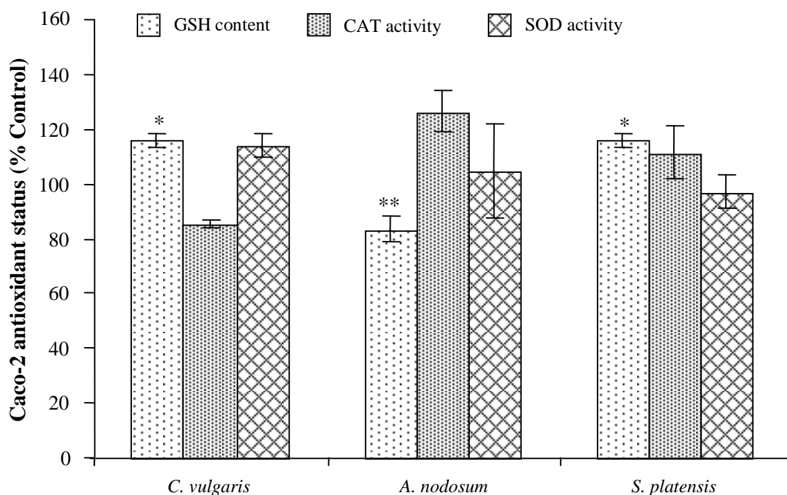
Figure 2: GSH content, catalase and superoxide dismutase activity in Caco-2 cells supplemented with methanolic extracts of Chlorella vulgaris , Ascophyllum nodosum and Spirulina platensis for 24 hrs. Data are the means of three independent experiments, with standard errors represented by vertical bars. ** Mean value was significantly different from that of the control ( P < 0.01 ), * Mean value was significantly different from that of the control ( P < 0.05 ), ANOVA followed by Dunnett's test.
