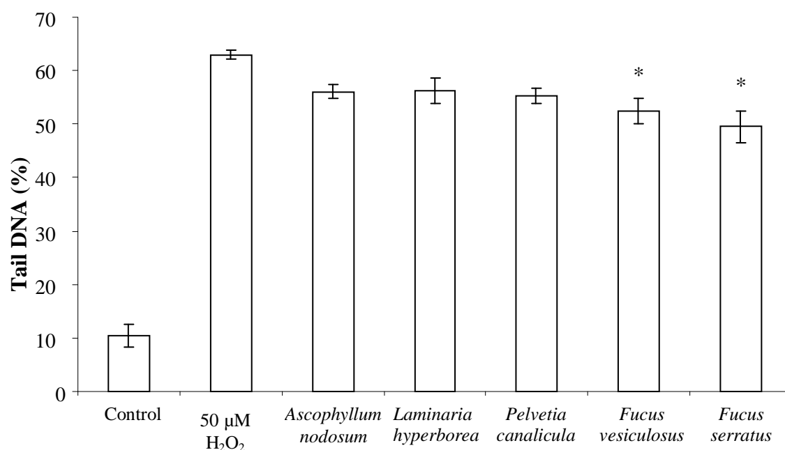
Figure 2. DNA damage in Caco-2 cells following pre-treatment with or without seaweed extracts (100 µg/mL) for 24 hrs then exposed to 50 µM -H 2 O 2 for 30 mins at 37°C. DNA damage was assessed by the comet assay (explained earlier) in which % tail DNA was measured. Data are the means of four independent experiments, with SEM represented by vertical bars. Statistical analysis was by repeated measures ANOVA followed by the Dunnett's test. Mean value was significantly different from that for H 2 O 2 -challenged cells ( P < 0.05 ). n = 4 independent experiments.
