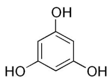
Figure 3. Structure of phloroglucinol.
