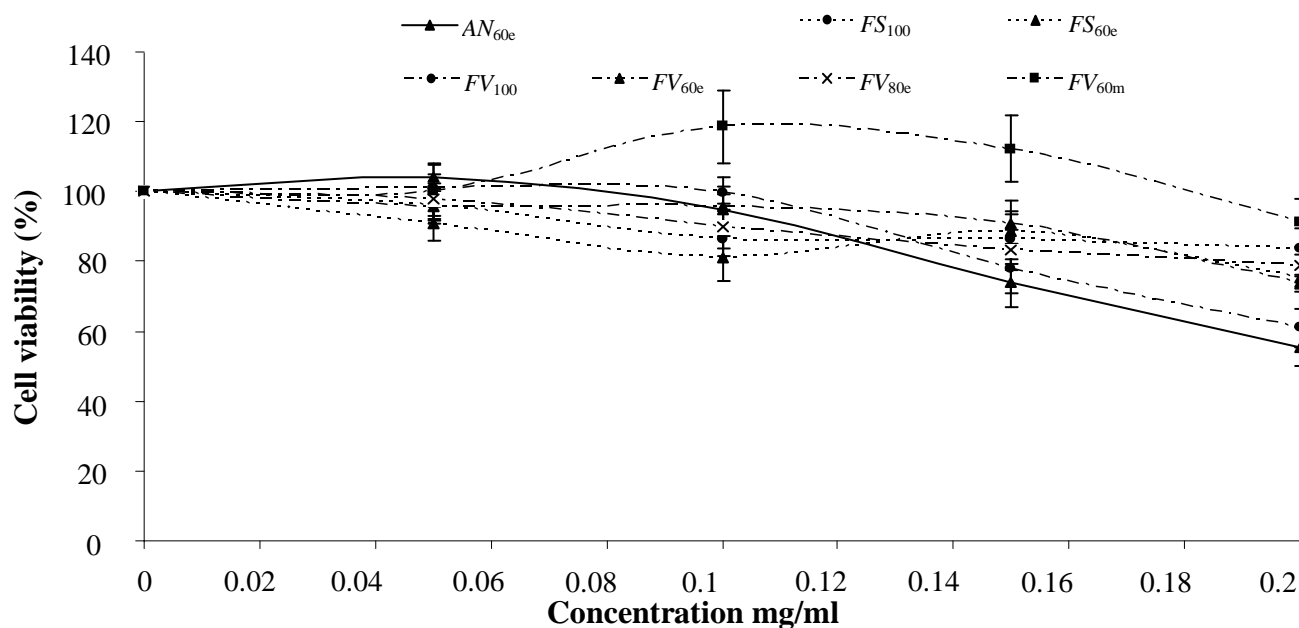
Figure 1A & B: Viability of Caco-2 cells following addition of increasing concentrations (0-2 mg/ml [A] or (0-0.2 mg/ml [B]) of seaweed extracts as determined by the MTT assay. A. nodosum is represented by (—), F. serratus is represented by (.....). F. vesiculosus is represented by (- · -). Solvents are represented as follows: H 2 O- ● (AN 100 , FS 100 , FV 100 ), 60% EtOH- ▲ (AN 60e , FS 60e , FV 60e ), 80% EtOH- × (AN 80e , FS 80e , FV 80e ), 60% MeOH- ■ (AN 60m , FS 60m , FV 60m ). Data are the means of four independent experiments, with standard errors represented by vertical bars. * Denotes that mean value was significantly different from that of control cells ( P < 0.05 ), n=4 independent experiments.
