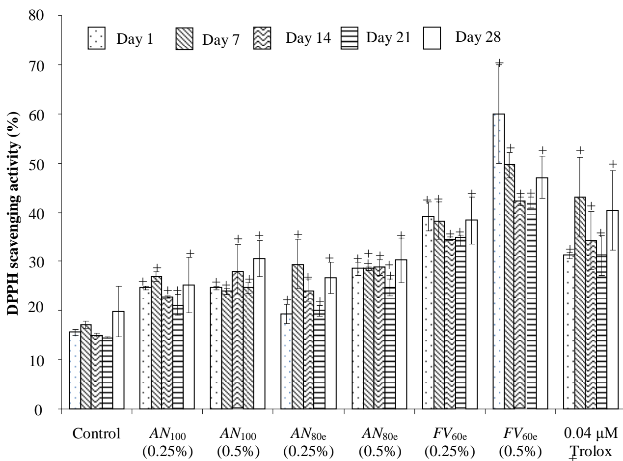
Figure 4. The DPPH-scavenging activity stability of yogurt samples over 28 days storage at 4°C. Data are the means of four independent experiments, with standard errors represented by vertical bars. + denotes significantly higher ( P < 0.05 ) DPPH radical scavenging activity, on each measurement day, between seaweed extract enriched yogurt samples and the corresponding controls.
