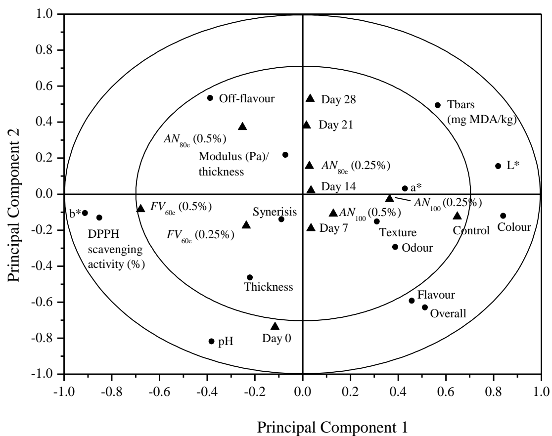
Figure 3. APLSR for the various seaweed-enriched yogurts. ▲=Yogurt sample, ●=sensory descriptor, chemical and instrumental variables. The concentric circles represent 100% and 50% explained variance, respectively.
