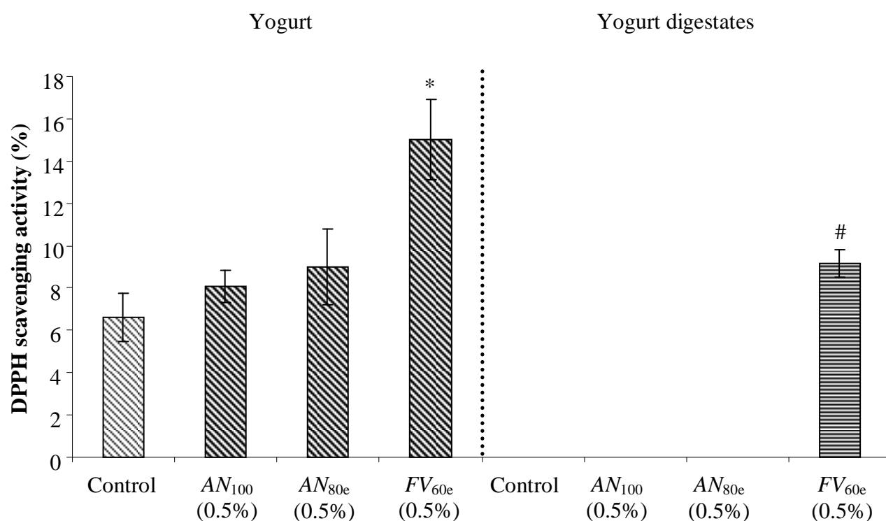
Figure 5. The DPPH-scavenging activity of yogurt samples before and after an in-vitro digestion procedure. Data are the means of four independent experiments, with standard errors represented by vertical bars. * denotes significantly higher DPPH scavenging activity values compared to other yogurt samples as determined using repeated measures ANOVA followed by Tukey's post-test. # denotes significantly different DPPH scavenging activity values compared to other digested yogurt samples
