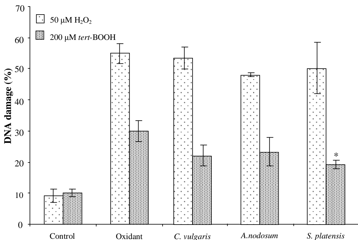
Figure 2: DNA damage in Caco-2 cells, expressed as percent tail DNA. Cells were incubated with methanolic extracts of Chlorella vulgaris , Ascophyllum nodosum and Spirulina platensis for 24 hrs, media was removed and replaced with media containing 50 \mu\text{M} \text{H}_2\text{O}_2 or 200 \mu\text{M} tert -BOOH for a further 30 mins. Data are the means of four independent experiments, with standard errors represented by vertical bars. * Mean value was significantly different from that for \text{H}_2\text{O}_2 or tert -BOOH, ANOVA followed by Dunnett's test.
