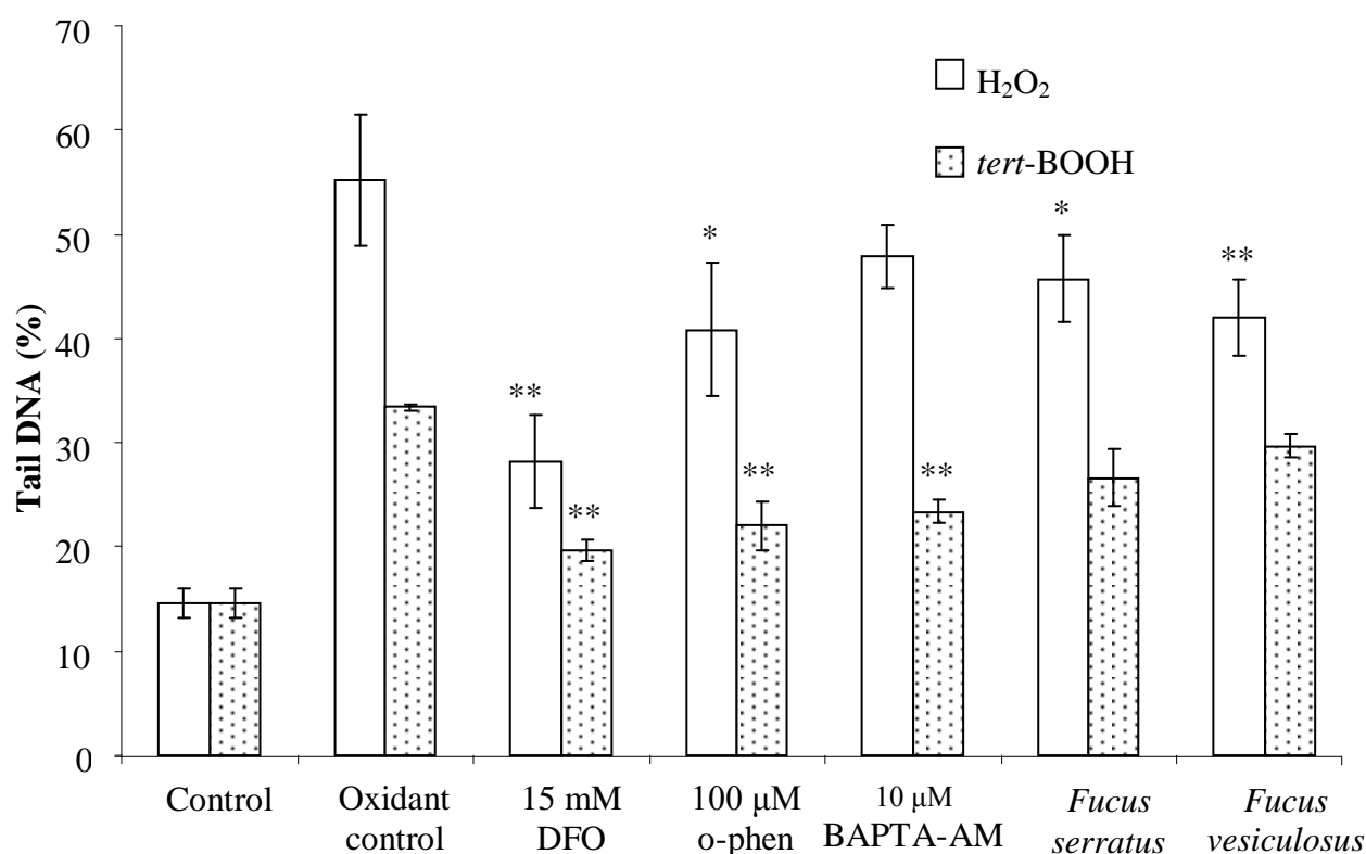
Figure 2: DNA damage in Caco-2 cells, expressed as percent tail DNA. Cells were incubated with metal chelators, 15 mM desferoxamine mesylate, 100 \mu M 1,10-phenanthroline, 10 \mu M BAPTA-AM for 30 mins or seaweed extracts Fucus serratus or Fucus vesiculosus for 24 hrs, media was removed and replaced with media containing 50 \mu M H 2 O 2 [□] or 200 \mu M tert-BOOH [▤] for a further 30 mins. Statistical analysis was by repeated measures ANOVA followed by the Dunnett's test. * Mean value was significantly different from that for H 2 O 2 or tert-BOOH -challenged cells ( P < 0.05 ). ** Mean value was significantly different from that for H 2 O 2 or tert-BOOH -challenged cells ( P < 0.01 ).
