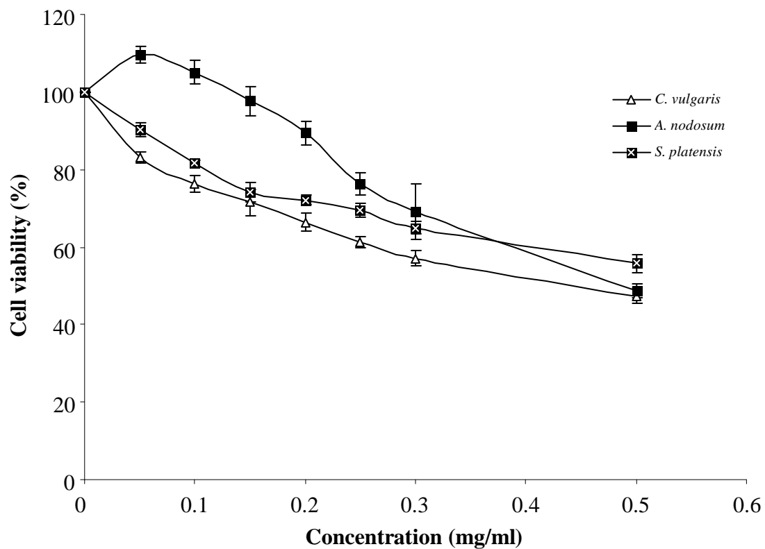
Figure 1: Viability of Caco-2 cells following addition of increasing levels (mg/ml) of Chlorella vulgaris (-Δ-), Ascophyllum nodosum (-■-) and Spirulina platensis (×) at concentrations ranging from 0.05-0.5 mg/ml. Data are the means of six independent experiments, with standard errors represented by vertical bars.
