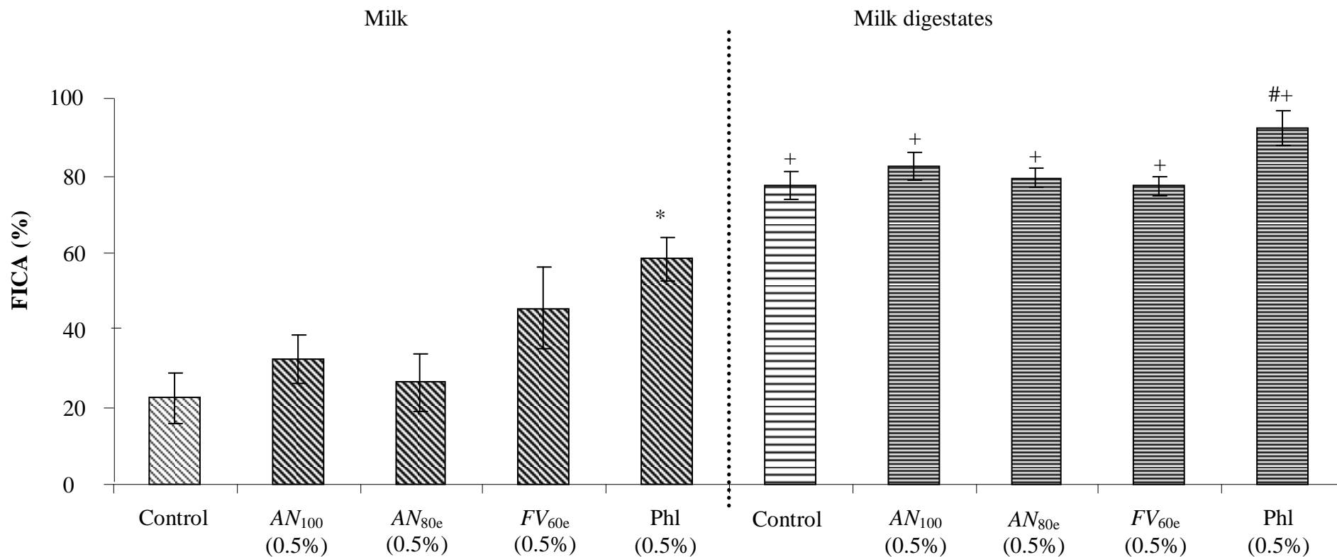
Figure 4. The ferrous-ion chelating activity (FICA) (%) of milk samples before and after an in-vitro digestion procedure. Data are the means of four independent experiments, with standard errors represented by vertical bars. * and # denotes significantly higher FICA between milk samples and milk digestates, respectively. + denotes significantly different FICA between different a milk sample and its corresponding digestate.
