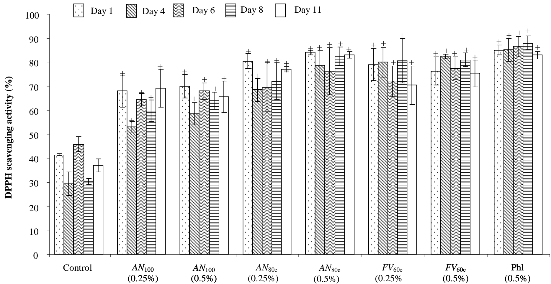
Figure 2. The DPPH-scavenging activity % (stability) of milk samples over 11 days storage at 4°C. Data are the means of three independent experiments, with standard errors represented by vertical bars. + denotes significantly higher ( P < 0.05 ) DPPH radical scavenging activity, on each measurement day, between seaweed extract enriched milk samples and the corresponding controls.
