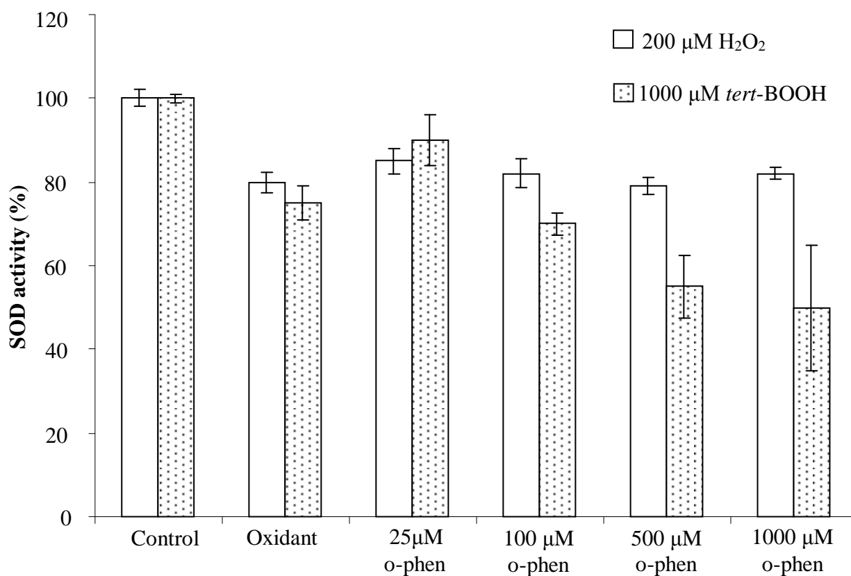
Figure 1: SOD activity, expressed as a percentage of the control value. Caco-2 cells were exposed to 200 µM H 2 O 2 [□] or 1000 µM tert -BOOH [▤] for 30 mins following a preincubation with metal ion chelator, 1,10-phenanthroline for 24 hrs. Statistical analysis was by repeated measures ANOVA followed by the Dunnett's test.
