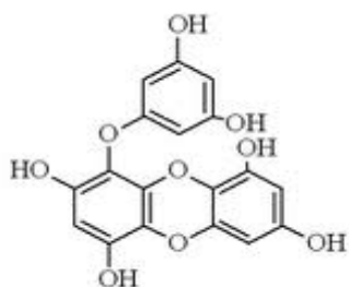
Figure 4. Structure of eckol.
