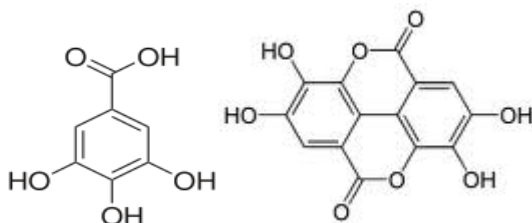
Figure 2. Structures of gallic acid and ellagic acid.
