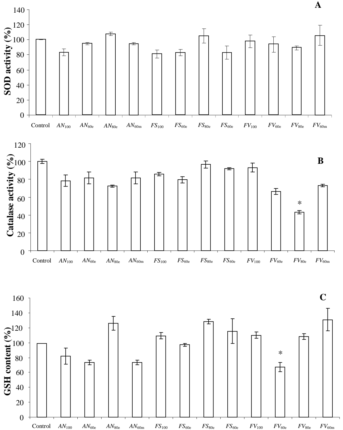
Figure 2: SOD activity (A), catalase activity (B) and GSH content (C) in Caco-2 cells following 24 hrs incubation with seaweed extracts, expressed as a percentage of the control value. Statistical analysis was by repeated measures ANOVA followed by the Dunnett's test. * Denotes that mean value was significantly different from that of control cells ( P < 0.05 ), n=4 independent experiments.
