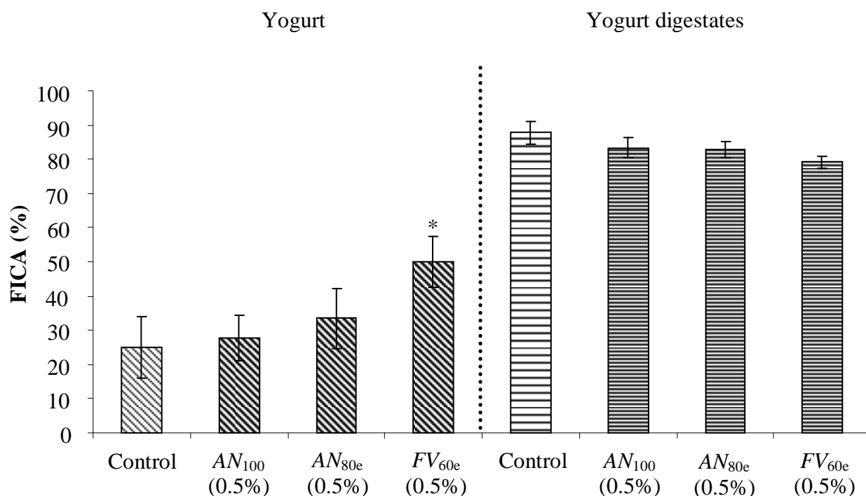
Figure 6. The ferrous-ion chelating activity (FICA) of yogurt samples before and after an in-vitro digestion procedure. Data are the means of four independent experiments, with standard errors represented by vertical bars. * denotes significantly different FICA values compared to other samples as determined using repeated measures ANOVA followed by Tukey's post-test.
