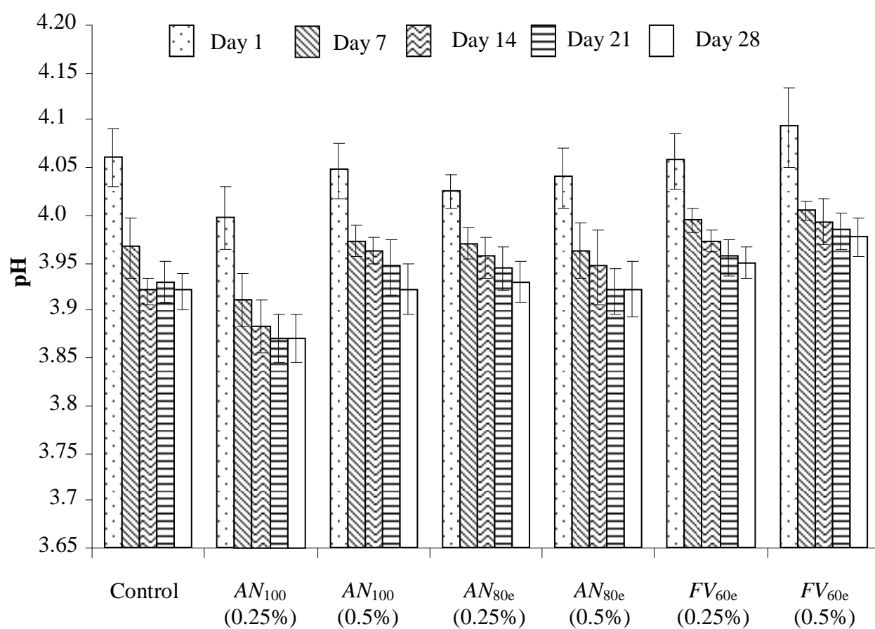
Figure 1. pH change in yogurt samples over 28 days storage at 4°C. Data are the means of four independent experiments, with standard errors represented by vertical bars. Statistical analysis was by one-way ANOVA followed by the Tukey's test. No significant differences between treatment means on each measurement day ( P > 0.05 ).
