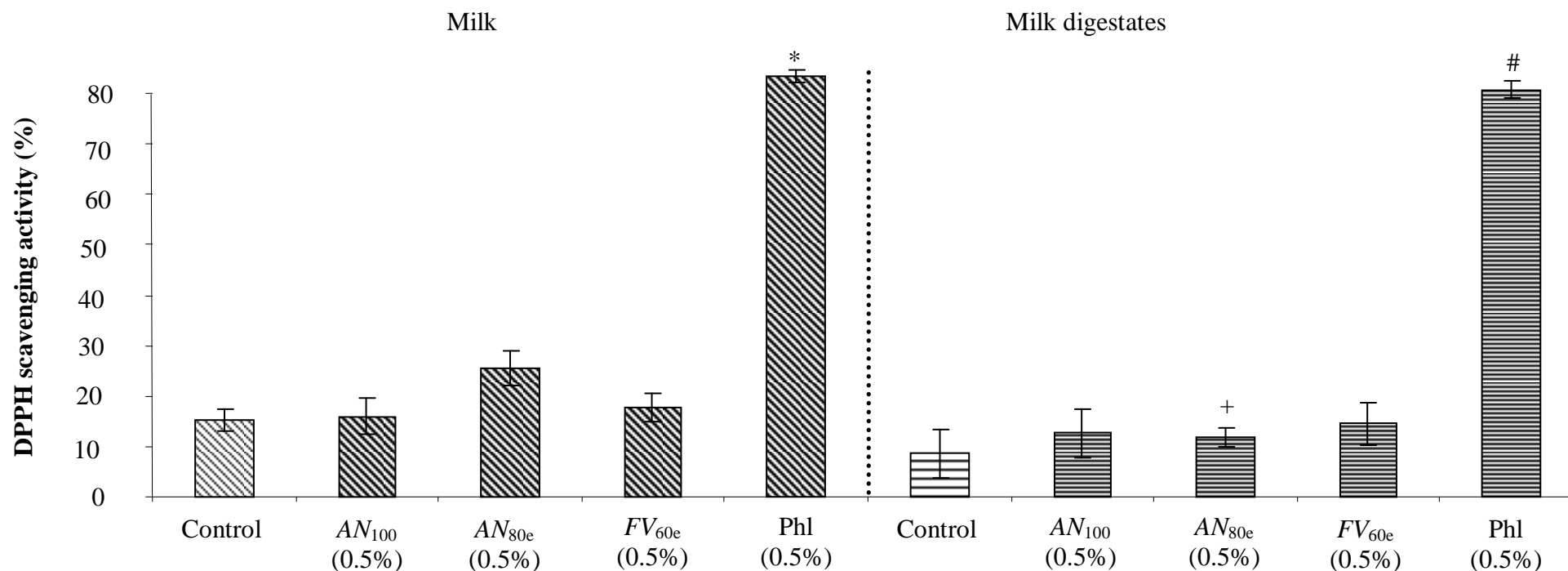
Figure 3. The DPPH-scavenging activity of milk samples before and after an in-vitro digestion procedure. Data are the means of four independent experiments, with standard errors represented by vertical bars and determined using repeated measures ANOVA followed by Tukey's post-test. * and # denotes significantly higher DPPH scavenging activity values between milk samples and milk digestates, respectively. + denotes significant different DPPH scavenging activity values between different a milk sample and its corresponding digestate.
