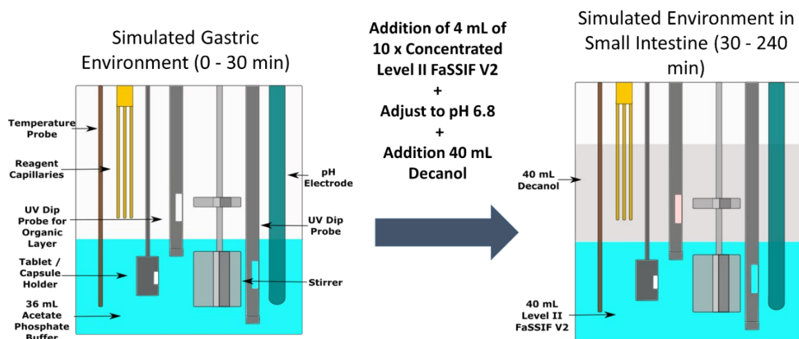
Figure 2: Schematic of the biphasic dissolution test using the inForm platform. Adapted from O'Dwyer et al. [39]
