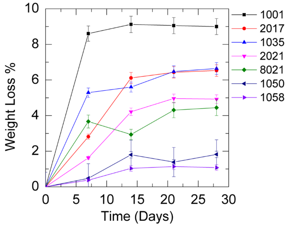
FIGURE 5. Standardized weight loss for 8 composites from all Experimental Design series under C1 assay.
