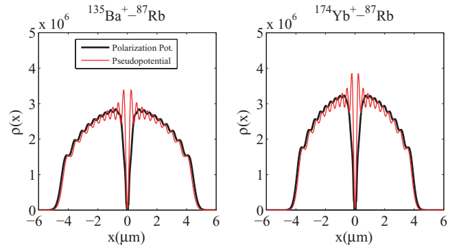
FIG. 3. (Color online) The single-particle densities of a TG gas of 20 particles in the presence of a central ion for ^{135}\text{Ba}^+ - ^{87}\text{Rb} and ^{174}\text{Yb}^+ - ^{87}\text{Rb} systems with a typical trapping frequency, \omega = 70\text{Hz} (thick black line). The short range phases in each case are chosen to be \phi_e = \frac{\pi}{4} and \phi_o = -\frac{\pi}{4} . The thin red line in the plots represents the result of a pseudopotential approximation for the ion, using a large value for the scattering length.
