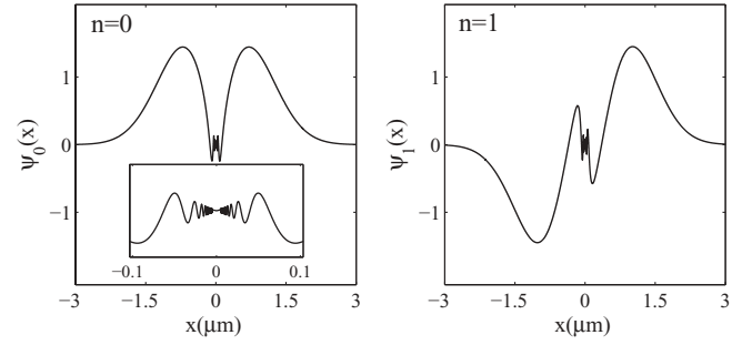
FIG. 2. The first two trap states of a harmonic trap with a centrally embedded ion for a ^{135}\text{Ba}^+ - ^{87}\text{Rb} system for axial trapping frequency, \omega = 70\text{Hz} . The inset for the n = 0 state shows a zoom in of the region around zero where the wave function is rapidly oscillating. The short-range phases are chosen to be \phi_e = \frac{\pi}{4} and \phi_o = -\frac{\pi}{4} .
