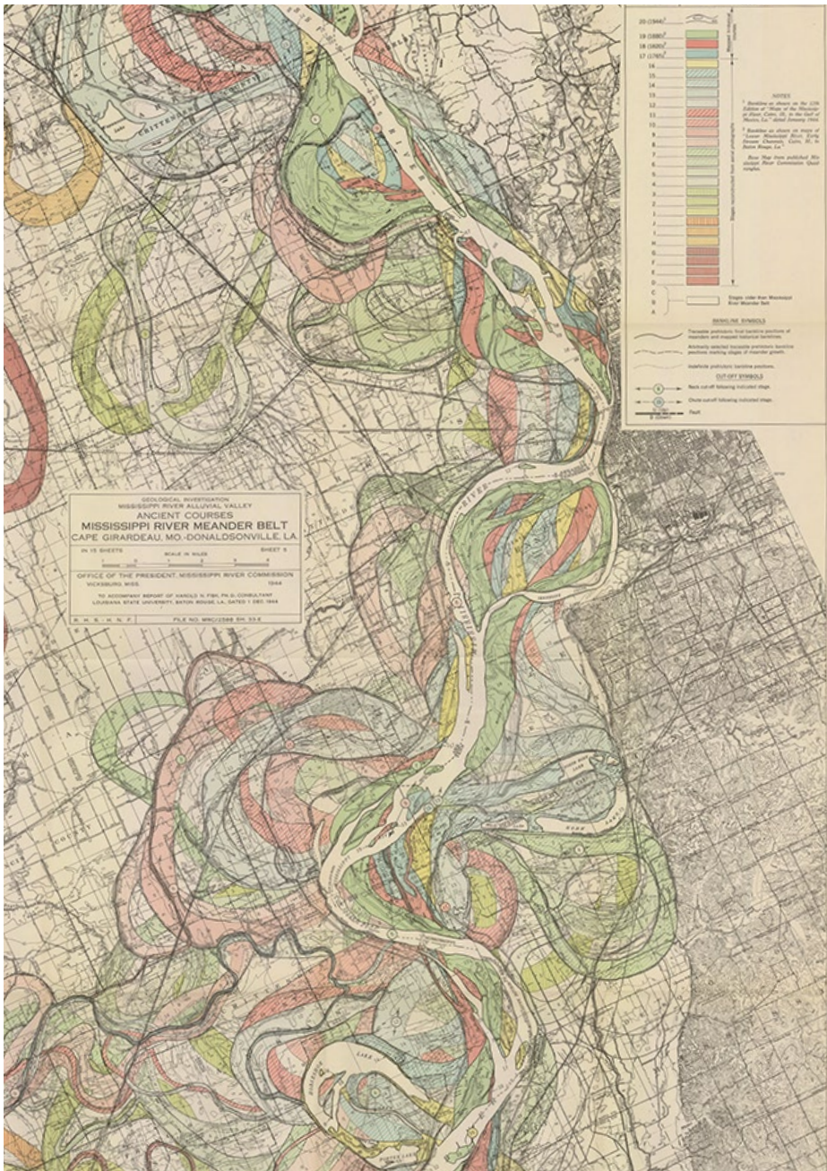
Fig. 01 Harold Norman Fisk, Geological Investigation of the Alluvial Valley of the Lower Mississippi River (Vicksburg, Miss.: 1945), M.R.C. print. Plate 22-5.
