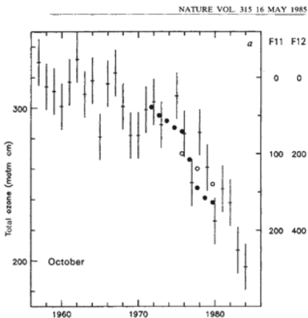
Fig. 05 J. C. Farman, B. G. Gardiner and J. D. Shanklin, “Large Losses of Total Ozone in Antarctica Reveal Seasonal \text{ClO}_x/\text{NO}_x Interaction,” Nature 315 (May 1985): 207–210.
