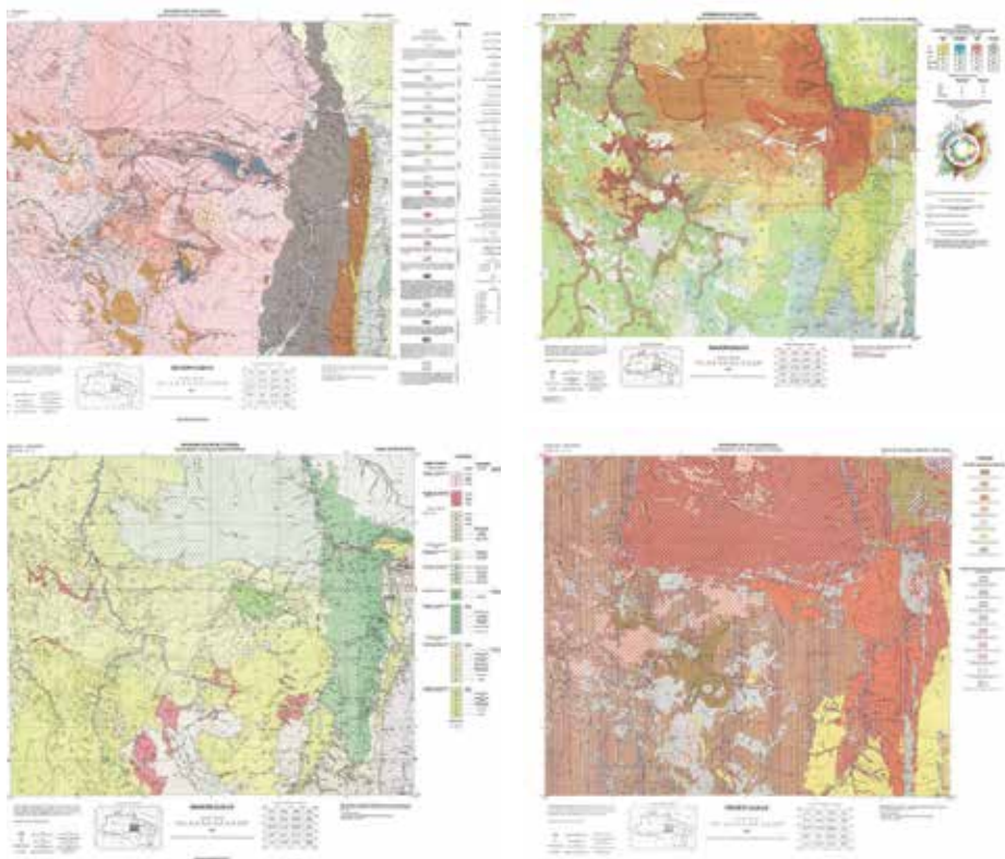
Deep terrain: Samples of the cartographic inventory produced by RADAM on the region between the Xingu and Araguaia Rivers, southern tributaries of the Amazon. Respectively, the maps describe geology, land potential, phytogeography, and agricultural suitability. Fig. 06 – Fig. 09
