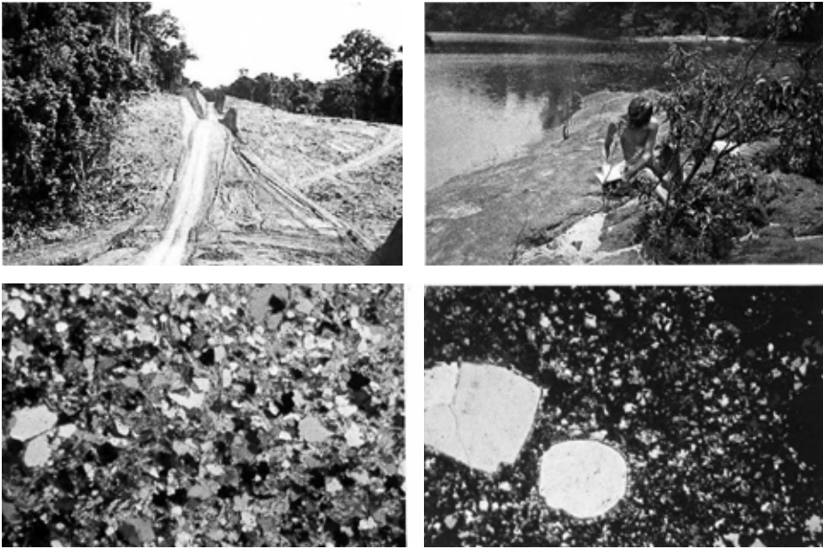
Fig. 12 – Geological taxonomy : Sample images of the RADAM catalogue describing field-work research used for the geological classification of soil profiles in Amazonia. Fig. 15
