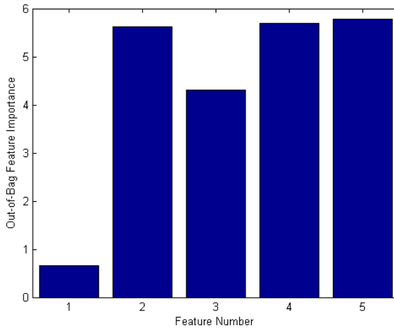
Figure 5.8 – Feature importance
