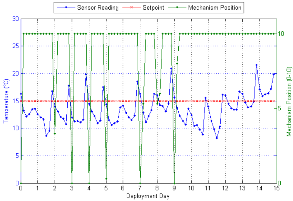
Figure 4.8 – Simulated PID response to Deployment IV
