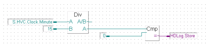
Figure 4-8 FUPLA clock programming
