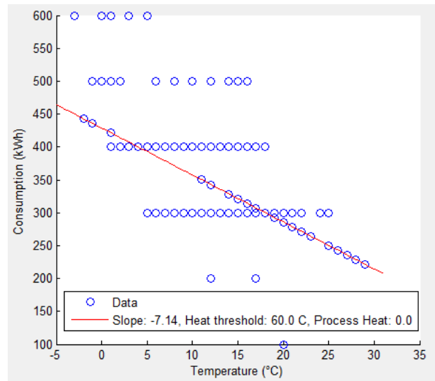
Figure 4-22 Failed heat curve
