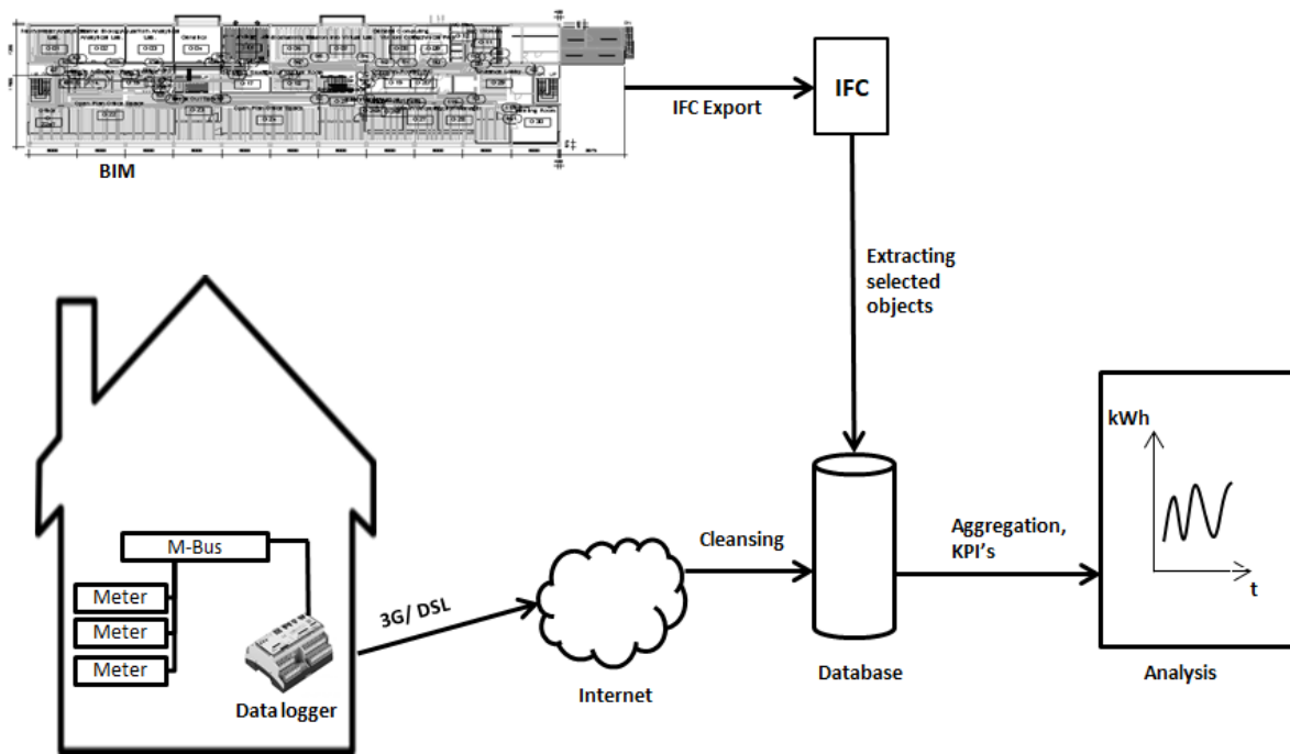
Figure 3-40 Computing architecture
