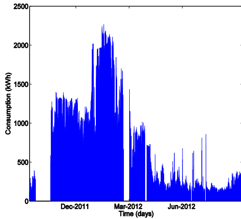
Figure 4-16 Raw gas consumption
