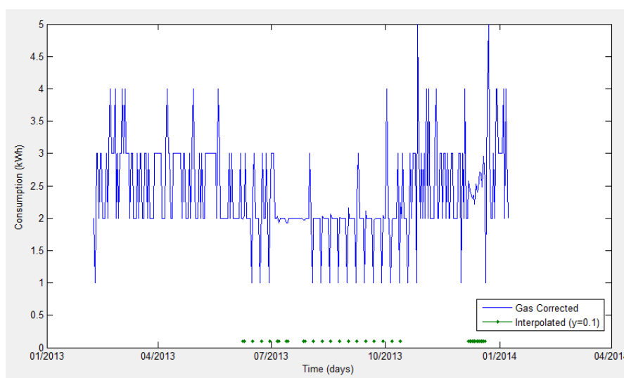
Figure 4-13 Corrected gas consumption
