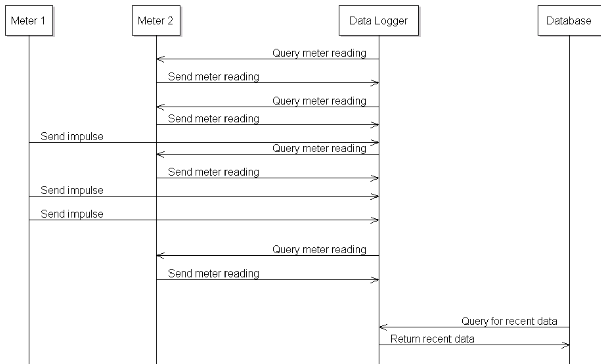
Figure 2-3 Data logger sequence diagram
