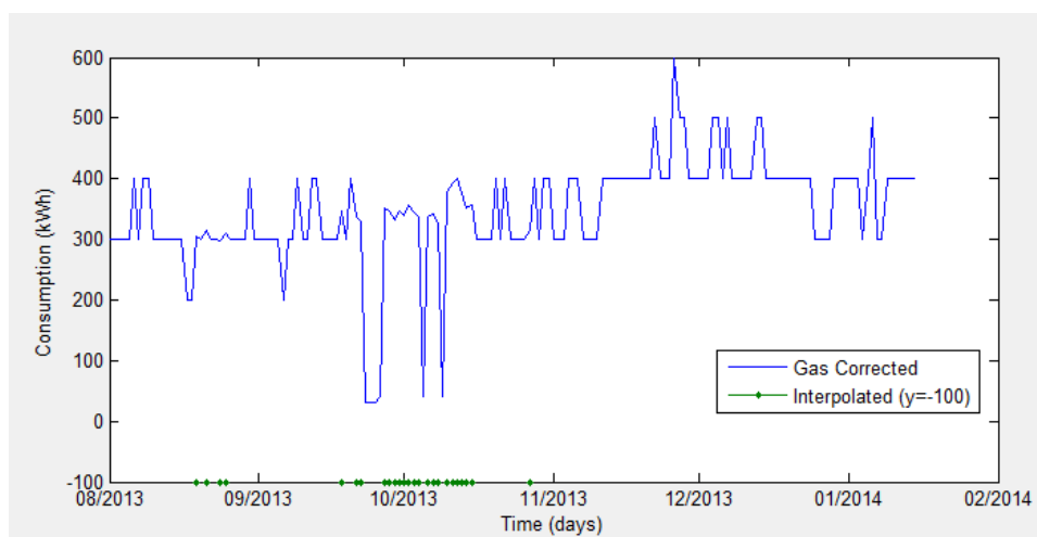
Figure 4-21 Cleansed raw consumption
