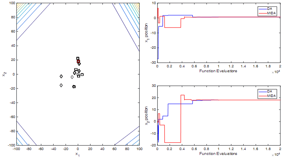
Figure 9: Trajectory of elite dragonfly for the FN15 benchmark function ( \diamond : DA, \square : MIDA).
