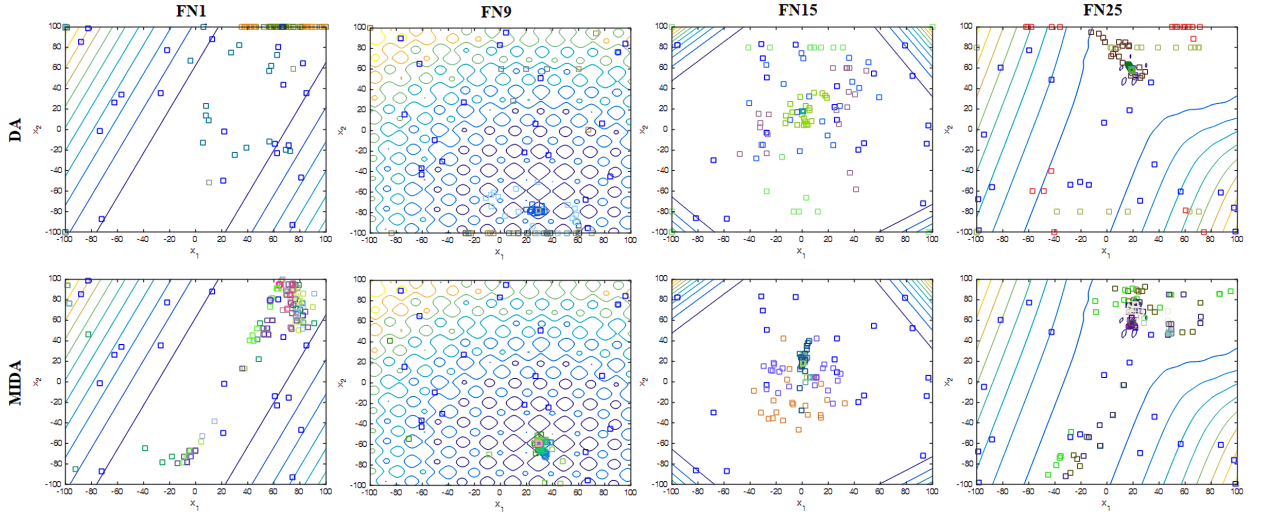
Figure 6: Search history analysis results of the MIDA and DA.
