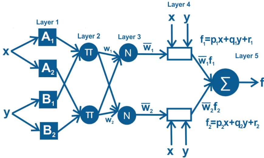
Figure 3: General ANFIS model architecture [72]
