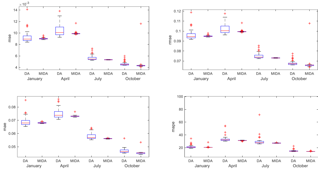
Figure 21: Distribution of ANFIS model error metrics in test phase using DA and MIDA
