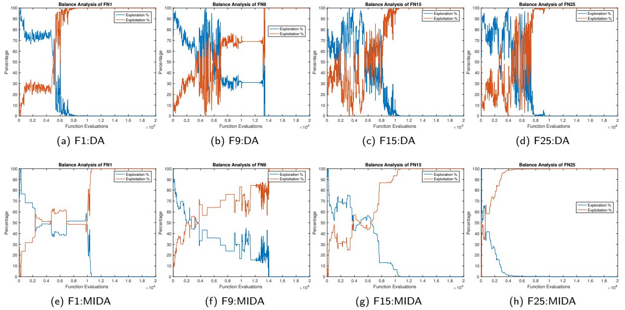
Figure 13: Balance analysis results of the MIDA and DA.
