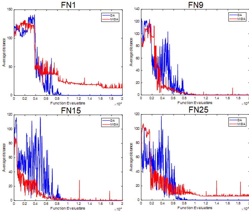
Figure 11: Average distance analysis of dragonflies
