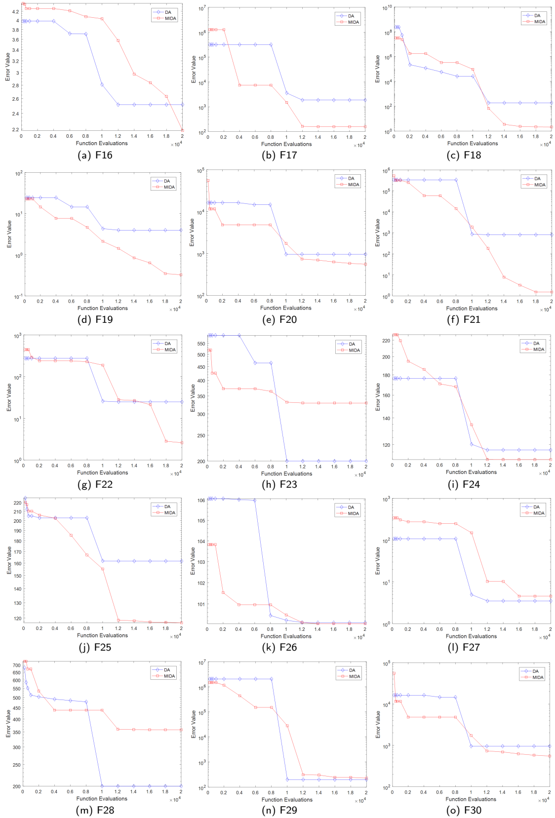
Figure 15: Convergence curves of the MIDA and DA for F16-F30 functions.
