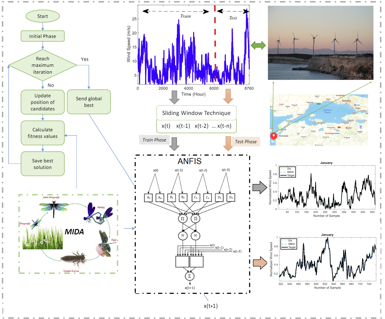
Figure 16: The structure of the ANFIS and MIDA hybrid forecasting model.
