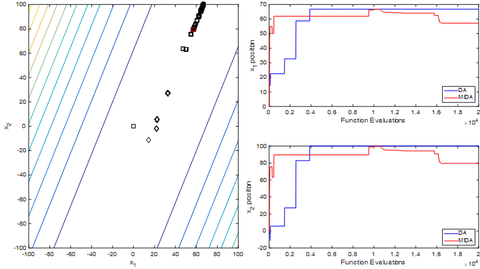
Figure 7: Trajectory of elite dragonfly for the FN1 benchmark function ( \diamond : DA, \square : MIDA).
