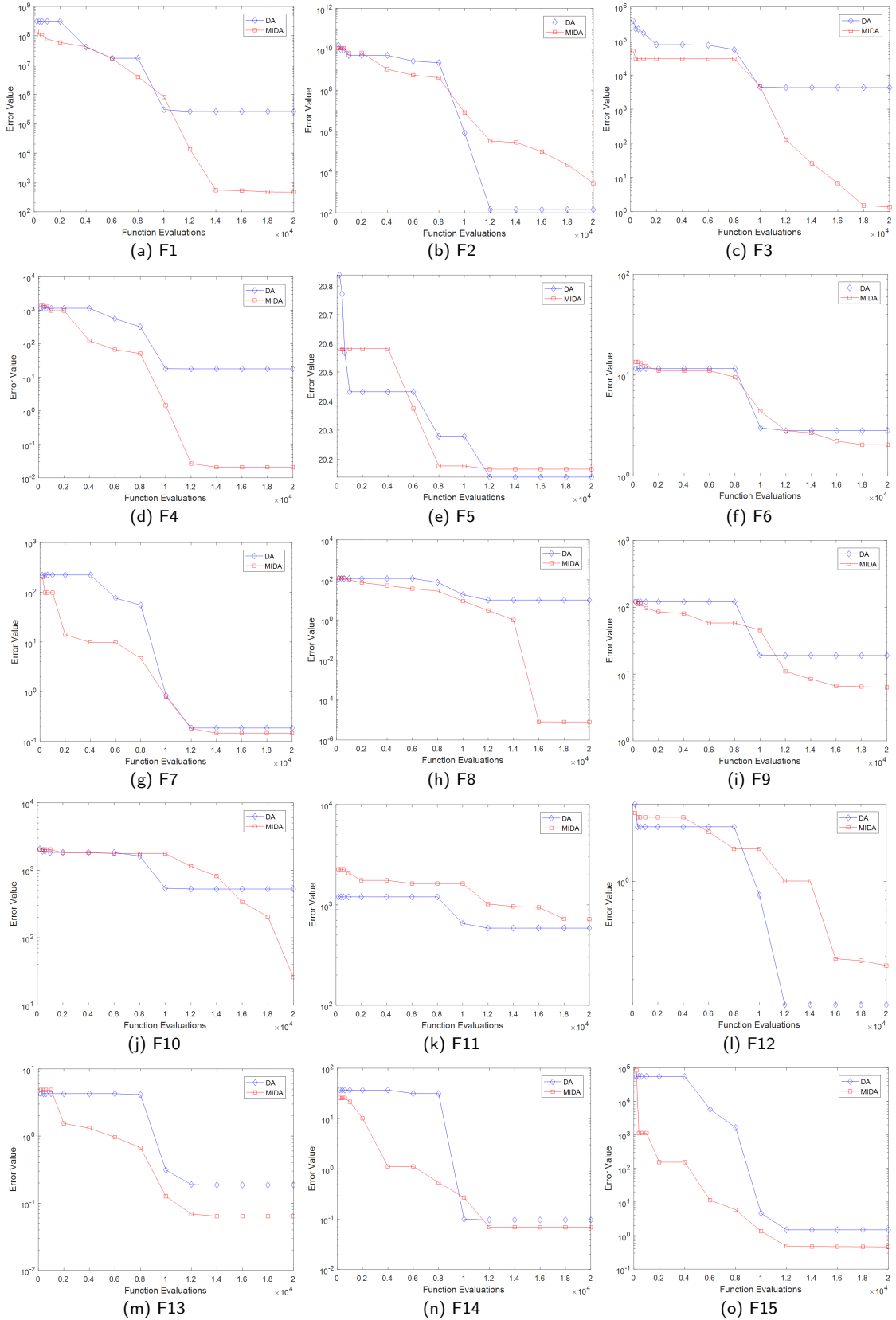
Figure 14: Convergence curves of the MIDA and DA for F1-F15 functions.
