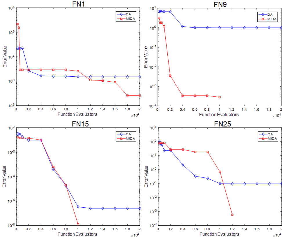
Figure 5: Convergence analysis results of the proposed MIDA and DA.
