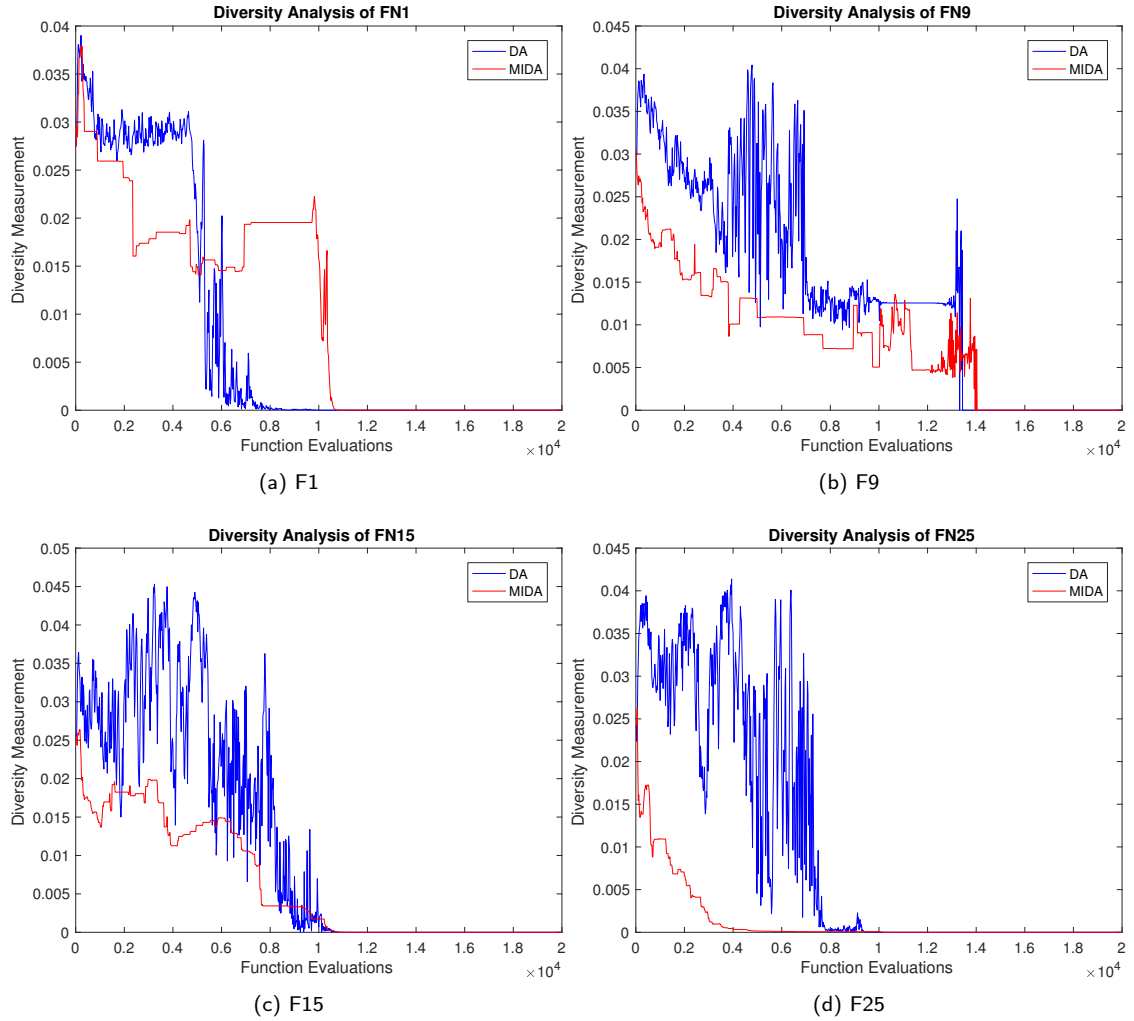
Figure 12: Diversity analysis results of the MIDA and DA.
