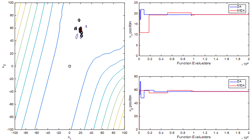
Figure 10: Trajectory of elite dragonfly for the FN25 benchmark function ( \diamond : DA, \square : MIDA).
