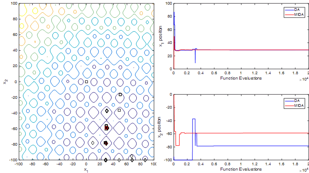
Figure 8: Trajectory of elite dragonfly for the FN9 benchmark function ( \diamond : DA, \square : MIDA).
