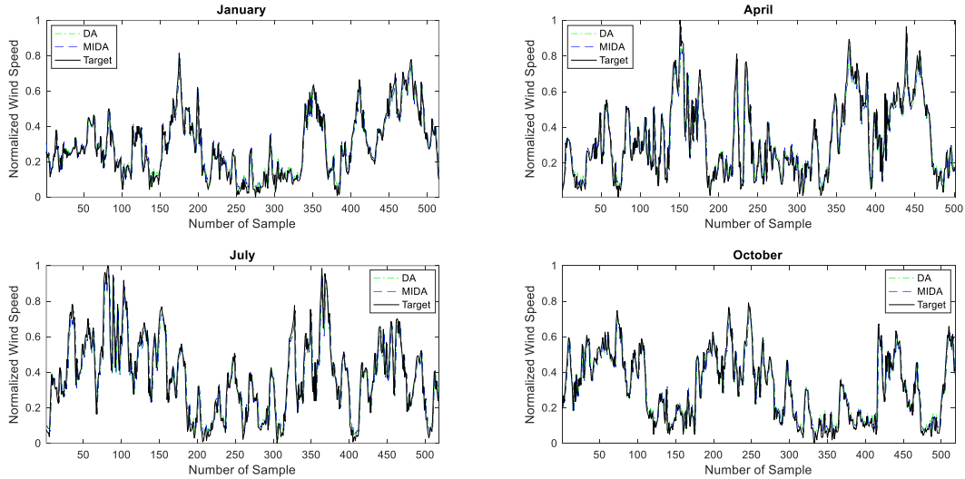
Figure 18: Training results for the best ANFIS parameters as obtained by DA and MIDA in 50 runs.
