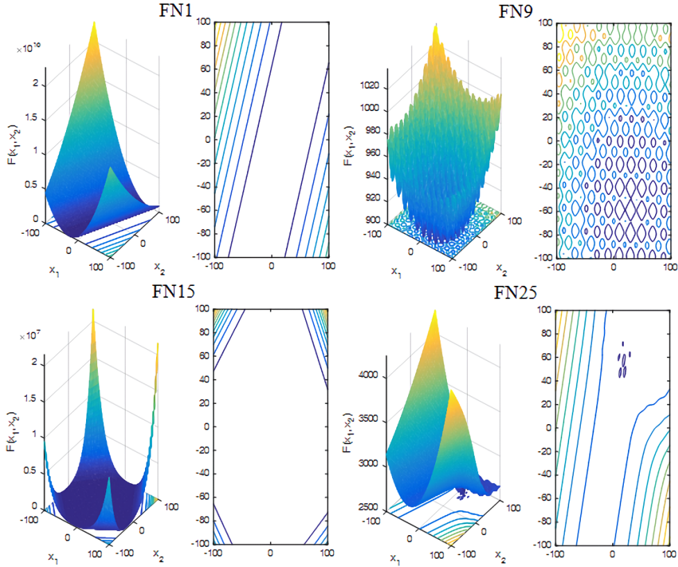
Figure 4: Unimodal, multimodal and composition benchmark functions used for performance analysis of the proposed MIDA
