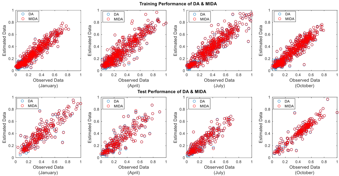
Figure 20: Scatter results for the best ANFIS parameters as obtained by DA and MIDA in 50 runs.
