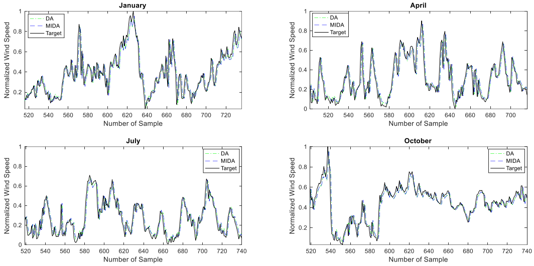
Figure 19: Test results for the best ANFIS parameters as obtained by DA and MIDA in 50 runs.
