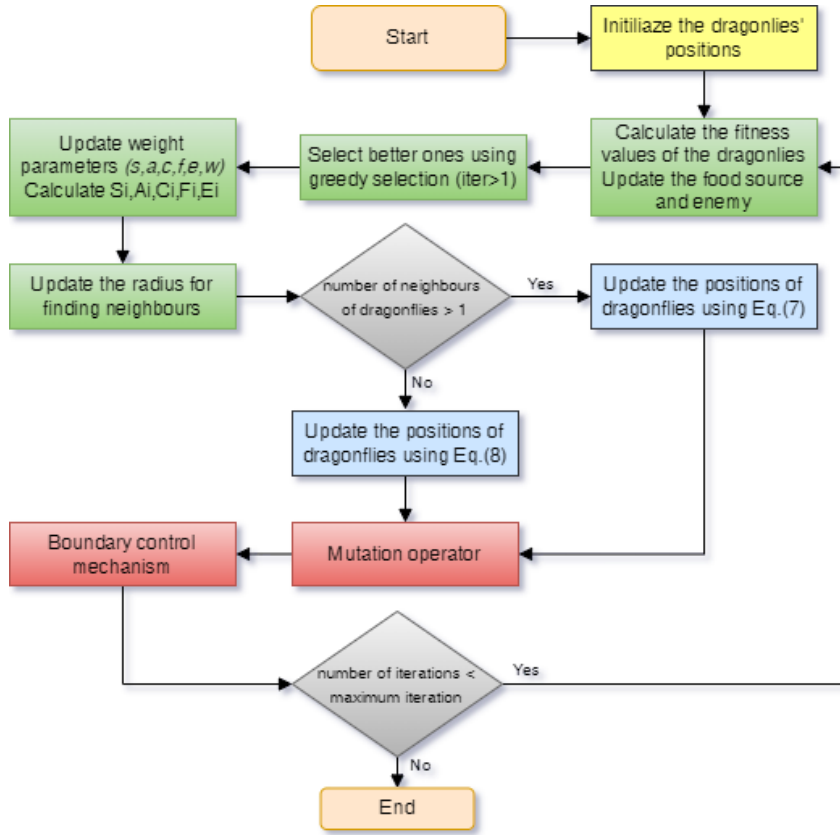
Figure 2: Flowchart of MIDA
