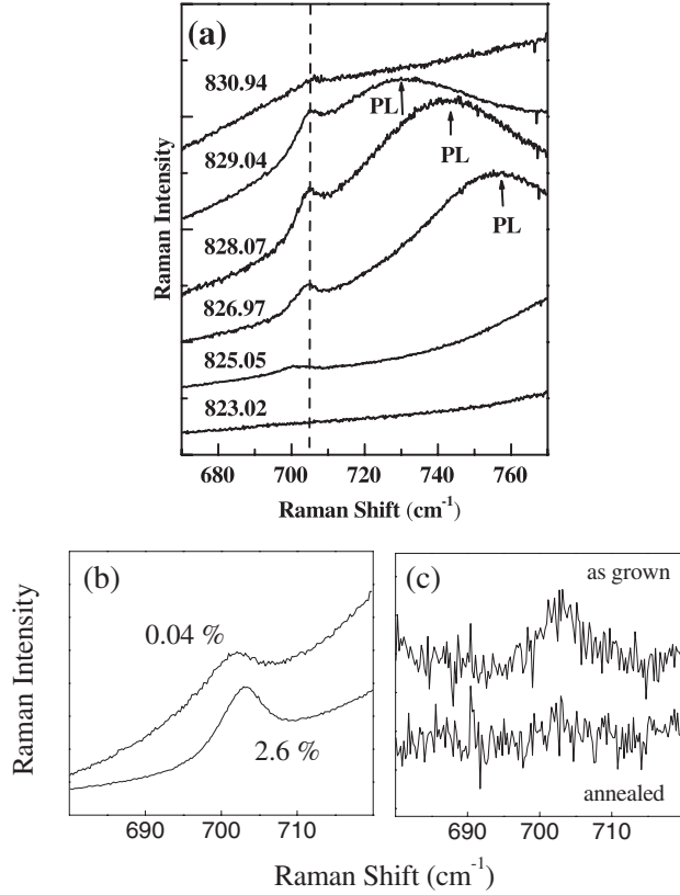
FIG. 1. (a) Data for the 1.4% Mn sample. The dashed line indicates the position of the 1S_{3/2} \rightarrow 2S_{3/2} acceptor transition. Numbers on the left indicate the laser wavelength, \lambda_L , in nm. The broad peak, PL, is due to e - A^0 photoluminescence. (b) Data at two, PM (0.04%) and FM (2.6%), Mn concentrations obtained with \lambda_L = 826.5 nm. (c) Comparison between the as-grown and the annealed 9% Mn sample after a linear background subtraction ( \lambda_L = 827.3 nm).
