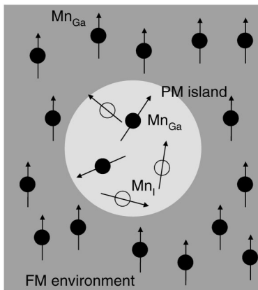
FIG. 5. Schematic diagram of a PM nanoisland. Interstitial (substitutional) ions are indicated by open (closed) circles. The island radius is \sim 5 –10 nm. The \text{Mn}_{\text{Ga}} spins are oriented randomly inside the island, but along the same direction outside.
