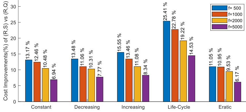
Figure 6: Cost gains of the (R, S) model across demand and dispatching cost settings
