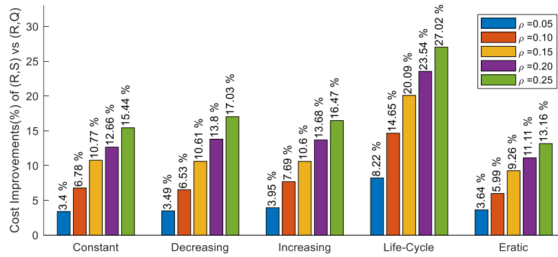
Figure 5: Cost gains of the (R, S) model across demand and CV settings
