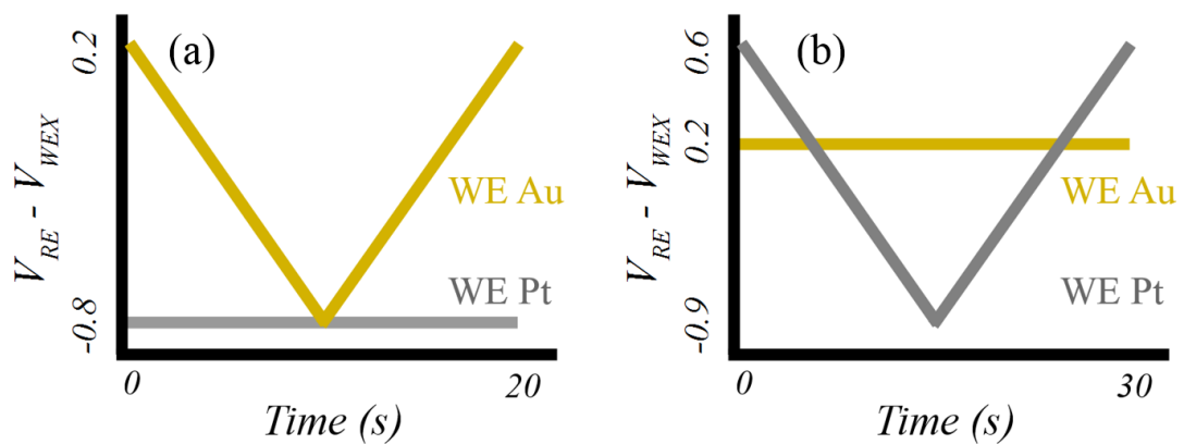
Figure 4.14: Voltages applied by system for dissolved oxygen measurement and electrode clean for, (a) Cleaning scan performed on micro-bands between dissolved oxygen measurements, (b) Voltammetric test required for dissolved oxygen.
