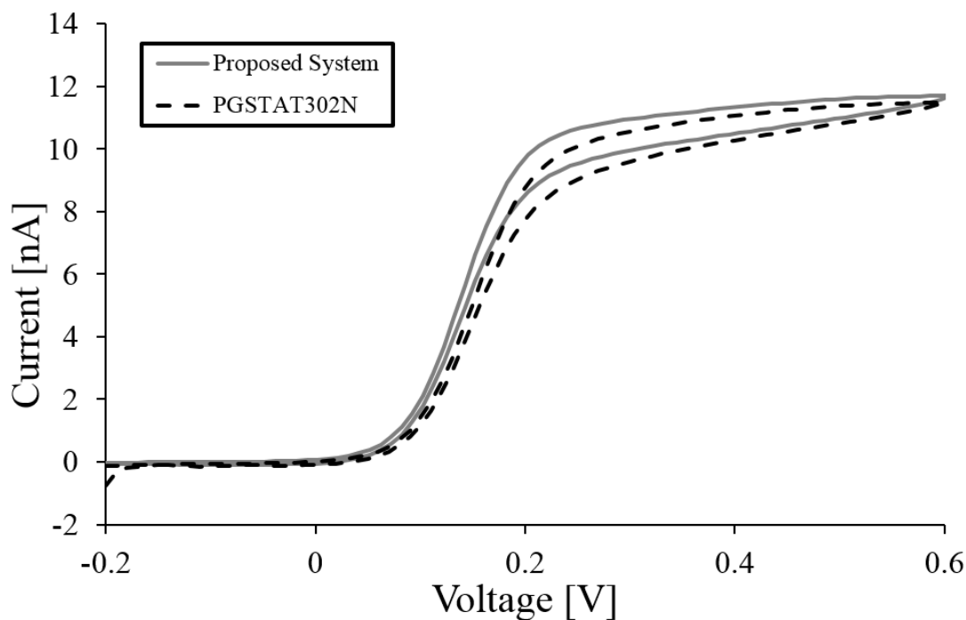
Figure 4.5 Generator Collector Cyclic Voltammogram of 1mM FcCOOH using an interdigitated ultramicro band sensor, swept at 100mV/s using the proposed system and a laboratory benchtop potentiostat. (WE2 maintained at -0.2).
