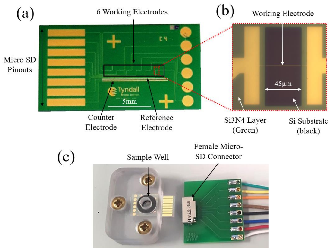
Figure 3.1: (a) Tyndall ultramicro sensor chip, (b) Optical micrograph of ultramicro electrode, (c) Chip holder and micro SD connector.
