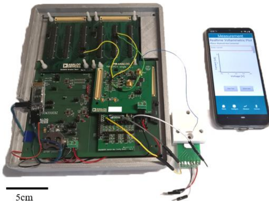
Figure 4.7: Proof of concept portable dual electrode system inside a 3d-printed enclosure, interfacing to an ultramicro electrochemical sensor with smartphone interface.
