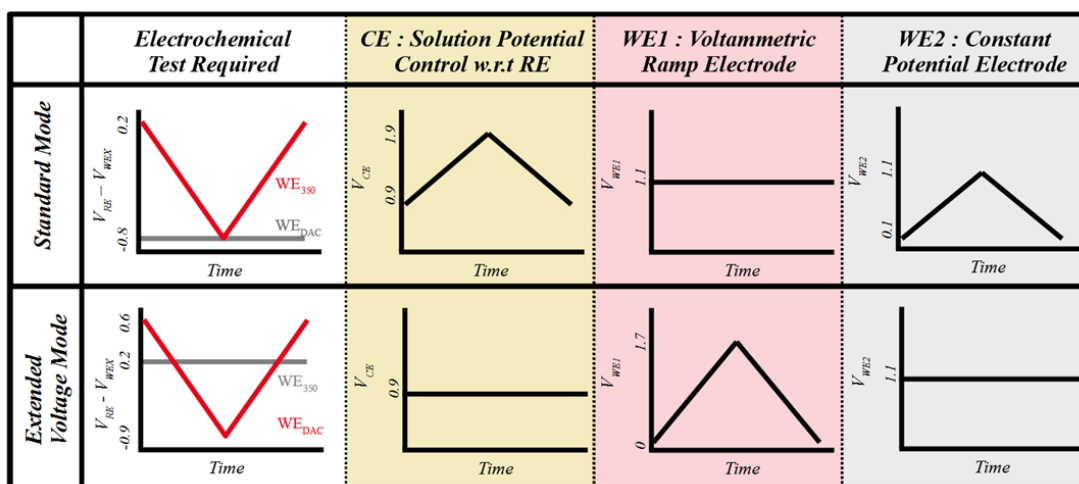
Figure 4.3: Voltage levels applied by system to realise standard and extended voltage levels.
