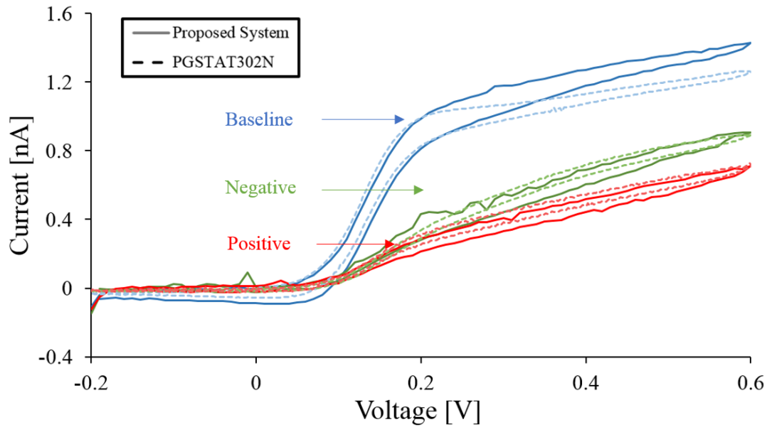
Figure 5.5: Cyclic Voltammogram of 1 \mu m microband electrochemical sensor using 1Mm FcCOOH for pre-test, negative BVD virus serum application and positive BVD serum application on Autolab PGSTAT302N and ADuCM350.
