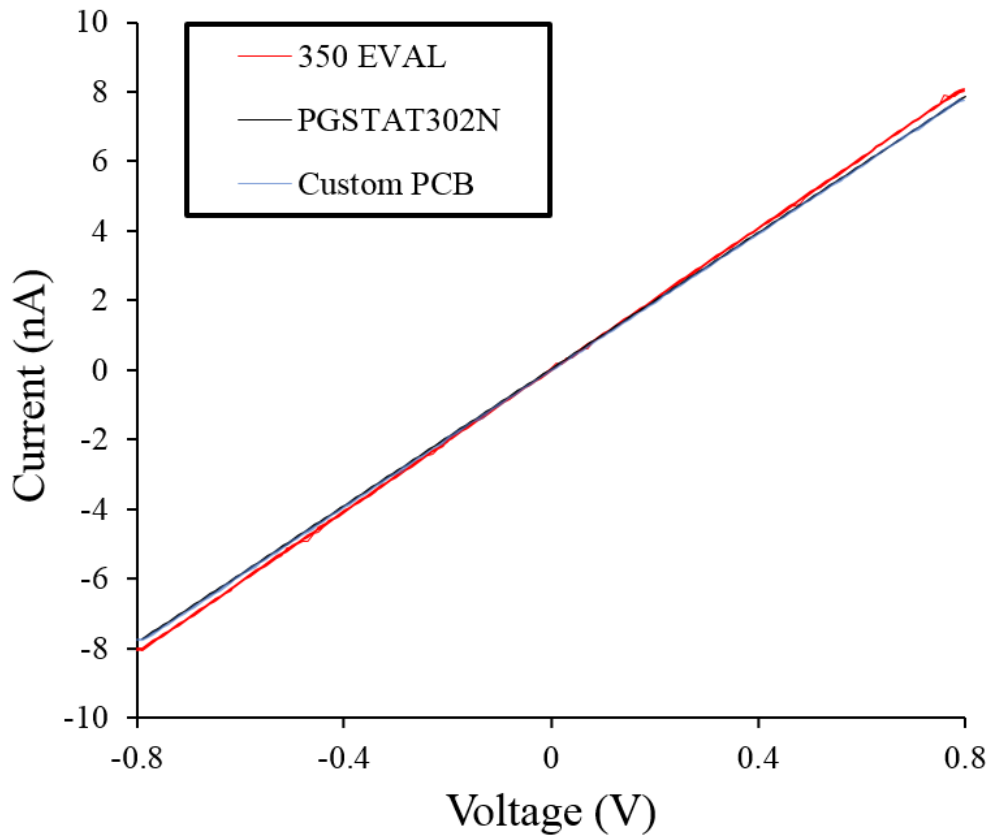
Figure 4.11: Cyclic Voltammetry scan across full range of ADuCM350 for the Custom PCB, ADuCM350 evaluation board and the Metrohm PGSTAT302N potentiostat.
