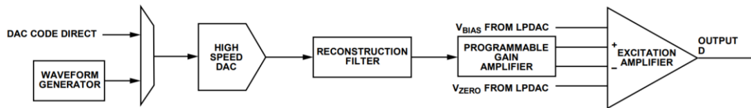
Figure 5.9: Overview of excitation signal generation path, used in the ADuCM355.
