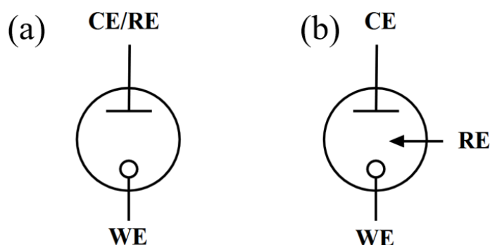
Figure 3.15: Connections of Counter, Reference and Working electrode for (a) 2 electrode and (b) 3 electrode measurements.
