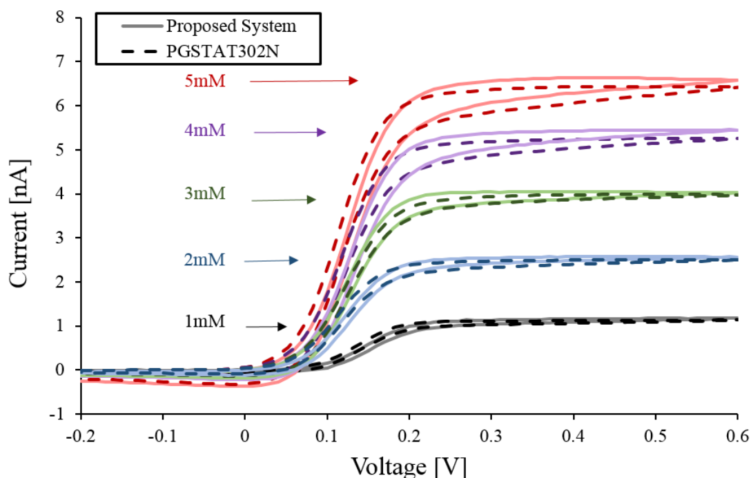
Figure 3.17: Cyclic voltammetry scan measuring varying concentrations of \text{FcCOOH} using nanowire sensor, swept at 100 mV/s, where the solid line is the result obtained using the proposed system. While the dashed line is the result obtained using the PGSTAT302N.
