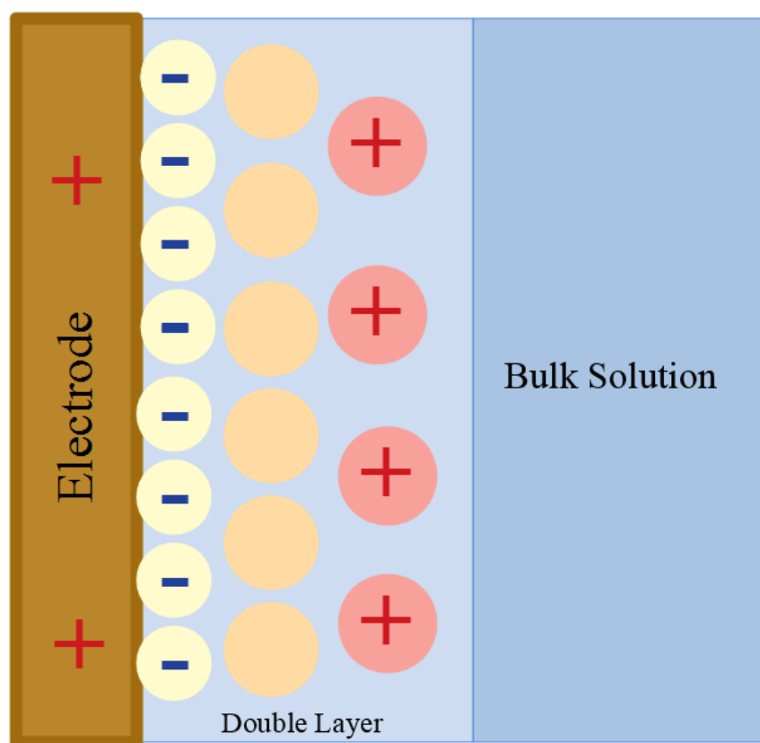
Figure 2.5: Simplified diagram of double layer capacitance for an electrochemical cell.
