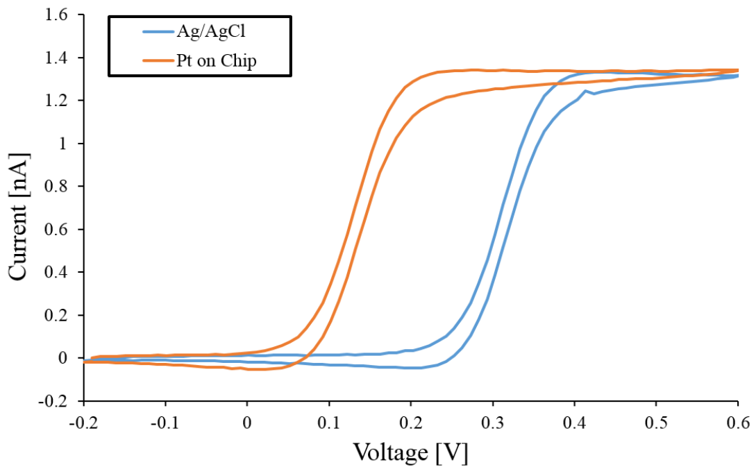
Figure 2.2: Electrochemical test using a silver/silver chloride aqueous reference electrode and a platinum on chip pseudo reference electrode.
