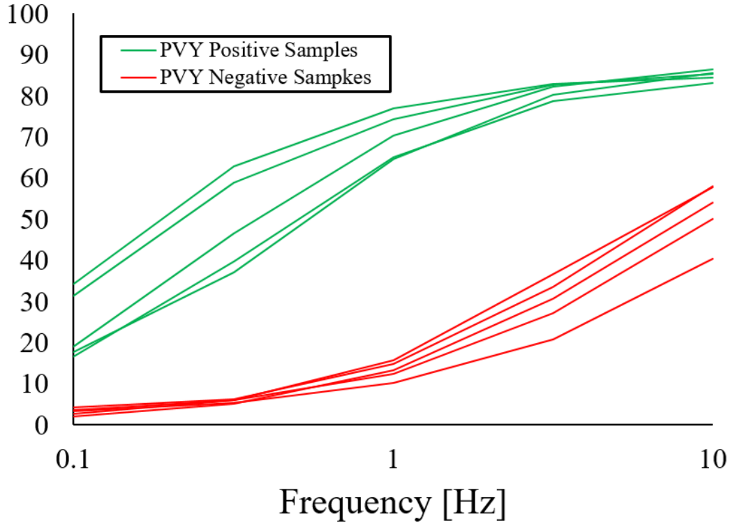
Figure 5.31: Bode plot of impedance magnitude of a positive and negative PVY sample on 0.1Mm Ferriferrocyanide using ultramicroband immunosensors, performed by the developed data acquisition system in Teagasc Carlow.
