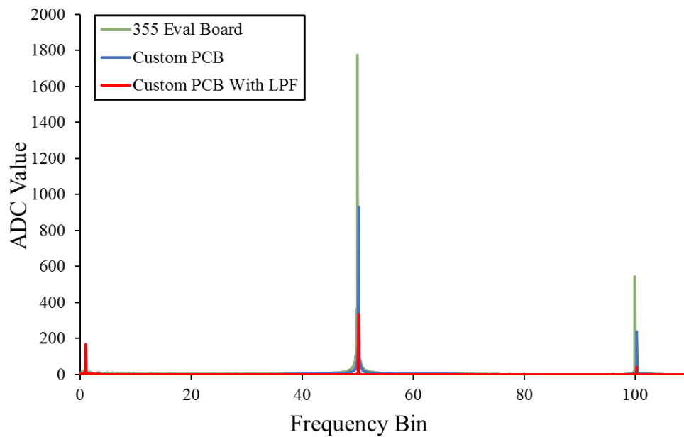
Figure 5.13: Spectral response of dummy cell signal path using different board configurations which shows that a shorter signal path and a LPF reduces the effect of ambient noise .
