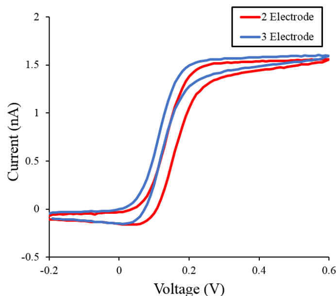
Figure 3.16: 2 vs 3 electrode electrochemical measurements for the same ultramicroband electrochemical sensor using proposed system.
