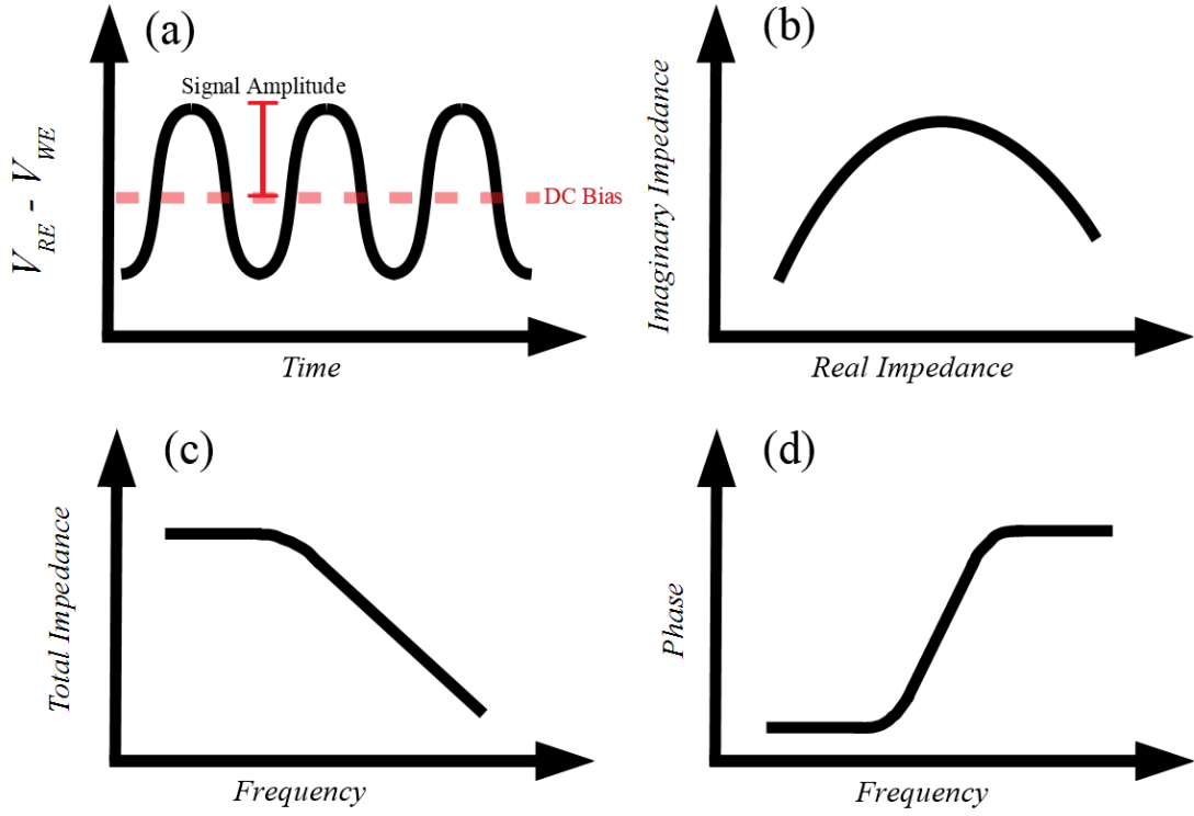
Figure 2.15: EIS applied signals and resultant graphs: (a) AC signal applied with a DC bias, (b) Nyquist Plot of real vs imaginary impedance, (c) Bode Plot of frequency vs total impedance, (d) Bode Plot of frequency vs phase.
