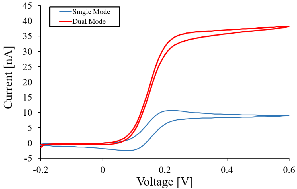
Figure 4.4: Cyclic Voltammogram fusing dual electrode proof of concept system at 100mV/s of interdigitated ultramicro band electrochemical sensor for single and dual electrode configurations (WE 2 maintained at -0.2 V for dual mode).
