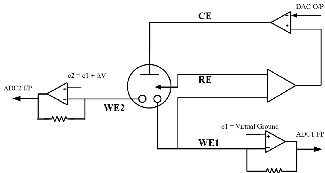
Figure 2.13: Example of bipotentiostat circuit, with a control amplifier, electromoter and two trans-impedance amplifiers.
