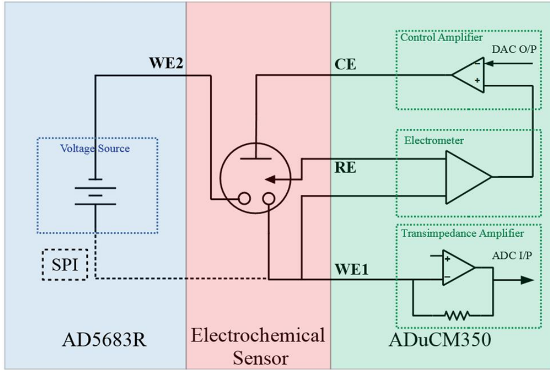
Figure 4.2: Circuit diagram of dual electrode interface system proof of concept, which includes the potentiostatic circuit from Chapter 3 and a voltage source to maintain a constant potential between WE1 and WE2.
