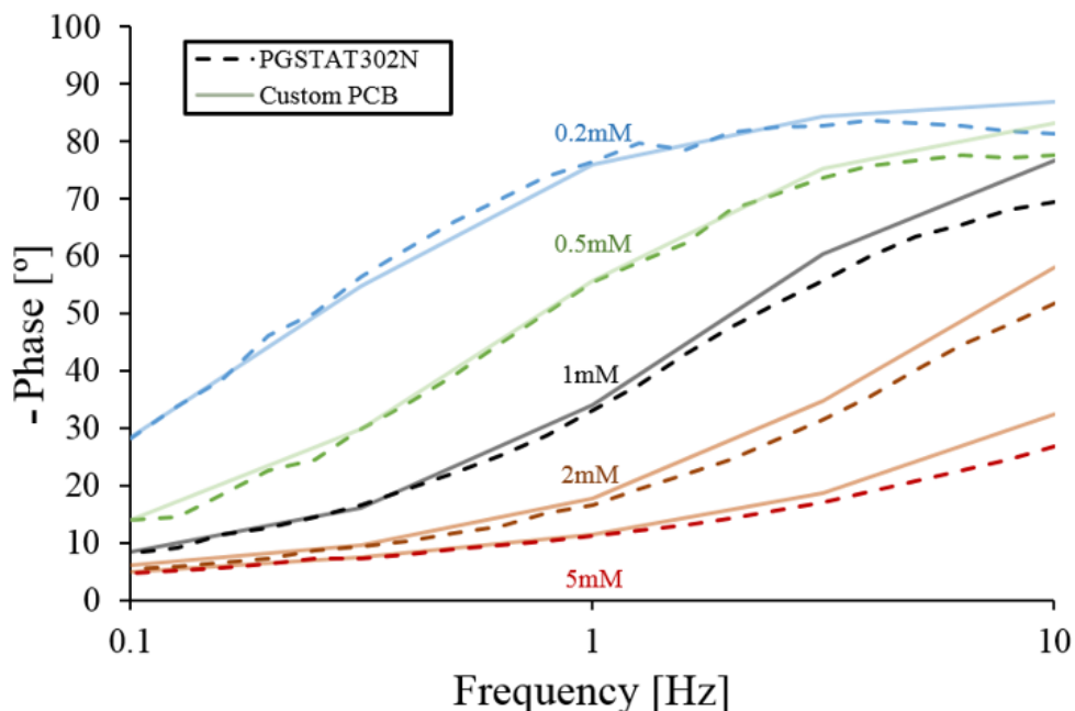
Figure 5.245: Phase response of EIS scan from 0.1 Hz to 10 Hz, AC amplitude 5 mV, 0.2 V DC bias for various concentrations of FcCOOH using both the custom PCB inside a low cost faraday cage and the PGSTAT302N for an ultra microband electrode.
