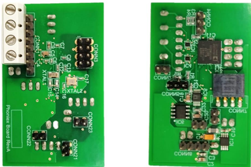
Figure 4.10: Front and back of the 6 layer data acquisition PCB, dimensions; 57 mm by 36 mm. To minimise the footprint, the ADuCM350 was placed at the back of the PCB.
