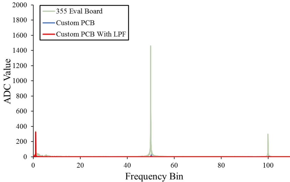
Figure 5.14: Spectral response of RCAL signal path using different board configurations which shows that a shorter signal path significantly reduces the effect of 50 Hz noise.
