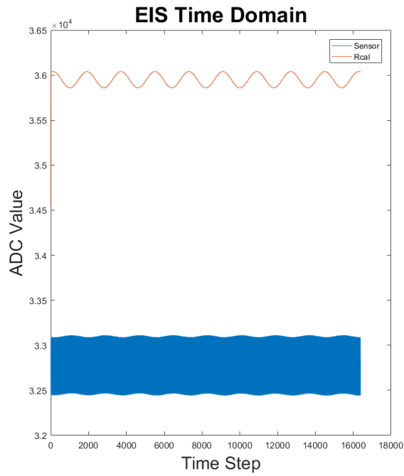
Figure 5.27: Raw ADC values of EIS measurement on 1\text{ G}\Omega , 1\text{ nF} dummy cell using the proposed system in an environment without high volumes of ambient electromagnetic noise.
