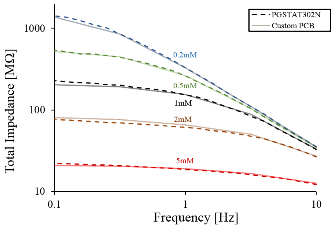
Figure 5.234: Magnitude response of EIS scan from 0.1 Hz to 10 Hz, AC amplitude 5 mV, 0.2 V DC bias for various concentrations of FcCOOH using both the custom PCB inside a low cost faraday cage and the PGSTAT302N for an ultra microband electrode.
