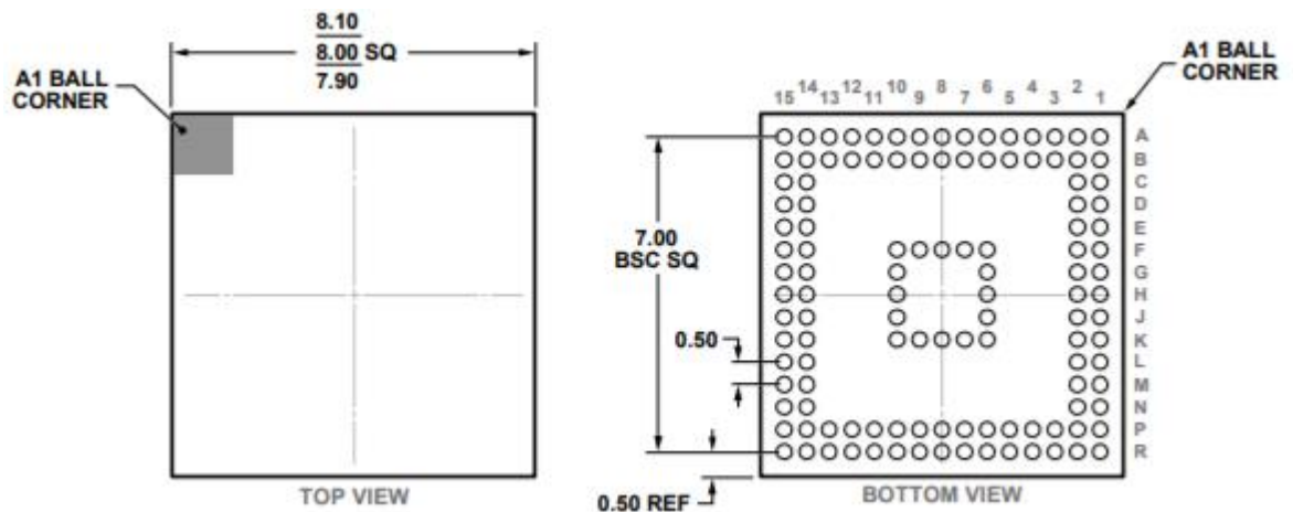
Figure 4.9: Top and bottom view of ADuCM350 IC package. This BC-120-3 package requires a multilayer board to route all required signals to and from the chip.
