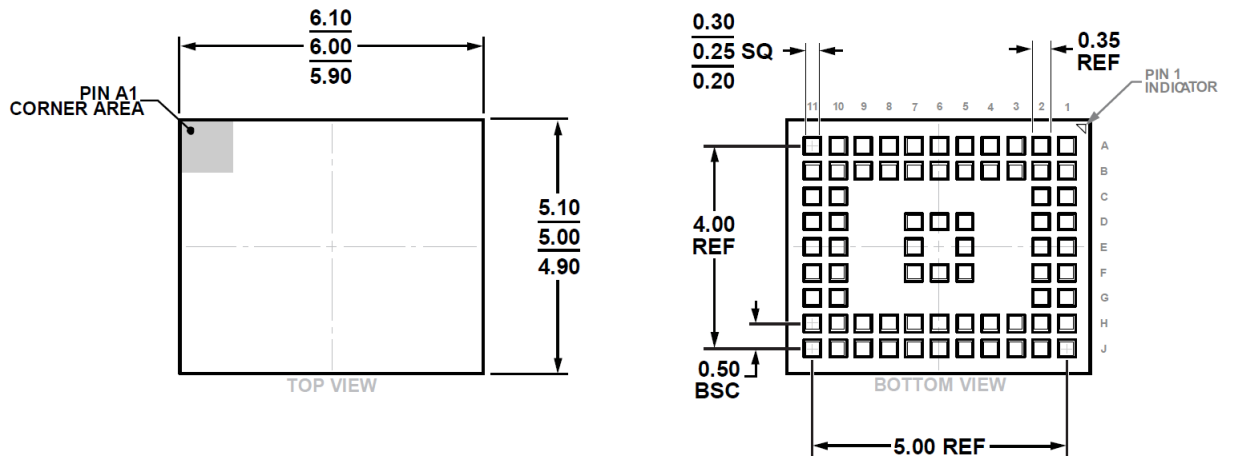
Figure 5.15: Top and bottom view of ADuCM355 chip.
