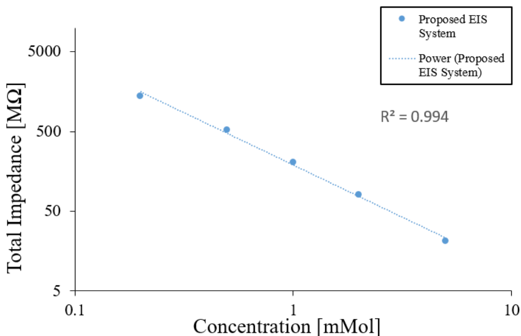
Figure 5.256: Calibration plot for EIS measurements using the proposed system at 0.1Hz in varying concentrations of Ferri-Ferrocyanide, n=1 .
