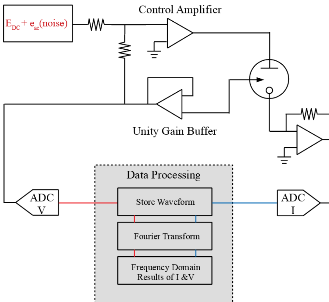
Figure 2.19: Example of typical potentiostatic apparatus, including control amplifier, unity gain buffer and trans-impedance amplifier with ADCs to measure both the applied voltage and resultant current. Also included, are the data processing steps used for Fourier analysis of AC current and voltage.
