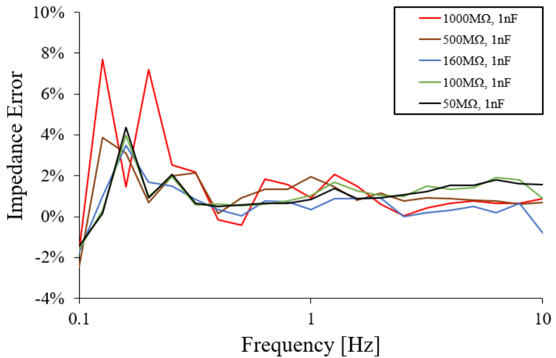
Figure 5.20: Error between of system and Autolab PGSTAT302N, for EIS test using various dummy cells of similar impedance values expected from electrochemical ultramicro immunosensors.
