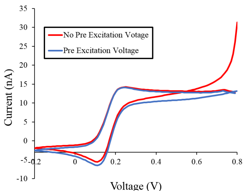
Figure 3.14: 0.1mMol FcCOOH CV, scanned from 0.8 V to -0.2 V at 100mV/s using no pre-excitation voltage and a pre-excitation voltage to interface between the proposed system and an interdigitated electrochemical sensor.
