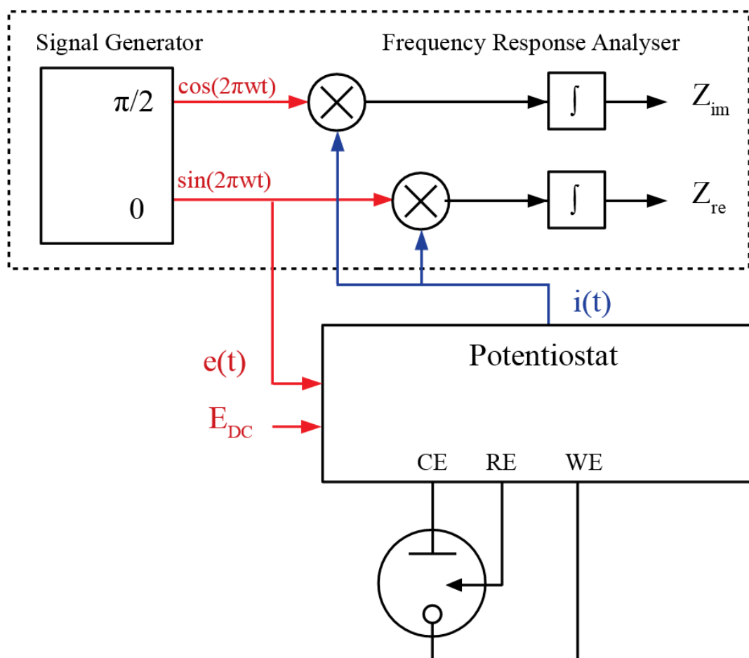
Figure 2.18 Example of system used to measure the impedance of an electrochemical cell based on a frequency response analyser. The red lines in the diagram represent the voltage paths, while the blue represent the resultant current path. The crosses in the diagram represent signal mixers.
