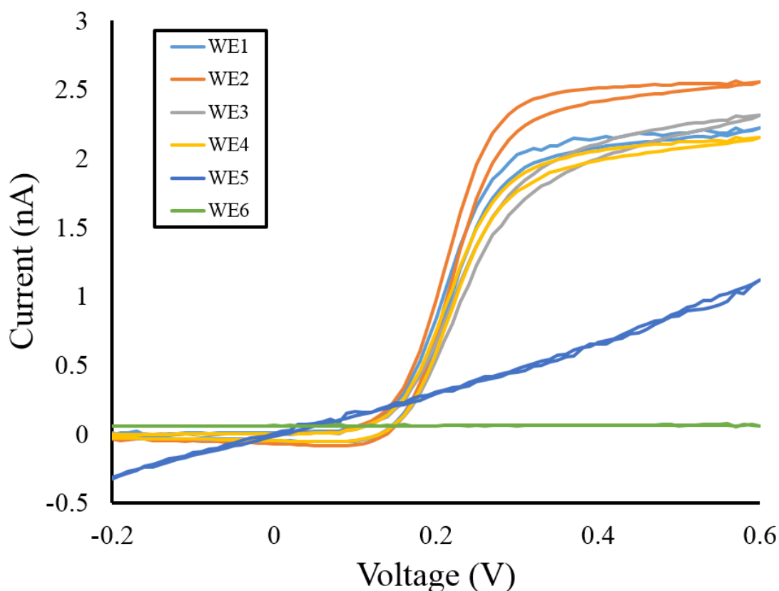
Figure 3.11: Multiplexed output ultramicro band sensor in FcCOOH using proof of concept system, demonstrating that the proposed system can interface to multiple Working Electrodes.
