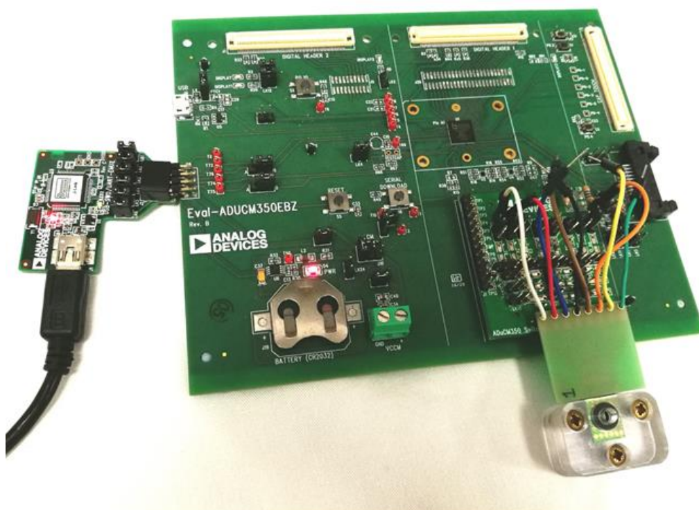
Figure 3.8: System interfacing to electrochemical sensor.
