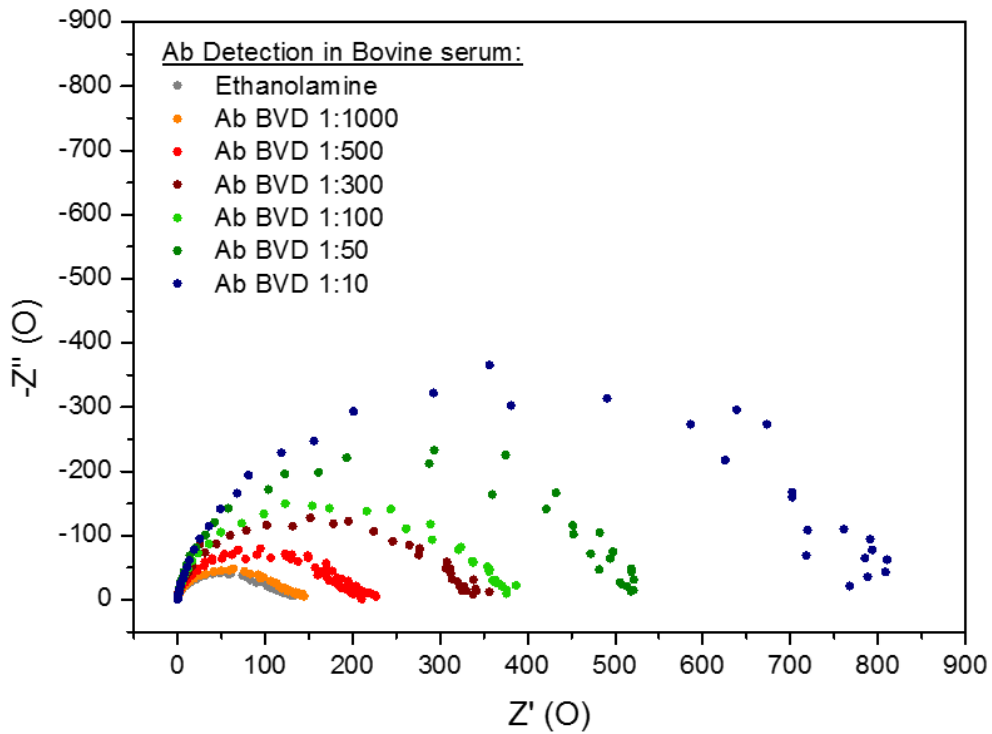
Figure 5.6: EIS plot for varying concentrations of BVD antibody for a nanowire electrochemical sensor using PGSTAT302N [13].
