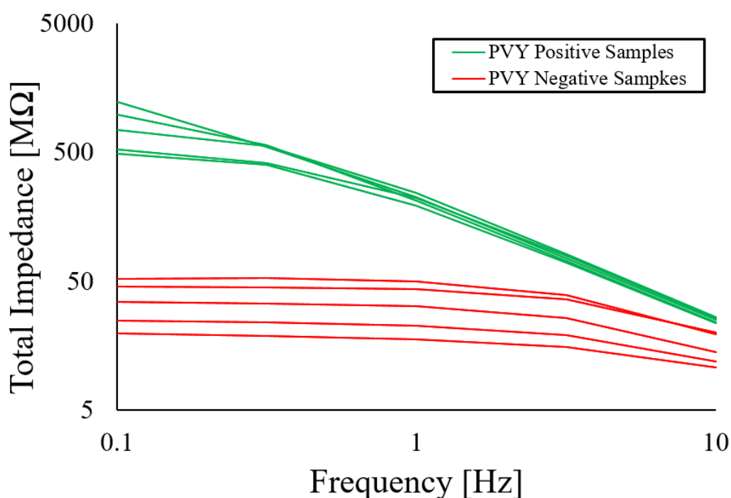
Figure 5.30: Bode plot of impedance magnitude of a positive and negative PVY sample on 0.1Mm Ferriferrocyanide using ultramicroband immunosensors, performed by the developed data acquisition system in Teagasc Carlow.
