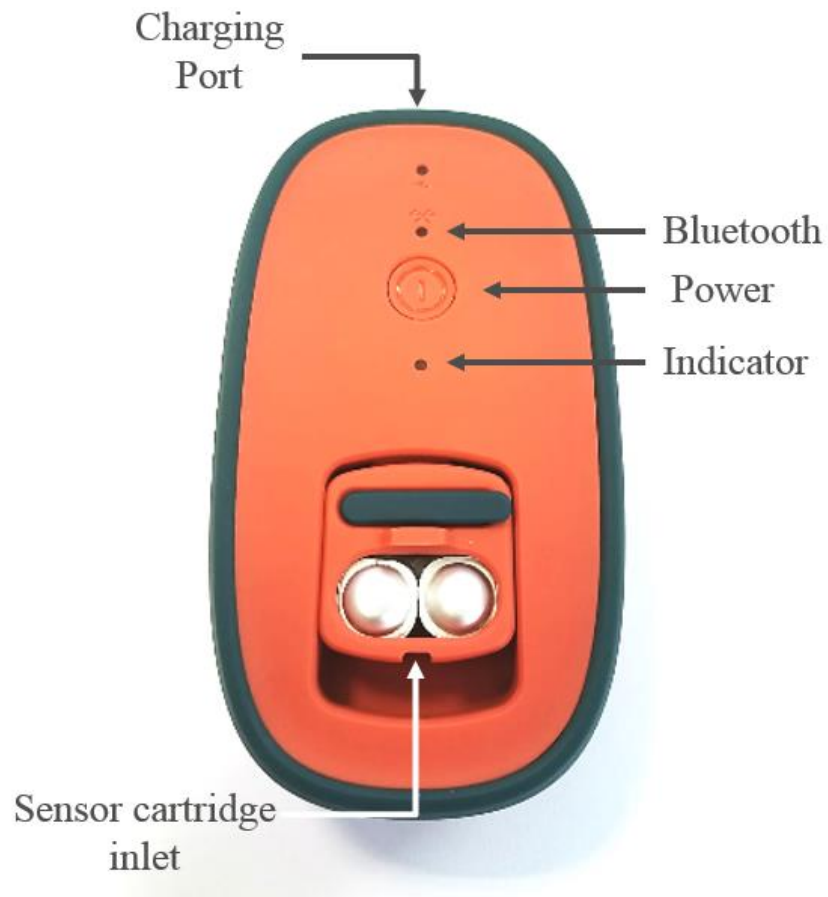
Figure 5.18: On farm diagnosis prototype device which includes the sensor cartridge and an inlet, indicator lights, a power button and charging port.
