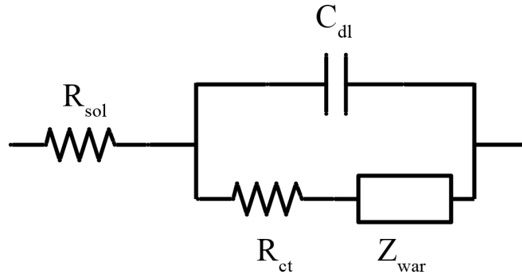
Figure 2.4: Randles circuit model of electrode-electrolyte interface.
