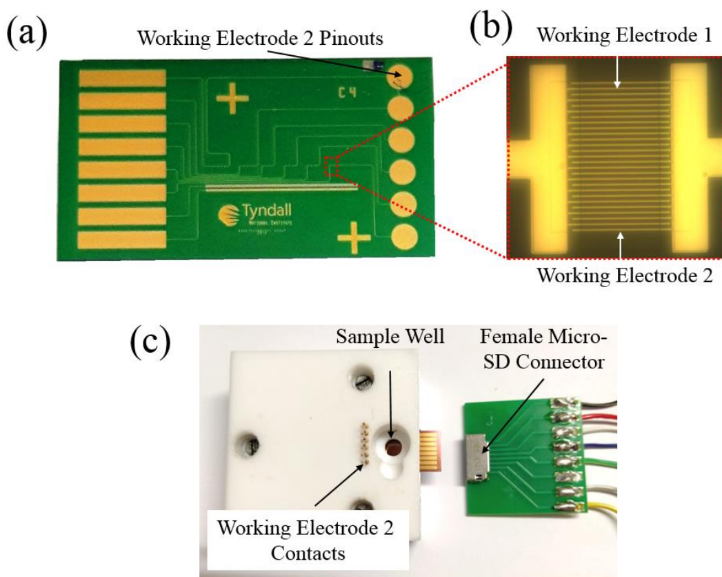
Figure 4.1: (a) Tyndall ultramicro band sensor chip with CE , RE and 6 WE1 accounting for the contact pads on the lefthand side and 6 WE2 accounting for the contact pads on the right hand side, (b) Optical micrograph of interdigitated 1\mu\text{m} ultramicro band with 2\mu\text{m} spacing, (c) Interdigitated chip holder and micro sd connector.
