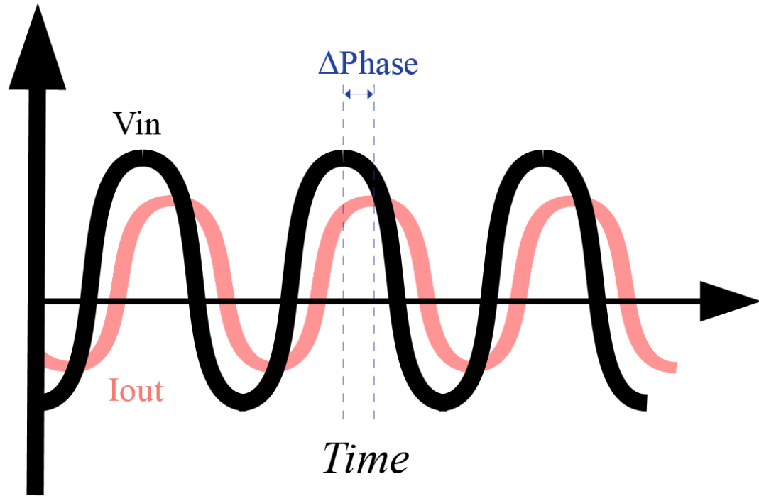
Figure 2.17: Representation of the applied sinusoidal input voltage and resultant current output of an EIS excitation signal, which stimulated at a given frequency.
