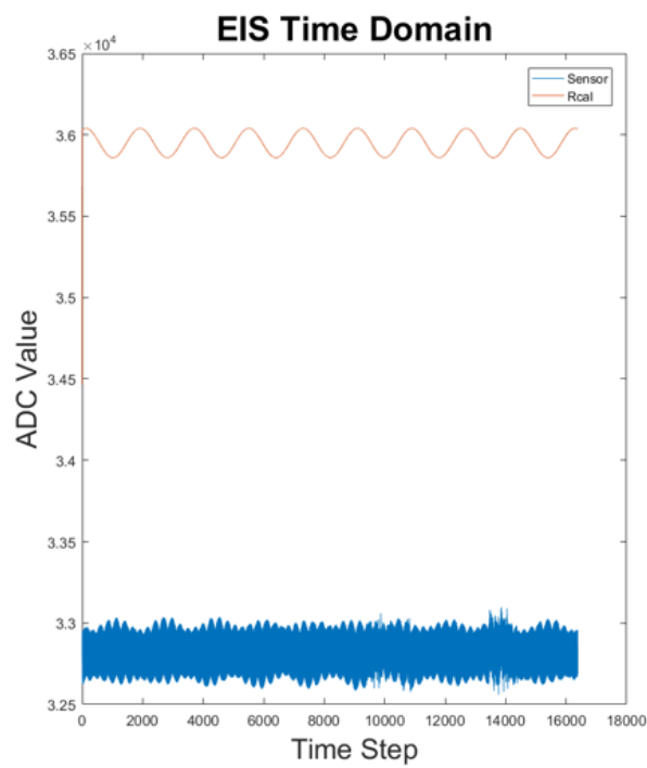
Figure 5.268: Raw ADC values of EIS measurement on 1\text{ G}\Omega , 1\text{ nF} dummy cell, with measurements taken in proximity to the AIX200 atomic vapour deposition machine.
