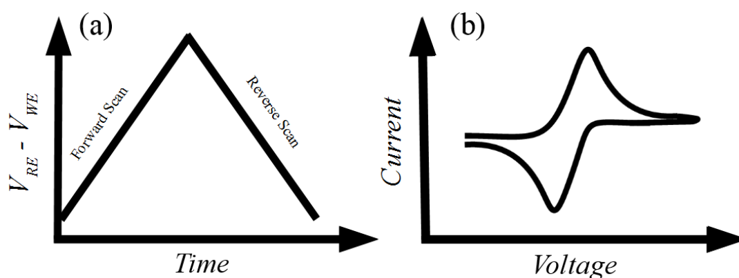
Figure 2.6: (a) CV voltage ramp, (b) Typical current response from CV.
