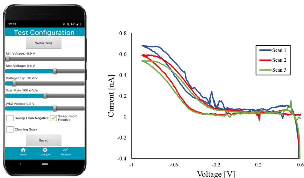
Figure 4.17: Screenshot of required dissolved oxygen measurement voltammogram configuration in Android smartphone application and three resultant current outputs recorded at a dissolved oxygen concentration of 3ppm, using the developed system. Note that the peak of these voltammograms represent the H_2O_2 being oxidised back to H_2 as outlined in equation 4.2.
