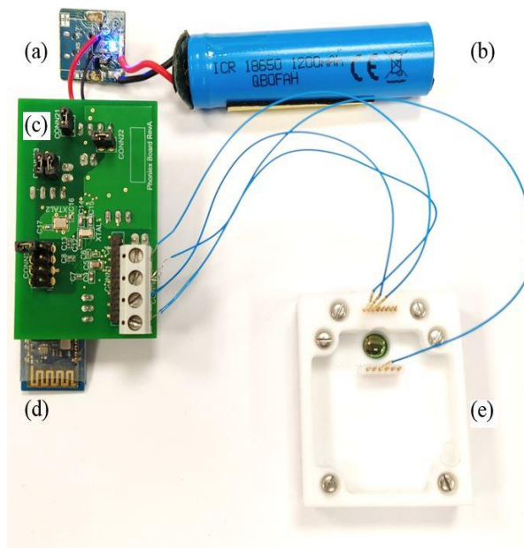
Figure 4.16: Dissolved oxygen measurement apparatus including, (a) Charger and Protection PCB, (b) Battery, (c) Proposed System PCB, (d) HC-05 Bluetooth Module, (e) Electrochemical Sensor.
