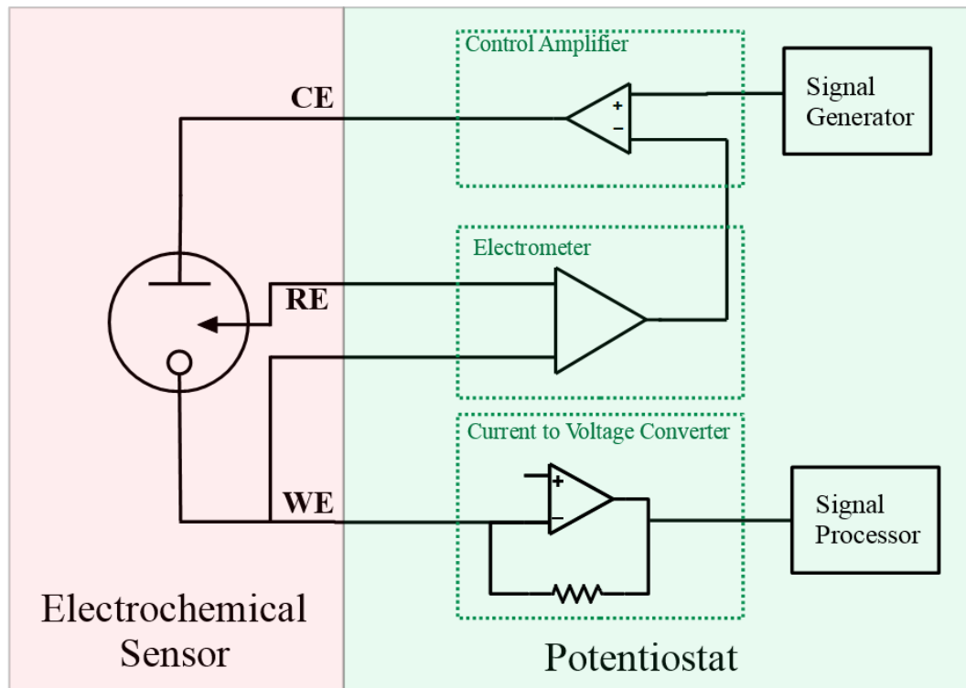
Figure 2.3: Potentiostat schematic for three electrode electrochemical cell.
