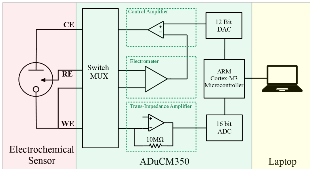
Figure 3.7: Simplified block diagram of ultramicro electrochemical interface proof of concept using ADuCM350 evaluation board.
