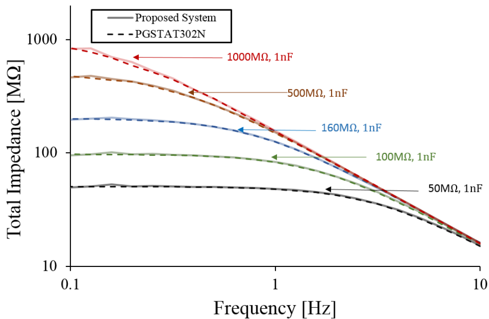
Figure 5.19: Magnitude response of system and Autolab PGSTAT302N, for EIS test using various dummy cells of similar impedance values expected from electrochemical ultramicro immunosensors.
