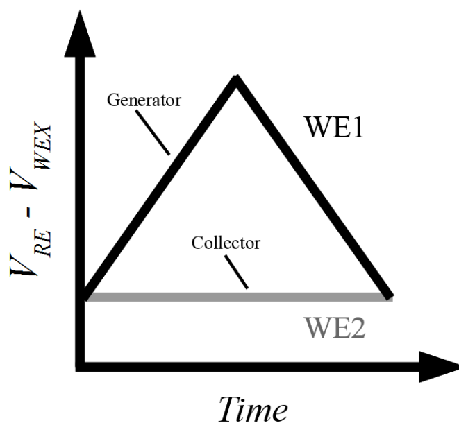
Figure 2.11: Example of voltage levels of generator collector voltammogram for WE1 and WE2.
