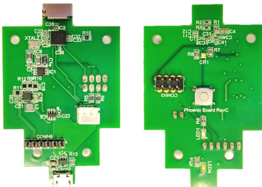
Figure 5.16: Front and back of portable EIS data acquisition PCB.
