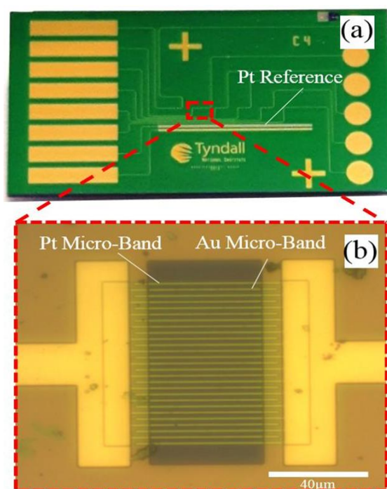
Figure 4.13: Tyndall National Institute electrochemical dissolved oxygen sensor, including, (a) Tyndall National Institute Electrochemical Sensor chip, (b) Microscopic view of gold and platinum deposited 1µm bands.
