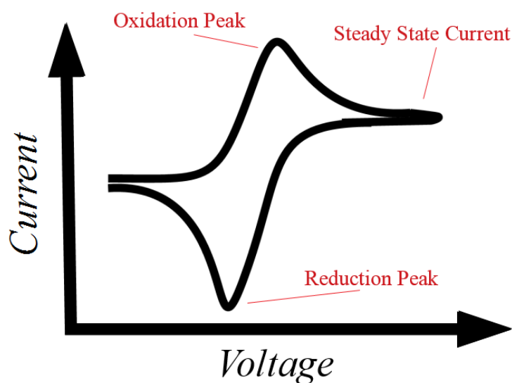
Figure 2.7: Points of interest on CV.
