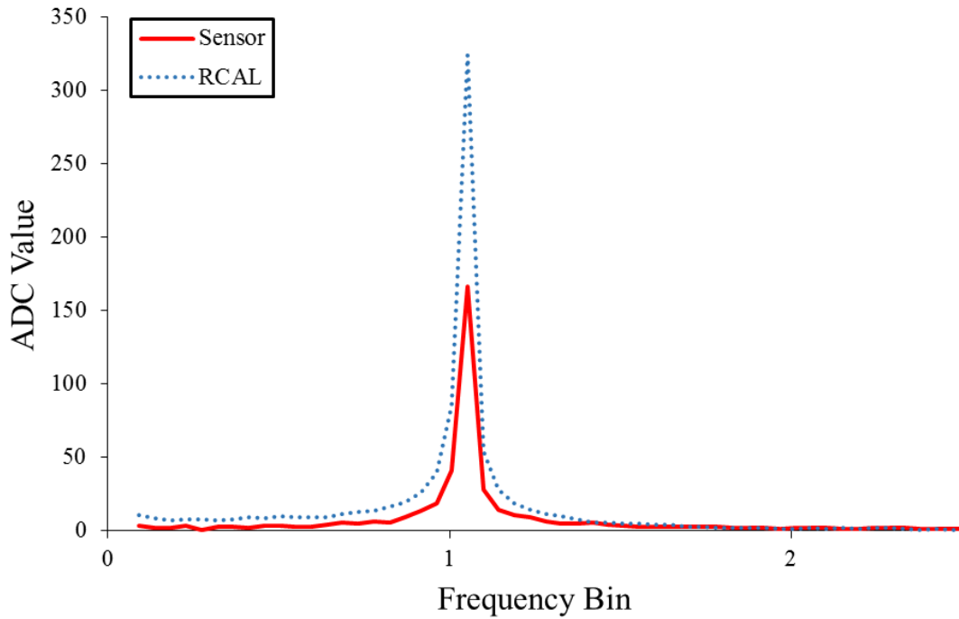
Figure 5.12: Spectral response for EIS measurement at 1Hz on 200M \Omega resistor using ADuCM355, compared against the known external 100 M \Omega RCAL resistor.
