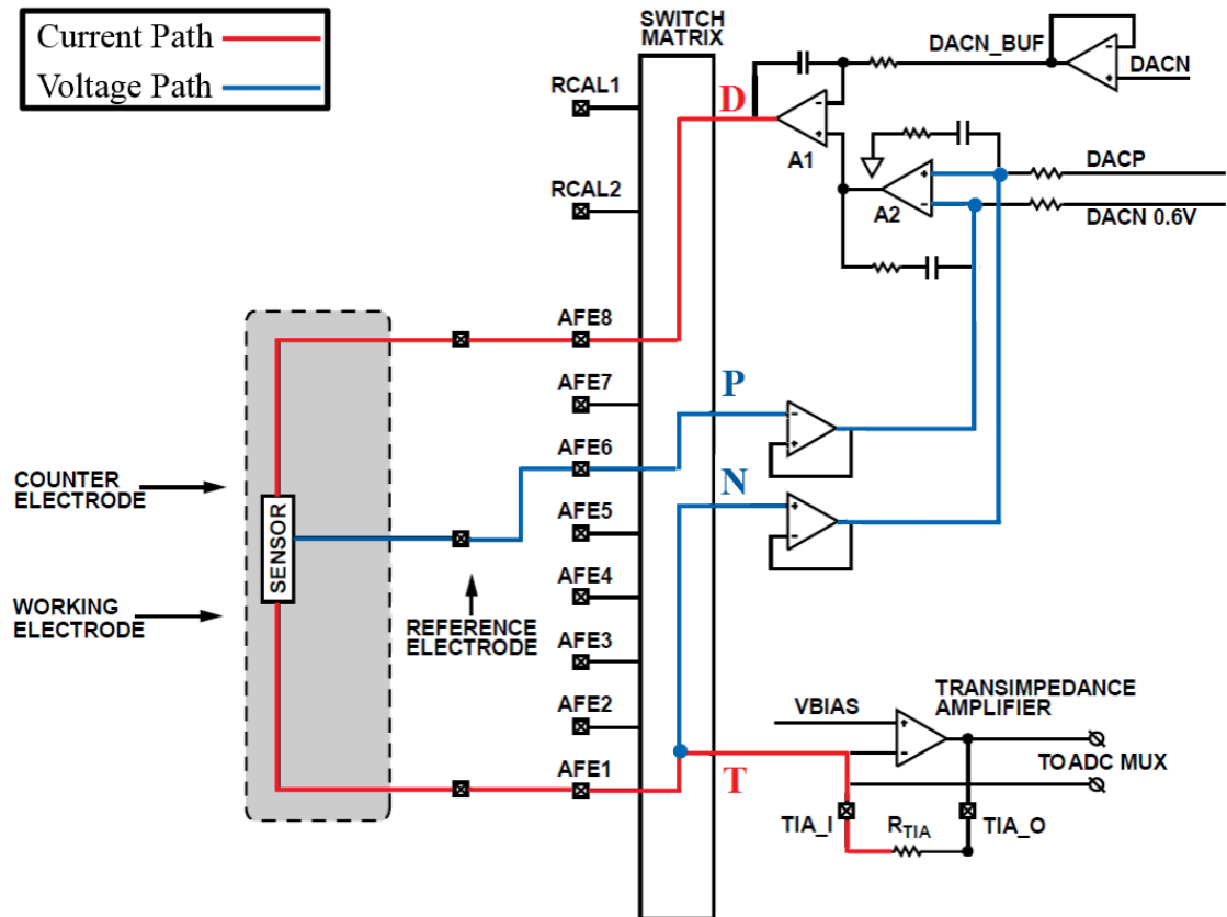
Figure 3.5: ADuCM350 AFE excitation loop for three electrode electrochemical sensor.
