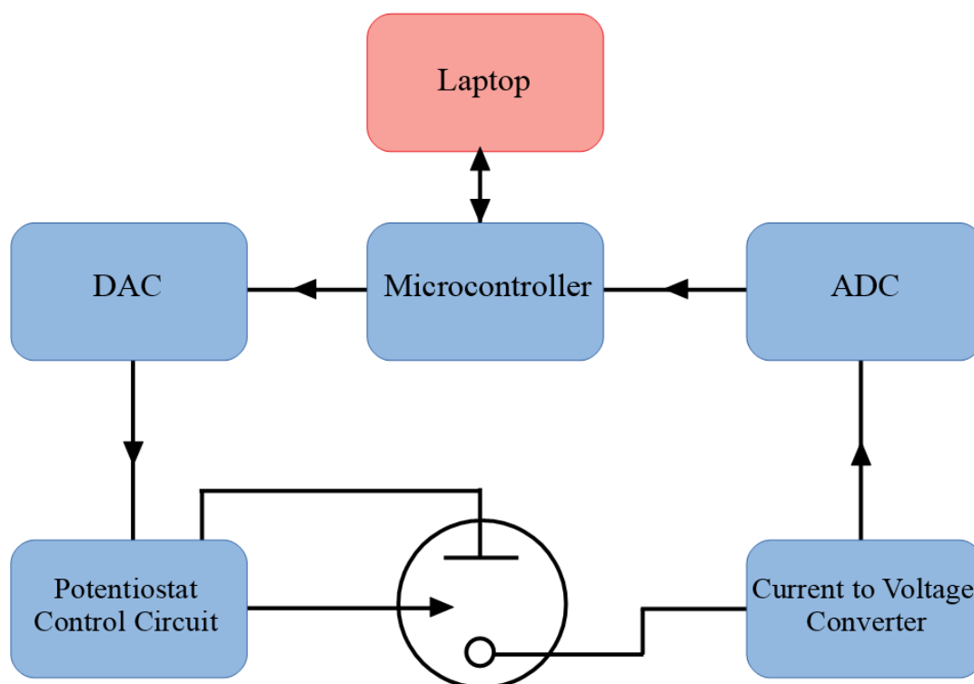
Figure 3.3: Block diagram of proposed system, consisting of a microcontroller for control of the system, DAC to provide an input signal to the potentiostat control circuit, a current to voltage converter and an ADC to read the resultant voltage from the voltammetric test.
