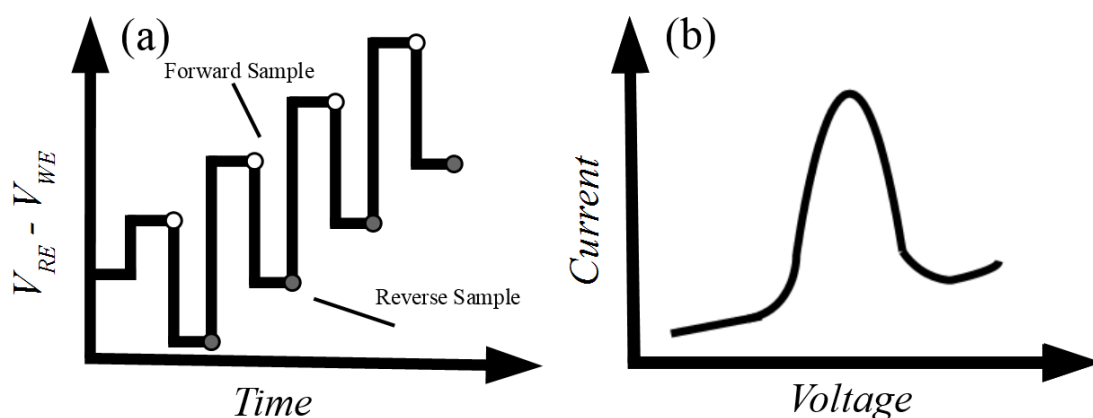
Figure 2.9: (a) SWV voltage ramp, (b) Typical current response from SWV.
