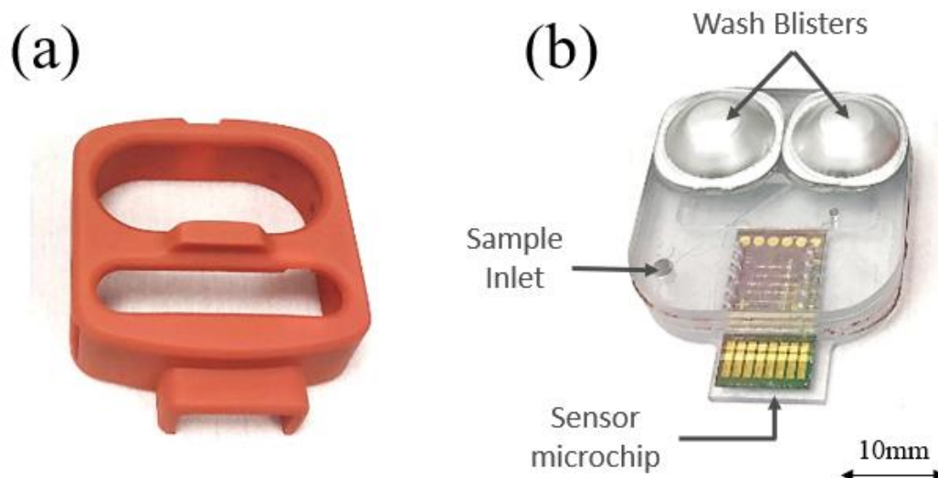
Figure 5.17: (a) Proposed Sensor Microfluidic Cartridge, (b) Proposed Sensor Microfluidic Platform which includes the electrochemical sensor under test, wash blisters and a sample inlet.
