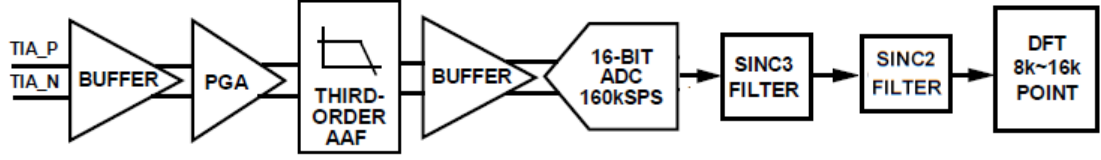
Figure 5.10: Block diagram of ADC, DFT and signal processing for EIS measurements using the ADuCM355.
