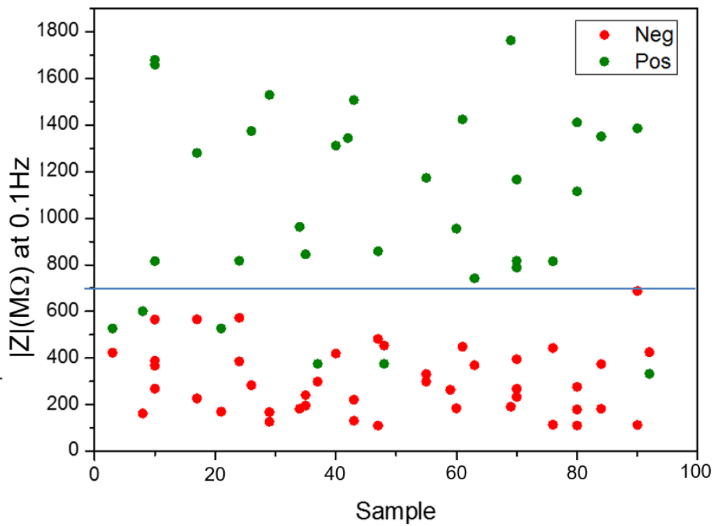
Figure 5.8: Scatter plot showing total impedance of various different BVD samples at 0.1 Hz using ultra microband electrochemical immunosensors.
