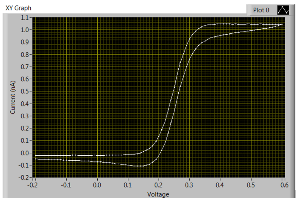
Figure 3.10: Ferrocene scan on ultramicro band electrochemical sensor using the proposed system on LabVIEW display.
