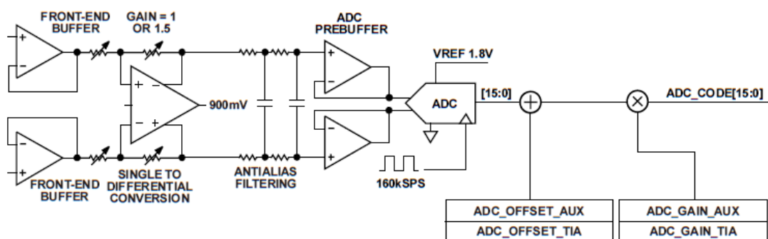
Figure 3.6: Post TIA signal processing for ADuCM350.
