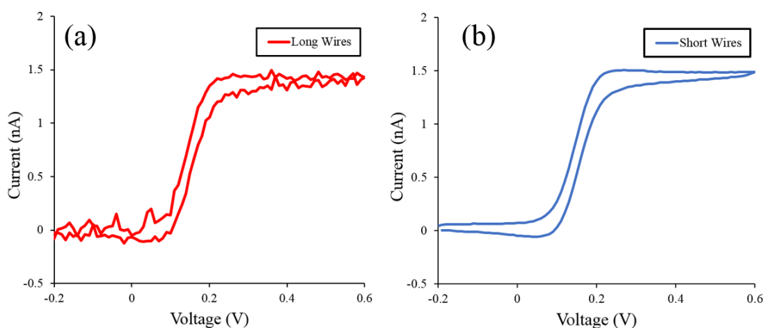
Figure 3.13: Ferrocene scan using (a) long wires and (b) short wires, to interface between proposed system and electrochemical sensor.
