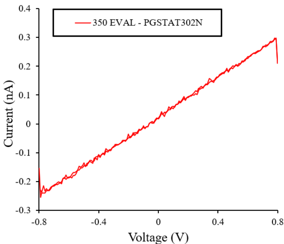
Figure 3.12: Difference between cyclic voltammetry scans for both potentiostat systems using 100 M \Omega resistor, swept at 200 mV/s.
