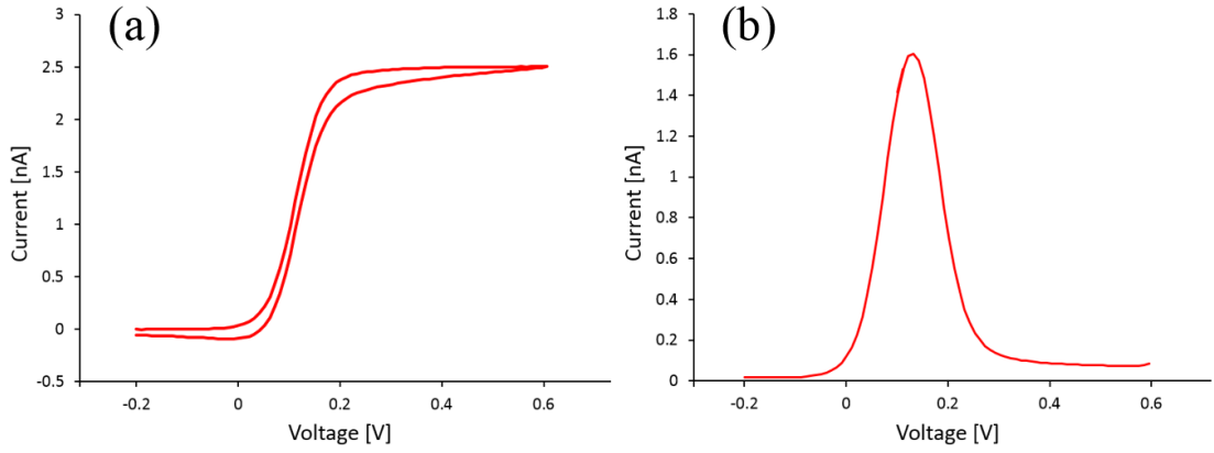
Figure 3.2: Electrochemical tests performed on 1μm ultramicro band sensor using 1mM FCOOH using laboratory potentiostat Autolab PGSTAT302N; (a) CV at 100mV/s, (b) SWV at 10Hz, swept at 100mV/s.
