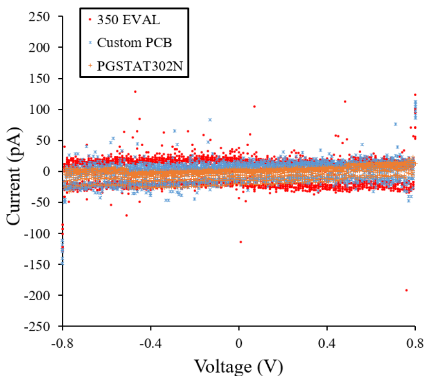
Figure 4.12: Current deviation from expected value for ten CVs swept at 200mV/s from - 0.8 V to 0.8 V using the ADuCM350 evaluation board, the custom PCB and the Metrohm PGSTAT302N.
