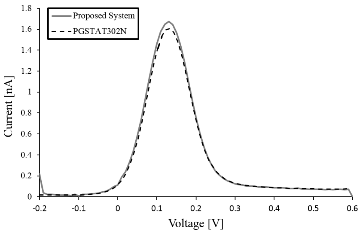
Figure 3.18: Square wave voltammogram at 10Hz, swept at 100mV/s of 1mM FcCOOH using microband sensor.
