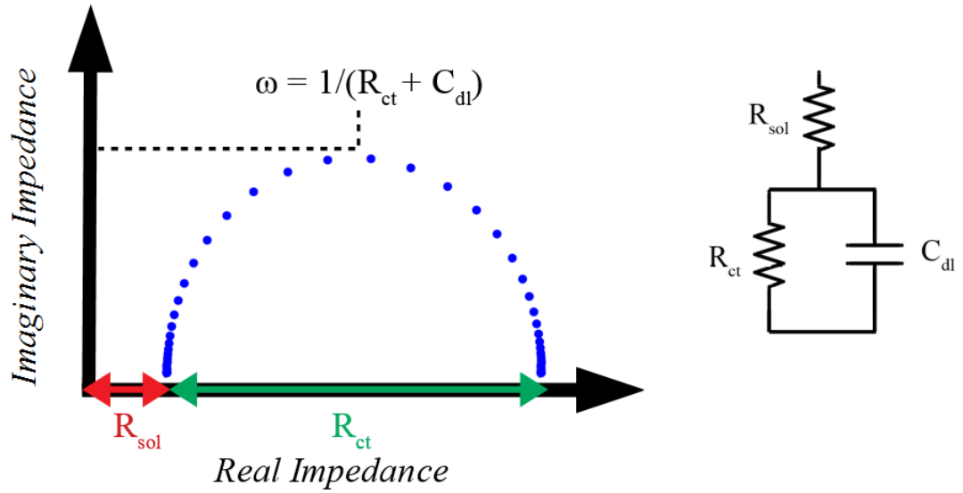
Figure 2.16 Randles circuit feature extraction from EIS Nyquist plot and simplified Randles circuit.
