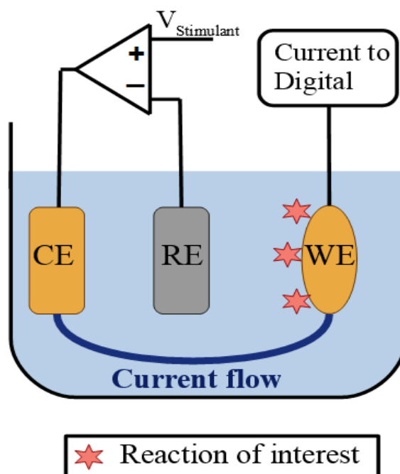
Figure 2.1: Three Electrode Electrochemical Sensor.
