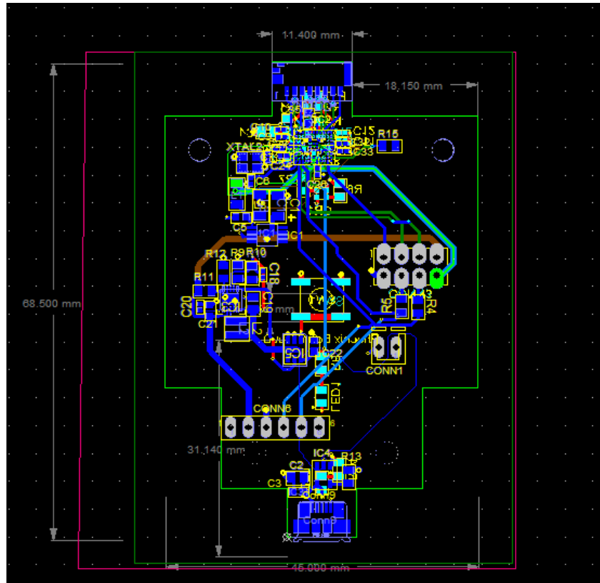
Figure A.10: All layers of EIS PCB Layout (poured shapes excluded).
