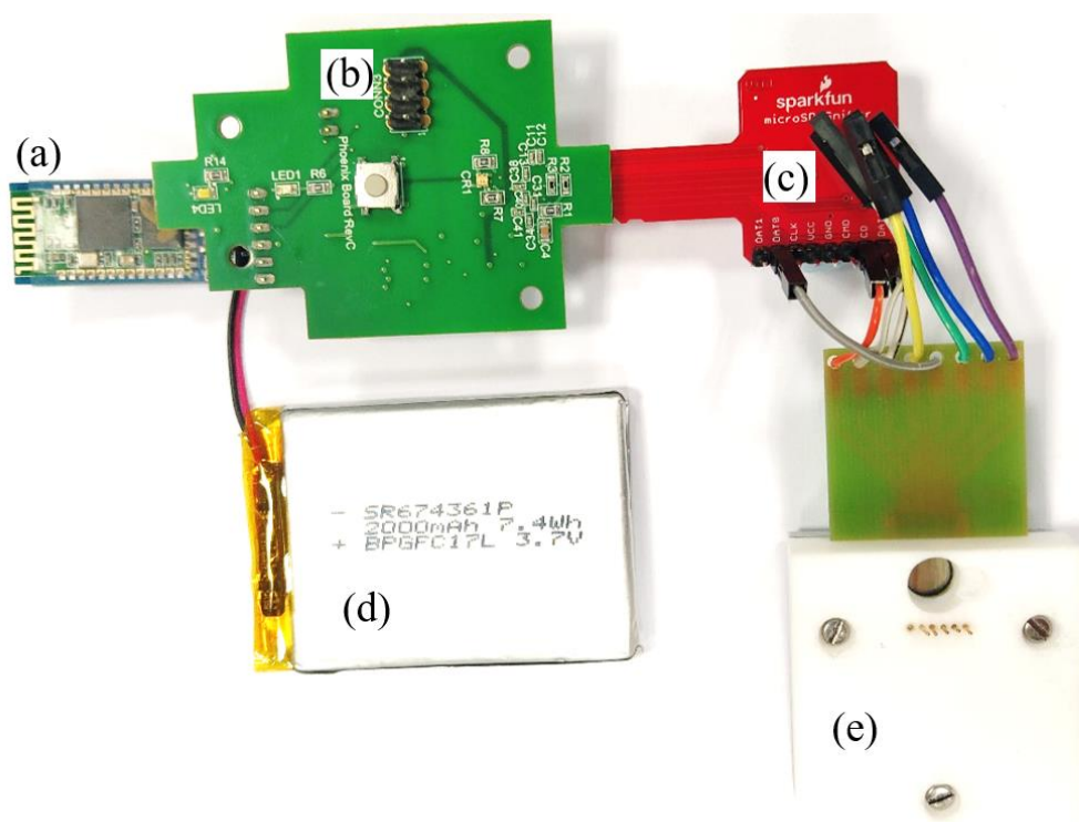
Figure 5.223: Measurement apparatus for EIS test; (a) HC-05 Bluetooth Module, (b) Proposed System PCB, (c) Sparkfun SD Edge connector, (d) Battery, (e) Electrochemical Sensor.
