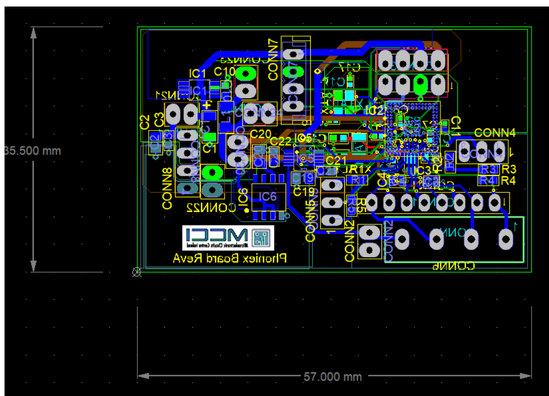
Figure A.5: All layers of voltammetric potentiostat PCB (poured shapes excluded).
