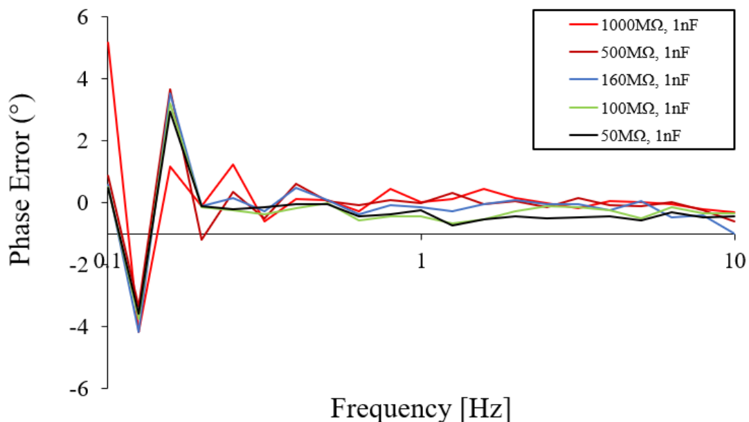
Figure 5.212: Phase response of system and Autolab PGSTAT302N, for EIS test various dummy cells of similar impedance values expected from electrochemical ultramicro immunosensors.
