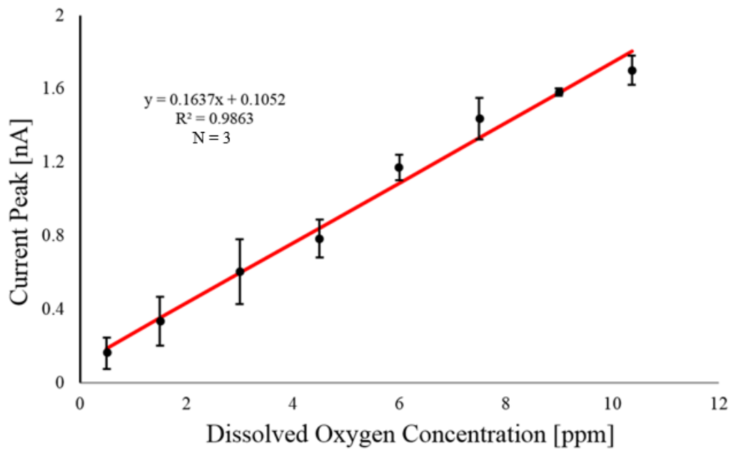
Figure 4.18: Dissolved oxygen calibration plot using river water.
