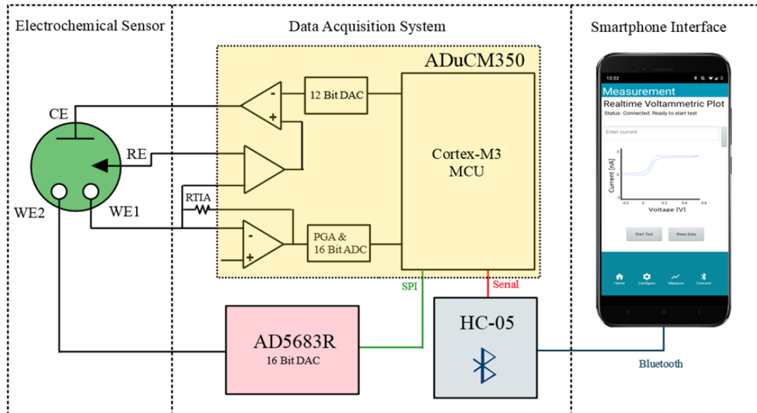
Figure 4.8: Block diagram of potable point of sample system, with separate electrochemical sensor. Data acquisition system consisting of the ADUCM350, the AD5683R connecting to the WE2, all controlled by the micro Controller in the ADUCM350. The HC-05 provides the necessary Bluetooth connection for the smartphone interface.
