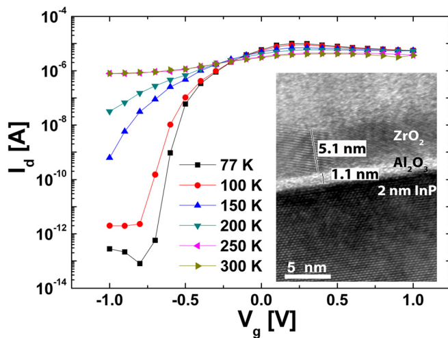
FIG. 1. (Color online) Typical transfer characteristics of high- k/\text{In}_{0.75}\text{Ga}_{0.25}\text{As} MOSHEMTs for L = 170 \text{ }\mu\text{m} and W = 20 \text{ }\mu\text{m} for various temperatures and V_{\text{ds}} = 50 \text{ mV} with a TEM image of the gate stack region shown in the inset.
