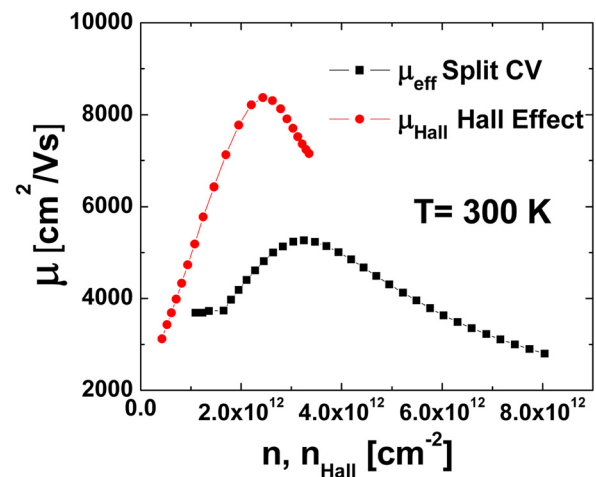
FIG. 2. (Color online) Comparison of \mu_{\text{Hall}} and \mu_{\text{eff}} ( f = 1 \text{ MHz} ) versus the corresponding carrier density ( n , n_{\text{Hall}} ) at room temperature for a high- k/\text{In}_{0.75}\text{Ga}_{0.25}\text{As} MOSHEMT with 2 nm InP top barrier layer, L = 170 \text{ }\mu\text{m} , W = 20 \text{ }\mu\text{m} , V_g = -1 \text{ V} to 1 \text{ V} range, and V_{\text{ds}} = 50 \text{ mV} .
