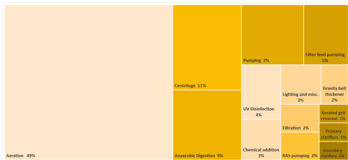
Figure 5.3: Breakdown of wastewater treatment plants (WWTP) power demand. Adapted from [14].
