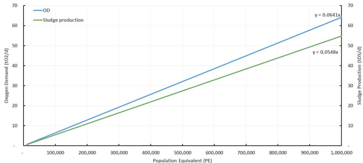
Figure 5.9: Oxygen demand and Sludge production relationship to WWTP PE based on a sludge production of 54.8 g TS/PE/d and 64.1 gO 2 /PE/d.
