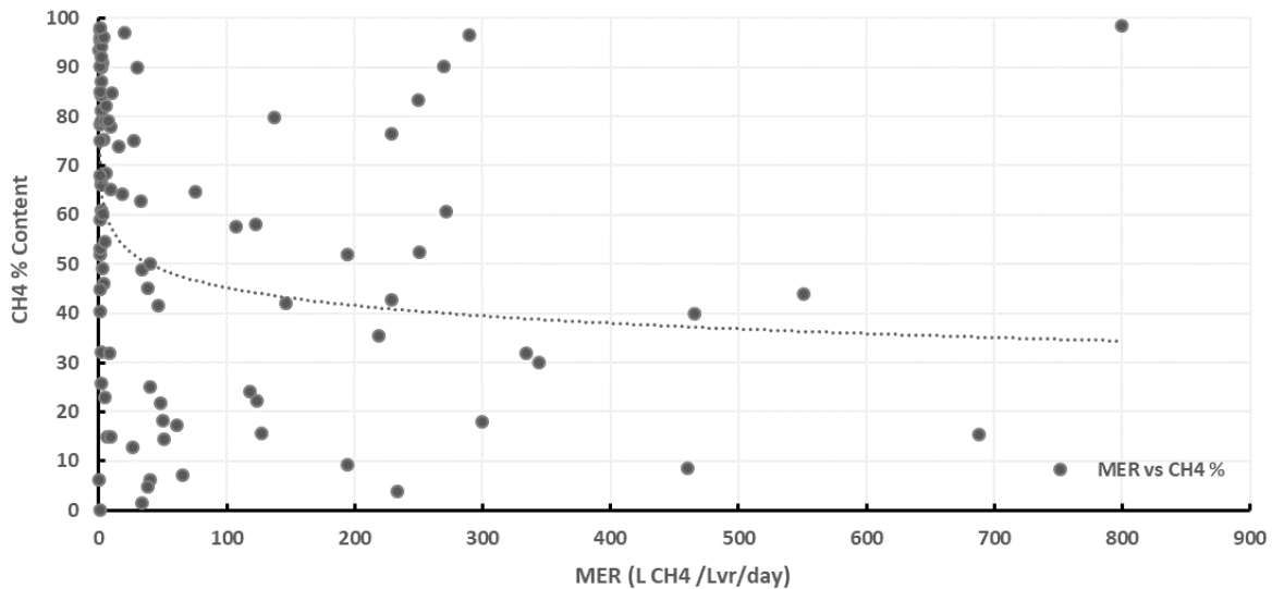
Figure 2.12: Relationship between MER and CH 4 percentage content.
