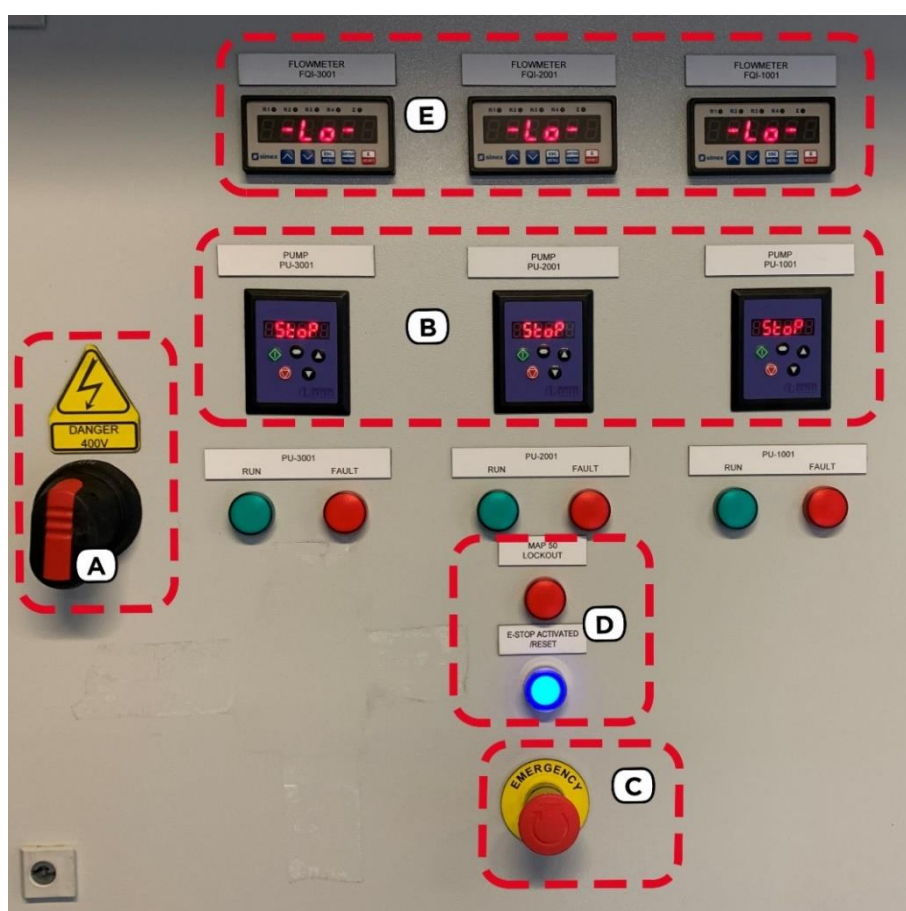
Figure 9: BHM Rig main control panel - A: Main power switch, B: Pump controls, C: Emergency shut off button, D: MAP 50 Lockout, "MAP 50" lockout is on during initial start-up and must be switched off by pressing the "E-stop/reset" button. E: Flow meter controls.
