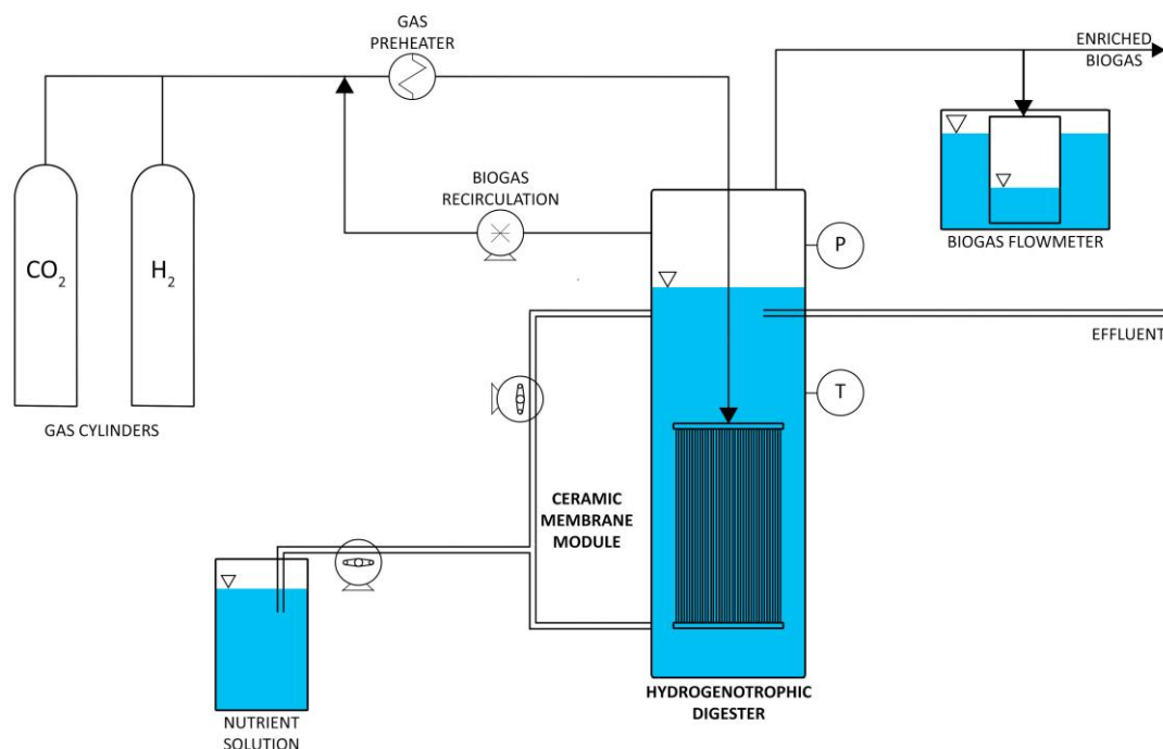
Figure 2.8: Diagram of a membrane bio-reactor experimental set-up.
