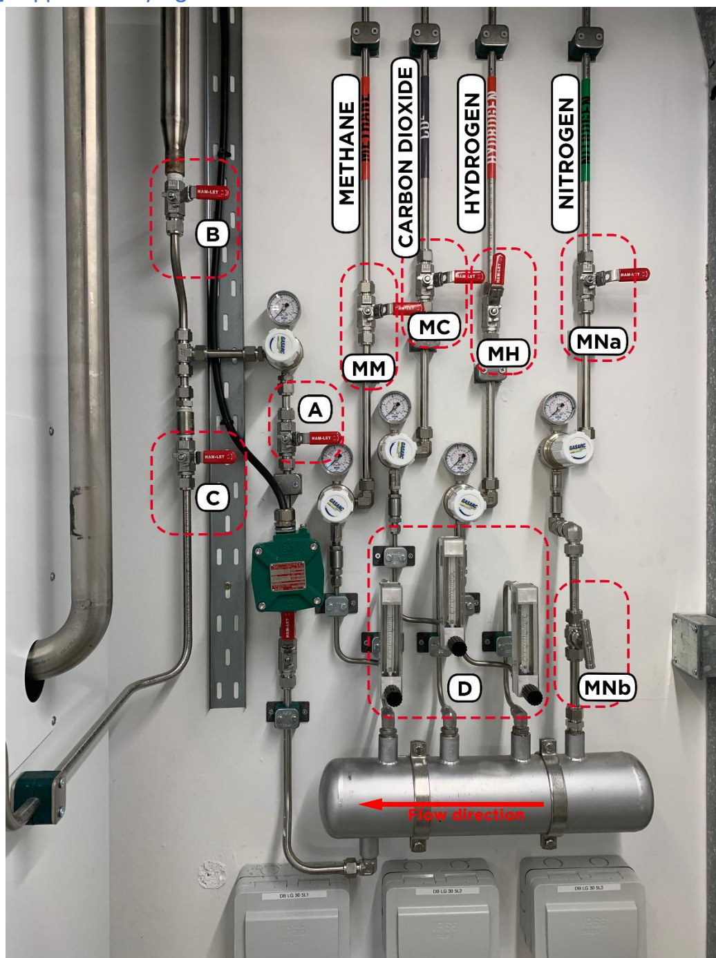
Figure S3.1: The external manifold panel before gas entry into the reactor skid. Where A- Manifold manual Parker A-Lok valve outlet valve (Post-solenoid valve); B- Manual Parker A-Lok valve leading to atmosphere (System by-pass for venting); C- Manual Parker A-Lok valve leading to the system inlet; D- Manual rotameters for methane, hydrogen and carbon dioxide); MO- Manual Parker A-Lok valve for the Manifold outlet (Pre solenoid valve); MM- Manual Parker A-Lok valve for the methane supply; MC- Manual Parker A-Lok valve for the carbon dioxide supply; MH- Manual Parker A-Lok valve for the hydrogen supply; MNa- Manual Parker A-Lok valve for the nitrogen supply; MNb- Needle valve for the regulation of nitrogen supply downstream.
