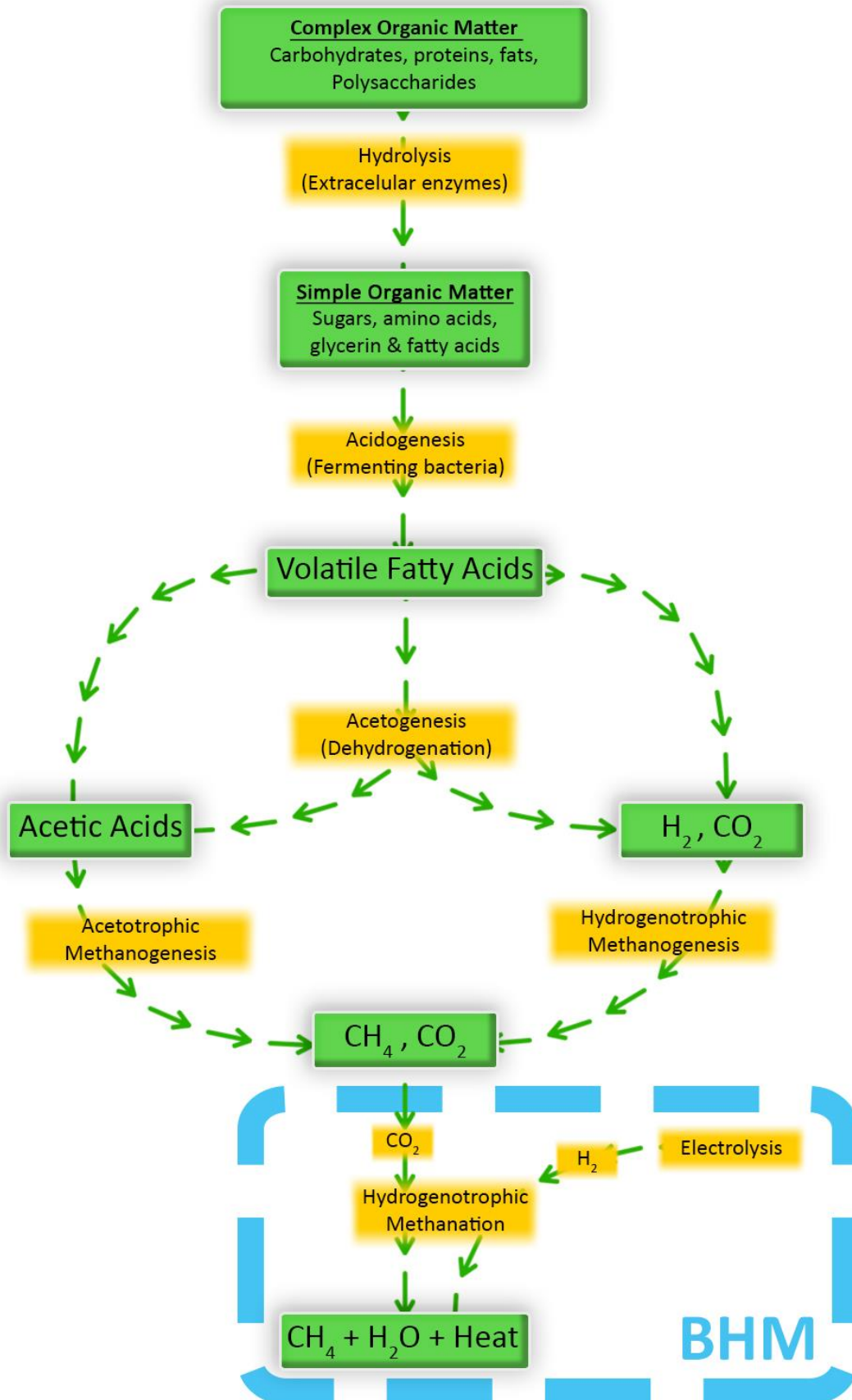
Figure 2.3: \text{CH}_4 formation through anaerobic digestion and biological hydrogen methanation.
