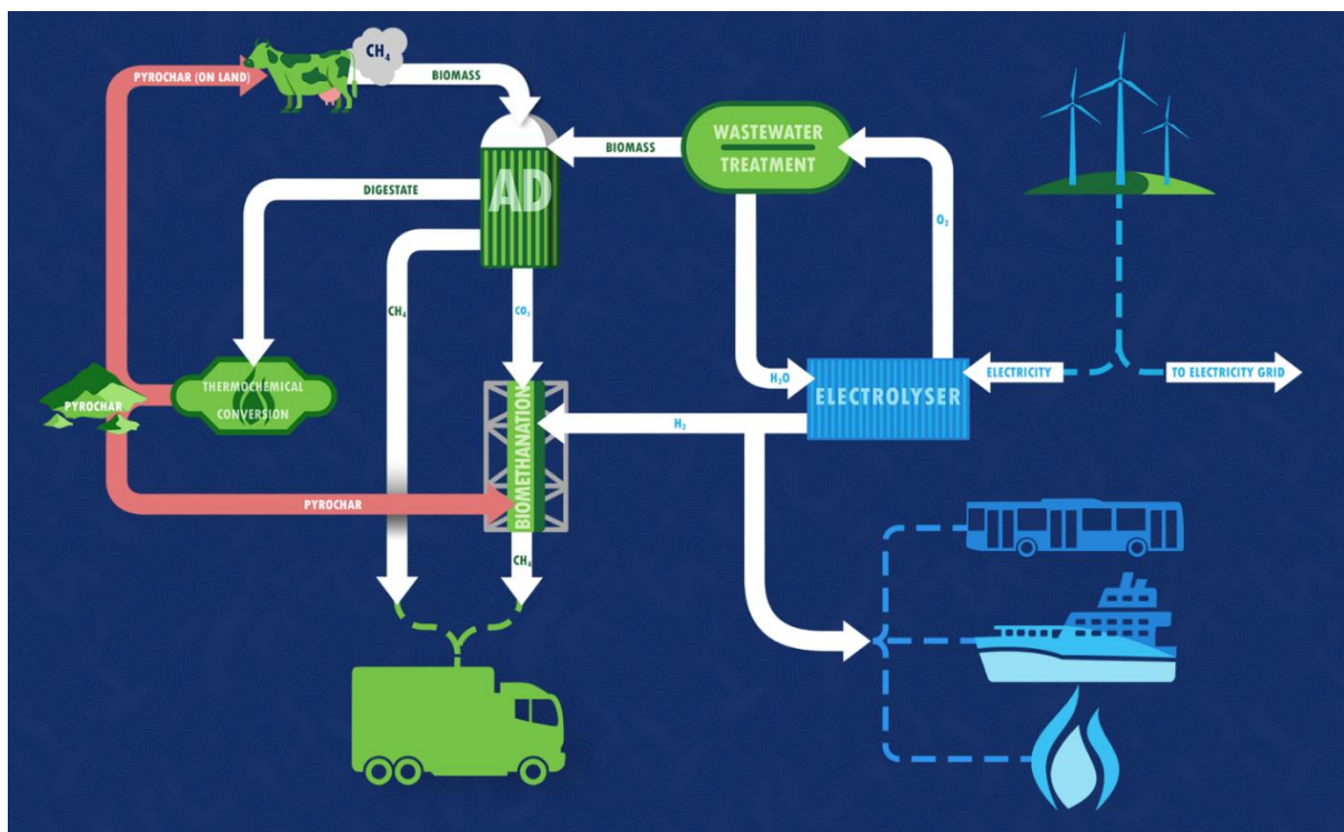
Figure 4.1: The proposed circular electrofuels production system.
