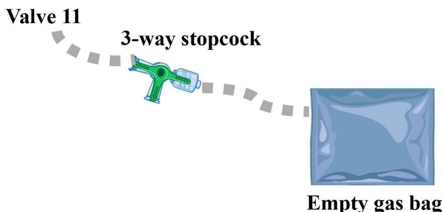
Figure 23: Gas flow measurement arrangement, comprising of an empty foil gas bag of approx. 2L volume (fully deflated), a 3-way stopcock valve and tubing. The empty gas bag is filled with the outflowing gas over a set time interval.
