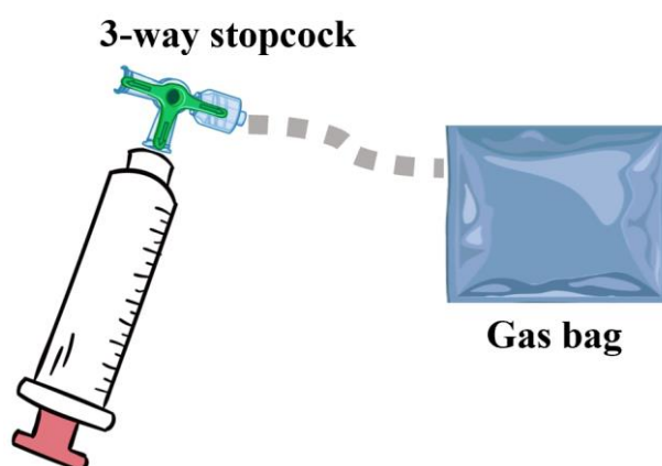
Figure 25: Connected gas tight syringe to the 3-way stopcock and filled gas bag. Syringe is filled and measured repeatedly until the gas bag is empty, giving an accurate volume over the timed period.
