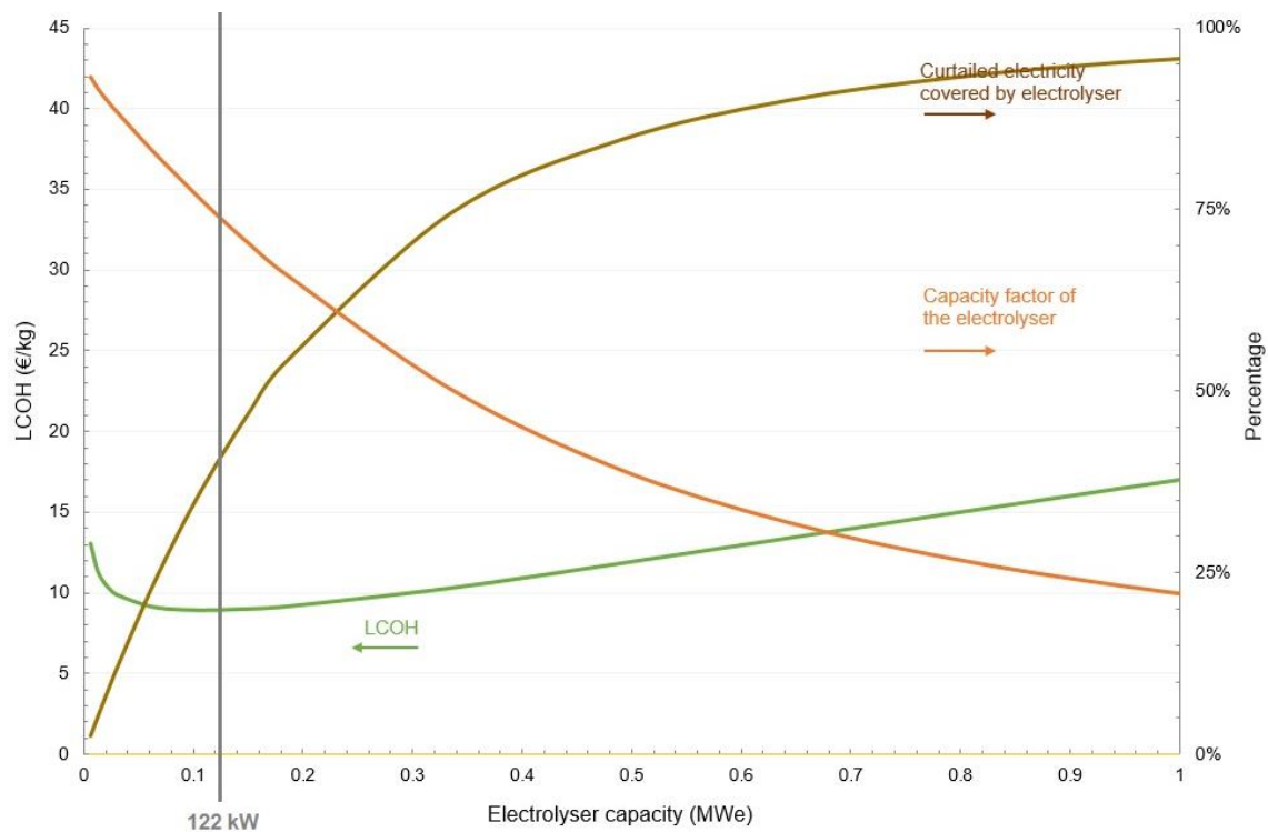
Figure 4.3: Electrolyser capacity and levelized cost of hydrogen. The optimal 122 kW system is represented by a vertical black line intersecting the Capacity Factor curve (orange), the Curtailed Energy Capture curve (brown) and the LCOH curve (green).
