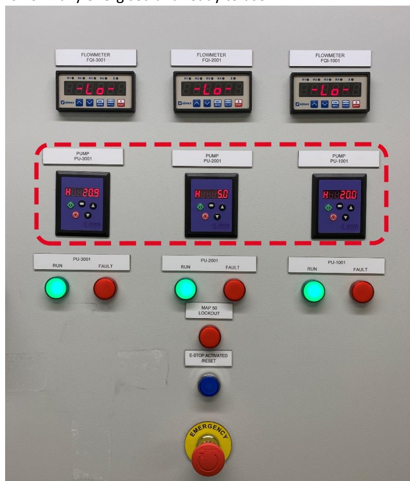
Figure 10: BHM Rig control panel fully operational. Highlighted are pump controls with pumps operating at set speeds.
