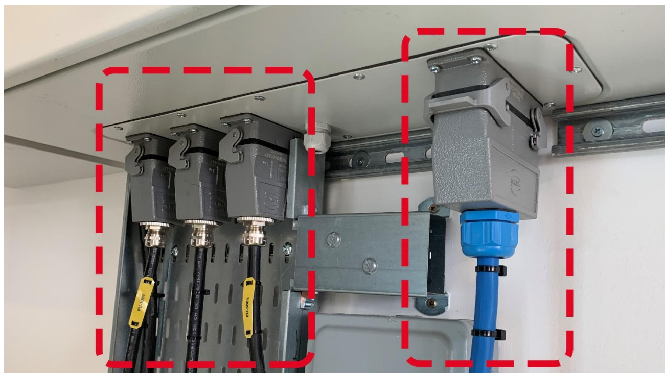
Figure 4: Connected three-phase plugs into the main reactor control box. Black cables labelled as PU-1001, PU-2001 and PU-3001, Blue labelled cable.
