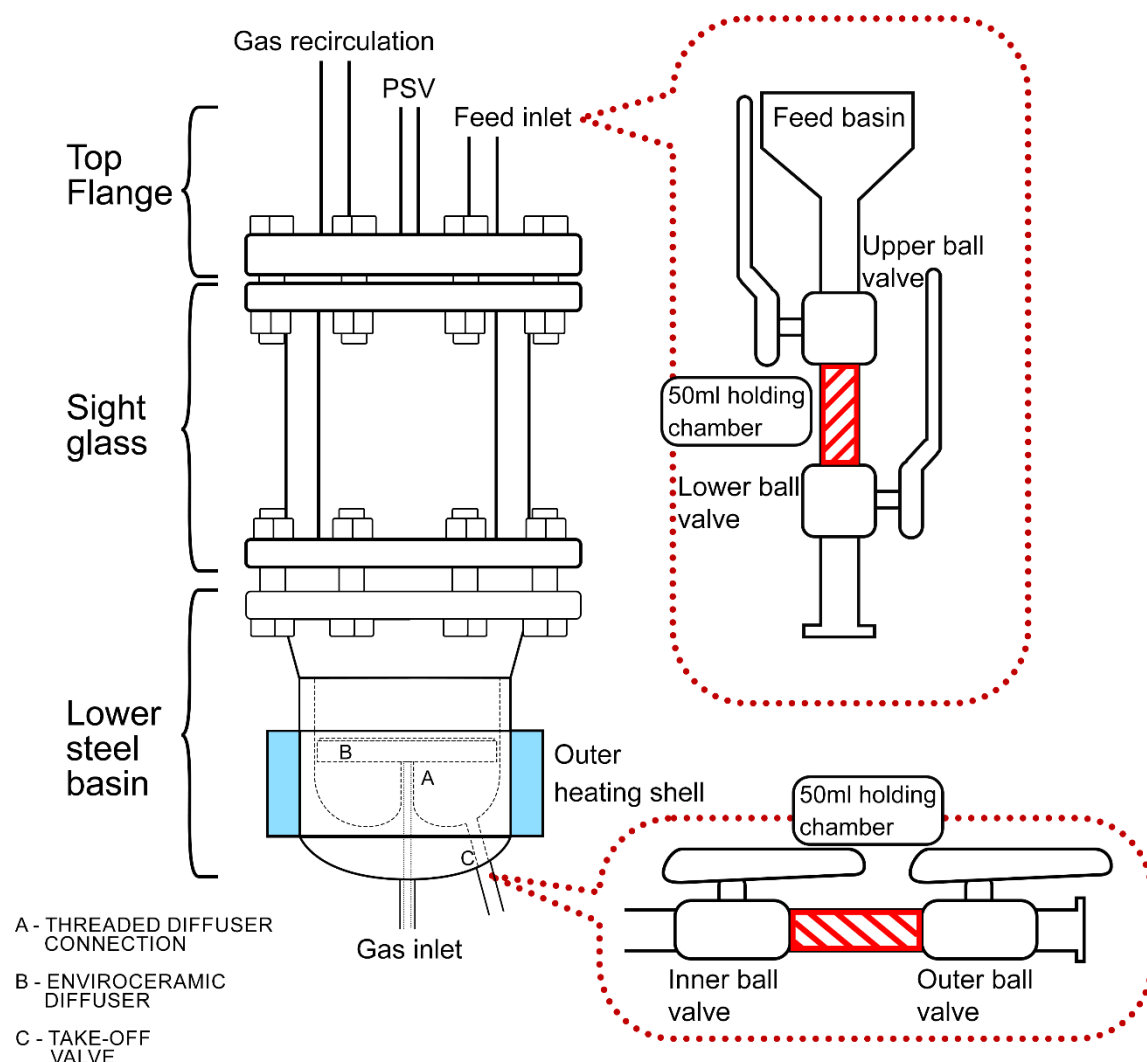
Figure 3.4: Profile of a methanation reactor chamber, where (A) is the threaded diffuser connection, (B) is the “Enviroceramic” diffuser and (C) is the liquid take-off line. PSV – Pressure safety valve.
