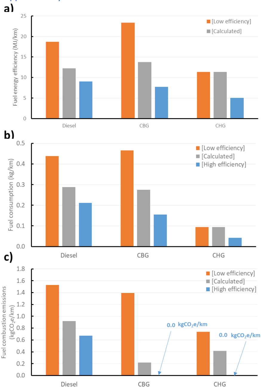
Figure S5.1: Fuel and HGV comparison (Lower is better); a) HGV Tank-to-Wheel efficiency (MJ/km); b) Fuel consumption (kg/km); c) Fuel combustion emissions (kgCO 2 e/km). Adapted from Table S5.1.
