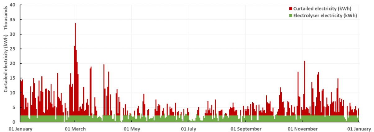
Figure 4.4: Surplus electricity captured by the 122 kW PEM electrolyser at the industrial site.
