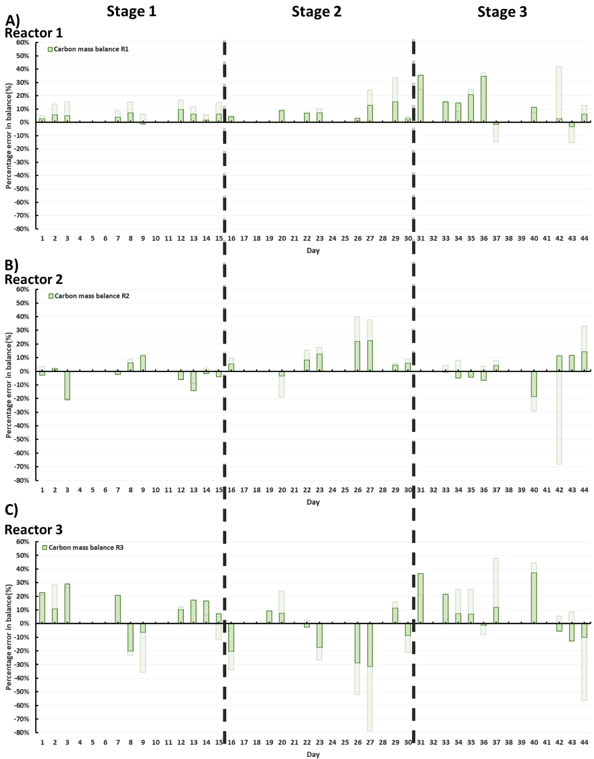
Figure 3.9: Percentage error in the carbon mass balance, across R1, R2 and R3, where; A) Error in balance – Inlet vs. R1 outlet; B) Error in balance – R1 outlet vs. R2 outlet; and C) Error in balance – R2 outlet vs. R3 outlet. Note the faded data columns represent the unadjusted errors in balance, based on Equation 3.7 values. The vertical dashed lines represent the change of flow rate from stages 1-3, as per Table 3.2.
