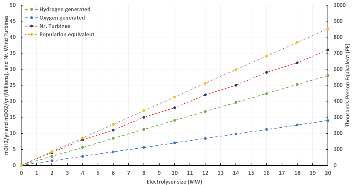
Figure 5.8: Electrolyser size vs H 2 and O 2 generated, and the number of wind turbines (8MW, 10% curtailment) required to supply oxygen to a wastewater treatment plant in an offshore wind (East) scenario.
