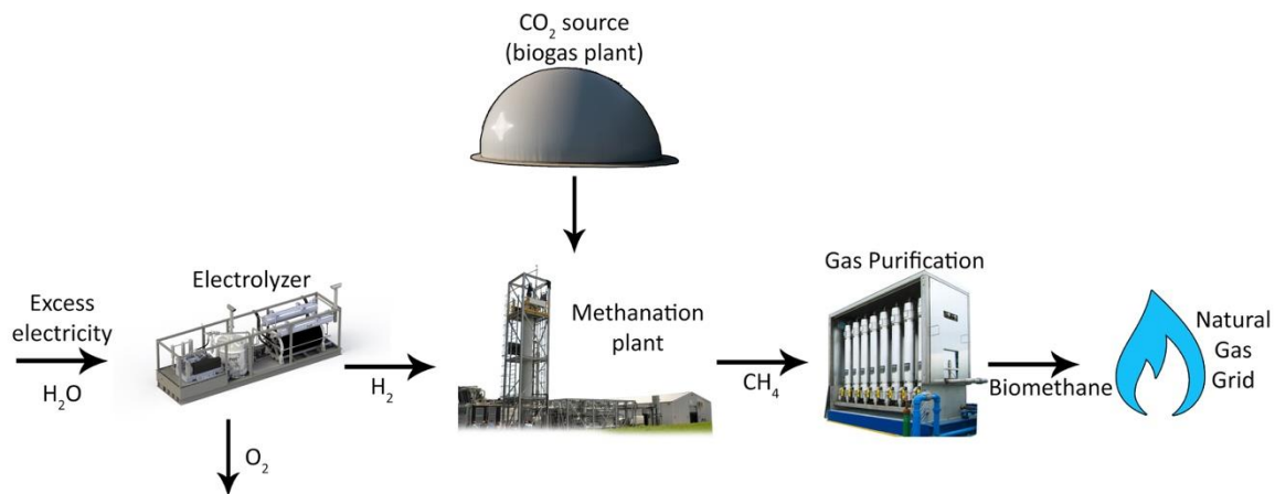
Figure 2.2: Ex-situ biological H_2 methanation schematic.
