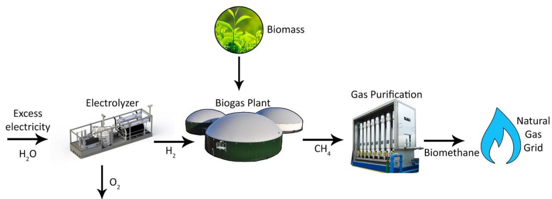
Figure 2.1: In-situ biological H_2 methanation schematic.
