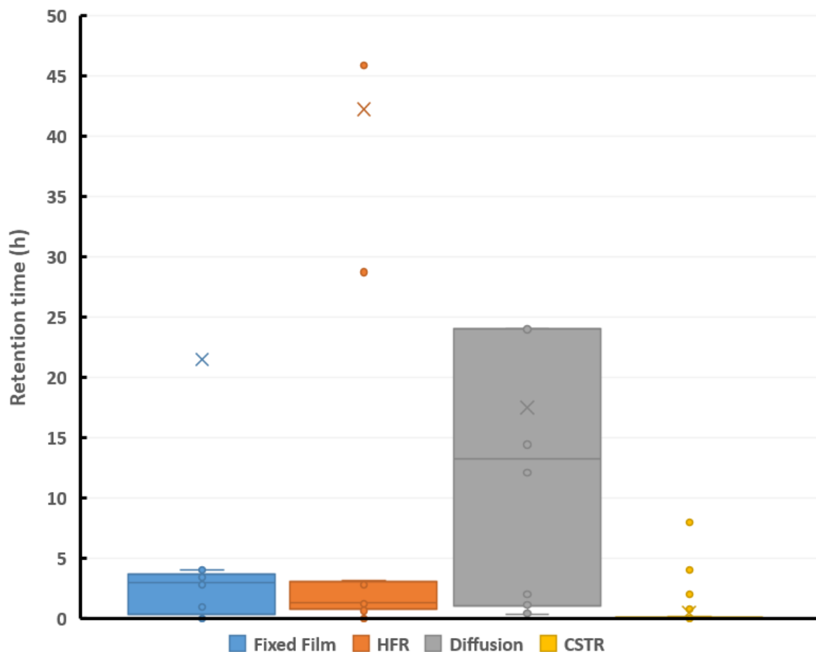
Figure 2.10: Comparison of retention time across reactor systems.
