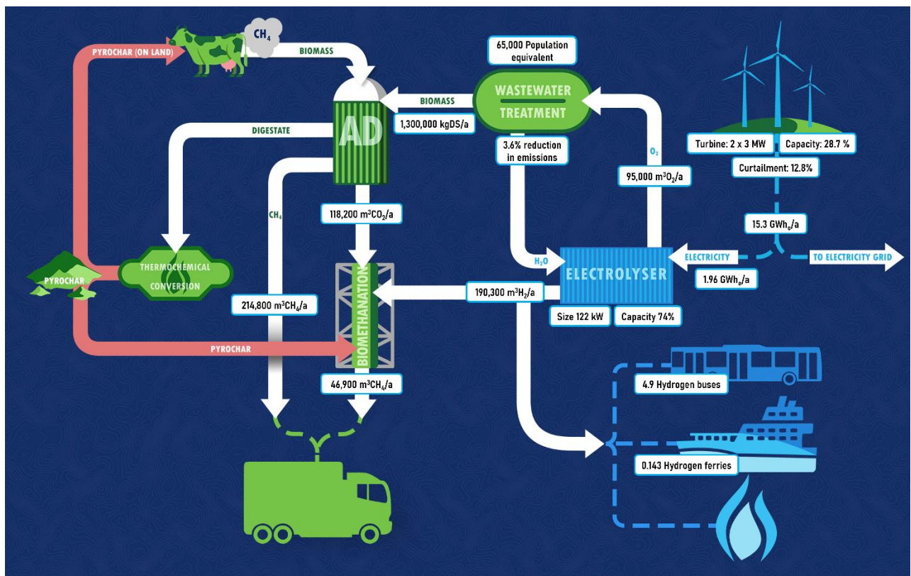
Figure 4.5: Summary flow diagram of the circular economy system at a local industrial site.
