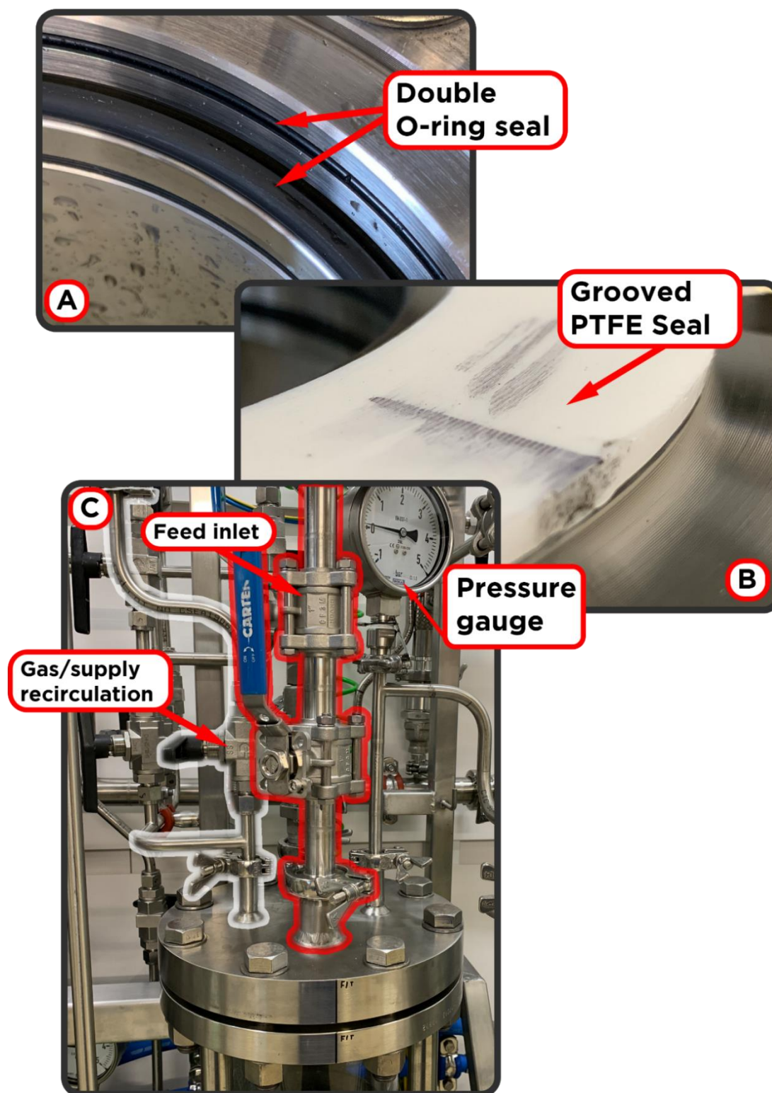
Figure S3.2: Annotated reactor components, where: Image A- Double O-ring seal of the bottom sight glass (identical for top flange); Image B- Grooved PTFE ring seated between two flanges for an airtight seal; Image C- Top flange reactor connections, Supply and gas recirculation lines, feed inlet line and pressure gauge/outlet line. Behind the feed inlet is a pressure safety valve, which cannot be observed in Image C.
