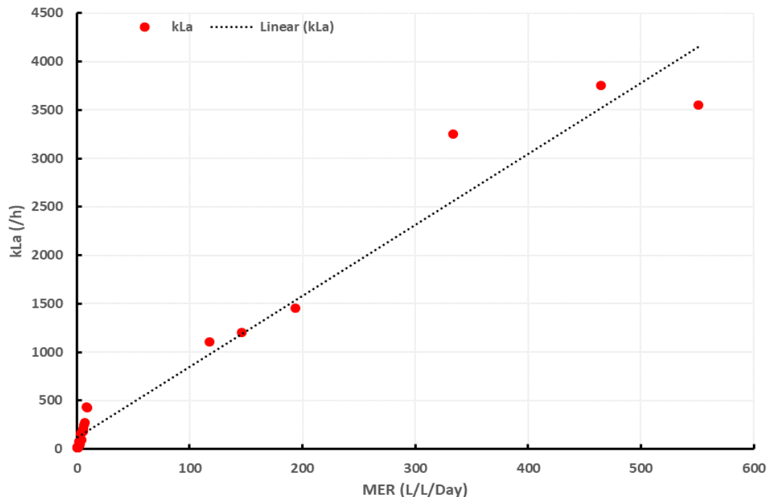
Figure 2.13: Comparison of MER vs k_{La} data in the literature.
