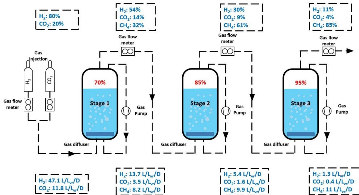
Figure 3.2: The simulated three-stage cascading biomethanation rig, adapted from Voelklein et al. [16]. L/L v /D refers to 'litres per litre-volume-reactor per day'.
