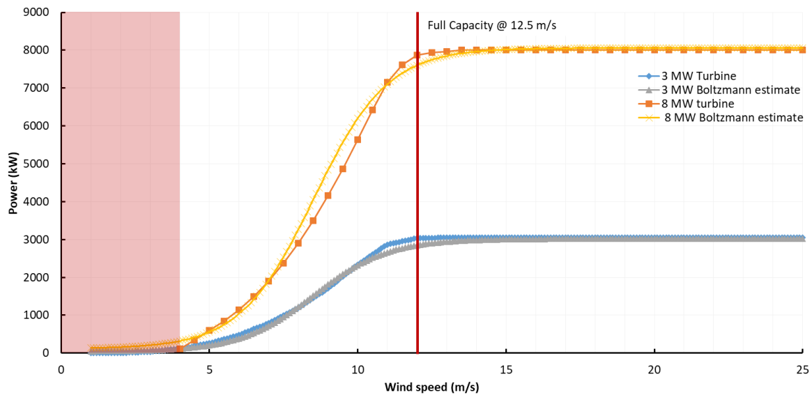
Figure 5.4: Wind turbine power curve compared to the Boltzmann estimate to investigate the estimated reliability.
