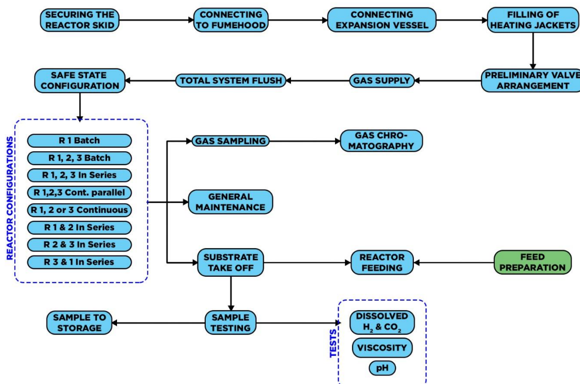
Figure 1: Preliminary procedure flow diagram for Hydrogen reactor skid set-up and operation.
