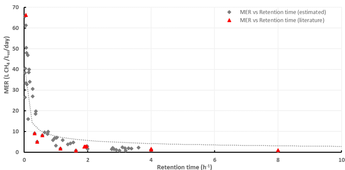
Figure 2.11: Relationship between MER and retention times.
