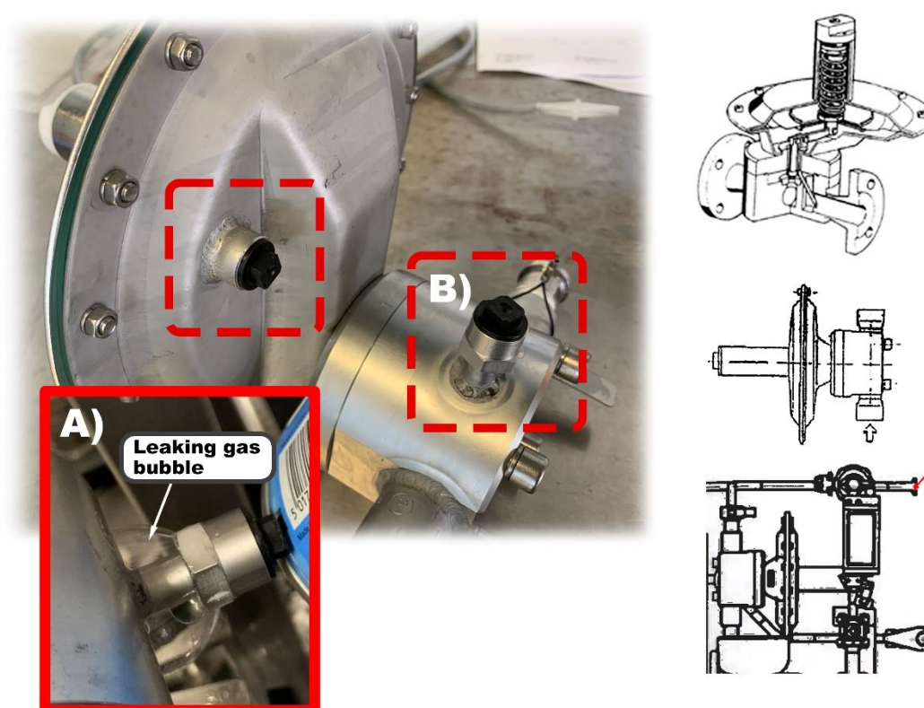
Figure 3.7: a) Image of leaking “nozzle” on the pressure indication and control valve. A bubble has formed by the use of a leak detector spray to reveal the leak. b) The leaking ‘nozzle’ is absent from the manual and general arrangement drawings.
