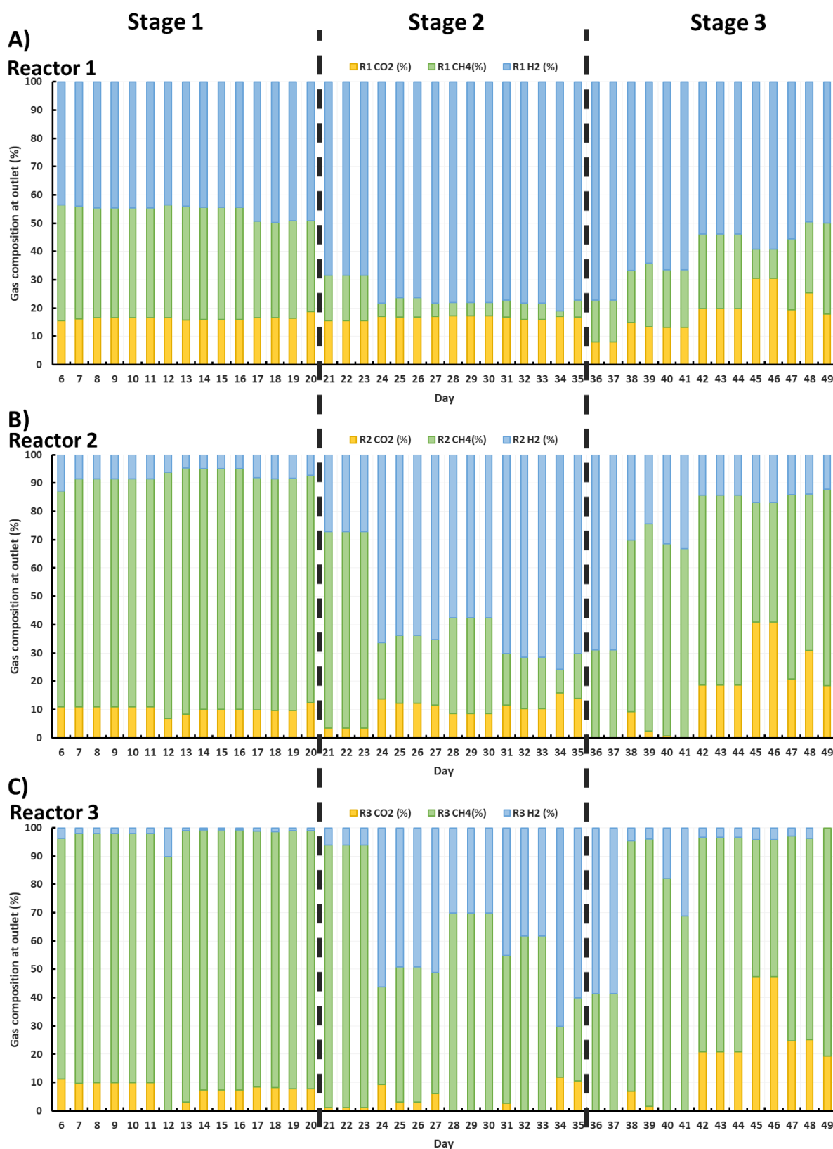
Figure S3.3: Gas composition across R1 (A), R2(B), and R3 (C). Where the reactor was shut off, or gas composition was not measured (e.g. weekends), gas composition from the previous day was substituted for better visualisation.
