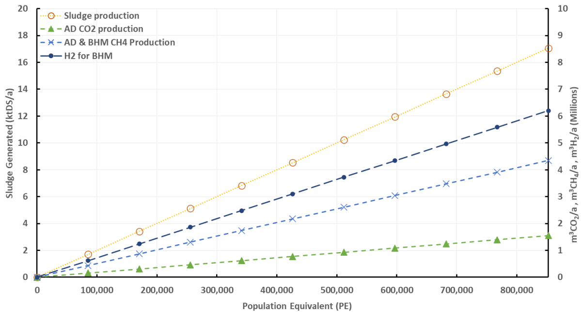
Figure 5.10: WWTP PE relationship to sludge generated, and resultant m^3 CH_4 and CO_2 produced from the digestion of sludge.
