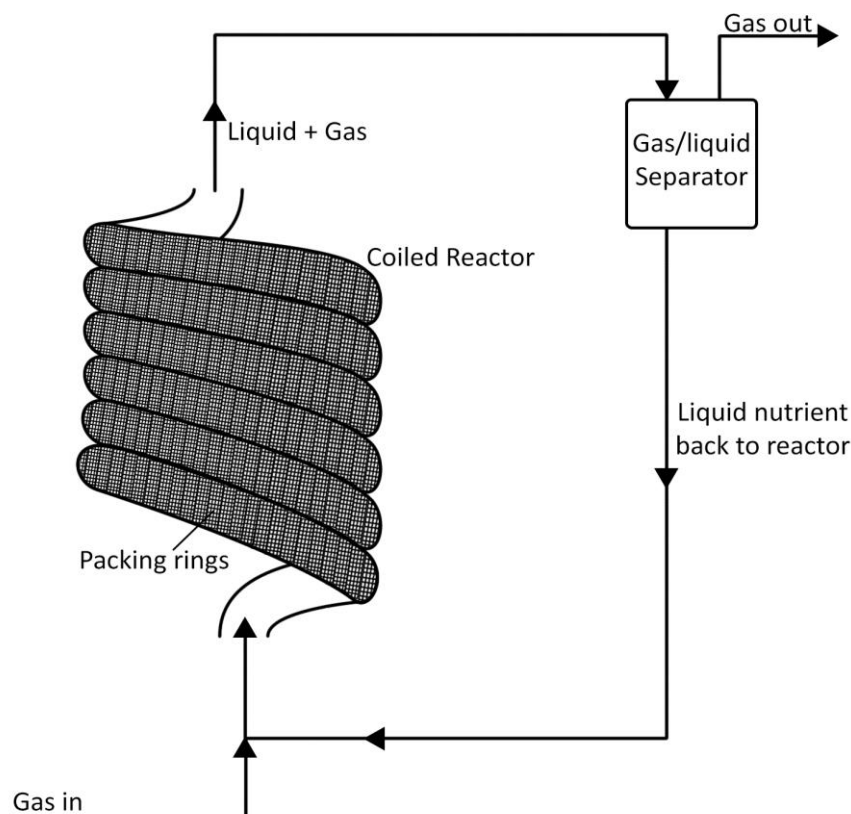
Figure 2.7: A novel BHM system using a tubular reactor setup of narrow diameter pipe and packed fixed biofilm.
