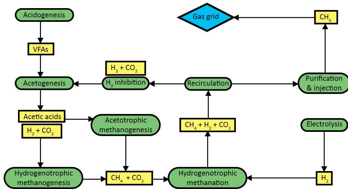
Figure 2.4: In-situ methanation failure process flow diagram.
