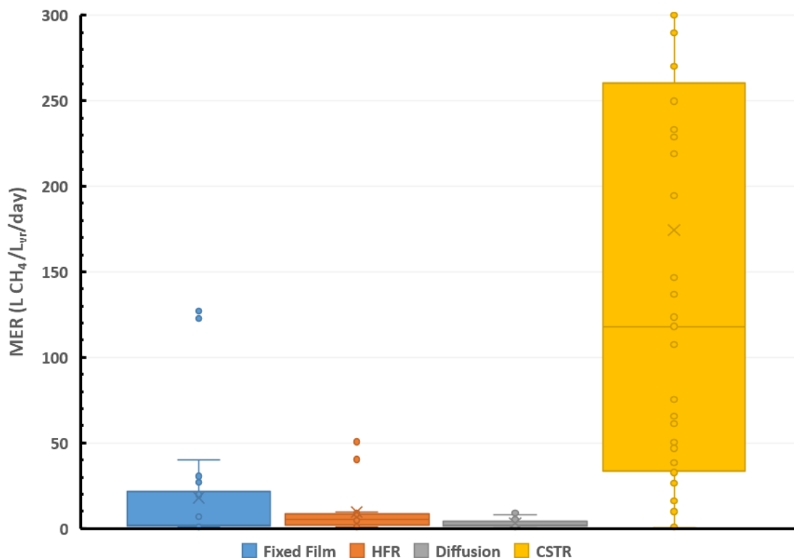
Figure 2.9: Comparison of MER across reactor systems.
