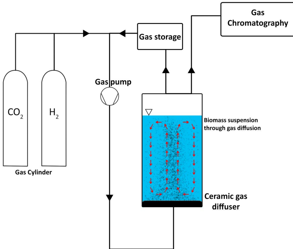
Figure 2.5: Modified CSTR with a ceramic diffuser base.
