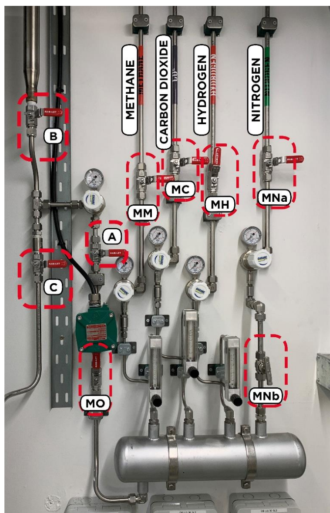
Figure 11: Labelled fume hood external lines supply and manifold.
