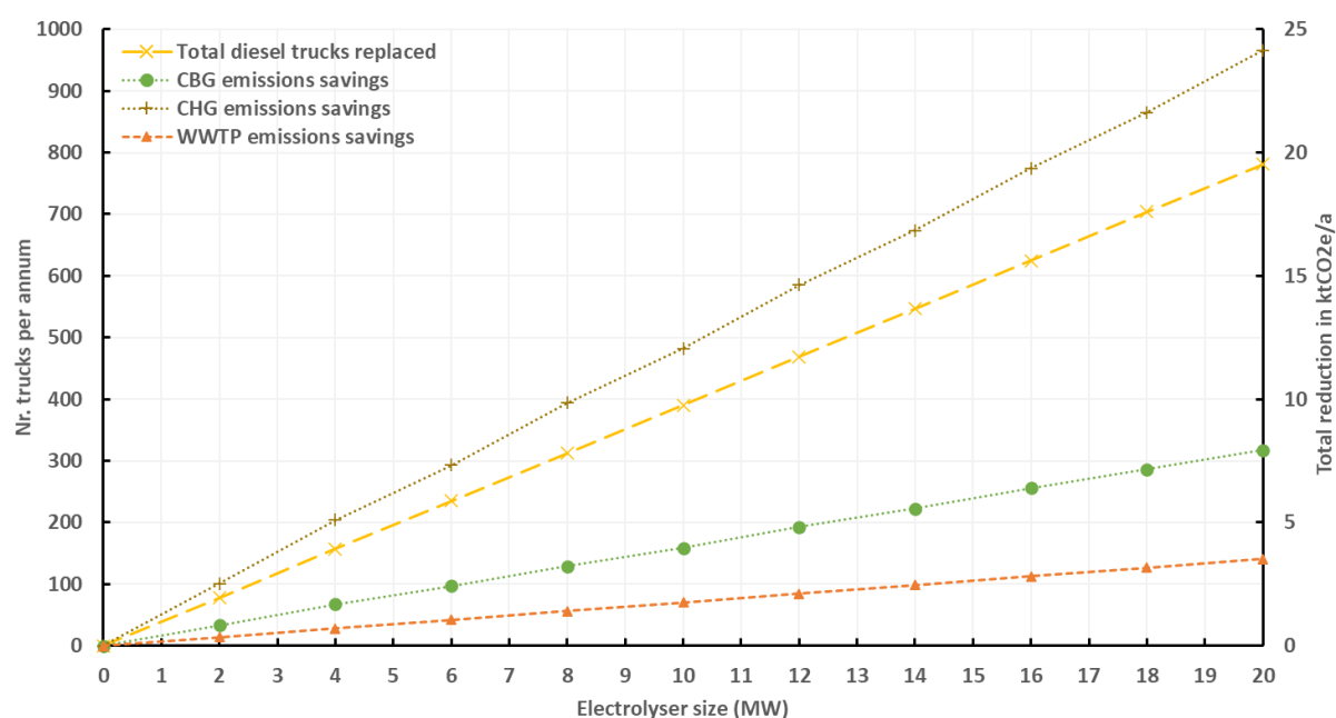
Figure 5.11: Relationship of electrolyser size to the number of diesel trucks replaced, emission savings using biomethane (CBG) and hydrogen (CHG) trucks in units of ktCO 2e /a and the WWTP emission reductions (ktCO 2e /a) due to the switch to pure O 2 .
