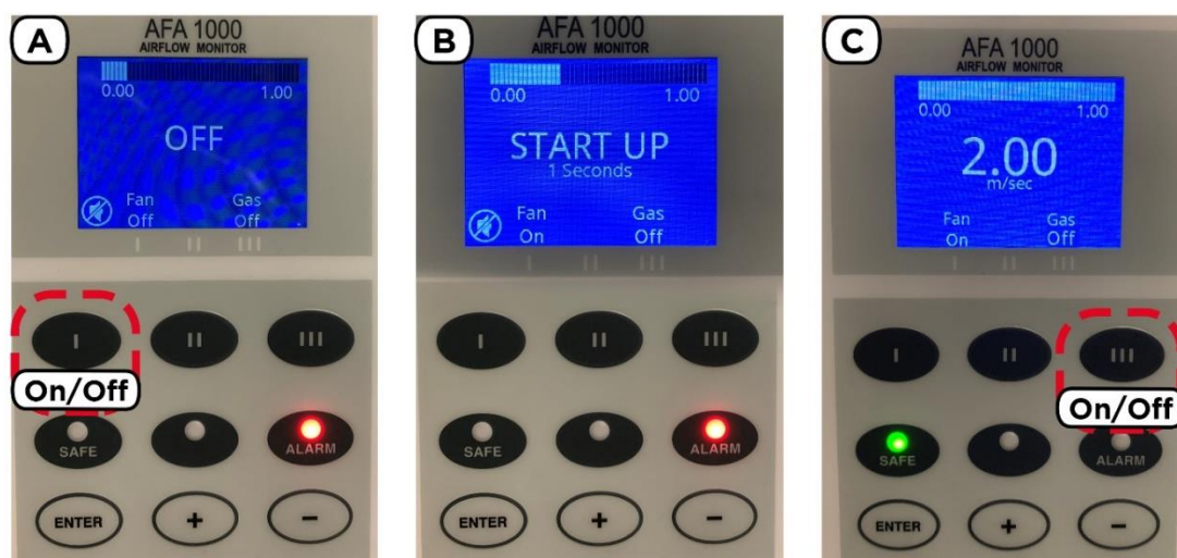
Figure 8: (a) Fume hood control panel with fan and gas off after switching on the breaker. (b) Control panel with the fan in the start-up sequence. (c) Fume hood operating and ready to receive a gas supply. Button highlighted in (c) for gas supply switch.
