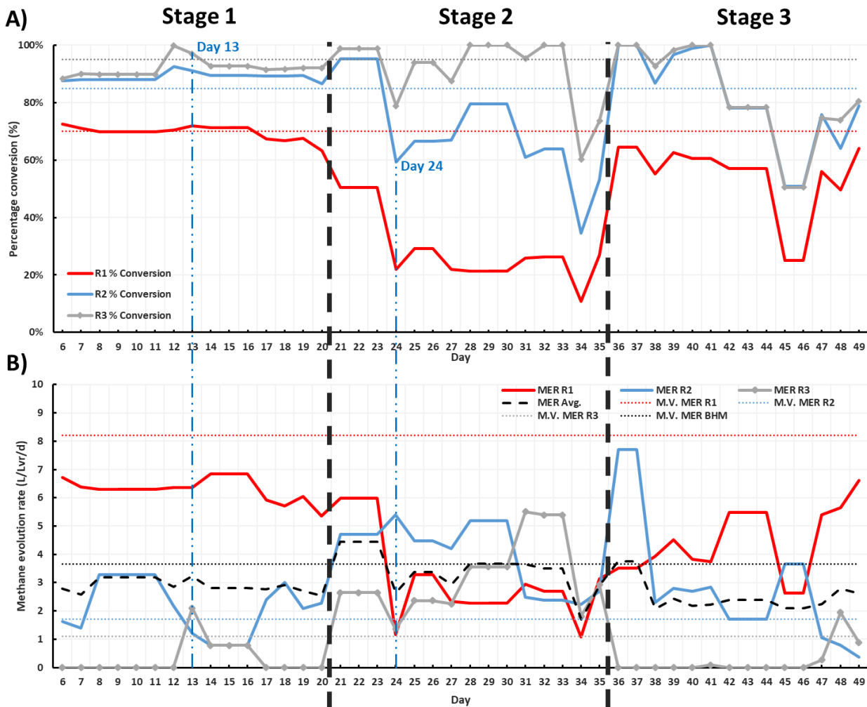
Figure 3.5: A) Percentage conversion of CO 2 in reactors 1 (red), 2 (blue) and 3 (grey). B) Methane Evolution Rates (MER); Dotted lines of respective colours indicate the peak performance of the simulated cascading system by Voelklein et al., the black dotted line denotes the average MER of the system, and the vertical dashed lines represent that change of flowrate from stages 1-3, as per Table 3.1 [16]. Days 13 and 24 are highlighted, indicating the data discussed earlier.
